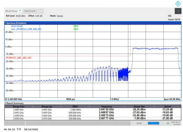
NTNV-n77(3450-3550)-PC2-30-20-L-DFT-BPSK-Outer_Full-PASS
