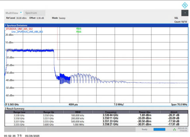
NTNV-n77(3450-3550)-PC2-30-20-H-DFT-BPSK-Outer_Full-PASS
