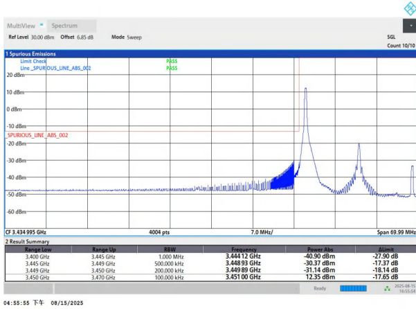
NTNV-n77(3450-3550)-PC2-30-20-L-DFT-BPSK-Edge_1RB_Left-PASS
