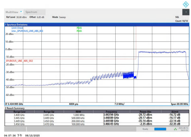
NTNV-n77(3450-3550)-PC2-30-20-L-DFT-QPSK-Outer_Full-PASS
