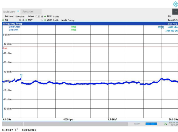
NTNV-n77(3450-3550)-PC2-30-30-M-DFT-QPSK-Edge_1RB_Left -6000-20000-PASS
