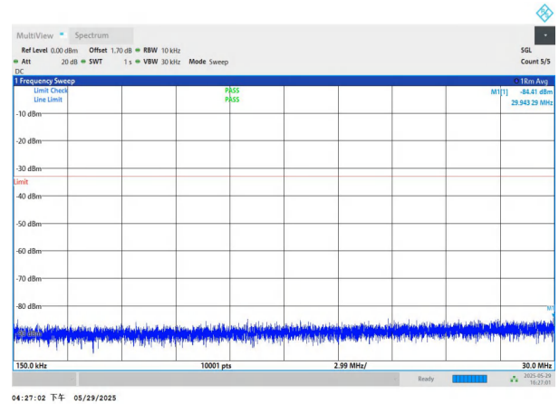
NTNV-n77(3450-3550)-PC2-30-40-M-DFT-BPSK-Edge_1RB_Left -0.15-30-PASS
