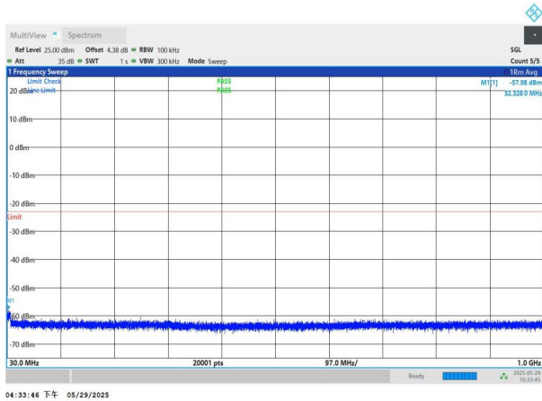
NTNV-n77(3450-3550)-PC2-30-60-L-DFT-BPSK-Edge_1RB_Left- 30-1000-PASS
