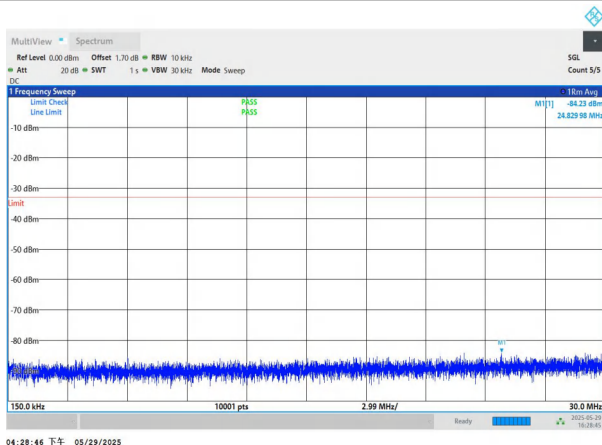
NTNV-n77(3450-3550)-PC2-30-40-M-DFT-QPSK-Edge_1RB_Left -0.15-30-PASS
