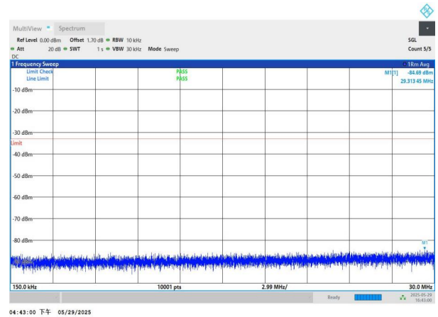
NTNV-n77(3450-3550)-PC2-30-80-L-DFT-BPSK-Edge_1RB_Left- 0.15-30-PASS
