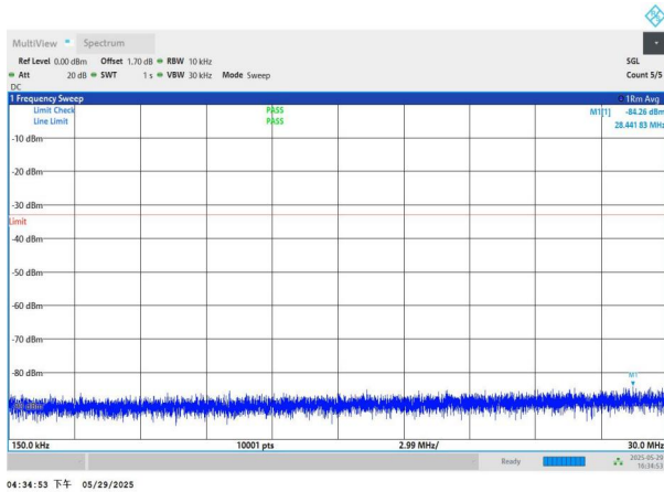
NTNV-n77(3450-3550)-PC2-30-60-L-DFT-QPSK-Edge_1RB_Left- 0.15-30-PASS
