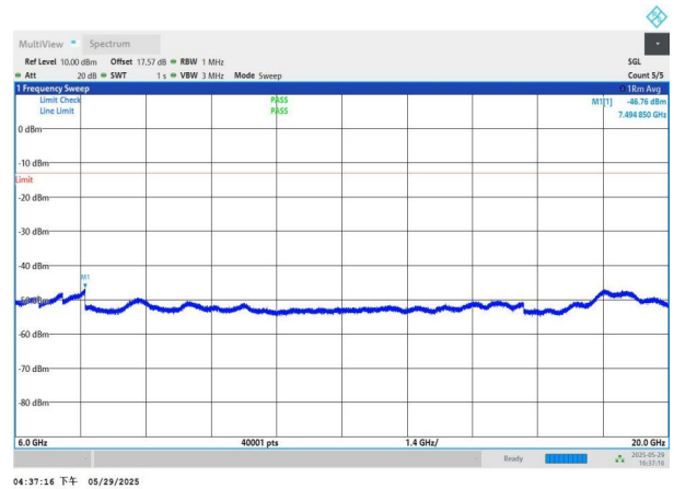
NTNV-n77(3450-3550)-PC2-30-60-M-DFT-BPSK-Edge_1RB_Left -6000-20000-PASS
