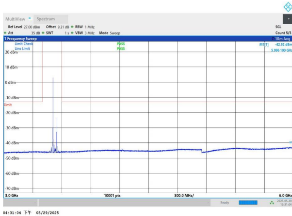
NTNV-n77(3450-3550)-PC2-30-40-H-DFT-BPSK-Edge_1RB_Left -3000-6000-PASS
