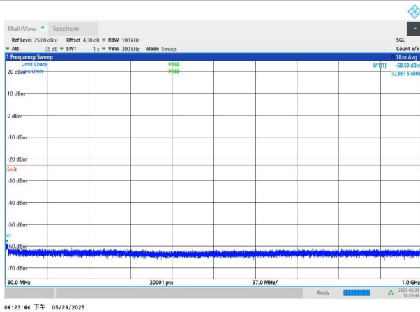
NTNV-n77(3450-3550)-PC2-30-40-L-DFT-BPSK-Edge_1RB_Left- 30-1000-PASS
