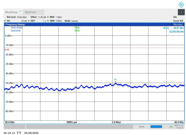
NTNV-n77(3450-3550)-PC2-30-30-L-DFT-QPSK-Edge_1RB_Left- 20000-40000-PASS
