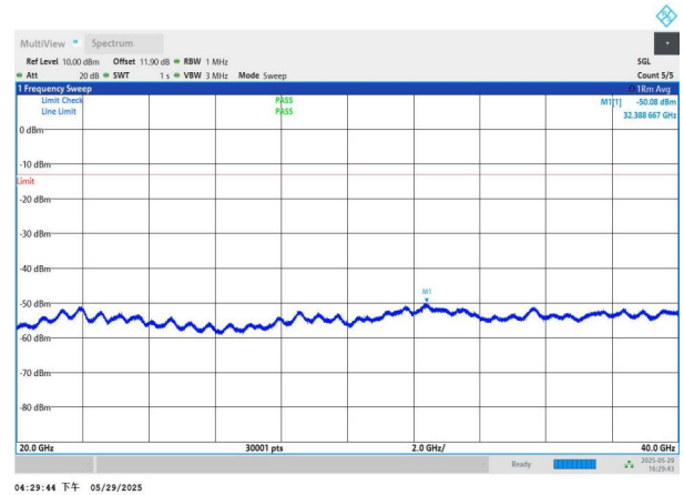
NTNV-n77(3450-3550)-PC2-30-40-M-DFT-QPSK-Edge_1RB_Left -20000-40000-PASS
