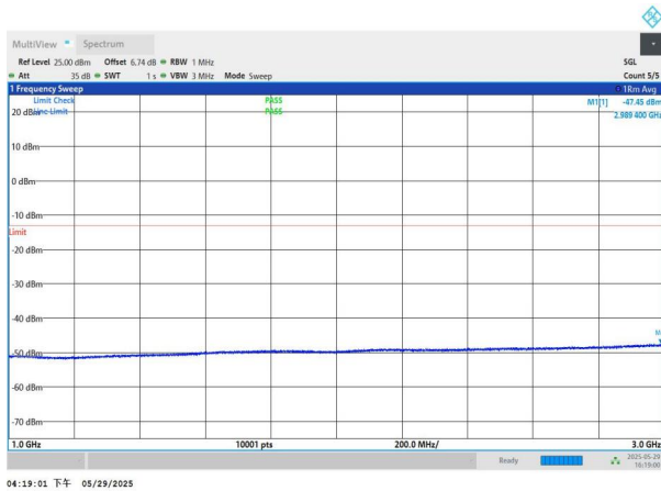
NTNV-n77(3450-3550)-PC2-30-30-M-DFT-QPSK-Edge_1RB_Left -1000-3000-PASS
