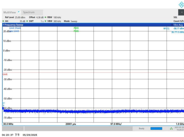
NTNV-n77(3450-3550)-PC2-30-30-H-DFT-BPSK-Edge_1RB_Left -30-1000-PASS
