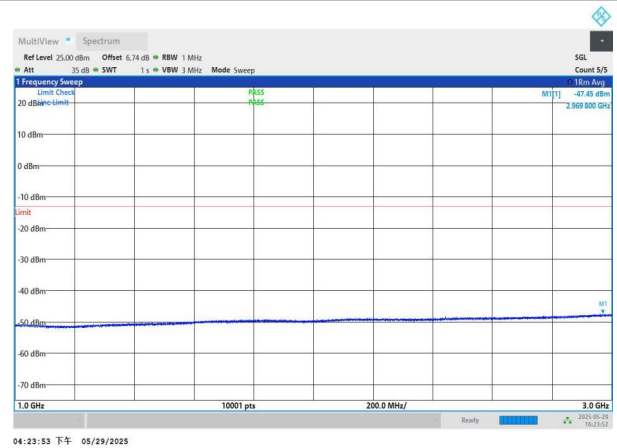
NTNV-n77(3450-3550)-PC2-30-40-L-DFT-BPSK-Edge_1RB_Left- 1000-3000-PASS
