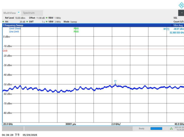
NTNV-n77(3450-3550)-PC2-30-60-L-DFT-BPSK-Edge_1RB_Left- 20000-40000-PASS
