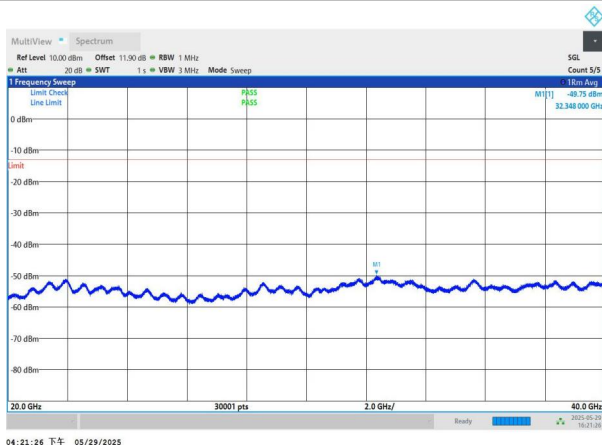
NTNV-n77(3450-3550)-PC2-30-30-H-DFT-BPSK-Edge_1RB_Left -20000-40000-PASS
