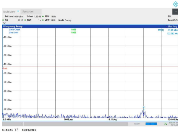
NTNV-n77(3450-3550)-PC2-30-30-M-DFT-BPSK-Edge_1RB_Left -0.009-0.15-PASS
