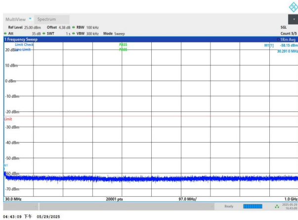
NTNV-n77(3450-3550)-PC2-30-80-L-DFT-BPSK-Edge_1RB_Left- 30-1000-PASS
