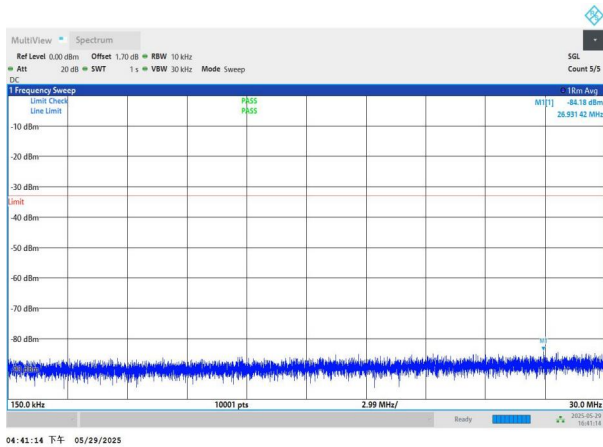
NTNV-n77(3450-3550)-PC2-30-60-H-DFT-QPSK-Edge_1RB_Left -0.15-30-PASS
