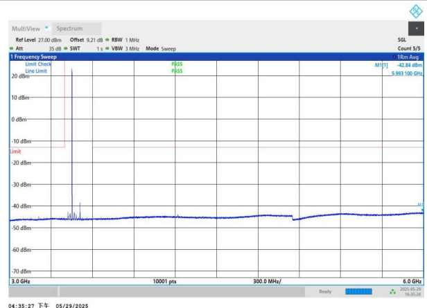
NTNV-n77(3450-3550)-PC2-30-60-L-DFT-QPSK-Edge_1RB_Left- 3000-6000-PASS
