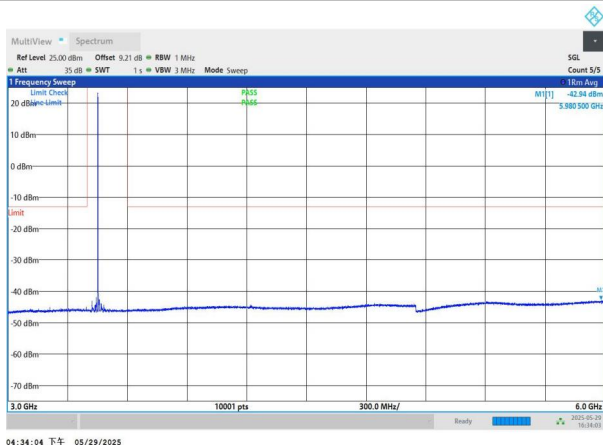
NTNV-n77(3450-3550)-PC2-30-60-L-DFT-BPSK-Edge_1RB_Left- 3000-6000-PASS
