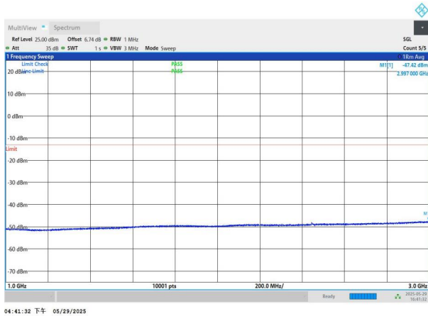
NTNV-n77(3450-3550)-PC2-30-60-H-DFT-QPSK-Edge_1RB_Left -1000-3000-PASS
