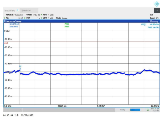
NTNV-n77(3450-3550)-PC2-30-30-M-DFT-BPSK-Edge_1RB_Left -6000-20000-PASS
