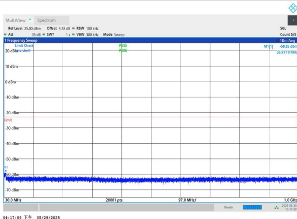
NTNV-n77(3450-3550)-PC2-30-30-M-DFT-BPSK-Edge_1RB_Left -30-1000-PASS
