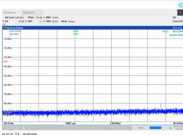
NTNV-n77(3450-3550)-PC2-30-60-M-DFT-QPSK-Edge_1RB_Left -0.15-30-PASS
