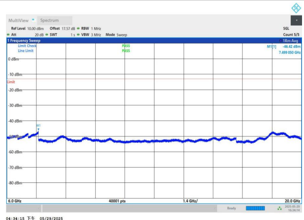
NTNV-n77(3450-3550)-PC2-30-60-L-DFT-BPSK-Edge_1RB_Left- 6000-20000-PASS
