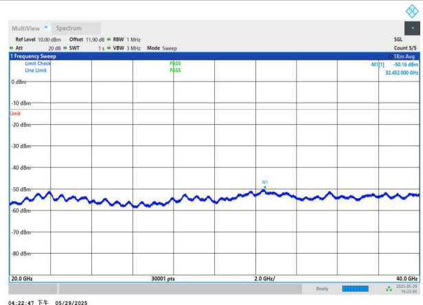
NTNV-n77(3450-3550)-PC2-30-30-H-DFT-QPSK-Edge_1RB_Left -20000-40000-PASS
