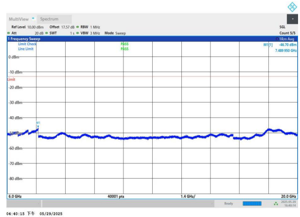
NTNV-n77(3450-3550)-PC2-30-60-H-DFT-BPSK-Edge_1RB_Left 6000-20000-PASS
