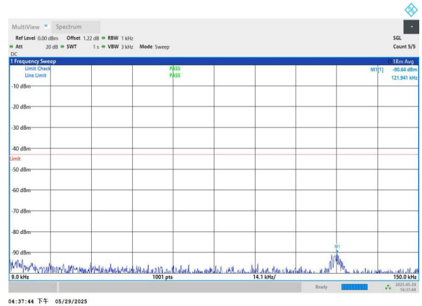
NTNV-n77(3450-3550)-PC2-30-60-M-DFT-QPSK-Edge_1RB_Left -0.009-0.15-PASS
