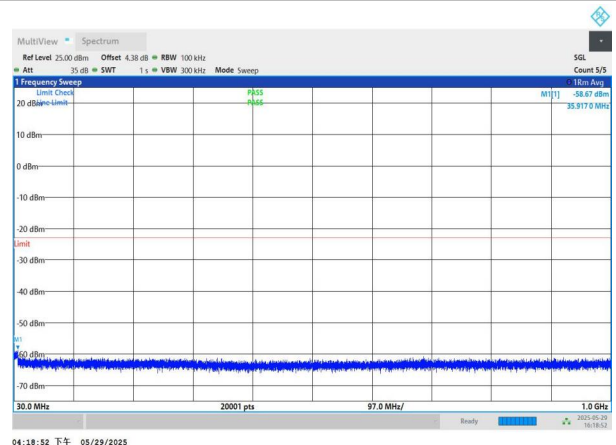
NTNV-n77(3450-3550)-PC2-30-30-M-DFT-QPSK-Edge_1RB_Left -30-1000-PASS
