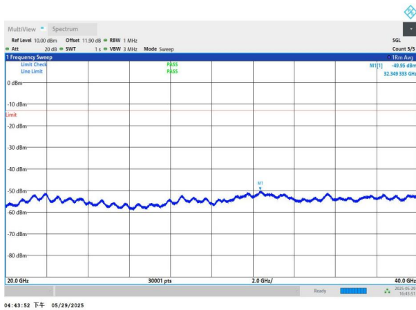
NTNV-n77(3450-3550)-PC2-30-80-L-DFT-BPSK-Edge_1RB_Left- 20000-40000-PASS
