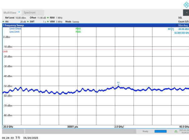
NTNV-n77(3450-3550)-PC2-30-40-L-DFT-BPSK-Edge_1RB_Left- 20000-40000-PASS
