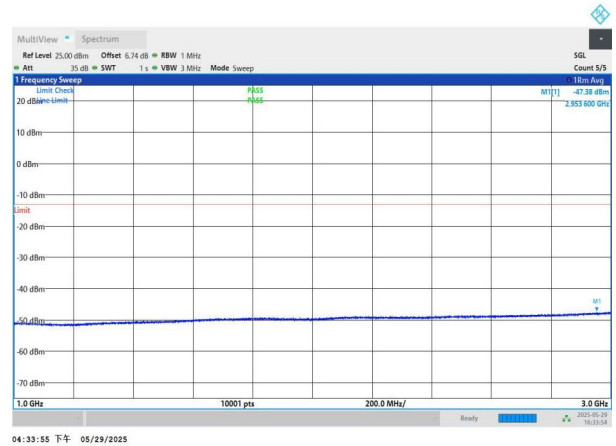
NTNV-n77(3450-3550)-PC2-30-60-L-DFT-BPSK-Edge_1RB_Left- 1000-3000-PASS
