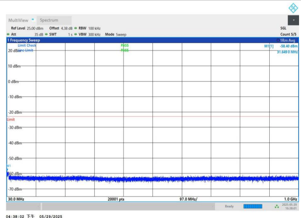
NTNV-n77(3450-3550)-PC2-30-60-M-DFT-QPSK-Edge_1RB_Left -30-1000-PASS
