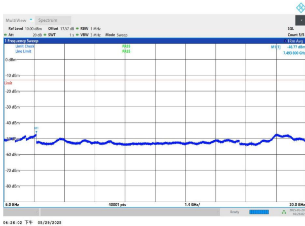
NTNV-n77(3450-3550)-PC2-30-40-L-DFT-QPSK-Edge_1RB_Left- 6000-20000-PASS
