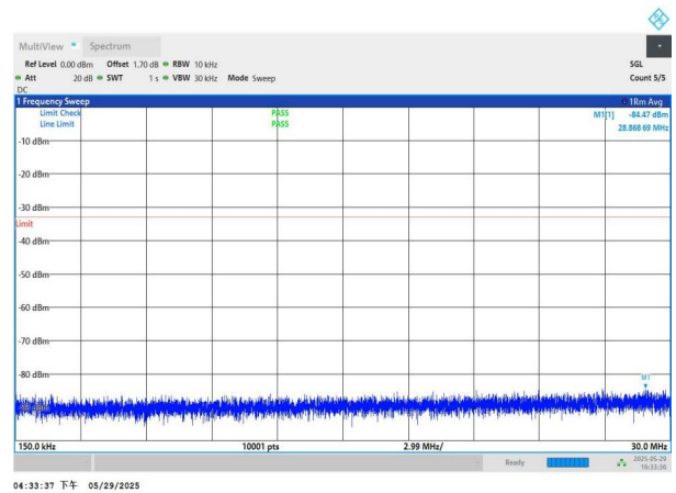
NTNV-n77(3450-3550)-PC2-30-60-L-DFT-BPSK-Edge_1RB_Left- 0.15-30-PASS
