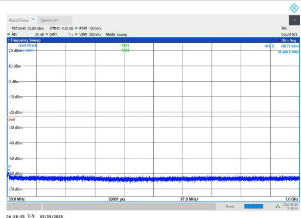
NTNV-n77(3450-3550)-PC2-30-40-M-DFT-QPSK-Edge_1RB_Left -30-1000-PASS
