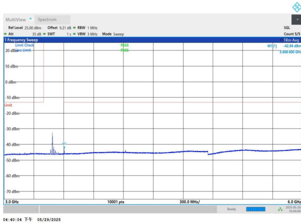
NTNV-n77(3450-3550)-PC2-30-60-H-DFT-BPSK-Edge_1RB_Left -3000-6000-PASS
