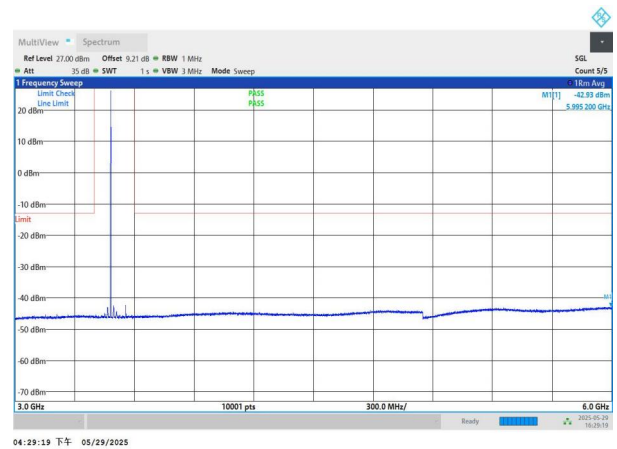
NTNV-n77(3450-3550)-PC2-30-40-M-DFT-QPSK-Edge_1RB_Left -3000-6000-PASS
