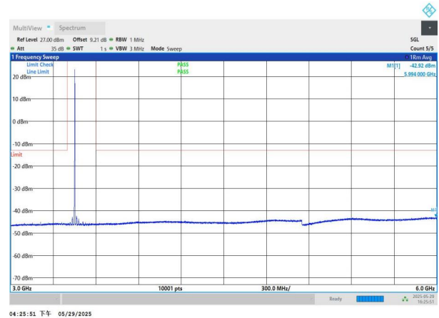
NTNV-n77(3450-3550)-PC2-30-40-L-DFT-QPSK-Edge_1RB_Left- 3000-6000-PASS
