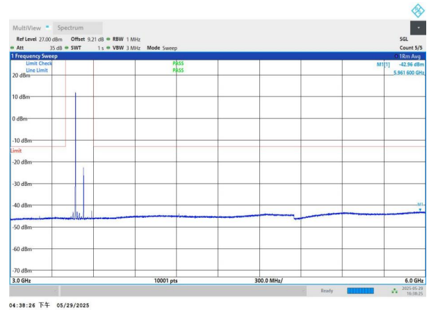
NTNV-n77(3450-3550)-PC2-30-60-M-DFT-QPSK-Edge_1RB_Left -3000-6000-PASS
