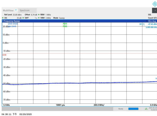
NTNV-n77(3450-3550)-PC2-30-60-M-DFT-QPSK-Edge_1RB_Left -1000-3000-PASS
