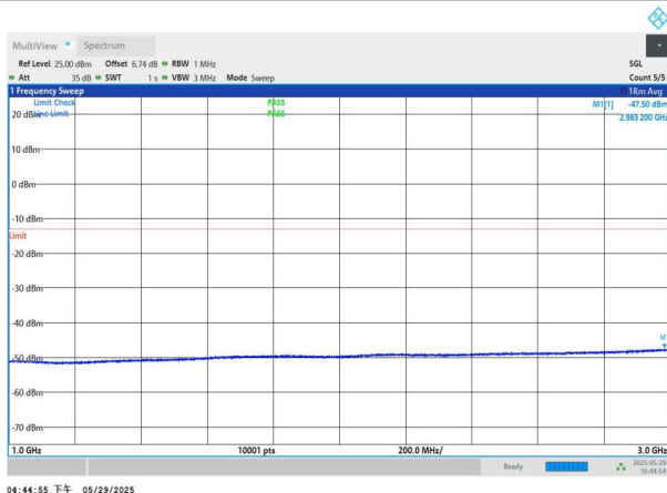
NTNV-n77(3450-3550)-PC2-30-80-L-DFT-QPSK-Edge_1RB_Left- 1000-3000-PASS
