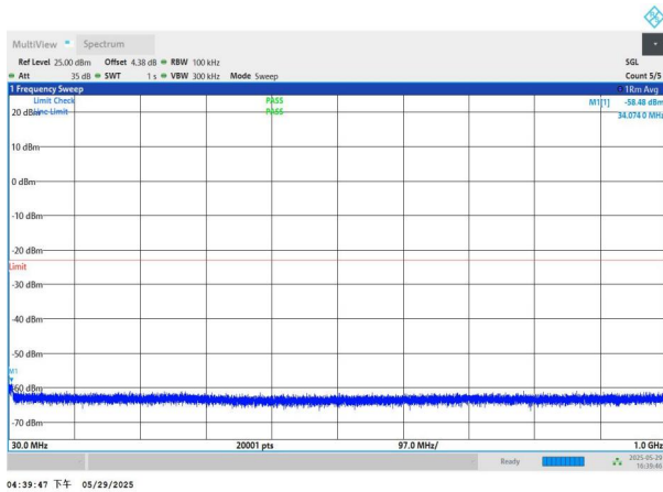
NTNV-n77(3450-3550)-PC2-30-60-H-DFT-BPSK-Edge_1RB_Left -30-1000-PASS
