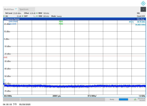
NTNV-n77(3450-3550)-PC2-30-60-L-DFT-QPSK-Edge_1RB_Left- 30-1000-PASS
