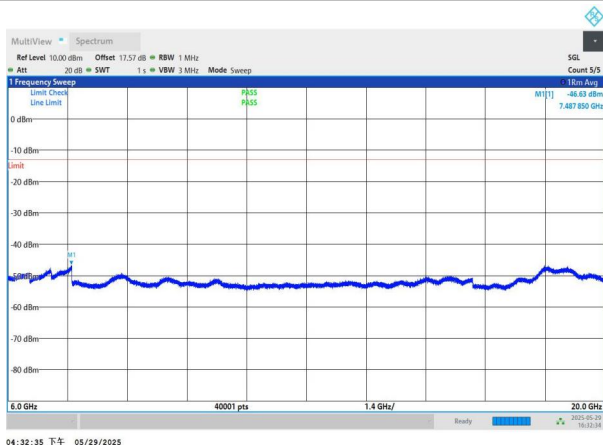
NTNV-n77(3450-3550)-PC2-30-40-H-DFT-QPSK-Edge_1RB_Left -6000-20000-PASS
