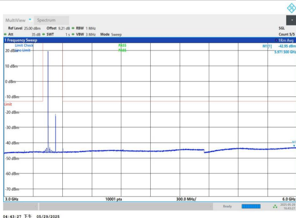
NTNV-n77(3450-3550)-PC2-30-80-L-DFT-BPSK-Edge_1RB_Left- 3000-6000-PASS
