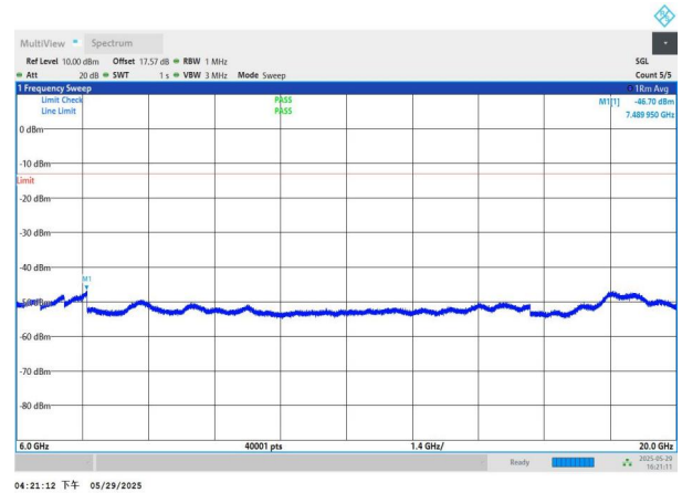
NTNV-n77(3450-3550)-PC2-30-30-H-DFT-BPSK-Edge_1RB_Left 6000-20000-PASS
