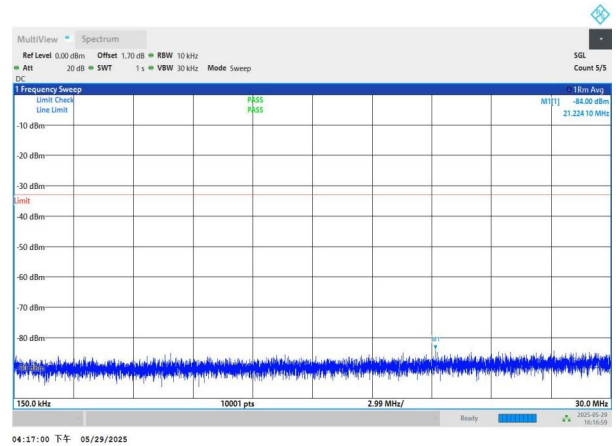
NTNV-n77(3450-3550)-PC2-30-30-M-DFT-BPSK-Edge_1RB_Left -0.15-30-PASS
