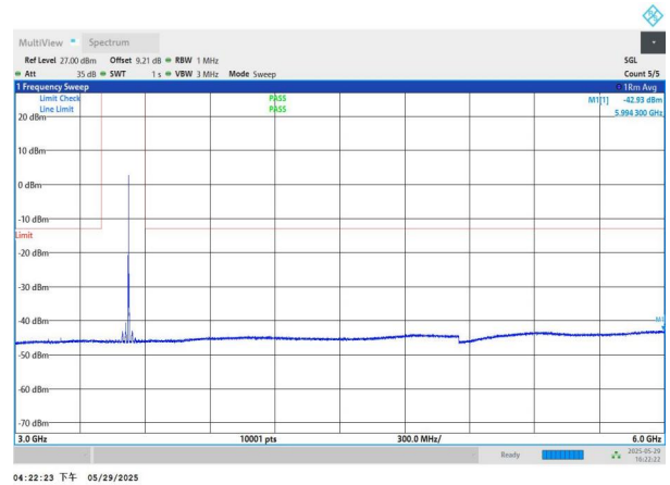
NTNV-n77(3450-3550)-PC2-30-30-H-DFT-QPSK-Edge_1RB_Left -3000-6000-PASS
