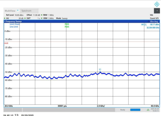
NTNV-n77(3450-3550)-PC2-30-60-H-DFT-QPSK-Edge_1RB_Left -20000-40000-PASS
