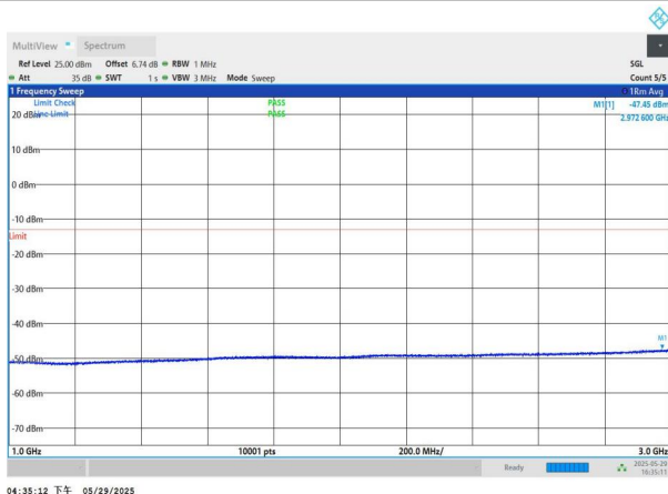
NTNV-n77(3450-3550)-PC2-30-60-L-DFT-QPSK-Edge_1RB_Left- 1000-3000-PASS
