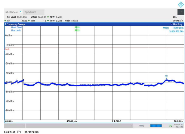
NTNV-n77(3450-3550)-PC2-30-40-M-DFT-BPSK-Edge_1RB_Left -6000-20000-PASS
