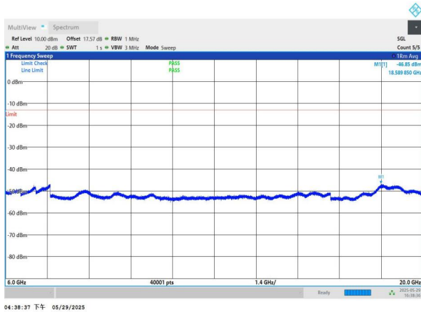
NTNV-n77(3450-3550)-PC2-30-60-M-DFT-QPSK-Edge_1RB_Left -6000-20000-PASS
