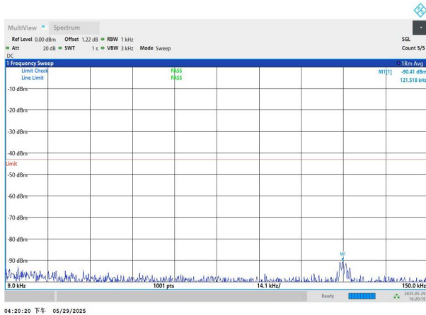
NTNV-n77(3450-3550)-PC2-30-30-H-DFT-BPSK-Edge_1RB_Left -0.009-0.15-PASS
