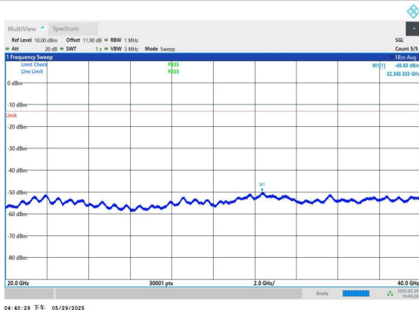
NTNV-n77(3450-3550)-PC2-30-60-H-DFT-BPSK-Edge_1RB_Left -20000-40000-PASS
