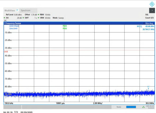
NTNV-n77(3450-3550)-PC2-30-40-H-DFT-BPSK-Edge_1RB_Left 0.15-30-PASS
