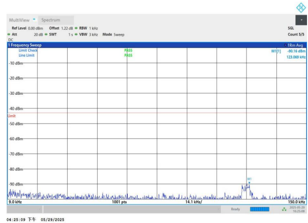
NTNV-n77(3450-3550)-PC2-30-40-L-DFT-QPSK-Edge_1RB_Left- 0.009-0.15-PASS
