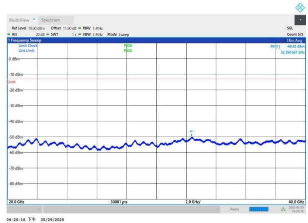
NTNV-n77(3450-3550)-PC2-30-40-L-DFT-QPSK-Edge_1RB_Left- 20000-40000-PASS
