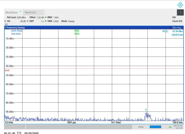
NTNV-n77(3450-3550)-PC2-30-30-H-DFT-QPSK-Edge_1RB_Left -0.009-0.15-PASS
