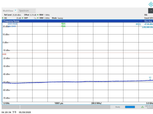
NTNV-n77(3450-3550)-PC2-30-40-M-DFT-QPSK-Edge_1RB_Left -1000-3000-PASS
