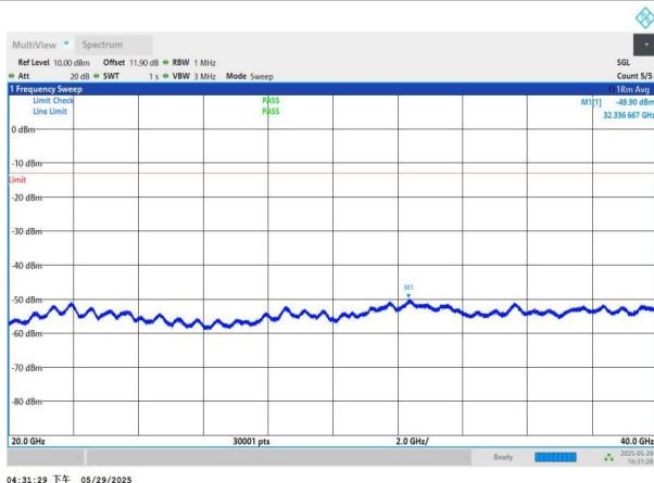
NTNV-n77(3450-3550)-PC2-30-40-H-DFT-BPSK-Edge_1RB_Left -20000-40000-PASS
