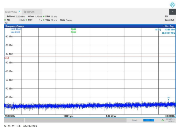
NTNV-n77(3450-3550)-PC2-30-60-H-DFT-BPSK-Edge_1RB_Left 0.15-30-PASS
