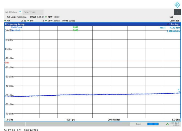
NTNV-n77(3450-3550)-PC2-30-40-M-DFT-BPSK-Edge_1RB_Left -1000-3000-PASS
