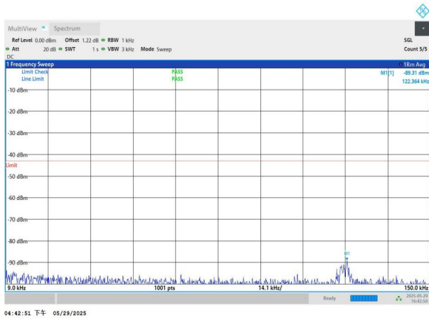
NTNV-n77(3450-3550)-PC2-30-80-L-DFT-BPSK-Edge_1RB_Left- 0.009-0.15-PASS
