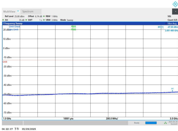
NTNV-n77(3450-3550)-PC2-30-30-H-DFT-QPSK-Edge_1RB_Left -1000-3000-PASS
