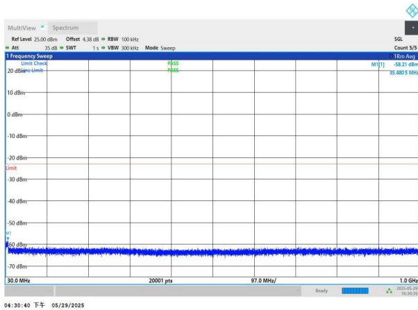
NTNV-n77(3450-3550)-PC2-30-40-H-DFT-BPSK-Edge_1RB_Left -30-1000-PASS
