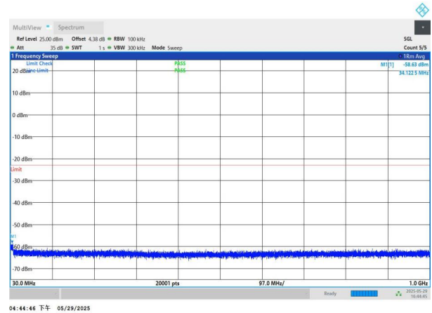
NTNV-n77(3450-3550)-PC2-30-80-L-DFT-QPSK-Edge_1RB_Left- 30-1000-PASS
