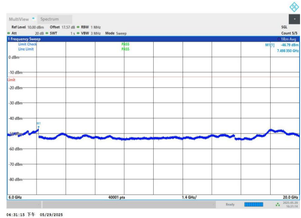
NTNV-n77(3450-3550)-PC2-30-40-H-DFT-BPSK-Edge_1RB_Left 6000-20000-PASS
