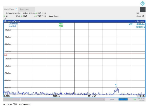
NTNV-n77(3450-3550)-PC2-30-40-M-DFT-QPSK-Edge_1RB_Left -0.009-0.15-PASS
