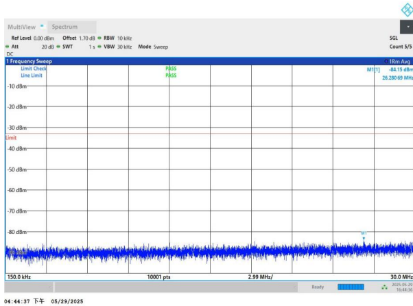
NTNV-n77(3450-3550)-PC2-30-80-L-DFT-QPSK-Edge_1RB_Left- 0.15-30-PASS
