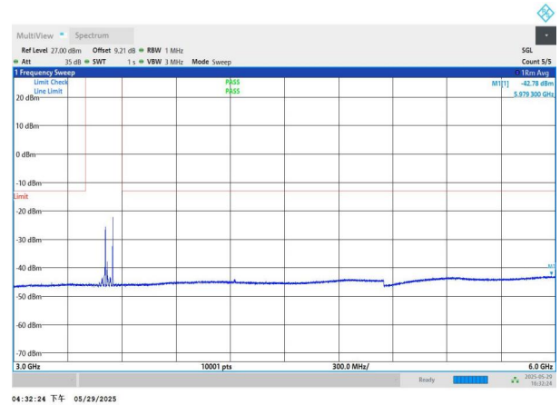
NTNV-n77(3450-3550)-PC2-30-40-H-DFT-QPSK-Edge_1RB_Left -3000-6000-PASS
