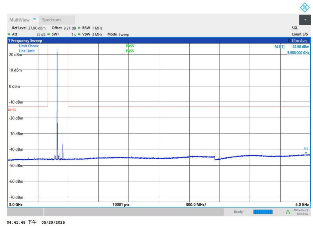
NTNV-n77(3450-3550)-PC2-30-60-H-DFT-QPSK-Edge_1RB_Left -3000-6000-PASS
