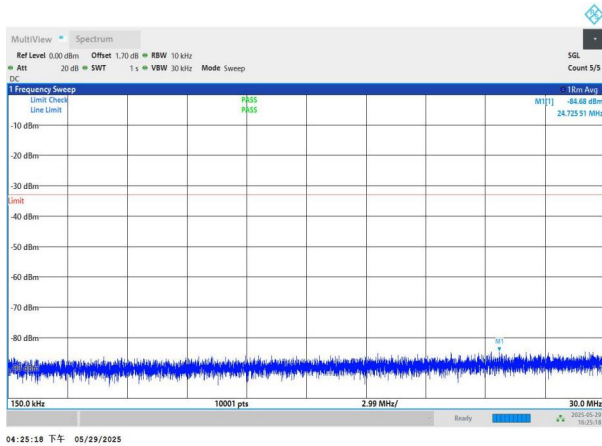
NTNV-n77(3450-3550)-PC2-30-40-L-DFT-QPSK-Edge_1RB_Left- 0.15-30-PASS
