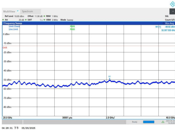
NTNV-n77(3450-3550)-PC2-30-40-M-DFT-BPSK-Edge_1RB_Left -20000-40000-PASS
