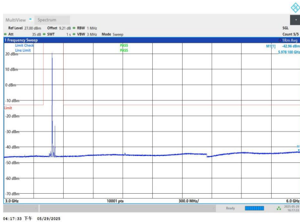
NTNV-n77(3450-3550)-PC2-30-30-M-DFT-BPSK-Edge_1RB_Left -3000-6000-PASS
