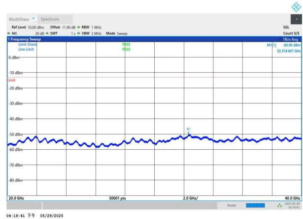
NTNV-n77(3450-3550)-PC2-30-30-M-DFT-QPSK-Edge_1RB_Left -20000-40000-PASS
