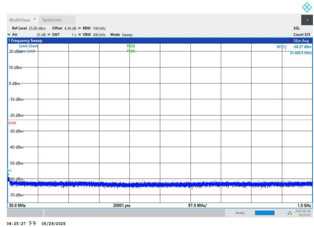
NTNV-n77(3450-3550)-PC2-30-40-L-DFT-QPSK-Edge_1RB_Left- 30-1000-PASS
