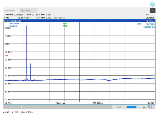
NTNV-n77(3450-3550)-PC2-30-80-L-DFT-QPSK-Edge_1RB_Left- 3000-6000-PASS
