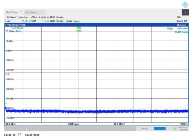
NTNV-n77(3450-3550)-PC2-30-40-H-DFT-QPSK-Edge_1RB_Left -30-1000-PASS
