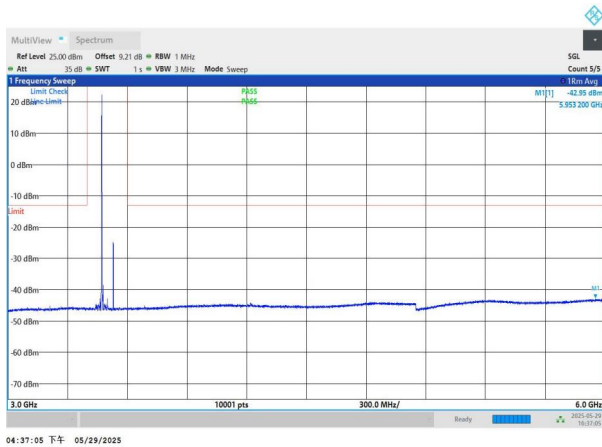
NTNV-n77(3450-3550)-PC2-30-60-M-DFT-BPSK-Edge_1RB_Left -3000-6000-PASS
