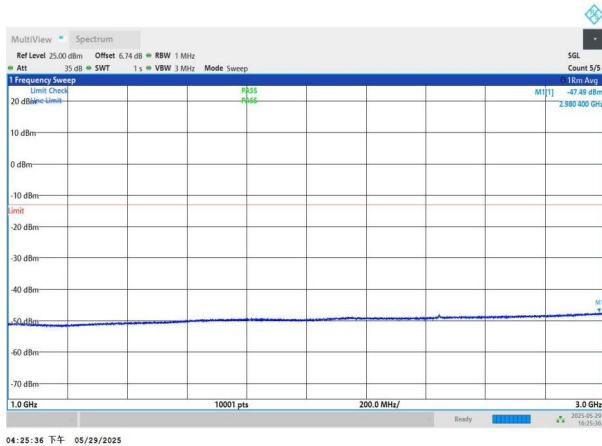
NTNV-n77(3450-3550)-PC2-30-40-L-DFT-QPSK-Edge_1RB_Left- 1000-3000-PASS
