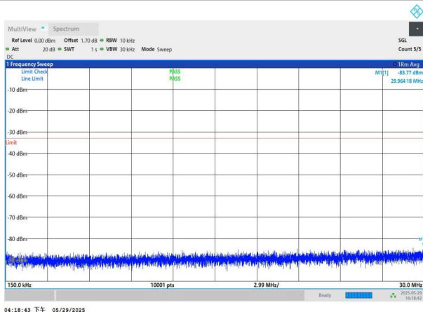
NTNV-n77(3450-3550)-PC2-30-30-M-DFT-QPSK-Edge_1RB_Left -0.15-30-PASS
