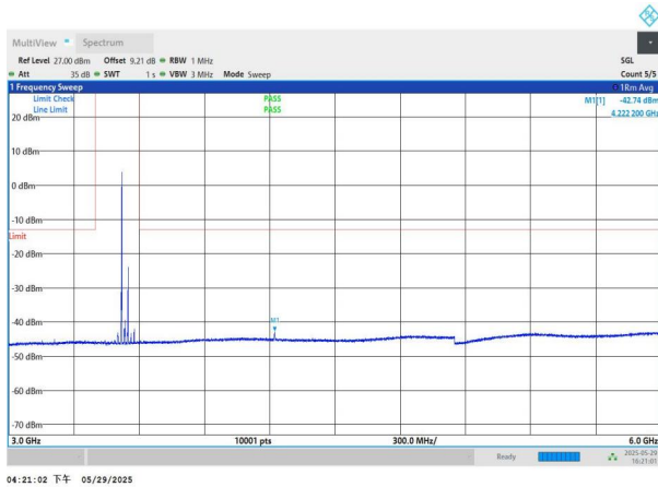
NTNV-n77(3450-3550)-PC2-30-30-H-DFT-BPSK-Edge_1RB_Left -3000-6000-PASS
