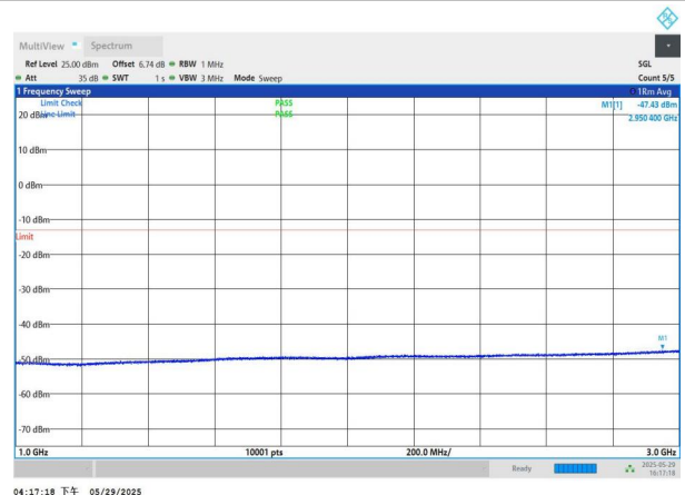
NTNV-n77(3450-3550)-PC2-30-30-M-DFT-BPSK-Edge_1RB_Left -1000-3000-PASS
