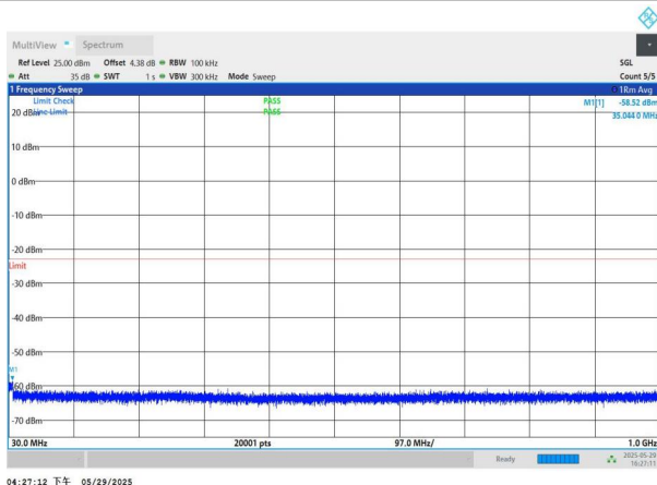
NTNV-n77(3450-3550)-PC2-30-40-M-DFT-BPSK-Edge_1RB_Left -30-1000-PASS
