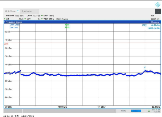
NTNV-n77(3450-3550)-PC2-30-40-L-DFT-BPSK-Edge_1RB_Left- 6000-20000-PASS
