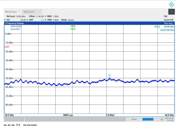
NTNV-n77(3450-3550)-PC2-30-40-H-DFT-QPSK-Edge_1RB_Left -20000-40000-PASS
