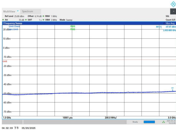
NTNV-n77(3450-3550)-PC2-30-40-H-DFT-QPSK-Edge_1RB_Left -1000-3000-PASS
