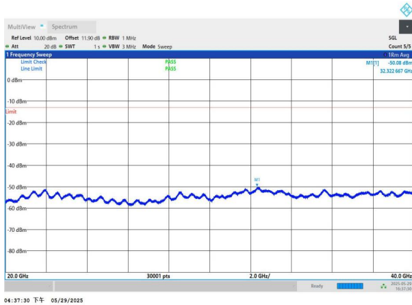
NTNV-n77(3450-3550)-PC2-30-60-M-DFT-BPSK-Edge_1RB_Left -20000-40000-PASS
