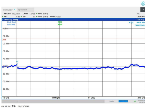
NTNV-n77(3450-3550)-PC2-30-30-L-DFT-QPSK-Edge_1RB_Left- 6000-20000-PASS
