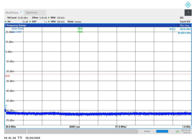
NTNV-n77(3450-3550)-PC2-30-60-H-DFT-QPSK-Edge_1RB_Left -30-1000-PASS
