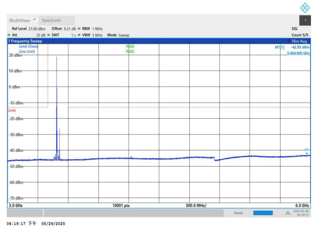
NTNV-n77(3450-3550)-PC2-30-30-M-DFT-QPSK-Edge_1RB_Left -3000-6000-PASS
