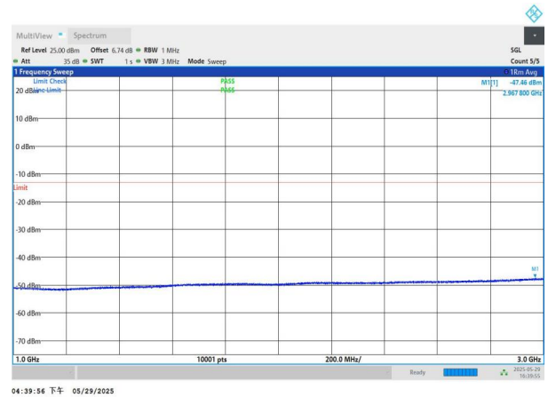
NTNV-n77(3450-3550)-PC2-30-60-H-DFT-BPSK-Edge_1RB_Left 1000-3000-PASS
