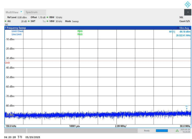
NTNV-n77(3450-3550)-PC2-30-30-H-DFT-BPSK-Edge_1RB_Left 0.15-30-PASS
