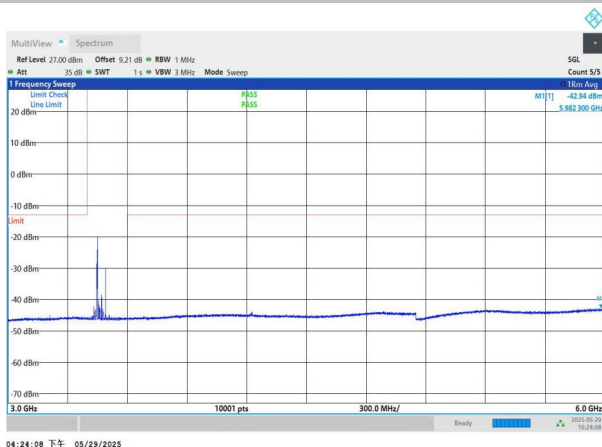
NTNV-n77(3450-3550)-PC2-30-40-L-DFT-BPSK-Edge_1RB_Left- 3000-6000-PASS
