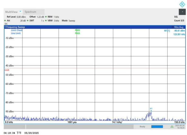
NTNV-n77(3450-3550)-PC2-30-30-M-DFT-QPSK-Edge_1RB_Left -0.009-0.15-PASS
