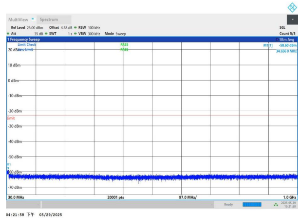
NTNV-n77(3450-3550)-PC2-30-30-H-DFT-QPSK-Edge_1RB_Left -30-1000-PASS
