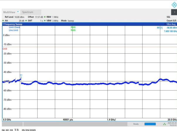
NTNV-n77(3450-3550)-PC2-30-30-H-DFT-QPSK-Edge_1RB_Left -6000-20000-PASS
