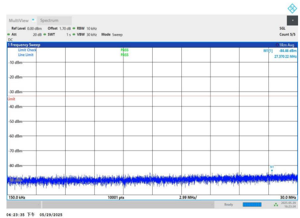
NTNV-n77(3450-3550)-PC2-30-40-L-DFT-BPSK-Edge_1RB_Left- 0.15-30-PASS
