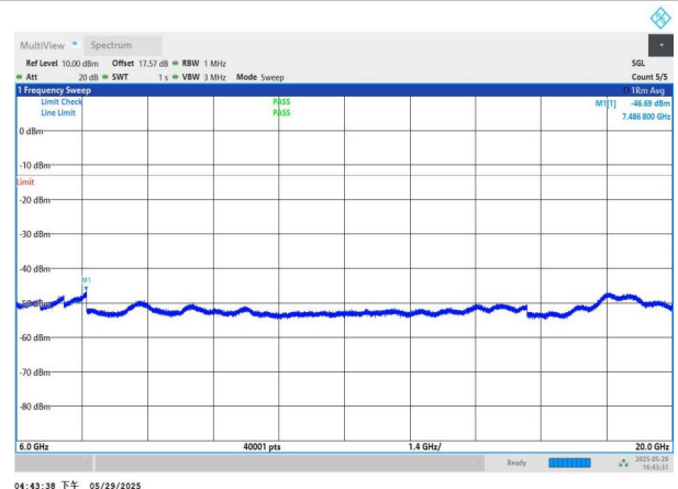
NTNV-n77(3450-3550)-PC2-30-80-L-DFT-BPSK-Edge_1RB_Left- 6000-20000-PASS
