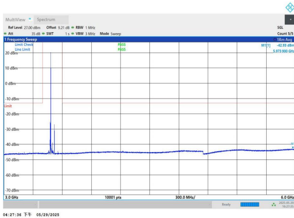
NTNV-n77(3450-3550)-PC2-30-40-M-DFT-BPSK-Edge_1RB_Left -3000-6000-PASS
