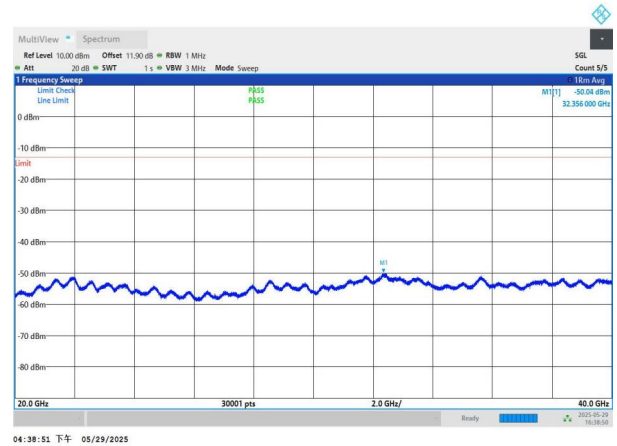
NTNV-n77(3450-3550)-PC2-30-60-M-DFT-QPSK-Edge_1RB_Left -20000-40000-PASS
