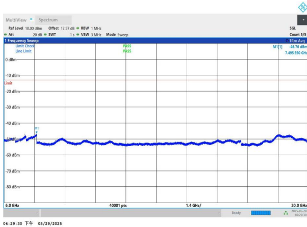
NTNV-n77(3450-3550)-PC2-30-40-M-DFT-QPSK-Edge_1RB_Left -6000-20000-PASS
