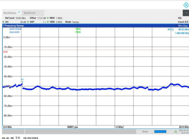
NTNV-n77(3450-3550)-PC2-30-60-H-DFT-QPSK-Edge_1RB_Left -6000-20000-PASS
