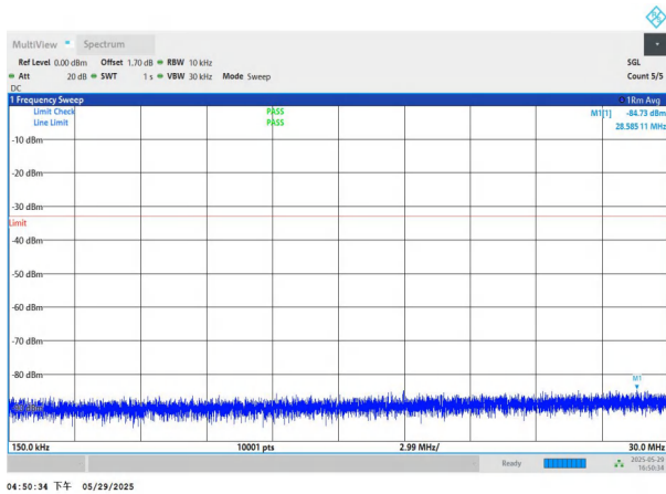
NTNV-n77(3450-3550)-PC2-30-80-H-DFT-QPSK-Edge_1RB_Left -0.15-30-PASS
