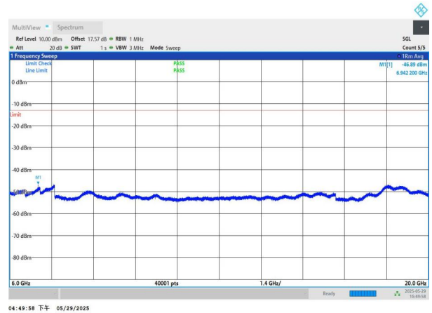
NTNV-n77(3450-3550)-PC2-30-80-H-DFT-BPSK-Edge_1RB_Left 6000-20000-PASS
