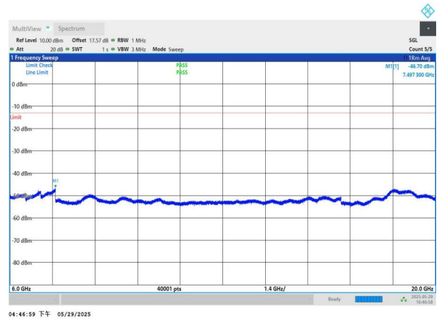
NTNV-n77(3450-3550)-PC2-30-80-M-DFT-BPSK-Edge_1RB_Left -6000-20000-PASS
