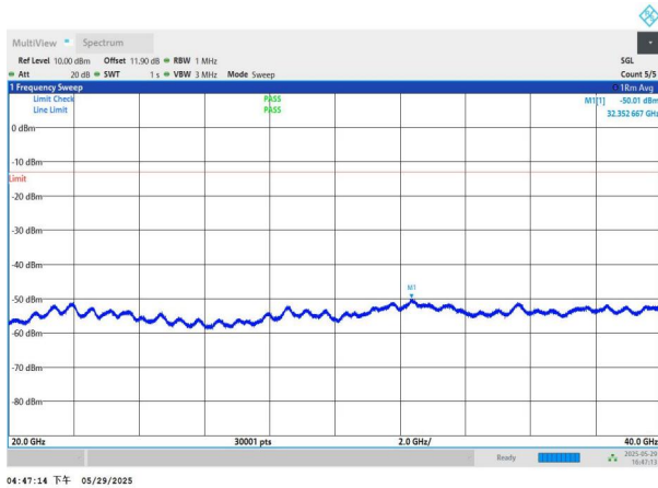
NTNV-n77(3450-3550)-PC2-30-80-M-DFT-BPSK-Edge_1RB_Left -20000-40000-PASS
