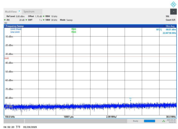
NTNV-n77(3450-3550)-PC2-30-100-M-DFT-BPSK-Edge_1RB_Lef t-0.15-30-PASS
