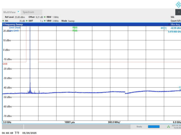
NTNV-n77(3450-3550)-PC2-30-80-M-DFT-BPSK-Edge_1RB_Left -3000-6000-PASS
