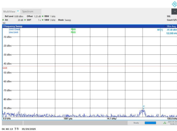
NTNV-n77(3450-3550)-PC2-30-80-M-DFT-BPSK-Edge_1RB_Left -0.009-0.15-PASS
