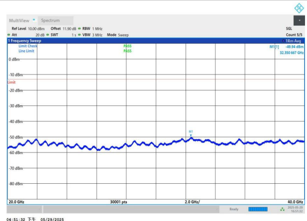
NTNV-n77(3450-3550)-PC2-30-80-H-DFT-QPSK-Edge_1RB_Left -20000-40000-PASS
