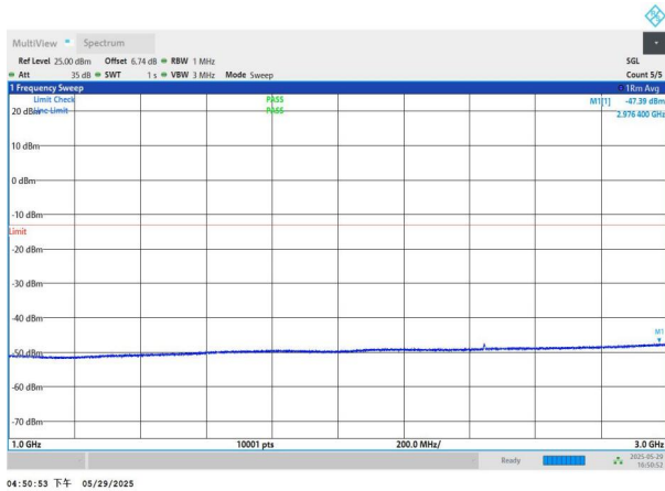
NTNV-n77(3450-3550)-PC2-30-80-H-DFT-QPSK-Edge_1RB_Left -1000-3000-PASS
