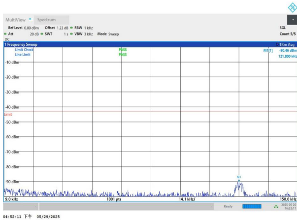
NTNV-n77(3450-3550)-PC2-30-100-M-DFT-BPSK-Edge_1RB_Le ft-0.009-0.15-PASS
