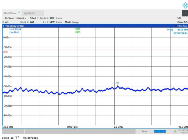
NTNV-n77(3450-3550)-PC2-30-100-M-DFT-BPSK-Edge_1RB_Le ft-20000-40000-PASS
