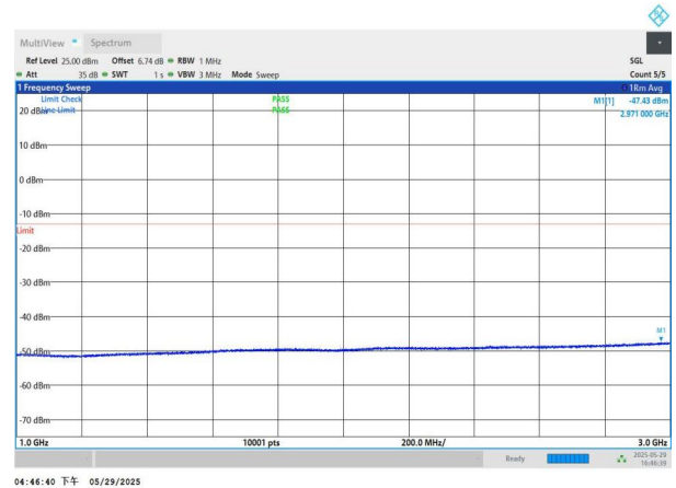
NTNV-n77(3450-3550)-PC2-30-80-M-DFT-BPSK-Edge_1RB_Left -1000-3000-PASS
