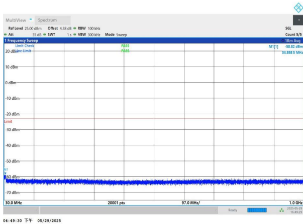
NTNV-n77(3450-3550)-PC2-30-80-H-DFT-BPSK-Edge_1RB_Left -30-1000-PASS
