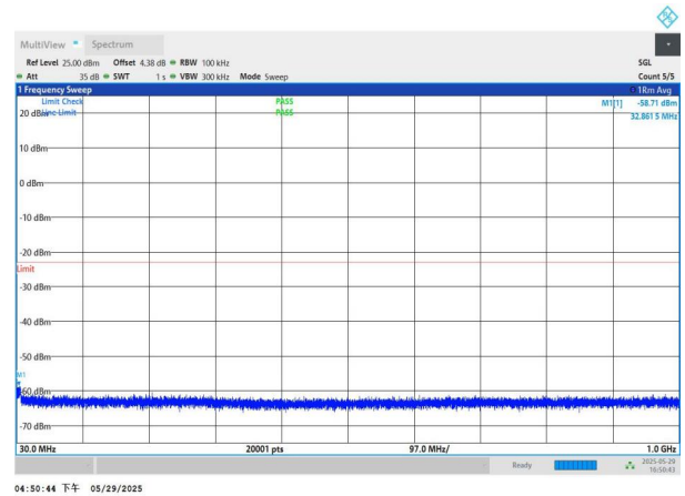
NTNV-n77(3450-3550)-PC2-30-80-H-DFT-QPSK-Edge_1RB_Left -30-1000-PASS
