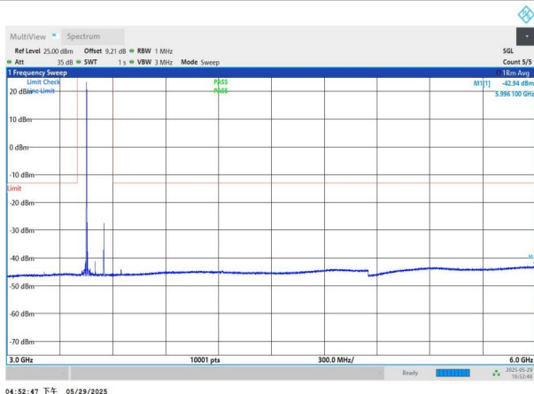
NTNV-n77(3450-3550)-PC2-30-100-M-DFT-BPSK-Edge_1RB_Le ft-3000-6000-PASS
