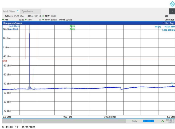
NTNV-n77(3450-3550)-PC2-30-80-H-DFT-BPSK-Edge_1RB_Left -3000-6000-PASS
