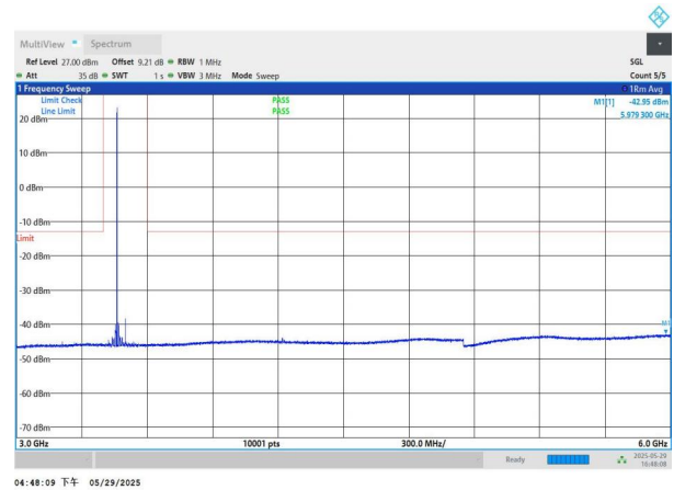
NTNV-n77(3450-3550)-PC2-30-80-M-DFT-QPSK-Edge_1RB_Left -3000-6000-PASS
