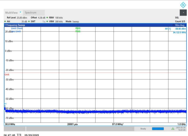
NTNV-n77(3450-3550)-PC2-30-80-M-DFT-QPSK-Edge_1RB_Left -30-1000-PASS
