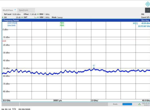
NTNV-n77(3450-3550)-PC2-30-80-H-DFT-BPSK-Edge_1RB_Left -20000-40000-PASS
