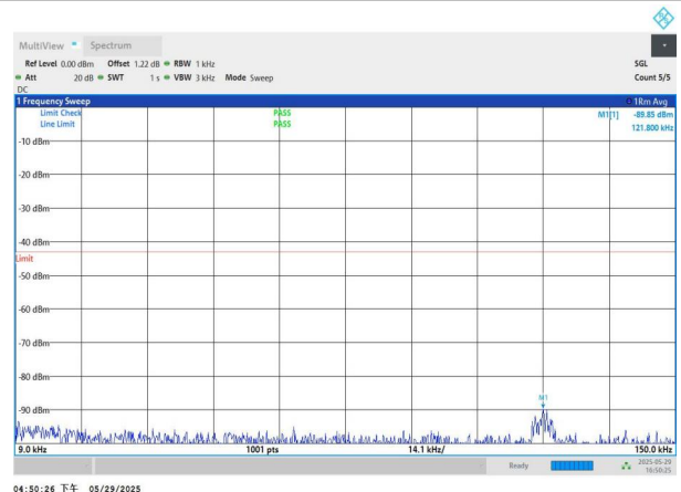
NTNV-n77(3450-3550)-PC2-30-80-H-DFT-QPSK-Edge_1RB_Left -0.009-0.15-PASS
