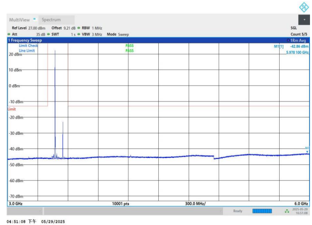
NTNV-n77(3450-3550)-PC2-30-80-H-DFT-QPSK-Edge_1RB_Left -3000-6000-PASS
