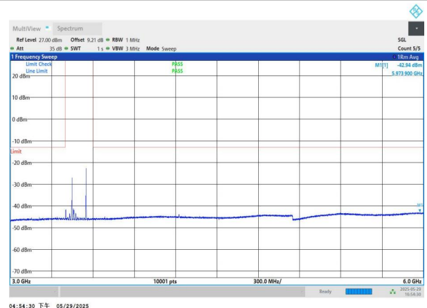
NTNV-n77(3450-3550)-PC2-30-100-M-DFT-QPSK-Edge_1RB_Le ft-3000-6000-PASS
