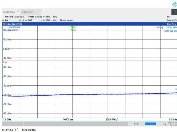
NTNV-n77(3450-3550)-PC2-30-80-M-DFT-QPSK-Edge_1RB_Left -1000-3000-PASS
