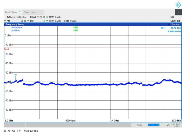
NTNV-n77(3450-3550)-PC2-30-100-M-DFT-BPSK-Edge_1RB_Lef t-6000-20000-PASS
