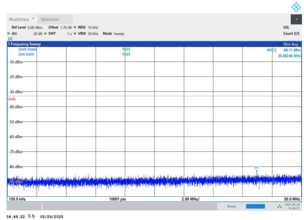
NTNV-n77(3450-3550)-PC2-30-80-M-DFT-BPSK-Edge_1RB_Left -0.15-30-PASS
