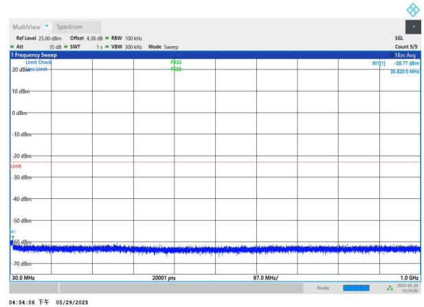
NTNV-n77(3450-3550)-PC2-30-100-M-DFT-QPSK-Edge_1RB_Le ft-30-1000-PASS
