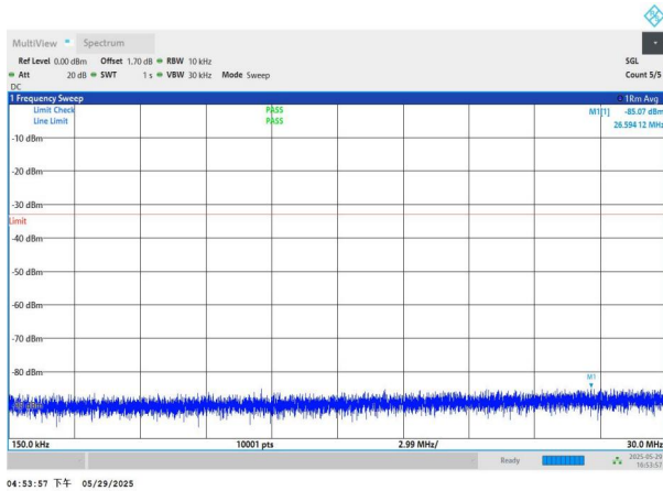
NTNV-n77(3450-3550)-PC2-30-100-M-DFT-QPSK-Edge_1RB_Le ft-0.15-30-PASS
