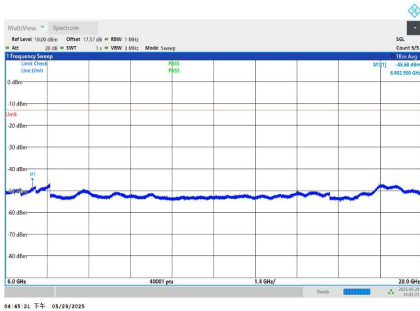
NTNV-n77(3450-3550)-PC2-30-80-L-DFT-QPSK-Edge_1RB_Left- 6000-20000-PASS
