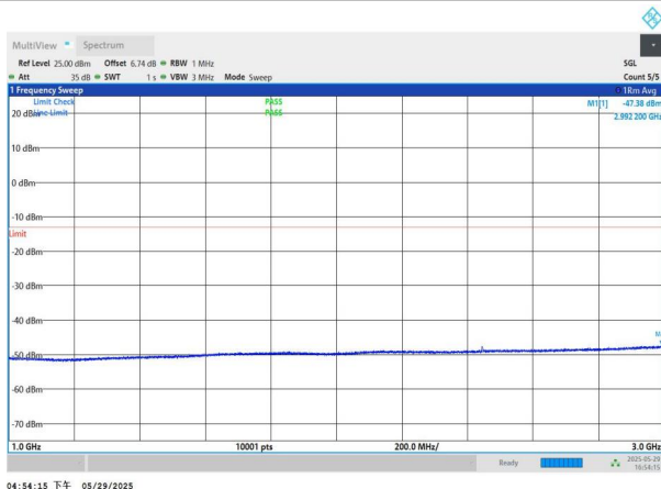
NTNV-n77(3450-3550)-PC2-30-100-M-DFT-QPSK-Edge_1RB_Le ft-1000-3000-PASS
