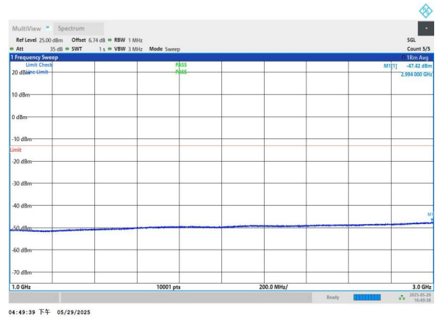
NTNV-n77(3450-3550)-PC2-30-80-H-DFT-BPSK-Edge_1RB_Left 1000-3000-PASS
