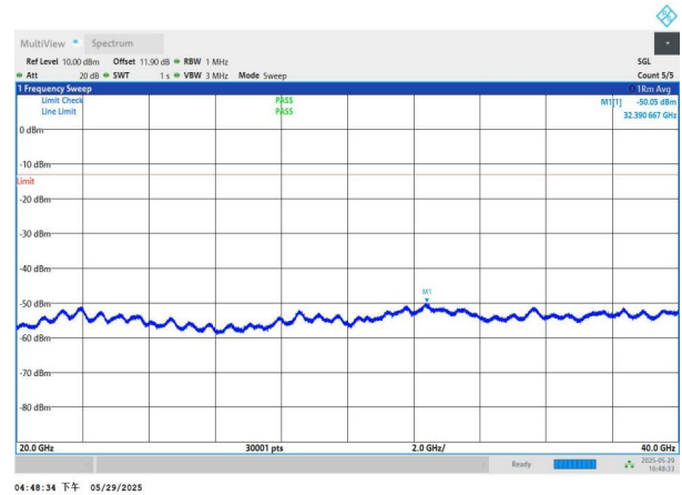
NTNV-n77(3450-3550)-PC2-30-80-M-DFT-QPSK-Edge_1RB_Left -20000-40000-PASS
