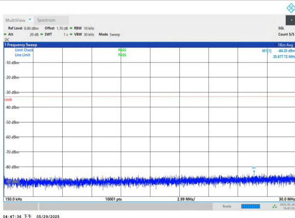
NTNV-n77(3450-3550)-PC2-30-80-M-DFT-QPSK-Edge_1RB_Left -0.15-30-PASS
