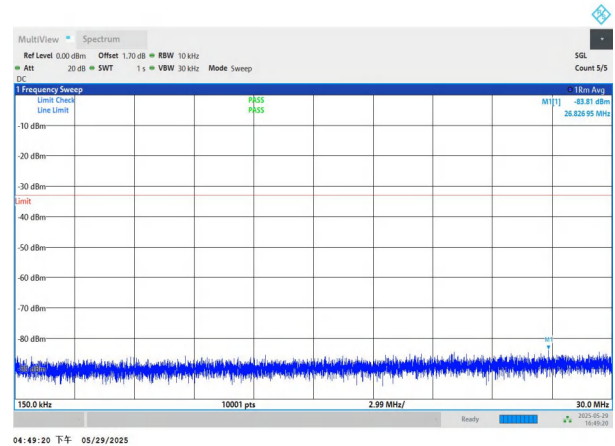
NTNV-n77(3450-3550)-PC2-30-80-H-DFT-BPSK-Edge_1RB_Left 0.15-30-PASS
