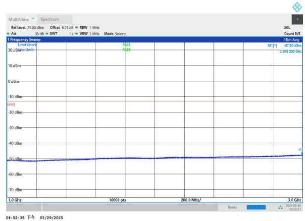
NTNV-n77(3450-3550)-PC2-30-100-M-DFT-BPSK-Edge_1RB_Lef t-1000-3000-PASS
