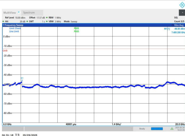
NTNV-n77(3450-3550)-PC2-30-80-H-DFT-QPSK-Edge_1RB_Left -6000-20000-PASS
