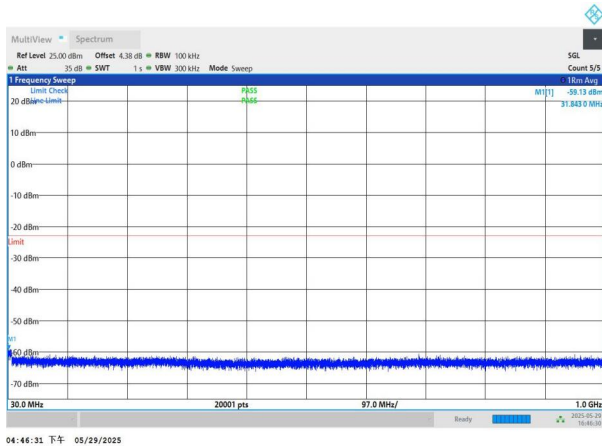
NTNV-n77(3450-3550)-PC2-30-80-M-DFT-BPSK-Edge_1RB_Left -30-1000-PASS
