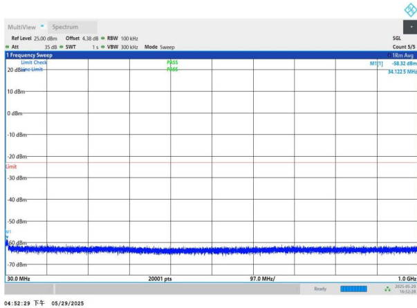
NTNV-n77(3450-3550)-PC2-30-100-M-DFT-BPSK-Edge_1RB_Le ft-30-1000-PASS
