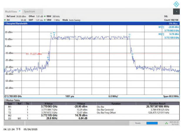
NTNV-n78(3700-3800)-PC2-30-30-H-DFT-256QAM-Outer_Full-A nt1-PASS
