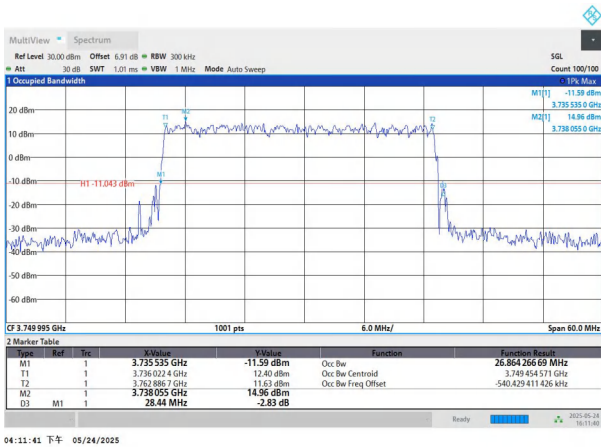
NTNV-n78(3700-3800)-PC2-30-30-M-DFT-256QAM-Outer_Full-A nt1-PASS
