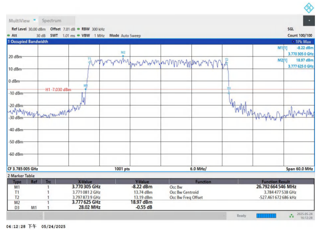
NTNV-n78(3700-3800)-PC2-30-30-H-DFT-BPSK-Outer_Full-Ant1- PASS
