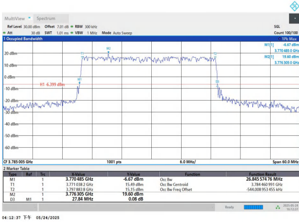
NTNV-n78(3700-3800)-PC2-30-30-H-DFT-QPSK-Outer_Full-Ant1 -PASS
