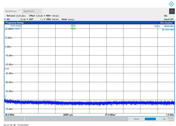
NTNV-n78(3700-3800)-PC2-30-40-L-DFT-QPSK-Edge_1RB_Left- 30-1000-PASS
