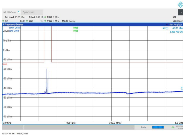
NTNV-n78(3700-3800)-PC2-30-40-M-DFT-BPSK-Edge_1RB_Left -3000-6000-PASS
