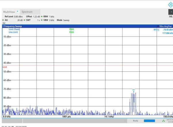
NTNV-n78(3700-3800)-PC2-30-60-H-DFT-BPSK-Edge_1RB_Left -0.009-0.15-PASS
