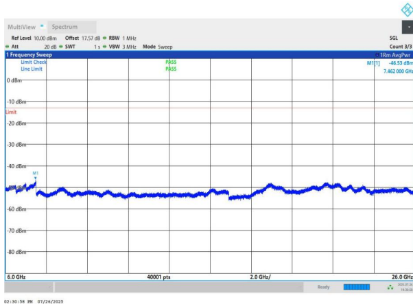
NTNV-n78(3700-3800)-PC2-30-40-M-DFT-QPSK-Edge_1RB_Left -6000-26000-PASS
