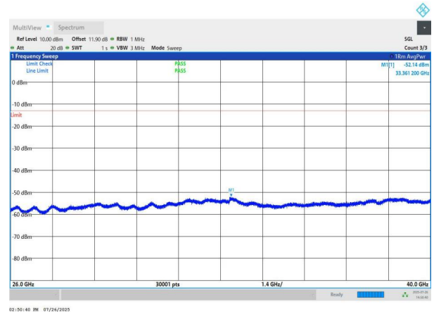
NTNV-n78(3700-3800)-PC2-30-60-M-DFT-QPSK-Edge_1RB_Left -26000-40000-PASS
