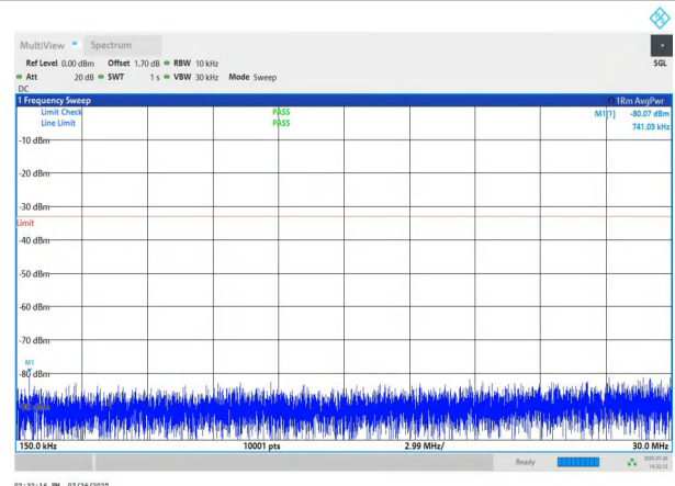
NTNV-n78(3700-3800)-PC2-30-40-H-DFT-BPSK-Edge_1RB_Left 0.15-30-PASS
