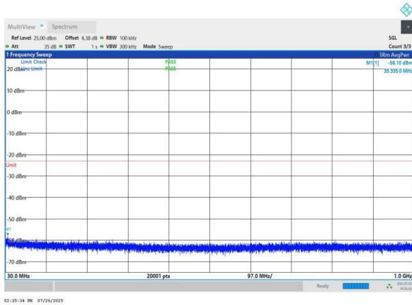
NTNV-n78(3700-3800)-PC2-30-50-L-DFT-BPSK-Edge_1RB_Left- 30-1000-PASS
