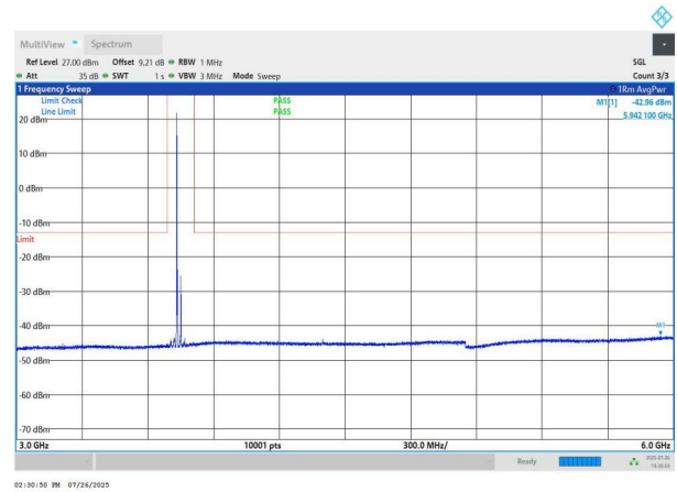
NTNV-n78(3700-3800)-PC2-30-40-M-DFT-QPSK-Edge_1RB_Left -3000-6000-PASS
