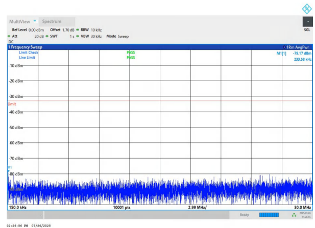
NTNV-n78(3700-3800)-PC2-30-40-L-DFT-BPSK-Edge_1RB_Left- 0.15-30-PASS
