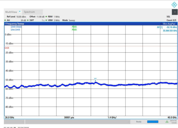
NTNV-n78(3700-3800)-PC2-30-50-H-DFT-QPSK-Edge_1RB_Left -26000-40000-PASS
