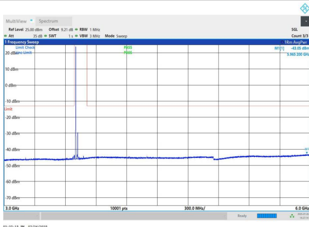
NTNV-n78(3700-3800)-PC2-30-40-L-DFT-BPSK-Edge_1RB_Left- 3000-6000-PASS
