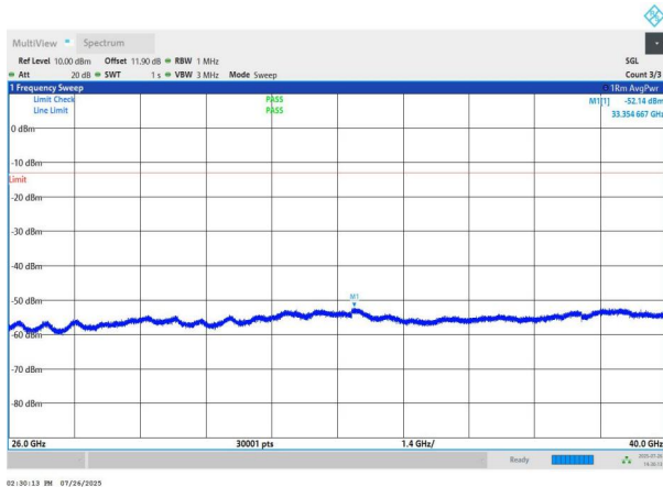
NTNV-n78(3700-3800)-PC2-30-40-M-DFT-BPSK-Edge_1RB_Left -26000-40000-PASS
