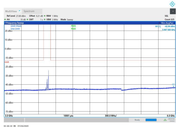
NTNV-n78(3700-3800)-PC2-30-50-H-DFT-QPSK-Edge_1RB_Left -3000-6000-PASS
