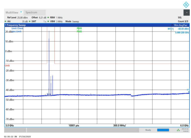
NTNV-n78(3700-3800)-PC2-30-60-M-DFT-QPSK-Edge_1RB_Left -3000-6000-PASS
