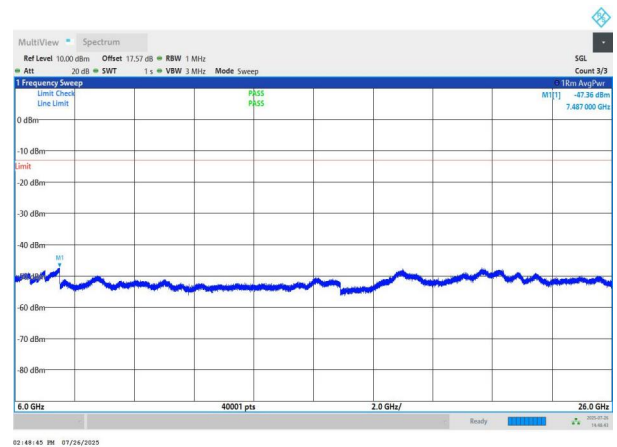
NTNV-n78(3700-3800)-PC2-30-60-M-DFT-BPSK-Edge_1RB_Left -6000-26000-PASS
