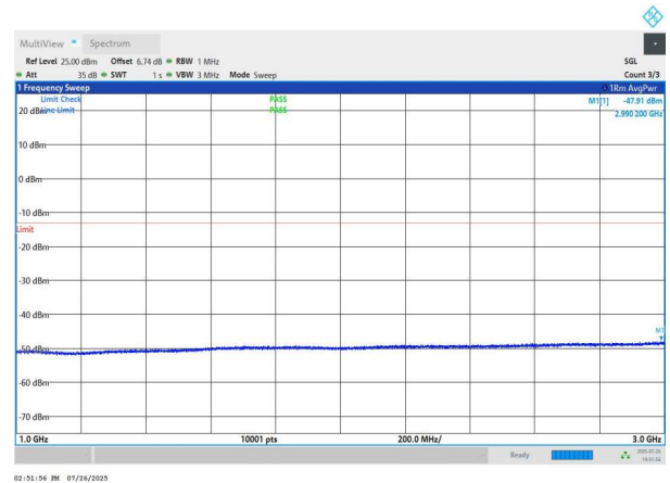
NTNV-n78(3700-3800)-PC2-30-60-H-DFT-BPSK-Edge_1RB_Left 1000-3000-PASS
