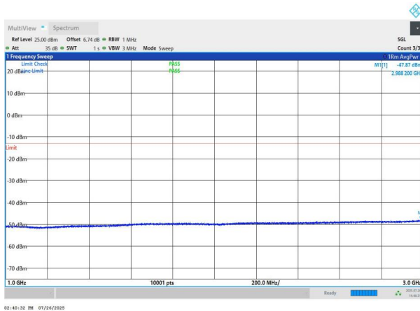
NTNV-n78(3700-3800)-PC2-30-50-M-DFT-QPSK-Edge_1RB_Left -1000-3000-PASS
