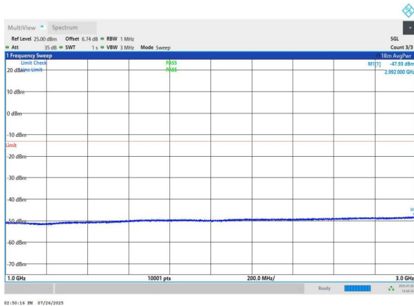
NTNV-n78(3700-3800)-PC2-30-60-M-DFT-QPSK-Edge_1RB_Left -1000-3000-PASS
