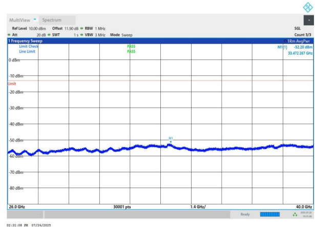
NTNV-n78(3700-3800)-PC2-30-40-M-DFT-QPSK-Edge_1RB_Left -26000-40000-PASS
