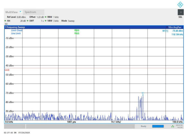
NTNV-n78(3700-3800)-PC2-30-40-L-DFT-QPSK-Edge_1RB_Left- 0.009-0.15-PASS
