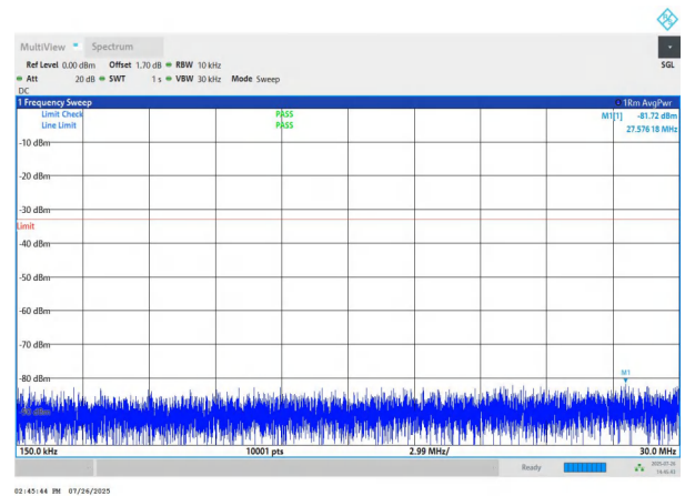
NTNV-n78(3700-3800)-PC2-30-60-L-DFT-BPSK-Edge_1RB_Left- 0.15-30-PASS
