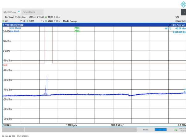
NTNV-n78(3700-3800)-PC2-30-50-L-DFT-BPSK-Edge_1RB_Left- 3000-6000-PASS
