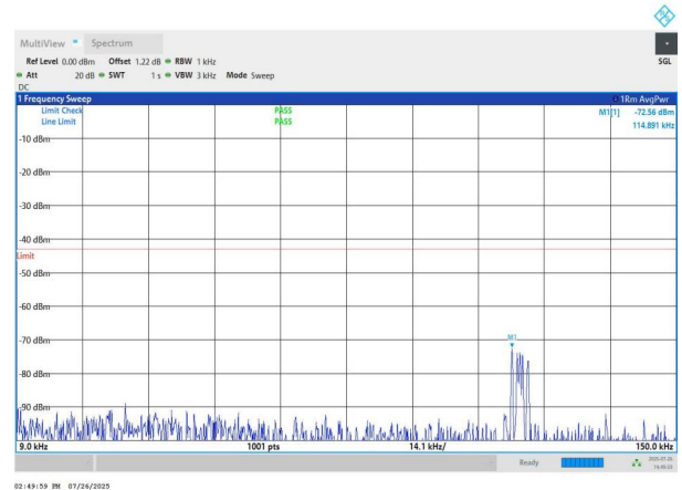
NTNV-n78(3700-3800)-PC2-30-60-M-DFT-QPSK-Edge_1RB_Left -0.009-0.15-PASS
