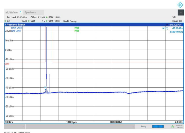
NTNV-n78(3700-3800)-PC2-30-50-L-DFT-QPSK-Edge_1RB_Left- 3000-6000-PASS
