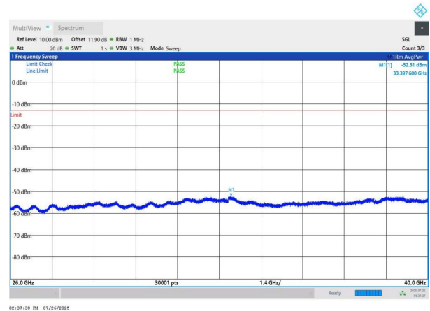
NTNV-n78(3700-3800)-PC2-30-50-L-DFT-QPSK-Edge_1RB_Left- 26000-40000-PASS
