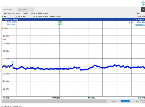
NTNV-n78(3700-3800)-PC2-30-40-H-DFT-QPSK-Edge_1RB_Left -6000-26000-PASS
