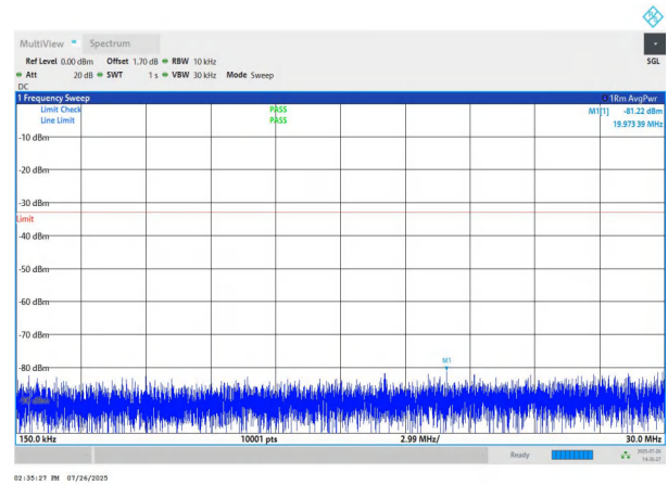
NTNV-n78(3700-3800)-PC2-30-50-L-DFT-BPSK-Edge_1RB_Left- 0.15-30-PASS
