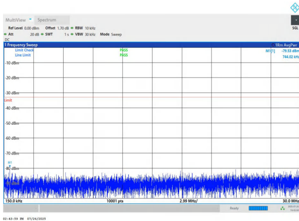
NTNV-n78(3700-3800)-PC2-30-50-H-DFT-QPSK-Edge_1RB_Left -0.15-30-PASS
