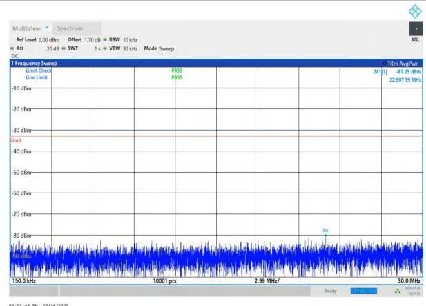
NTNV-n78(3700-3800)-PC2-30-60-H-DFT-BPSK-Edge_1RB_Left 0.15-30-PASS
