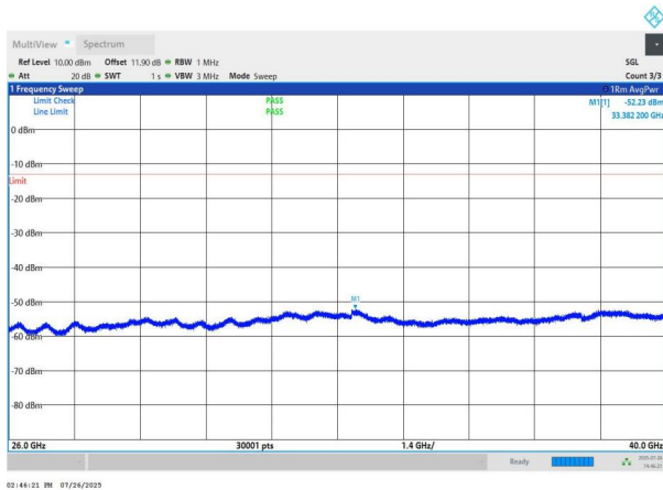
NTNV-n78(3700-3800)-PC2-30-60-L-DFT-BPSK-Edge_1RB_Left- 26000-40000-PASS
