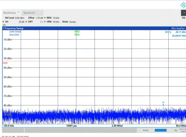
NTNV-n78(3700-3800)-PC2-30-40-M-DFT-QPSK-Edge_1RB_Left -0.15-30-PASS
