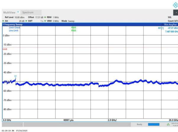
NTNV-n78(3700-3800)-PC2-30-40-L-DFT-QPSK-Edge_1RB_Left- 6000-26000-PASS
