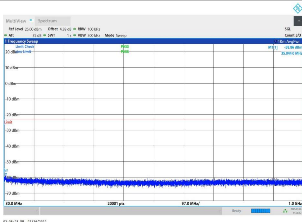
NTNV-n78(3700-3800)-PC2-30-50-M-DFT-BPSK-Edge_1RB_Left -30-1000-PASS
