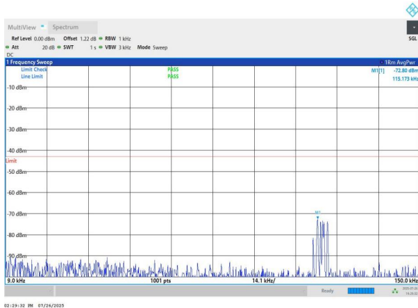
NTNV-n78(3700-3800)-PC2-30-40-M-DFT-BPSK-Edge_1RB_Left -0.009-0.15-PASS
