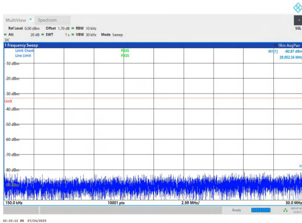
NTNV-n78(3700-3800)-PC2-30-40-H-DFT-QPSK-Edge_1RB_Left -0.15-30-PASS
