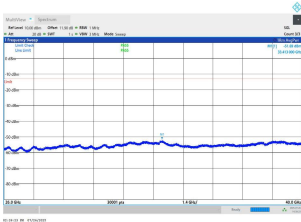
NTNV-n78(3700-3800)-PC2-30-50-M-DFT-BPSK-Edge_1RB_Left -26000-40000-PASS
