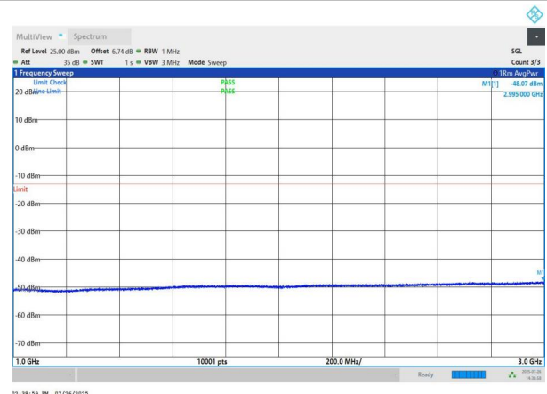
NTNV-n78(3700-3800)-PC2-30-50-M-DFT-BPSK-Edge_1RB_Left -1000-3000-PASS
