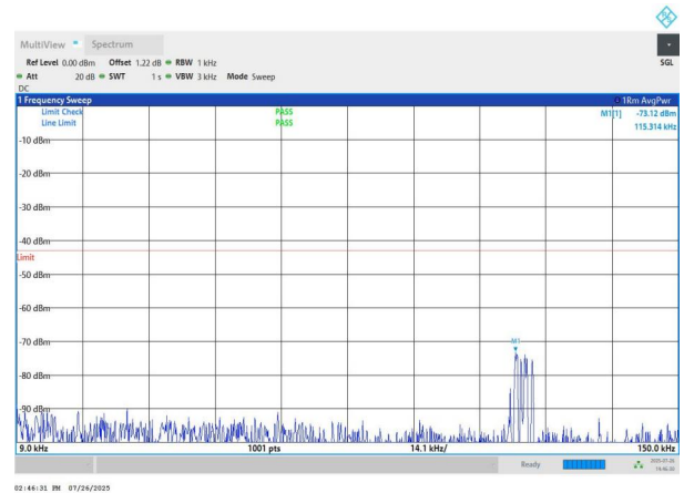
NTNV-n78(3700-3800)-PC2-30-60-L-DFT-QPSK-Edge_1RB_Left- 0.009-0.15-PASS
