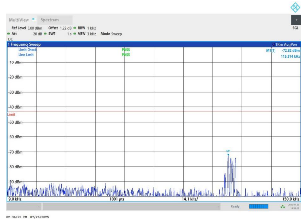
NTNV-n78(3700-3800)-PC2-30-50-L-DFT-QPSK-Edge_1RB_Left- 0.009-0.15-PASS
