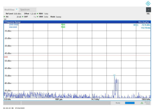
NTNV-n78(3700-3800)-PC2-30-40-M-DFT-QPSK-Edge_1RB_Left -0.009-0.15-PASS
