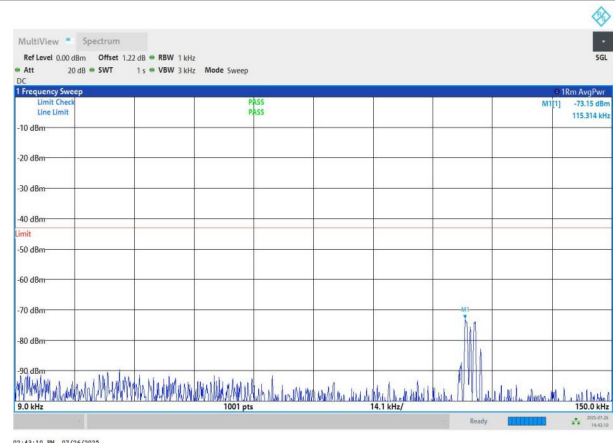
NTNV-n78(3700-3800)-PC2-30-50-H-DFT-QPSK-Edge_1RB_Left -0.009-0.15-PASS
