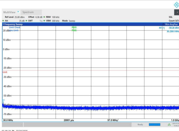
NTNV-n78(3700-3800)-PC2-30-60-M-DFT-BPSK-Edge_1RB_Left -30-1000-PASS
