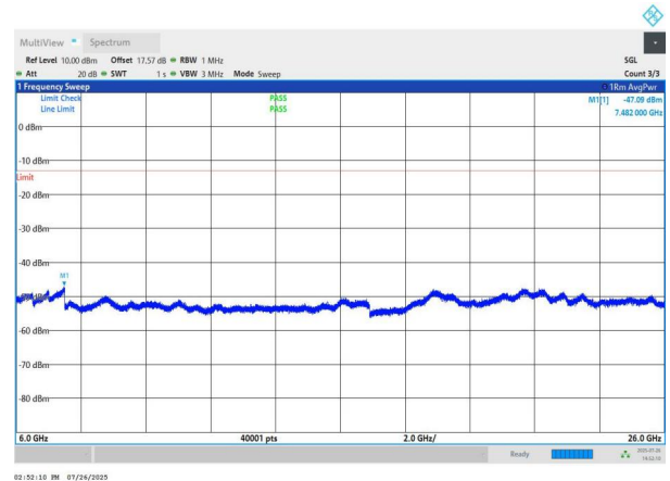
NTNV-n78(3700-3800)-PC2-30-60-H-DFT-BPSK-Edge_1RB_Left 6000-26000-PASS
