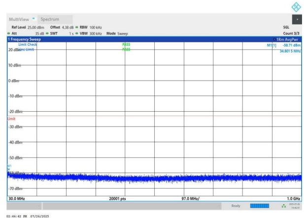
NTNV-n78(3700-3800)-PC2-30-60-L-DFT-QPSK-Edge_1RB_Left- 30-1000-PASS
