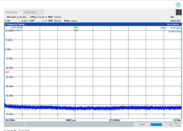
NTNV-n78(3700-3800)-PC2-30-40-M-DFT-QPSK-Edge_1RB_Left -30-1000-PASS
