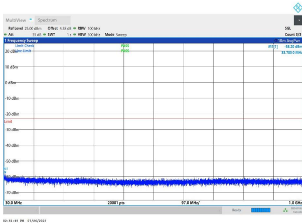
NTNV-n78(3700-3800)-PC2-30-60-H-DFT-BPSK-Edge_1RB_Left -30-1000-PASS
