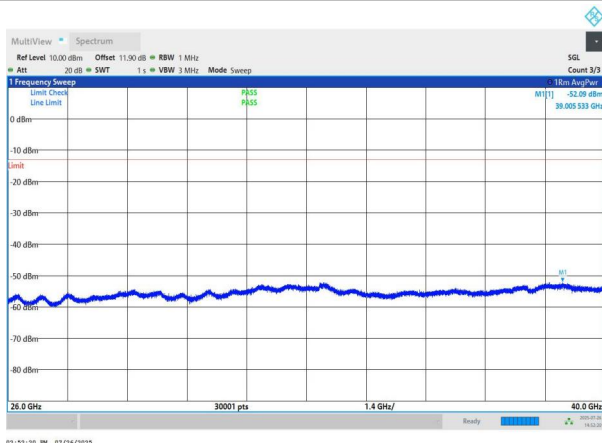
NTNV-n78(3700-3800)-PC2-30-60-H-DFT-BPSK-Edge_1RB_Left -26000-40000-PASS
