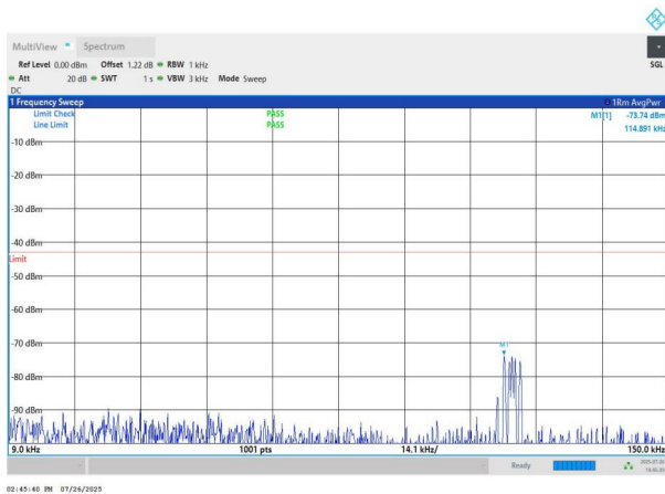
NTNV-n78(3700-3800)-PC2-30-60-L-DFT-BPSK-Edge_1RB_Left- 0.009-0.15-PASS
