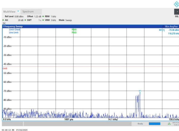
NTNV-n78(3700-3800)-PC2-30-60-M-DFT-BPSK-Edge_1RB_Left -0.009-0.15-PASS
