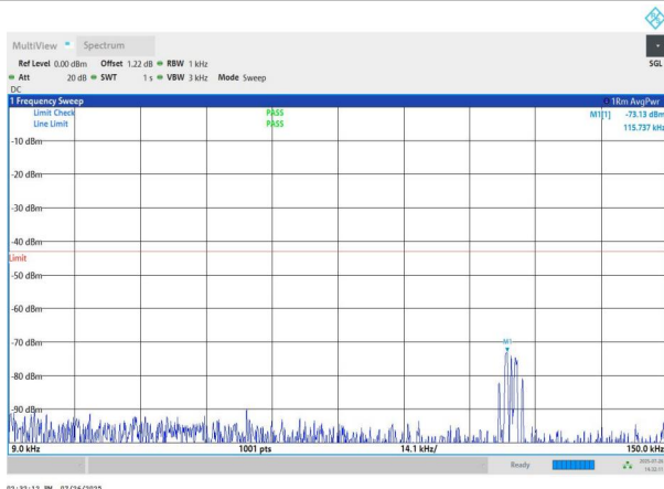
NTNV-n78(3700-3800)-PC2-30-40-H-DFT-BPSK-Edge_1RB_Left -0.009-0.15-PASS
