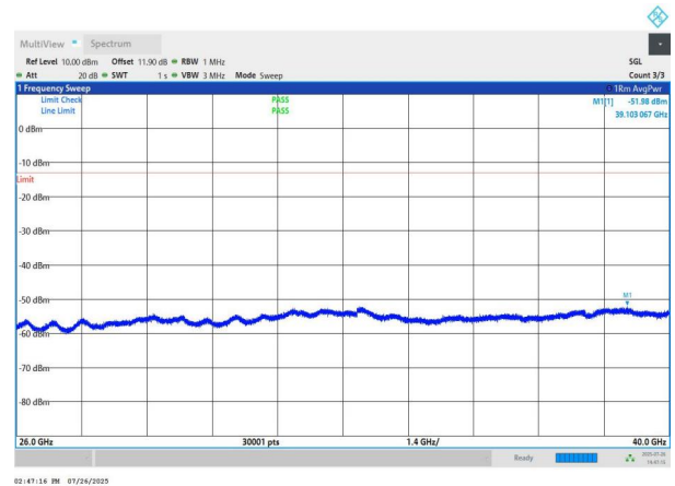
NTNV-n78(3700-3800)-PC2-30-60-L-DFT-QPSK-Edge_1RB_Left- 26000-40000-PASS
