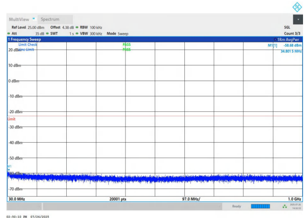
NTNV-n78(3700-3800)-PC2-30-60-M-DFT-QPSK-Edge_1RB_Left -30-1000-PASS
