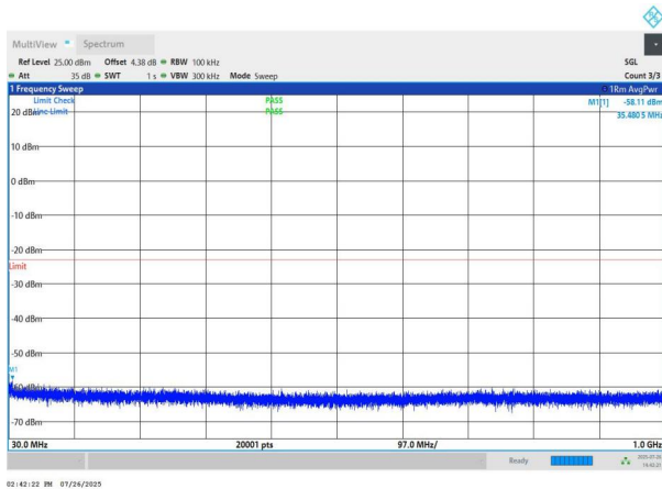
NTNV-n78(3700-3800)-PC2-30-50-H-DFT-BPSK-Edge_1RB_Left -30-1000-PASS
