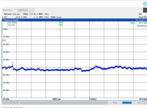
NTNV-n78(3700-3800)-PC2-30-50-H-DFT-QPSK-Edge_1RB_Left -6000-26000-PASS
