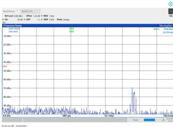
NTNV-n78(3700-3800)-PC2-30-50-M-DFT-BPSK-Edge_1RB_Left -0.009-0.15-PASS
