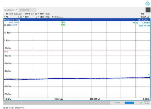
NTNV-n78(3700-3800)-PC2-30-50-H-DFT-BPSK-Edge_1RB_Left 1000-3000-PASS
