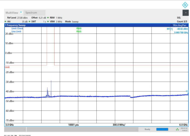
NTNV-n78(3700-3800)-PC2-30-60-L-DFT-QPSK-Edge_1RB_Left- 3000-6000-PASS
