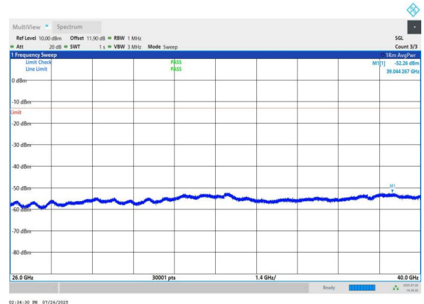
NTNV-n78(3700-3800)-PC2-30-40-H-DFT-QPSK-Edge_1RB_Left -26000-40000-PASS
