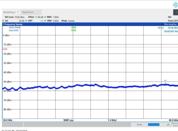
NTNV-n78(3700-3800)-PC2-30-50-H-DFT-BPSK-Edge_1RB_Left -26000-40000-PASS
