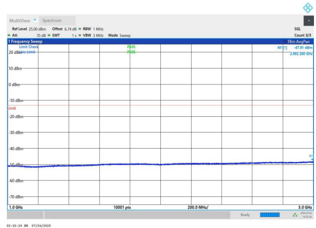
NTNV-n78(3700-3800)-PC2-30-40-H-DFT-BPSK-Edge_1RB_Left 1000-3000-PASS
