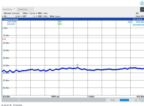
NTNV-n78(3700-3800)-PC2-30-60-M-DFT-BPSK-Edge_1RB_Left -26000-40000-PASS
