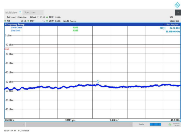
NTNV-n78(3700-3800)-PC2-30-40-L-DFT-QPSK-Edge_1RB_Left- 26000-40000-PASS
