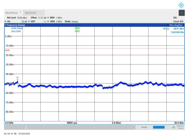
NTNV-n78(3700-3800)-PC2-30-50-M-DFT-BPSK-Edge_1RB_Left -6000-26000-PASS
