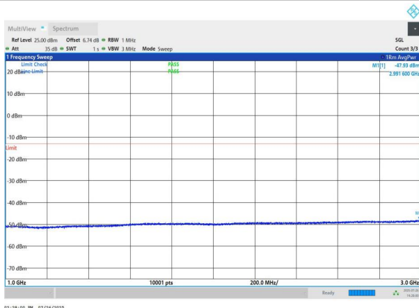
NTNV-n78(3700-3800)-PC2-30-40-L-DFT-QPSK-Edge_1RB_Left- 1000-3000-PASS
