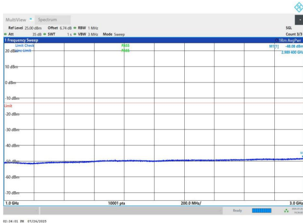
NTNV-n78(3700-3800)-PC2-30-40-H-DFT-QPSK-Edge_1RB_Left -1000-3000-PASS
