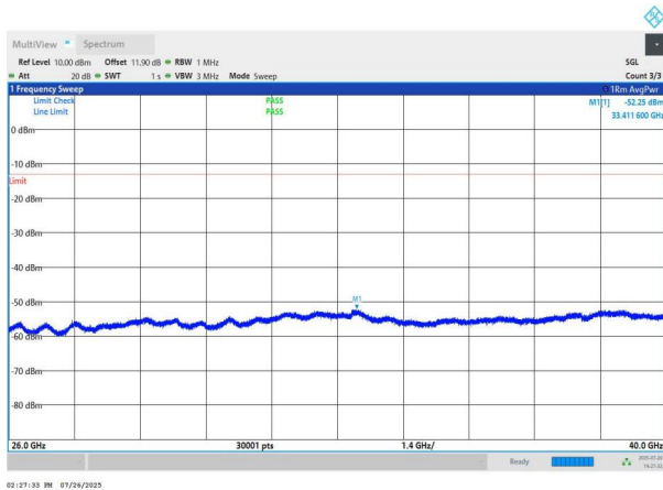
NTNV-n78(3700-3800)-PC2-30-40-L-DFT-BPSK-Edge_1RB_Left- 26000-40000-PASS
