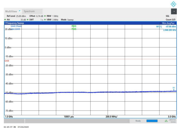
NTNV-n78(3700-3800)-PC2-30-60-L-DFT-BPSK-Edge_1RB_Left- 1000-3000-PASS
