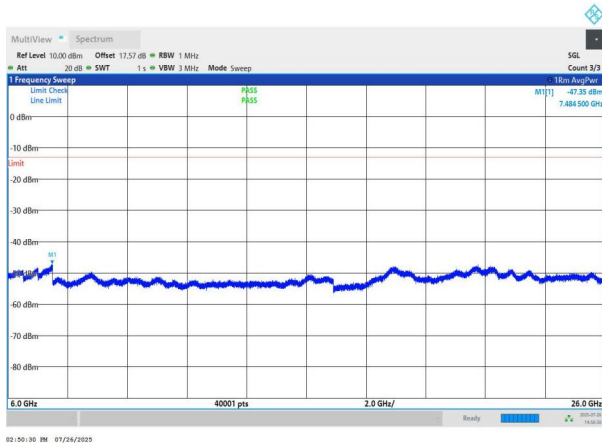
NTNV-n78(3700-3800)-PC2-30-60-M-DFT-QPSK-Edge_1RB_Left -6000-26000-PASS
