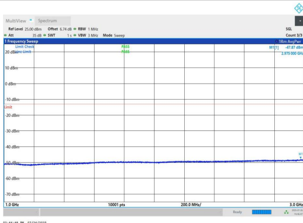
NTNV-n78(3700-3800)-PC2-30-60-L-DFT-QPSK-Edge_1RB_Left- 1000-3000-PASS
