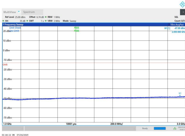
NTNV-n78(3700-3800)-PC2-30-50-H-DFT-QPSK-Edge_1RB_Left -1000-3000-PASS
