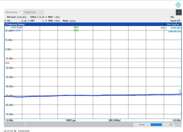
NTNV-n78(3700-3800)-PC2-30-40-L-DFT-BPSK-Edge_1RB_Left- 1000-3000-PASS
