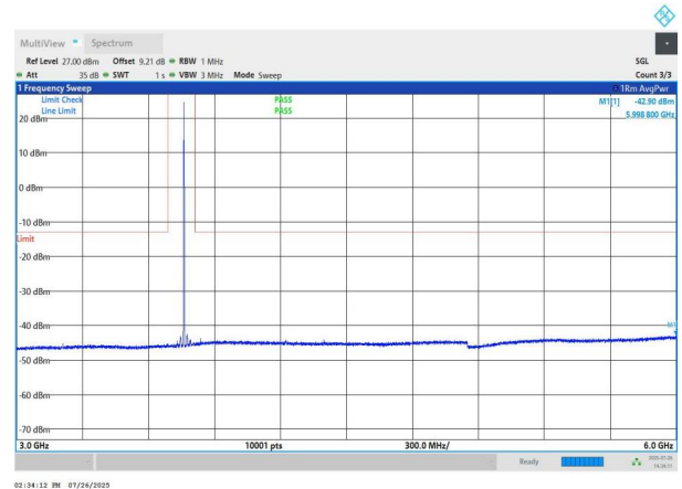
NTNV-n78(3700-3800)-PC2-30-40-H-DFT-QPSK-Edge_1RB_Left -3000-6000-PASS
