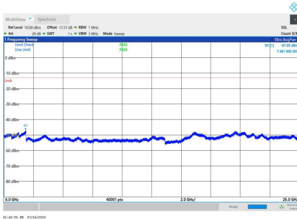
NTNV-n78(3700-3800)-PC2-30-50-M-DFT-QPSK-Edge_1RB_Left -6000-26000-PASS
