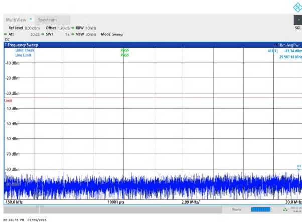
NTNV-n78(3700-3800)-PC2-30-60-L-DFT-QPSK-Edge_1RB_Left- 0.15-30-PASS
