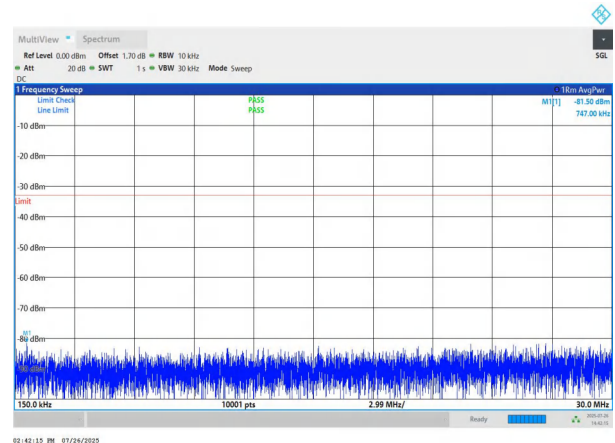
NTNV-n78(3700-3800)-PC2-30-50-H-DFT-BPSK-Edge_1RB_Left 0.15-30-PASS
