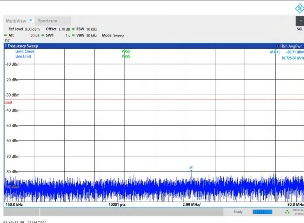
NTNV-n78(3700-3800)-PC2-30-50-M-DFT-QPSK-Edge_1RB_Left -0.15-30-PASS
