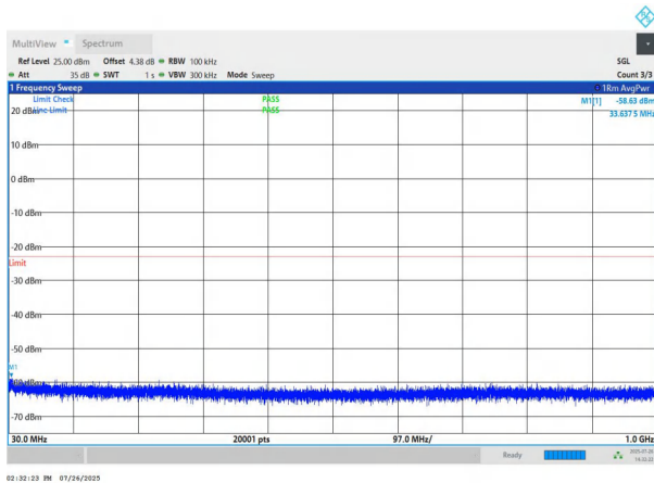
NTNV-n78(3700-3800)-PC2-30-40-H-DFT-BPSK-Edge_1RB_Left -30-1000-PASS
