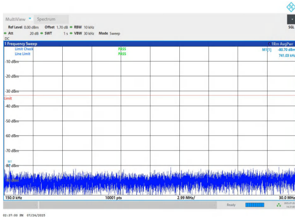
NTNV-n78(3700-3800)-PC2-30-50-L-DFT-QPSK-Edge_1RB_Left- 0.15-30-PASS
