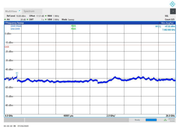
NTNV-n78(3700-3800)-PC2-30-40-H-DFT-BPSK-Edge_1RB_Left 6000-26000-PASS
