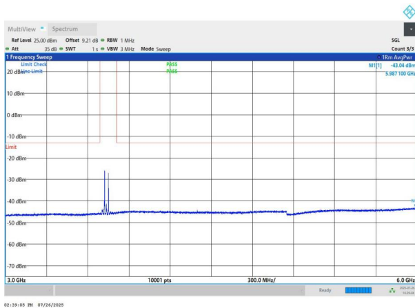
NTNV-n78(3700-3800)-PC2-30-50-M-DFT-BPSK-Edge_1RB_Left -3000-6000-PASS
