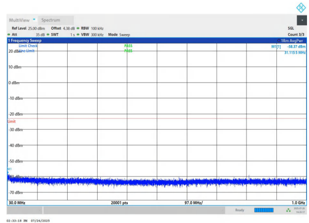
NTNV-n78(3700-3800)-PC2-30-40-H-DFT-QPSK-Edge_1RB_Left -30-1000-PASS
