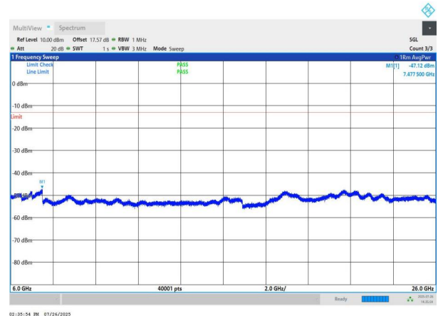
NTNV-n78(3700-3800)-PC2-30-50-L-DFT-BPSK-Edge_1RB_Left- 6000-26000-PASS
