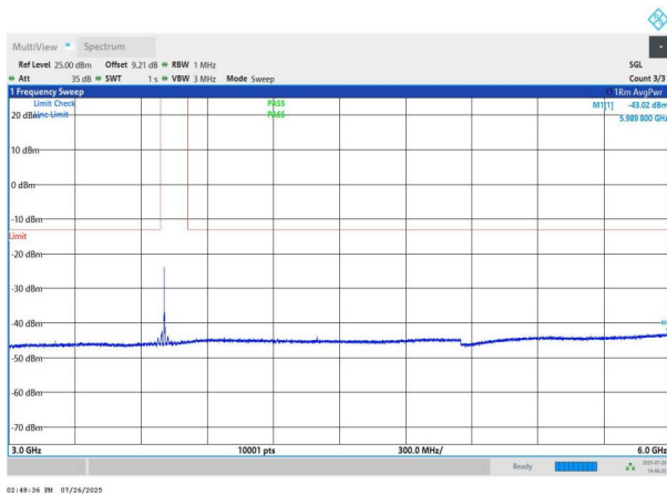
NTNV-n78(3700-3800)-PC2-30-60-M-DFT-BPSK-Edge_1RB_Left -3000-6000-PASS
