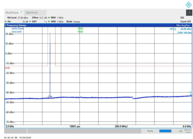
NTNV-n78(3700-3800)-PC2-30-50-M-DFT-QPSK-Edge_1RB_Left -3000-6000-PASS
