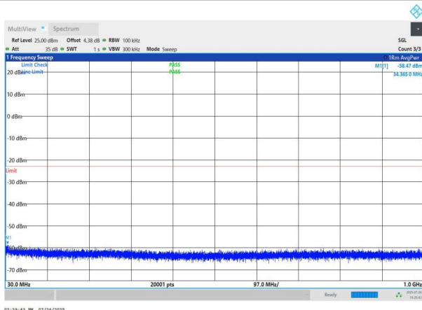
NTNV-n78(3700-3800)-PC2-30-40-M-DFT-BPSK-Edge_1RB_Left -30-1000-PASS
