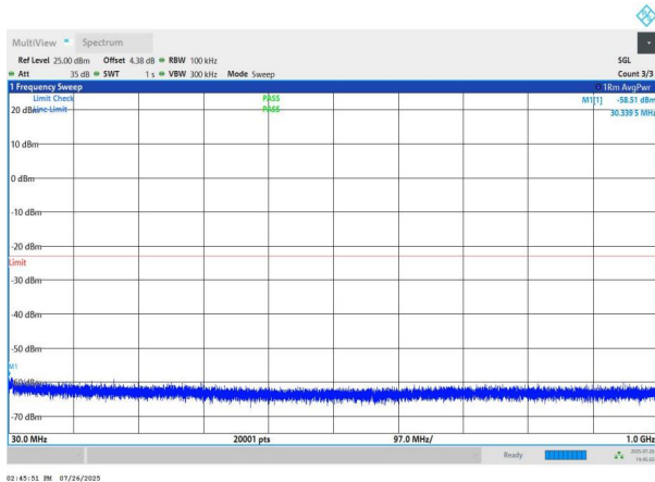
NTNV-n78(3700-3800)-PC2-30-60-L-DFT-BPSK-Edge_1RB_Left- 30-1000-PASS
