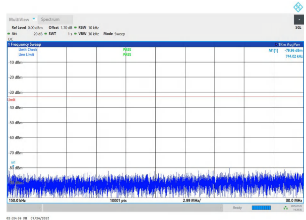
NTNV-n78(3700-3800)-PC2-30-40-M-DFT-BPSK-Edge_1RB_Left -0.15-30-PASS
