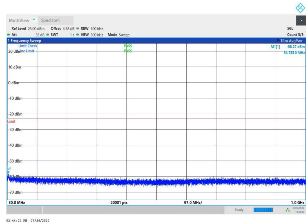
NTNV-n78(3700-3800)-PC2-30-50-H-DFT-QPSK-Edge_1RB_Left -30-1000-PASS
