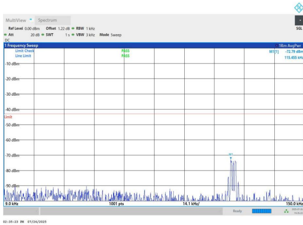
NTNV-n78(3700-3800)-PC2-30-50-L-DFT-BPSK-Edge_1RB_Left- 0.009-0.15-PASS
