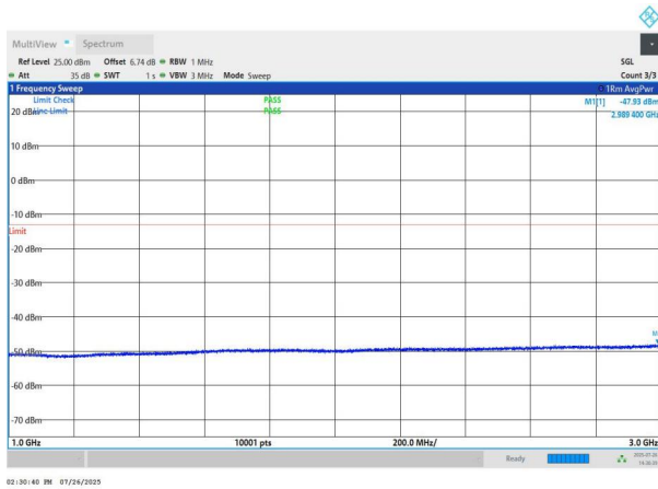
NTNV-n78(3700-3800)-PC2-30-40-M-DFT-QPSK-Edge_1RB_Left -1000-3000-PASS
