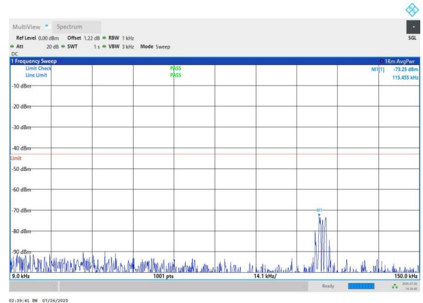
NTNV-n78(3700-3800)-PC2-30-50-M-DFT-QPSK-Edge_1RB_Left -0.009-0.15-PASS
