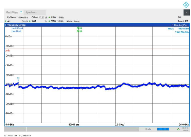
NTNV-n78(3700-3800)-PC2-30-40-M-DFT-BPSK-Edge_1RB_Left -6000-26000-PASS
