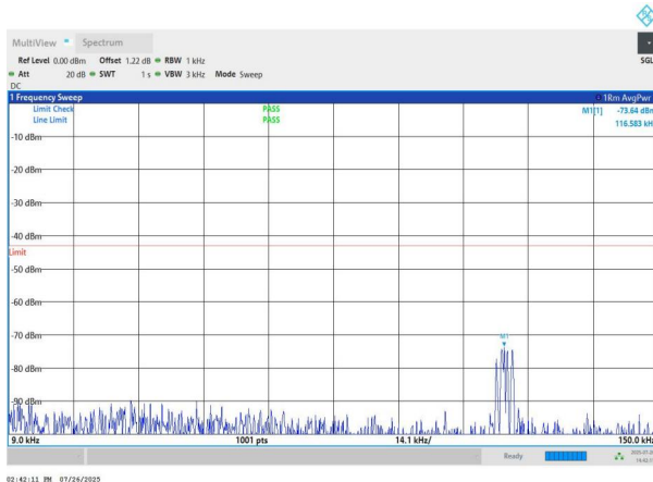
NTNV-n78(3700-3800)-PC2-30-50-H-DFT-BPSK-Edge_1RB_Left -0.009-0.15-PASS
