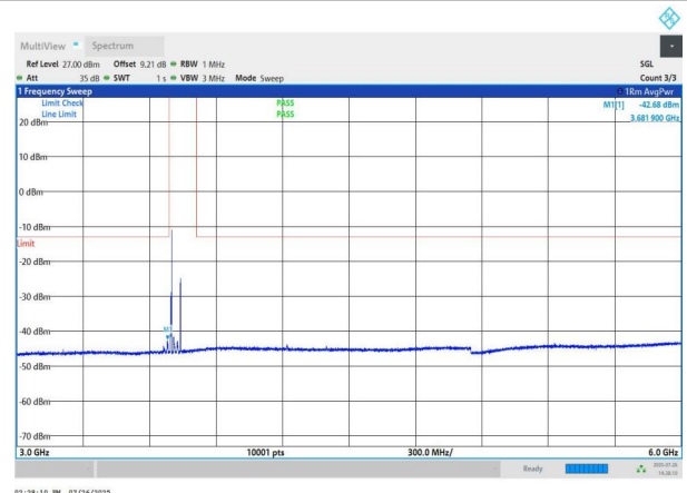
NTNV-n78(3700-3800)-PC2-30-40-L-DFT-QPSK-Edge_1RB_Left- 3000-6000-PASS
