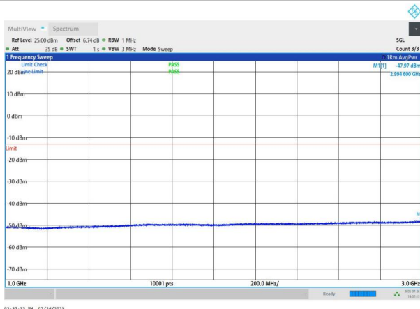
NTNV-n78(3700-3800)-PC2-30-50-L-DFT-QPSK-Edge_1RB_Left- 1000-3000-PASS
