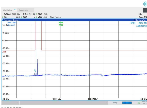
NTNV-n78(3700-3800)-PC2-30-60-L-DFT-BPSK-Edge_1RB_Left- 3000-6000-PASS
