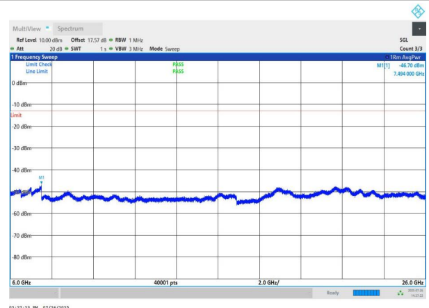
NTNV-n78(3700-3800)-PC2-30-40-L-DFT-BPSK-Edge_1RB_Left- 6000-26000-PASS
