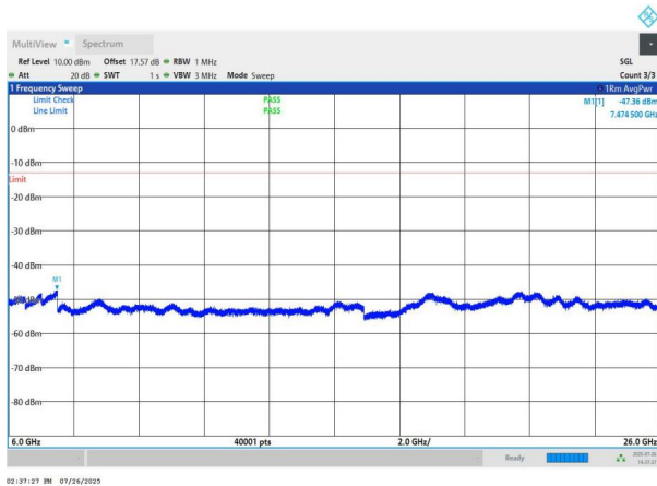
NTNV-n78(3700-3800)-PC2-30-50-L-DFT-QPSK-Edge_1RB_Left- 6000-26000-PASS
