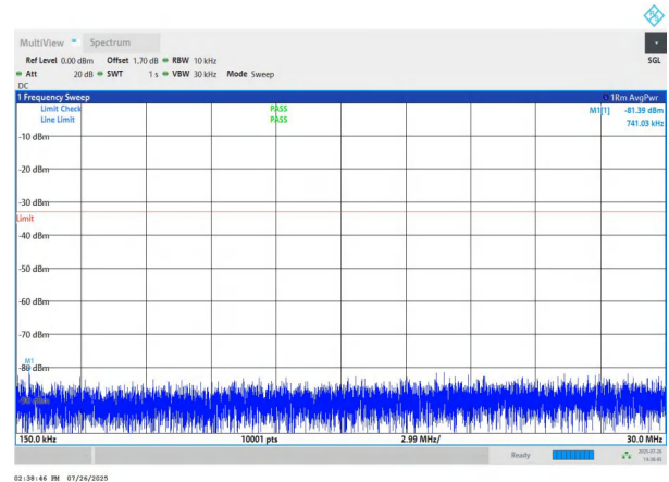
NTNV-n78(3700-3800)-PC2-30-50-M-DFT-BPSK-Edge_1RB_Left -0.15-30-PASS
