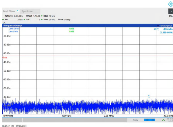
NTNV-n78(3700-3800)-PC2-30-40-L-DFT-QPSK-Edge_1RB_Left- 0.15-30-PASS
