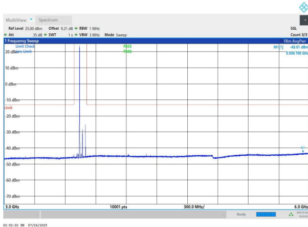
NTNV-n78(3700-3800)-PC2-30-60-H-DFT-BPSK-Edge_1RB_Left -3000-6000-PASS
