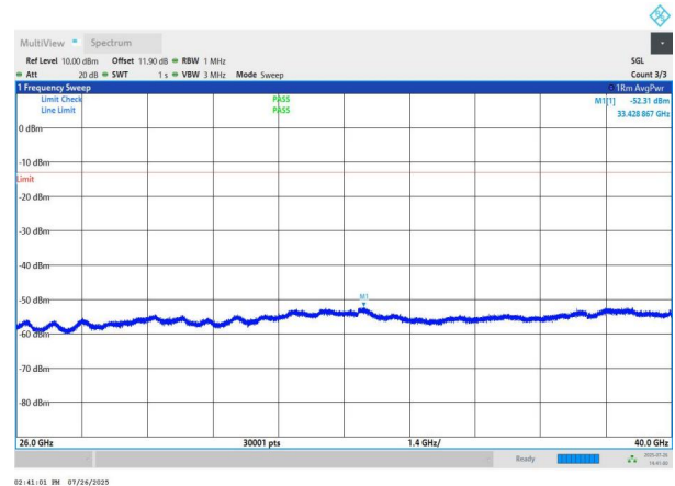
NTNV-n78(3700-3800)-PC2-30-50-M-DFT-QPSK-Edge_1RB_Left -26000-40000-PASS
