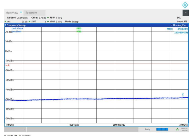
NTNV-n78(3700-3800)-PC2-30-40-M-DFT-BPSK-Edge_1RB_Left -1000-3000-PASS
