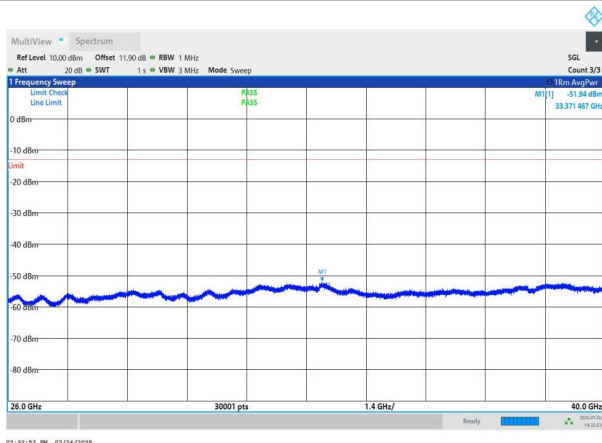
NTNV-n78(3700-3800)-PC2-30-40-H-DFT-BPSK-Edge_1RB_Left -26000-40000-PASS
