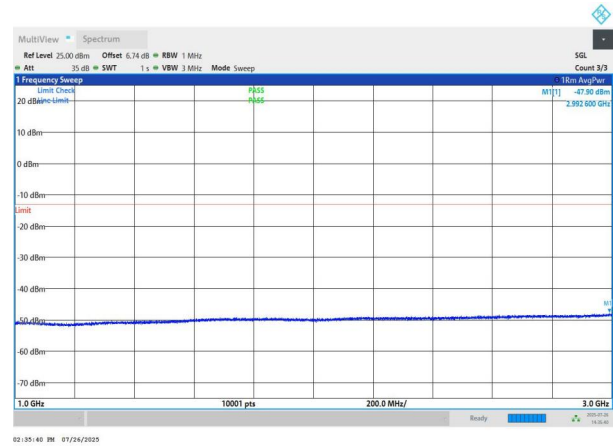
NTNV-n78(3700-3800)-PC2-30-50-L-DFT-BPSK-Edge_1RB_Left- 1000-3000-PASS
