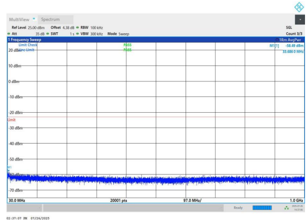
NTNV-n78(3700-3800)-PC2-30-50-L-DFT-QPSK-Edge_1RB_Left- 30-1000-PASS
