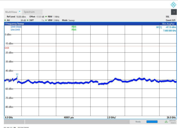
NTNV-n78(3700-3800)-PC2-30-60-L-DFT-BPSK-Edge_1RB_Left- 6000-26000-PASS
