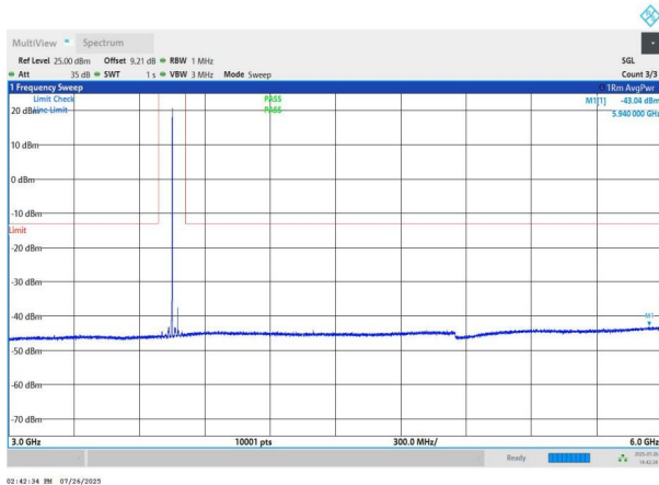
NTNV-n78(3700-3800)-PC2-30-50-H-DFT-BPSK-Edge_1RB_Left -3000-6000-PASS
