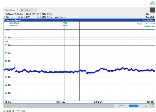
NTNV-n78(3700-3800)-PC2-30-50-H-DFT-BPSK-Edge_1RB_Left 6000-26000-PASS
