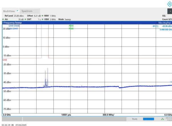
NTNV-n78(3700-3800)-PC2-30-40-H-DFT-BPSK-Edge_1RB_Left -3000-6000-PASS
