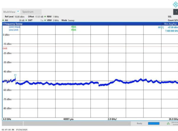
NTNV-n78(3700-3800)-PC2-30-60-L-DFT-QPSK-Edge_1RB_Left- 6000-26000-PASS
