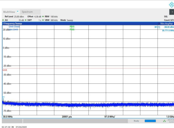
NTNV-n78(3700-3800)-PC2-30-40-L-DFT-BPSK-Edge_1RB_Left- 30-1000-PASS
