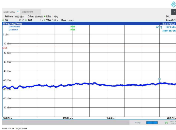
NTNV-n78(3700-3800)-PC2-30-80-L-DFT-BPSK-Edge_1RB_Left- 26000-40000-PASS
