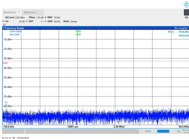
NTNV-n78(3700-3800)-PC2-30-90-L-DFT-QPSK-Edge_1RB_Left- 0.15-30-PASS
