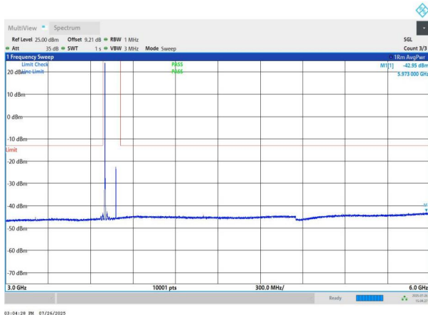
NTNV-n78(3700-3800)-PC2-30-80-L-DFT-BPSK-Edge_1RB_Left- 3000-6000-PASS
