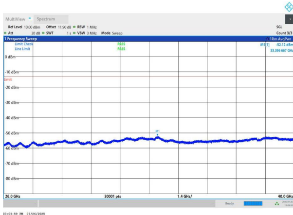
NTNV-n78(3700-3800)-PC2-30-80-H-DFT-BPSK-Edge_1RB_Left -26000-40000-PASS
