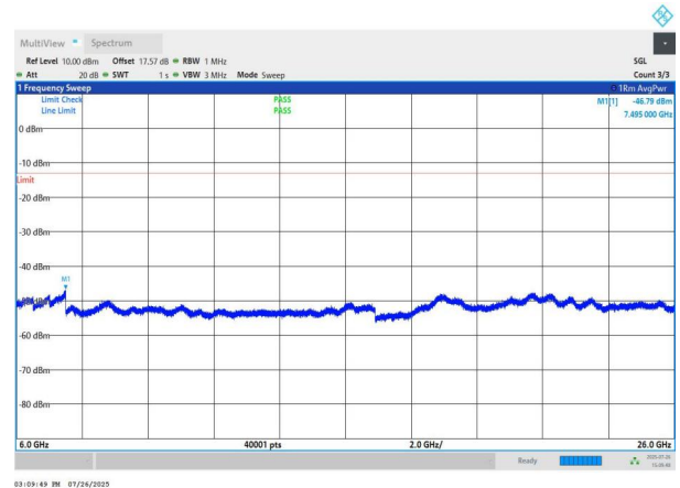
NTNV-n78(3700-3800)-PC2-30-80-H-DFT-BPSK-Edge_1RB_Left 6000-26000-PASS
