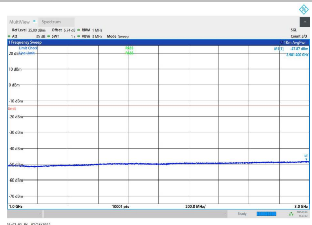
NTNV-n78(3700-3800)-PC2-30-80-M-DFT-BPSK-Edge_1RB_Left -1000-3000-PASS
