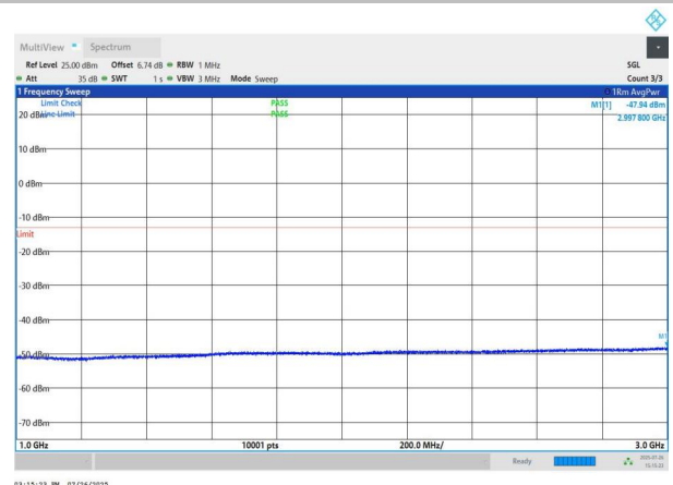
NTNV-n78(3700-3800)-PC2-30-90-M-DFT-BPSK-Edge_1RB_Left -1000-3000-PASS
