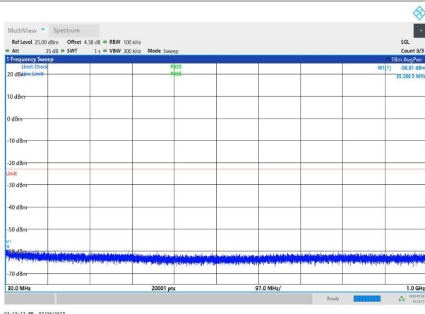
NTNV-n78(3700-3800)-PC2-30-90-M-DFT-BPSK-Edge_1RB_Left -30-1000-PASS
