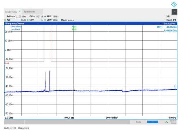
NTNV-n78(3700-3800)-PC2-30-70-M-DFT-QPSK-Edge_1RB_Left -3000-6000-PASS
