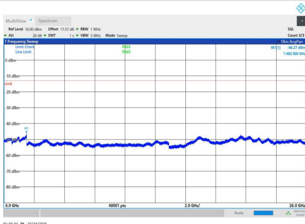
NTNV-n78(3700-3800)-PC2-30-60-H-DFT-QPSK-Edge_1RB_Left -6000-26000-PASS
