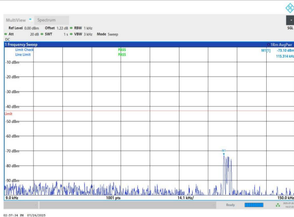
NTNV-n78(3700-3800)-PC2-30-70-M-DFT-BPSK-Edge_1RB_Left -0.009-0.15-PASS
