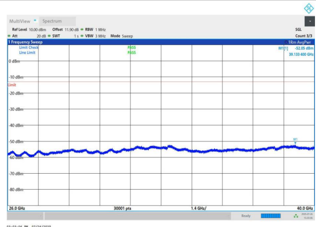
NTNV-n78(3700-3800)-PC2-30-70-H-DFT-QPSK-Edge_1RB_Left -26000-40000-PASS
