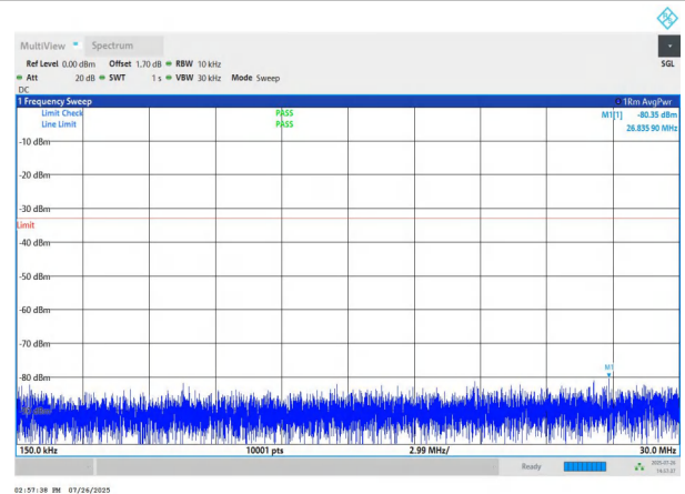
NTNV-n78(3700-3800)-PC2-30-70-M-DFT-BPSK-Edge_1RB_Left -0.15-30-PASS
