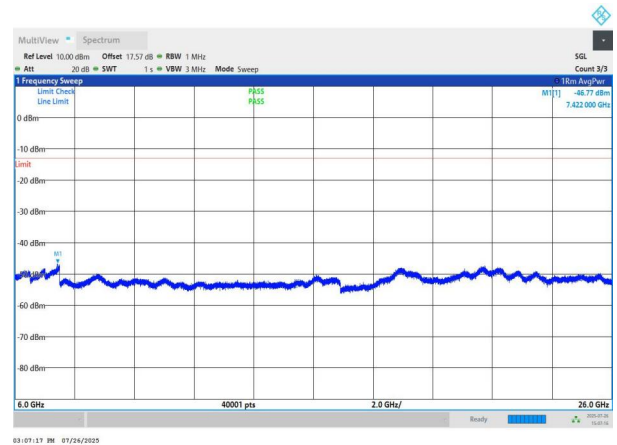
NTNV-n78(3700-3800)-PC2-30-80-M-DFT-BPSK-Edge_1RB_Left -6000-26000-PASS
