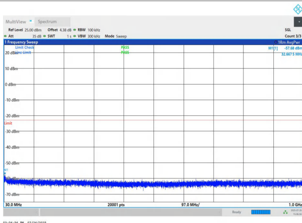
NTNV-n78(3700-3800)-PC2-30-80-M-DFT-BPSK-Edge_1RB_Left -30-1000-PASS
