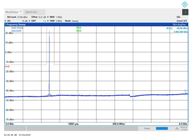
NTNV-n78(3700-3800)-PC2-30-70-H-DFT-QPSK-Edge_1RB_Left -3000-6000-PASS
