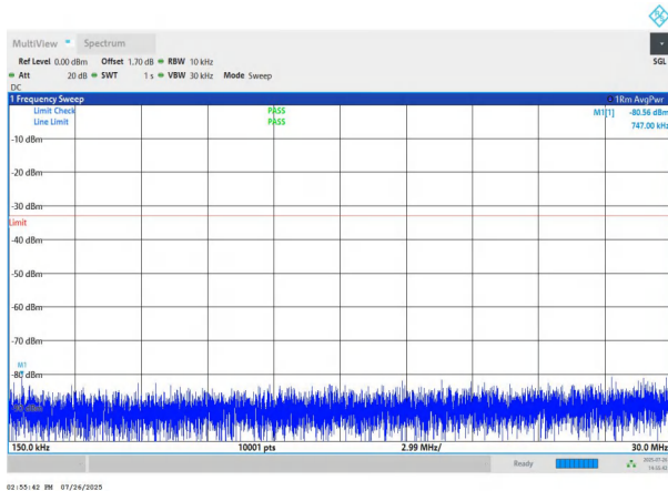
NTNV-n78(3700-3800)-PC2-30-70-L-DFT-QPSK-Edge_1RB_Left- 0.15-30-PASS
