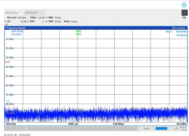
NTNV-n78(3700-3800)-PC2-30-80-M-DFT-BPSK-Edge_1RB_Left -0.15-30-PASS
