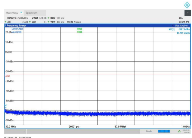
NTNV-n78(3700-3800)-PC2-30-70-M-DFT-QPSK-Edge_1RB_Left -30-1000-PASS
