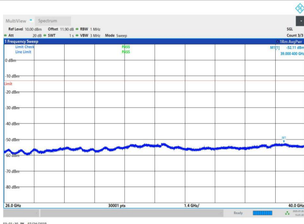
NTNV-n78(3700-3800)-PC2-30-70-H-DFT-BPSK-Edge_1RB_Left -26000-40000-PASS
