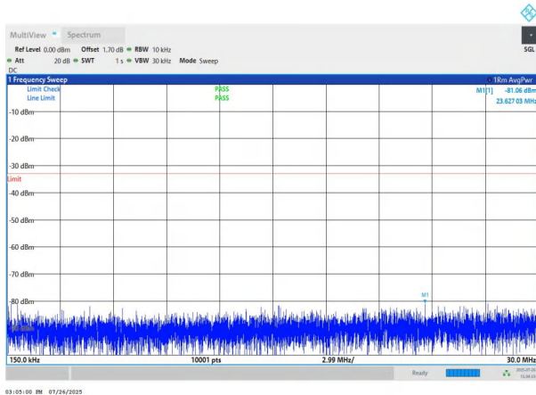
NTNV-n78(3700-3800)-PC2-30-80-L-DFT-QPSK-Edge_1RB_Left- 0.15-30-PASS
