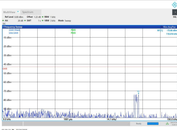
NTNV-n78(3700-3800)-PC2-30-80-H-DFT-BPSK-Edge_1RB_Left -0.009-0.15-PASS
