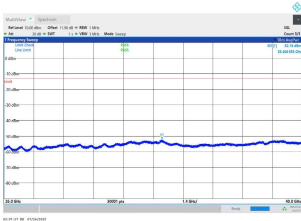
NTNV-n78(3700-3800)-PC2-30-80-M-DFT-BPSK-Edge_1RB_Left -26000-40000-PASS
