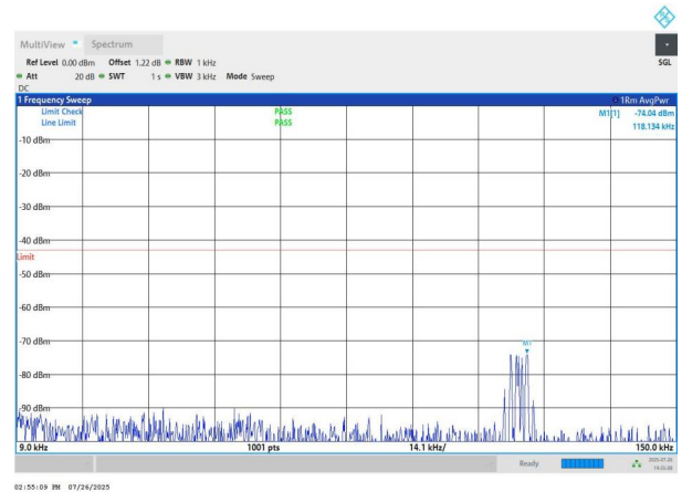
NTNV-n78(3700-3800)-PC2-30-70-L-DFT-QPSK-Edge_1RB_Left- 0.009-0.15-PASS
