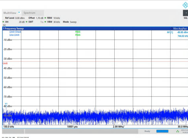
NTNV-n78(3700-3800)-PC2-30-70-M-DFT-QPSK-Edge_1RB_Left -0.15-30-PASS
