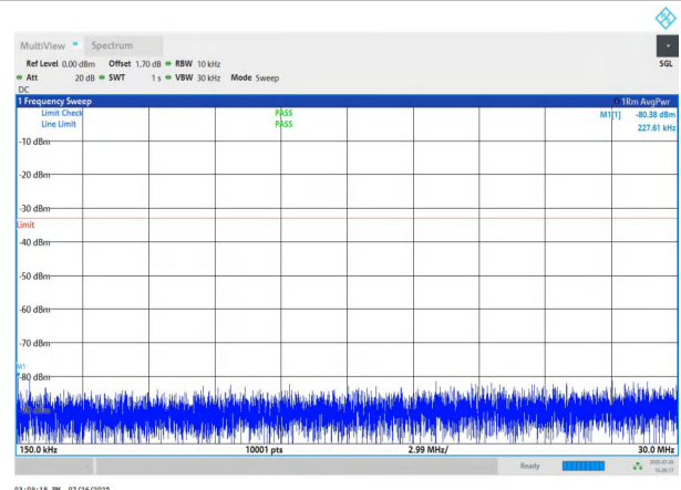
NTNV-n78(3700-3800)-PC2-30-80-H-DFT-BPSK-Edge_1RB_Left 0.15-30-PASS
