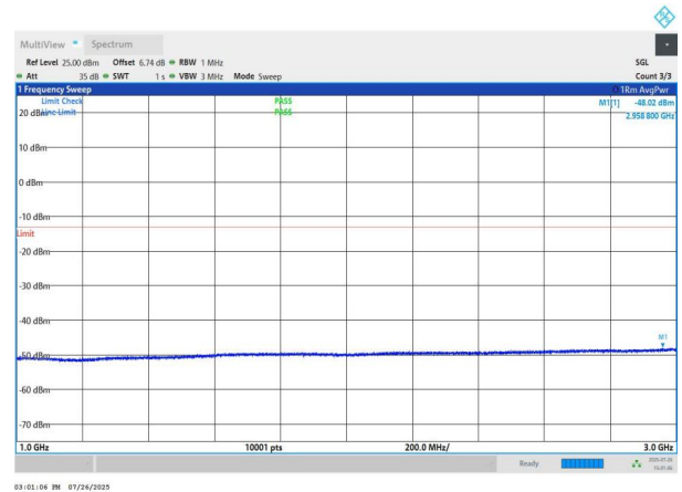
NTNV-n78(3700-3800)-PC2-30-70-H-DFT-BPSK-Edge_1RB_Left 1000-3000-PASS
