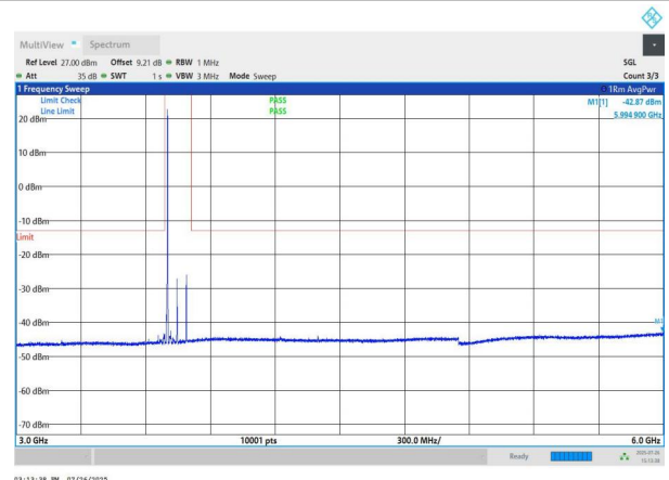
NTNV-n78(3700-3800)-PC2-30-90-L-DFT-QPSK-Edge_1RB_Left- 3000-6000-PASS
