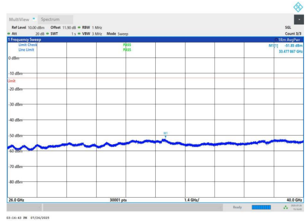
NTNV-n78(3700-3800)-PC2-30-90-M-DFT-QPSK-Edge_1RB_Left -26000-40000-PASS
