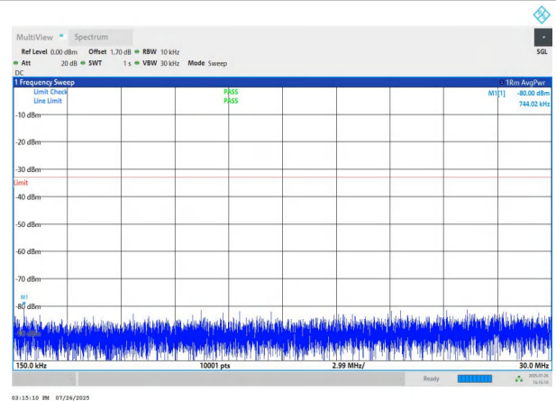
NTNV-n78(3700-3800)-PC2-30-90-M-DFT-BPSK-Edge_1RB_Left -0.15-30-PASS
