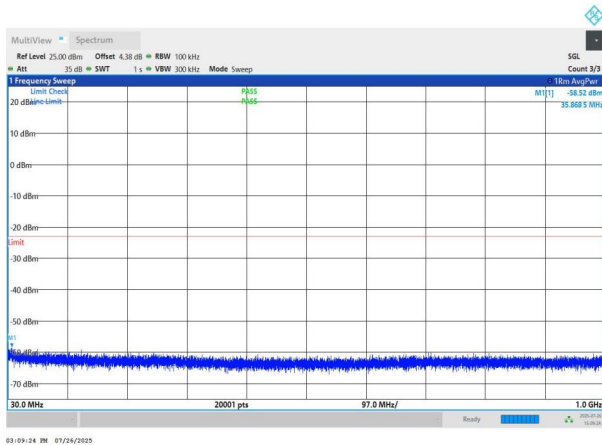
NTNV-n78(3700-3800)-PC2-30-80-H-DFT-BPSK-Edge_1RB_Left -30-1000-PASS
