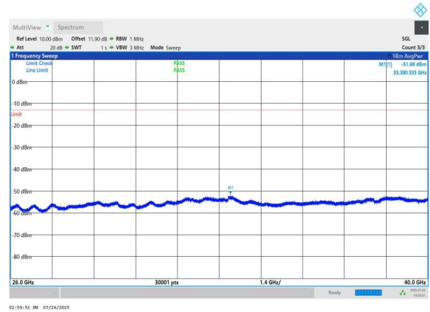
NTNV-n78(3700-3800)-PC2-30-70-M-DFT-QPSK-Edge_1RB_Left -26000-40000-PASS
