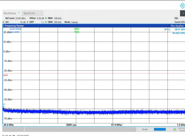
NTNV-n78(3700-3800)-PC2-30-70-M-DFT-BPSK-Edge_1RB_Left -30-1000-PASS
