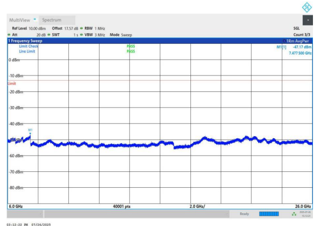
NTNV-n78(3700-3800)-PC2-30-90-L-DFT-BPSK-Edge_1RB_Left- 6000-26000-PASS
