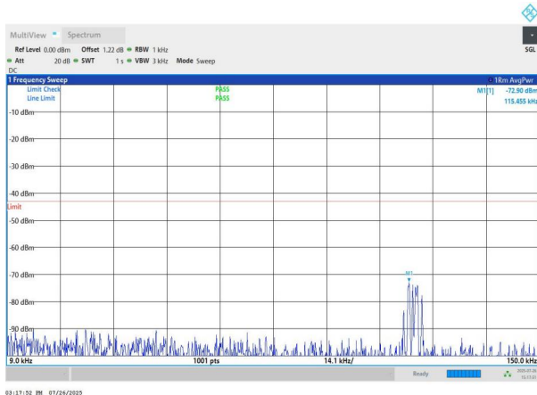
NTNV-n78(3700-3800)-PC2-30-90-H-DFT-BPSK-Edge_1RB_Left -0.009-0.15-PASS
