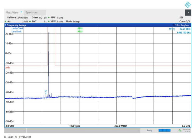
NTNV-n78(3700-3800)-PC2-30-90-M-DFT-QPSK-Edge_1RB_Left -3000-6000-PASS
