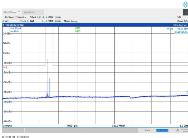
NTNV-n78(3700-3800)-PC2-30-80-H-DFT-BPSK-Edge_1RB_Left -3000-6000-PASS
