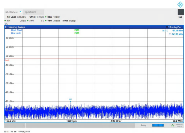
NTNV-n78(3700-3800)-PC2-30-90-L-DFT-BPSK-Edge_1RB_Left- 0.15-30-PASS
