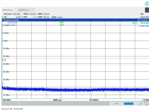
NTNV-n78(3700-3800)-PC2-30-70-H-DFT-BPSK-Edge_1RB_Left -30-1000-PASS
