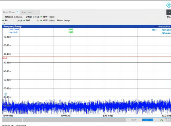
NTNV-n78(3700-3800)-PC2-30-90-M-DFT-QPSK-Edge_1RB_Left -0.15-30-PASS
