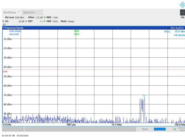
NTNV-n78(3700-3800)-PC2-30-80-L-DFT-BPSK-Edge_1RB_Left- 0.009-0.15-PASS
