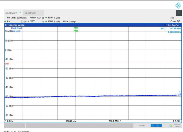
NTNV-n78(3700-3800)-PC2-30-70-M-DFT-BPSK-Edge_1RB_Left -1000-3000-PASS
