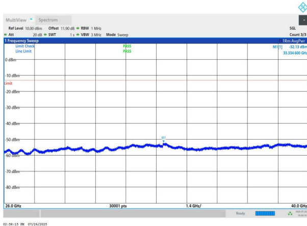
NTNV-n78(3700-3800)-PC2-30-70-M-DFT-BPSK-Edge_1RB_Left -26000-40000-PASS
