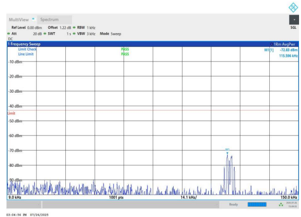
NTNV-n78(3700-3800)-PC2-30-80-L-DFT-QPSK-Edge_1RB_Left- 0.009-0.15-PASS
