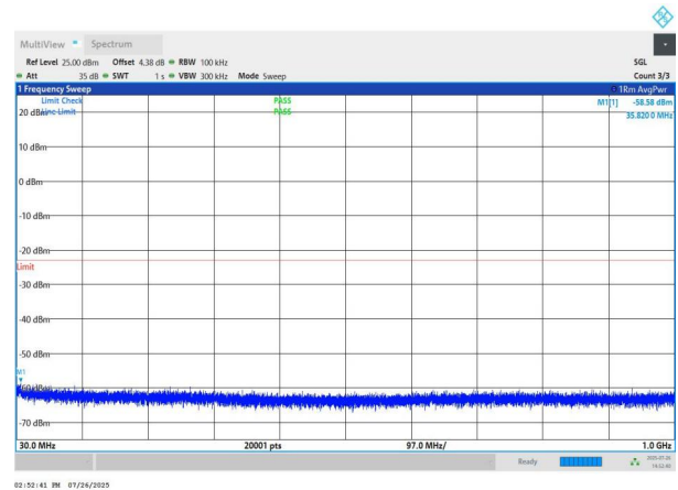
NTNV-n78(3700-3800)-PC2-30-60-H-DFT-QPSK-Edge_1RB_Left -30-1000-PASS
