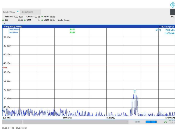
NTNV-n78(3700-3800)-PC2-30-90-M-DFT-BPSK-Edge_1RB_Left -0.009-0.15-PASS
