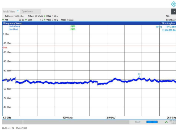
NTNV-n78(3700-3800)-PC2-30-70-M-DFT-QPSK-Edge_1RB_Left -6000-26000-PASS
