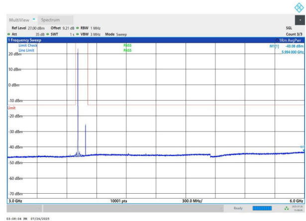
NTNV-n78(3700-3800)-PC2-30-80-M-DFT-QPSK-Edge_1RB_Left -3000-6000-PASS
