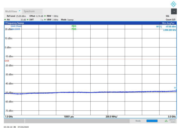
NTNV-n78(3700-3800)-PC2-30-80-L-DFT-BPSK-Edge_1RB_Left- 1000-3000-PASS
