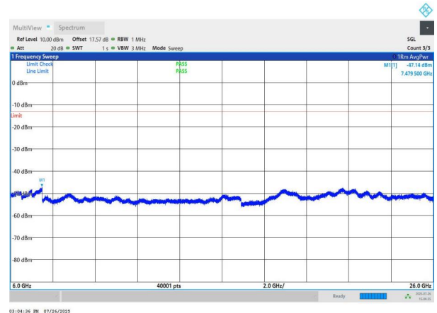
NTNV-n78(3700-3800)-PC2-30-80-L-DFT-BPSK-Edge_1RB_Left- 6000-26000-PASS
