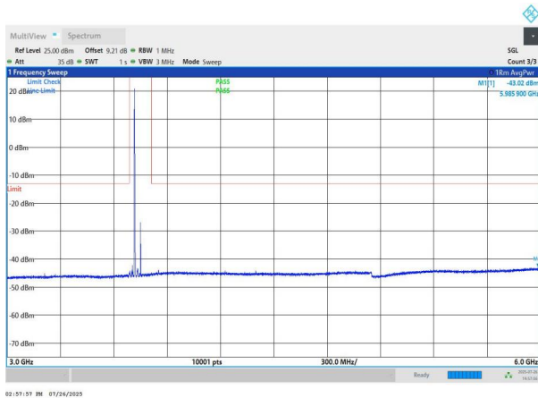
NTNV-n78(3700-3800)-PC2-30-70-M-DFT-BPSK-Edge_1RB_Left -3000-6000-PASS
