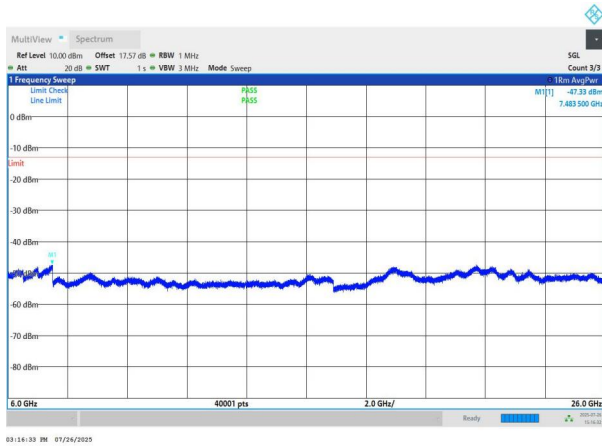
NTNV-n78(3700-3800)-PC2-30-90-M-DFT-QPSK-Edge_1RB_Left -6000-26000-PASS
