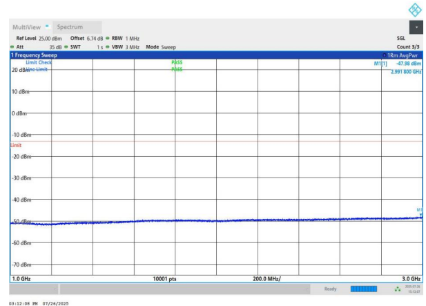
NTNV-n78(3700-3800)-PC2-30-90-L-DFT-BPSK-Edge_1RB_Left- 1000-3000-PASS
