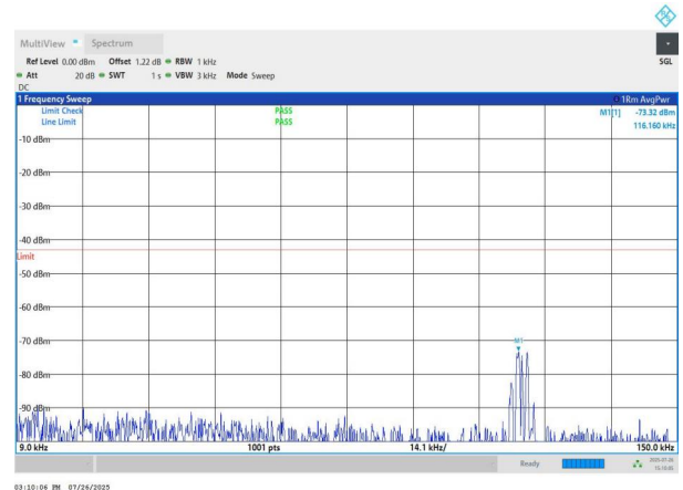
NTNV-n78(3700-3800)-PC2-30-80-H-DFT-QPSK-Edge_1RB_Left -0.009-0.15-PASS
