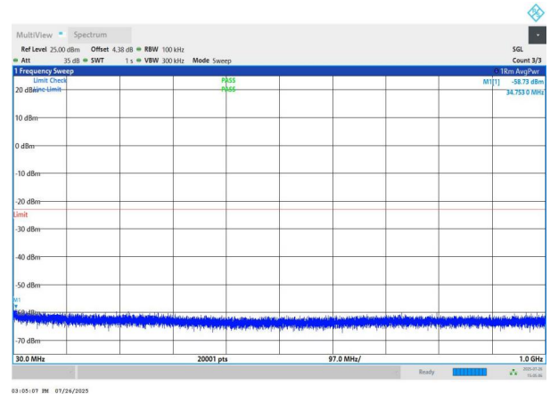
NTNV-n78(3700-3800)-PC2-30-80-L-DFT-QPSK-Edge_1RB_Left- 30-1000-PASS
