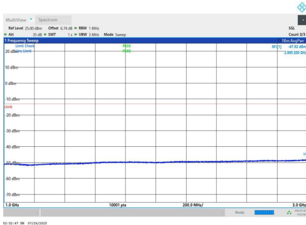
NTNV-n78(3700-3800)-PC2-30-60-H-DFT-QPSK-Edge_1RB_Left -1000-3000-PASS
