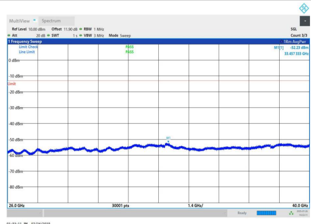
NTNV-n78(3700-3800)-PC2-30-60-H-DFT-QPSK-Edge_1RB_Left -26000-40000-PASS
