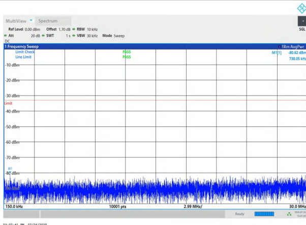
NTNV-n78(3700-3800)-PC2-30-80-M-DFT-QPSK-Edge_1RB_Left -0.15-30-PASS
