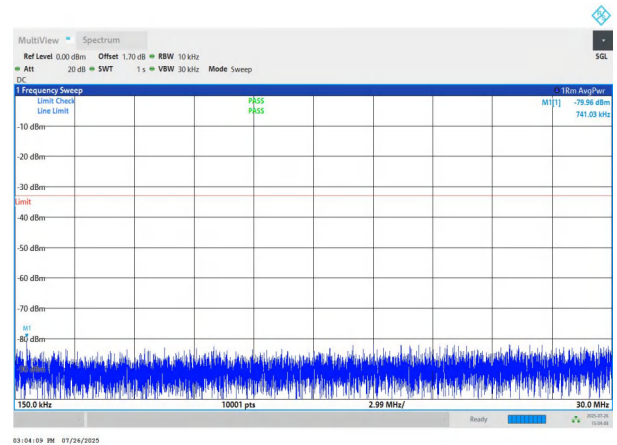
NTNV-n78(3700-3800)-PC2-30-80-L-DFT-BPSK-Edge_1RB_Left- 0.15-30-PASS
