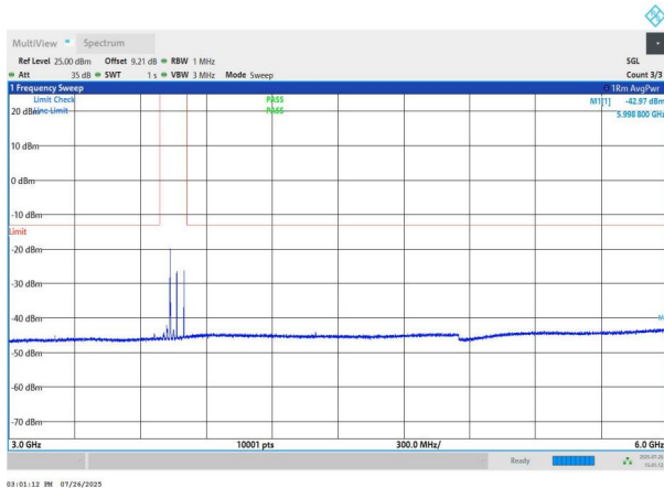
NTNV-n78(3700-3800)-PC2-30-70-H-DFT-BPSK-Edge_1RB_Left -3000-6000-PASS
