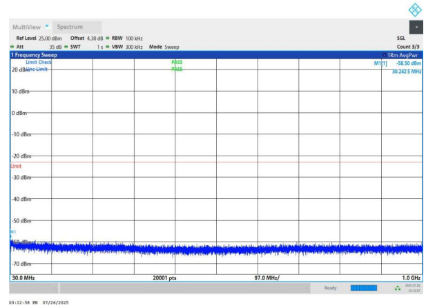
NTNV-n78(3700-3800)-PC2-30-90-L-DFT-QPSK-Edge_1RB_Left- 30-1000-PASS
