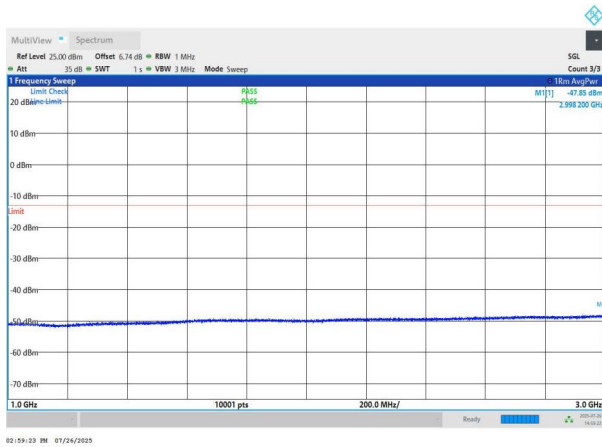
NTNV-n78(3700-3800)-PC2-30-70-M-DFT-QPSK-Edge_1RB_Left -1000-3000-PASS
