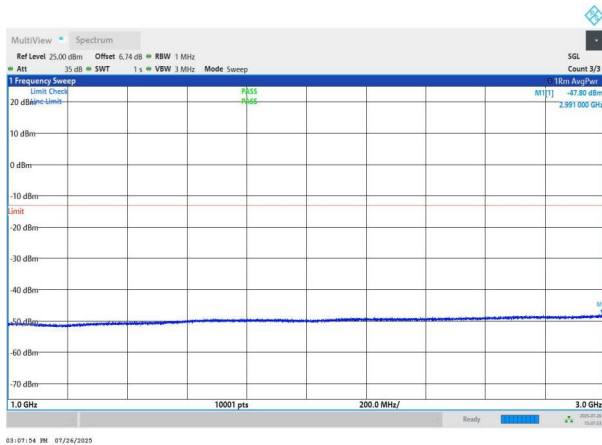
NTNV-n78(3700-3800)-PC2-30-80-M-DFT-QPSK-Edge_1RB_Left -1000-3000-PASS
