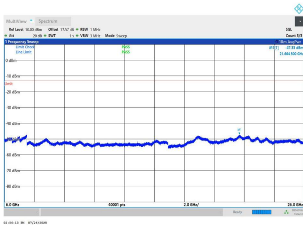
NTNV-n78(3700-3800)-PC2-30-70-L-DFT-QPSK-Edge_1RB_Left 6000-26000-PASS
