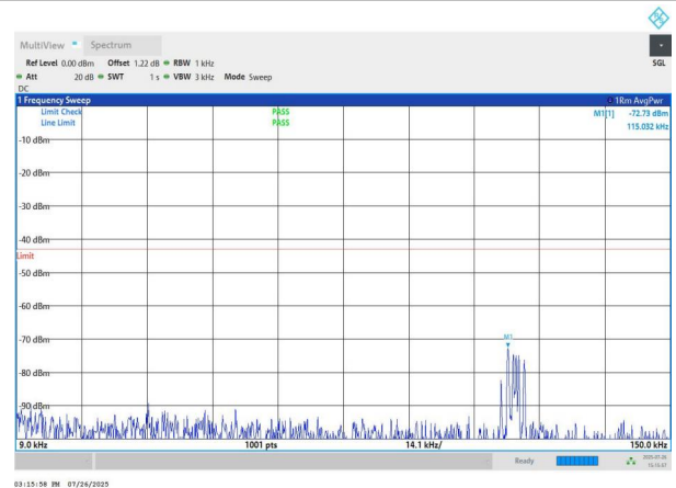
NTNV-n78(3700-3800)-PC2-30-90-M-DFT-QPSK-Edge_1RB_Left -0.009-0.15-PASS
