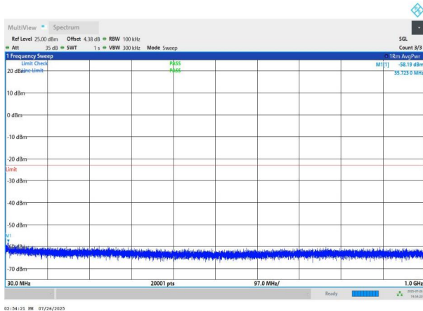
NTNV-n78(3700-3800)-PC2-30-70-L-DFT-BPSK-Edge_1RB_Left- 30-1000-PASS
