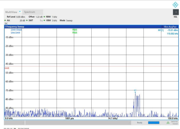
NTNV-n78(3700-3800)-PC2-30-70-H-DFT-QPSK-Edge_1RB_Left -0.009-0.15-PASS
