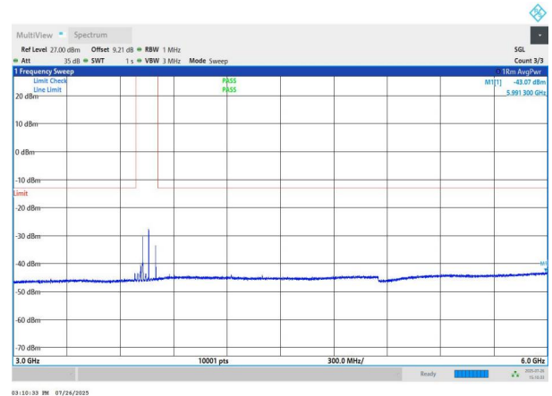
NTNV-n78(3700-3800)-PC2-30-80-H-DFT-QPSK-Edge_1RB_Left -3000-6000-PASS
