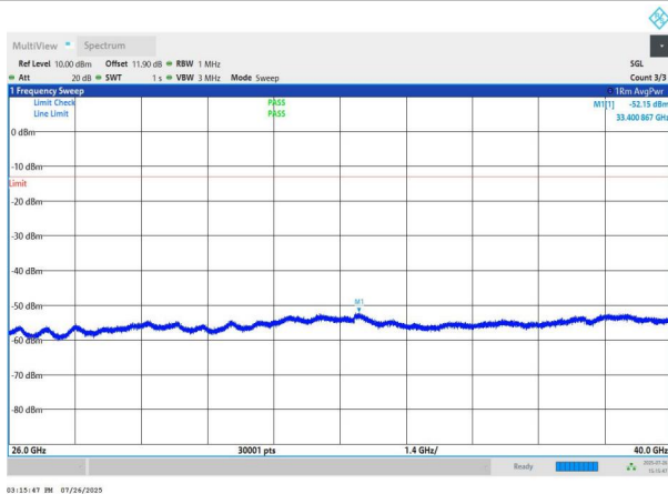
NTNV-n78(3700-3800)-PC2-30-90-M-DFT-BPSK-Edge_1RB_Left -26000-40000-PASS
