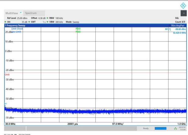
NTNV-n78(3700-3800)-PC2-30-90-M-DFT-QPSK-Edge_1RB_Left -30-1000-PASS
