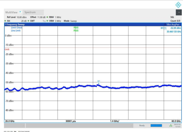
NTNV-n78(3700-3800)-PC2-30-80-H-DFT-QPSK-Edge_1RB_Left -26000-40000-PASS
