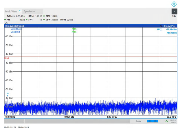
NTNV-n78(3700-3800)-PC2-30-70-H-DFT-BPSK-Edge_1RB_Left 0.15-30-PASS
