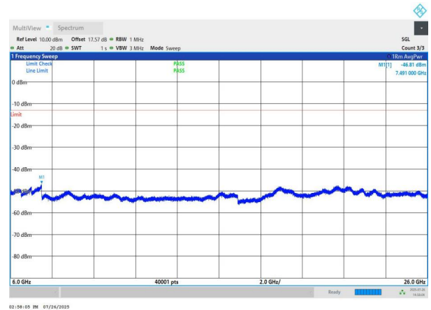
NTNV-n78(3700-3800)-PC2-30-70-M-DFT-BPSK-Edge_1RB_Left -6000-26000-PASS
