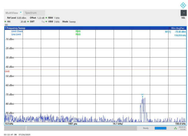
NTNV-n78(3700-3800)-PC2-30-90-L-DFT-QPSK-Edge_1RB_Left- 0.009-0.15-PASS
