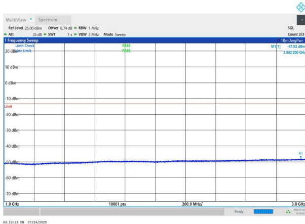
NTNV-n78(3700-3800)-PC2-30-80-H-DFT-QPSK-Edge_1RB_Left -1000-3000-PASS
