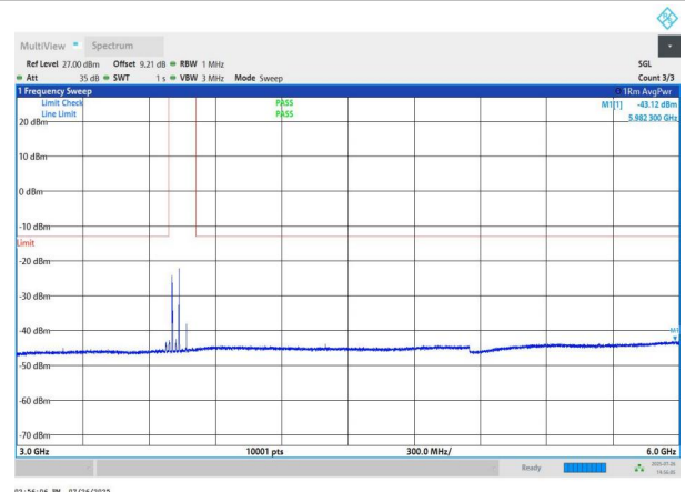
NTNV-n78(3700-3800)-PC2-30-70-L-DFT-QPSK-Edge_1RB_Left- 3000-6000-PASS
