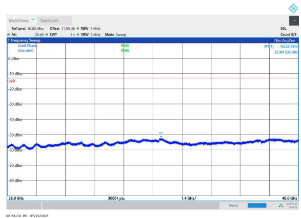
NTNV-n78(3700-3800)-PC2-30-70-L-DFT-QPSK-Edge_1RB_Left 26000-40000-PASS
