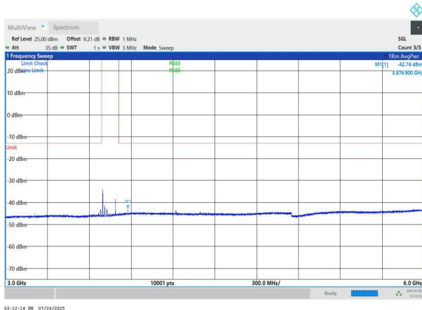
NTNV-n78(3700-3800)-PC2-30-90-L-DFT-BPSK-Edge_1RB_Left- 3000-6000-PASS
