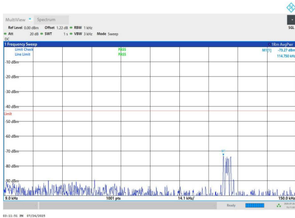
NTNV-n78(3700-3800)-PC2-30-90-L-DFT-BPSK-Edge_1RB_Left- 0.009-0.15-PASS
