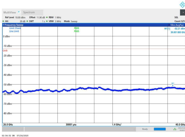
NTNV-n78(3700-3800)-PC2-30-70-L-DFT-BPSK-Edge_1RB_Left- 26000-40000-PASS
