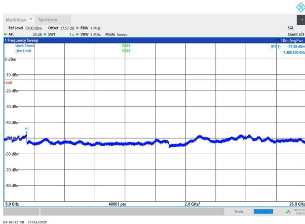
NTNV-n78(3700-3800)-PC2-30-80-M-DFT-QPSK-Edge_1RB_Left -6000-26000-PASS
