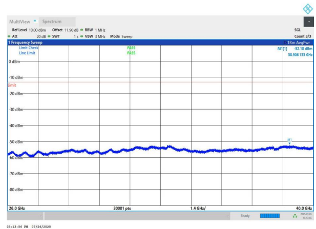
NTNV-n78(3700-3800)-PC2-30-90-L-DFT-QPSK-Edge_1RB_Left- 26000-40000-PASS
