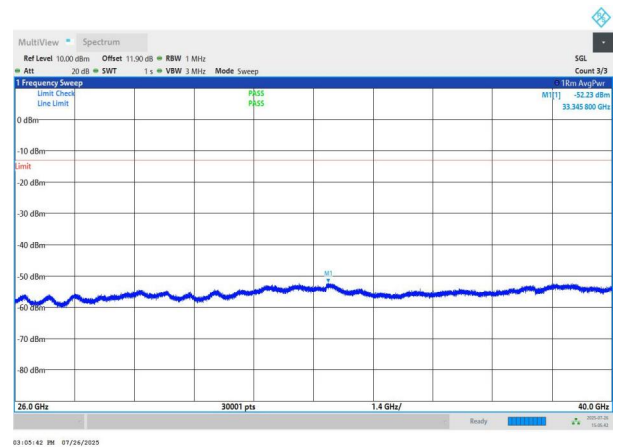
NTNV-n78(3700-3800)-PC2-30-80-L-DFT-QPSK-Edge_1RB_Left- 26000-40000-PASS
