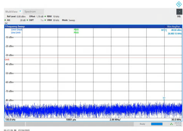
NTNV-n78(3700-3800)-PC2-30-90-H-DFT-BPSK-Edge_1RB_Left 0.15-30-PASS
