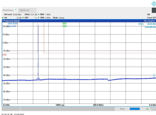
NTNV-n78(3700-3800)-PC2-30-70-L-DFT-BPSK-Edge_1RB_Left- 3000-6000-PASS
