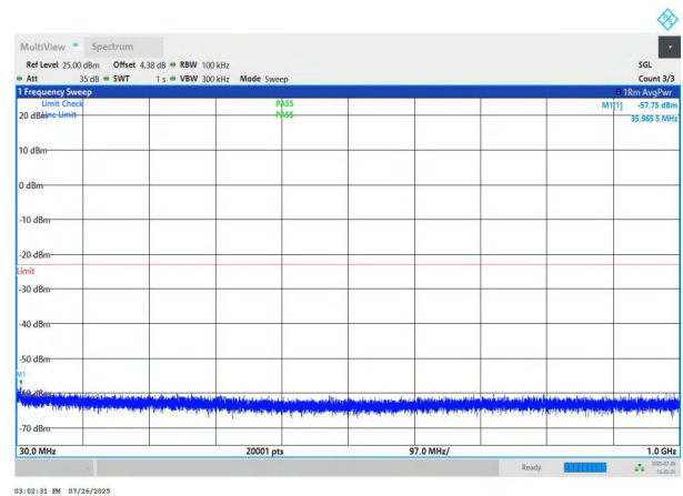
NTNV-n78(3700-3800)-PC2-30-70-H-DFT-QPSK-Edge_1RB_Left -30-1000-PASS
