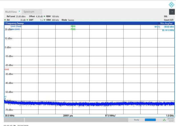
NTNV-n78(3700-3800)-PC2-30-80-M-DFT-QPSK-Edge_1RB_Left -30-1000-PASS
