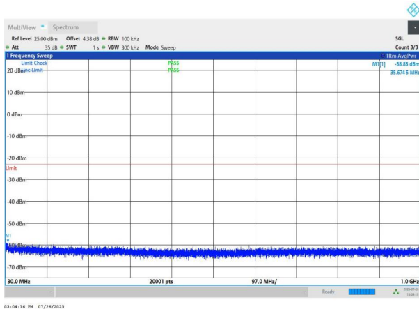
NTNV-n78(3700-3800)-PC2-30-80-L-DFT-BPSK-Edge_1RB_Left- 30-1000-PASS
