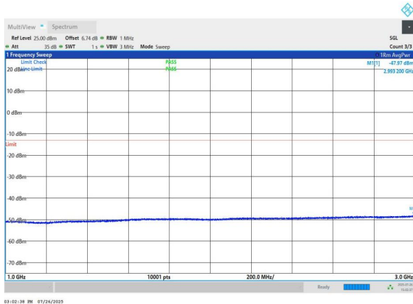
NTNV-n78(3700-3800)-PC2-30-70-H-DFT-QPSK-Edge_1RB_Left -1000-3000-PASS
