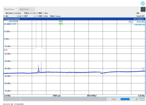
NTNV-n78(3700-3800)-PC2-30-60-H-DFT-QPSK-Edge_1RB_Left -3000-6000-PASS
