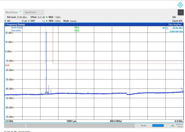
NTNV-n78(3700-3800)-PC2-30-80-L-DFT-QPSK-Edge_1RB_Left- 3000-6000-PASS
