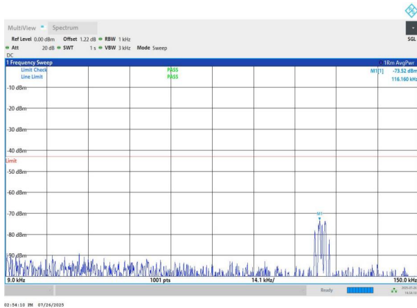
NTNV-n78(3700-3800)-PC2-30-70-L-DFT-BPSK-Edge_1RB_Left- 0.009-0.15-PASS
