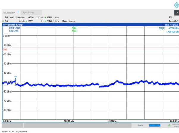
NTNV-n78(3700-3800)-PC2-30-80-L-DFT-QPSK-Edge_1RB_Left- 6000-26000-PASS
