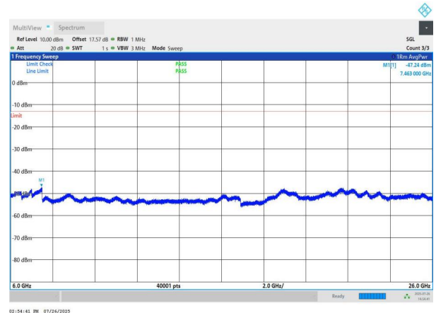
NTNV-n78(3700-3800)-PC2-30-70-L-DFT-BPSK-Edge_1RB_Left- 6000-26000-PASS
