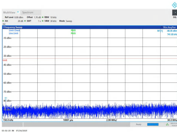
NTNV-n78(3700-3800)-PC2-30-70-H-DFT-QPSK-Edge_1RB_Left -0.15-30-PASS
