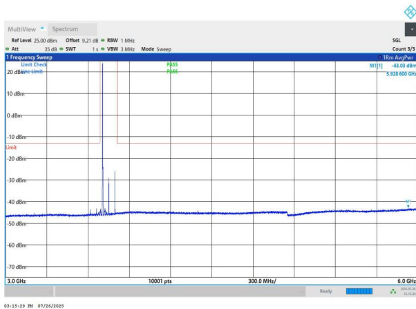
NTNV-n78(3700-3800)-PC2-30-90-M-DFT-BPSK-Edge_1RB_Left -3000-6000-PASS
