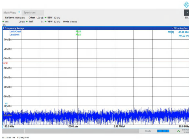
NTNV-n78(3700-3800)-PC2-30-80-H-DFT-QPSK-Edge_1RB_Left -0.15-30-PASS
