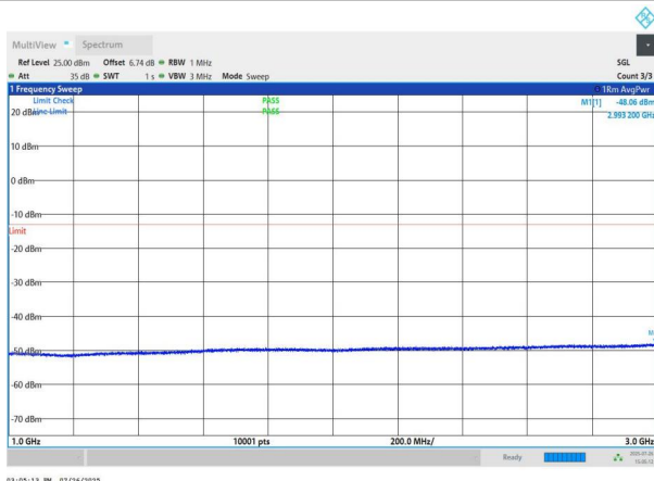
NTNV-n78(3700-3800)-PC2-30-80-L-DFT-QPSK-Edge_1RB_Left- 1000-3000-PASS
