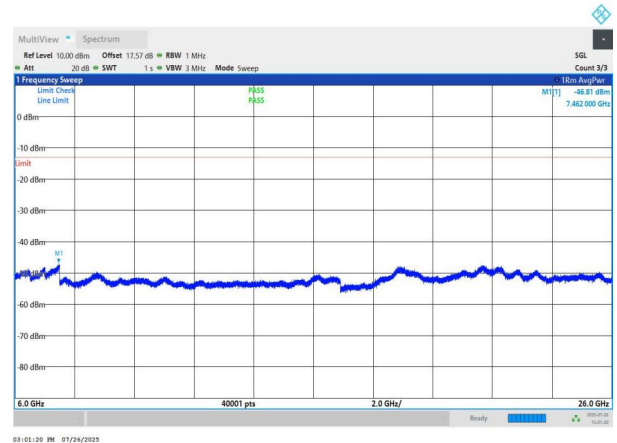
NTNV-n78(3700-3800)-PC2-30-70-H-DFT-BPSK-Edge_1RB_Left 6000-26000-PASS
