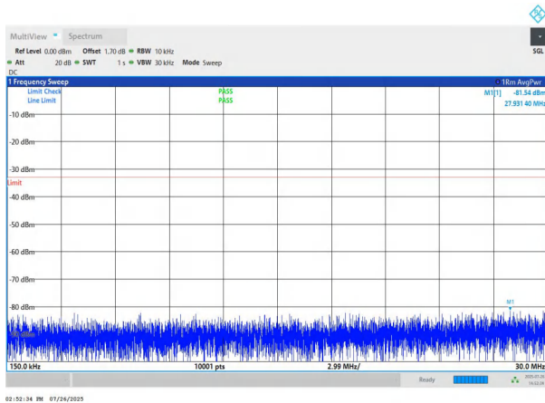
NTNV-n78(3700-3800)-PC2-30-60-H-DFT-QPSK-Edge_1RB_Left -0.15-30-PASS
