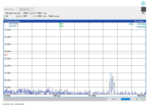
NTNV-n78(3700-3800)-PC2-30-70-M-DFT-QPSK-Edge_1RB_Left -0.009-0.15-PASS
