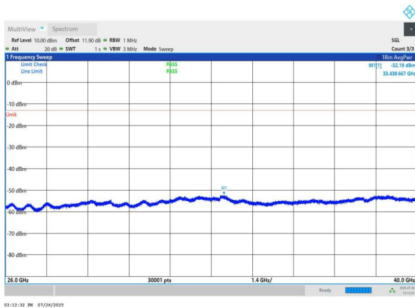
NTNV-n78(3700-3800)-PC2-30-90-L-DFT-BPSK-Edge_1RB_Left- 26000-40000-PASS
