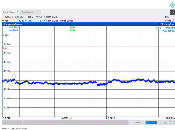
NTNV-n78(3700-3800)-PC2-30-90-L-DFT-QPSK-Edge_1RB_Left- 6000-26000-PASS
