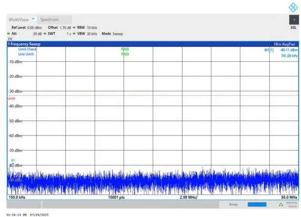
NTNV-n78(3700-3800)-PC2-30-70-L-DFT-BPSK-Edge_1RB_Left- 0.15-30-PASS
