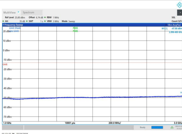
NTNV-n78(3700-3800)-PC2-30-90-L-DFT-QPSK-Edge_1RB_Left- 1000-3000-PASS
