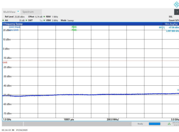
NTNV-n78(3700-3800)-PC2-30-90-M-DFT-QPSK-Edge_1RB_Left -1000-3000-PASS
