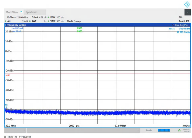
NTNV-n78(3700-3800)-PC2-30-70-L-DFT-QPSK-Edge_1RB_Left- 30-1000-PASS
