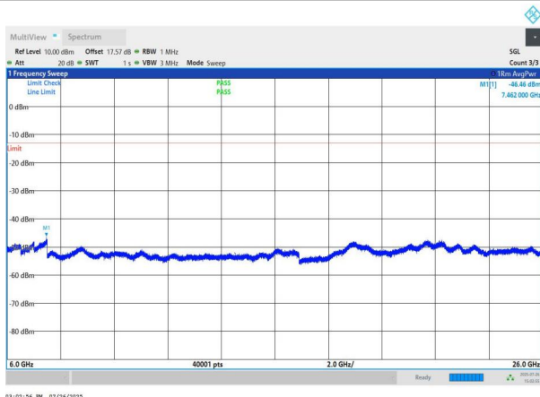
NTNV-n78(3700-3800)-PC2-30-70-H-DFT-QPSK-Edge_1RB_Left -6000-26000-PASS
