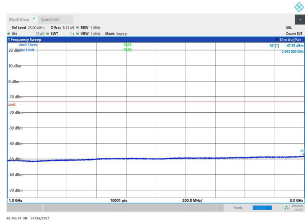
NTNV-n78(3700-3800)-PC2-30-70-L-DFT-BPSK-Edge_1RB_Left- 1000-3000-PASS
