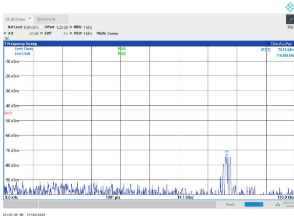
NTNV-n78(3700-3800)-PC2-30-70-H-DFT-BPSK-Edge_1RB_Left -0.009-0.15-PASS
