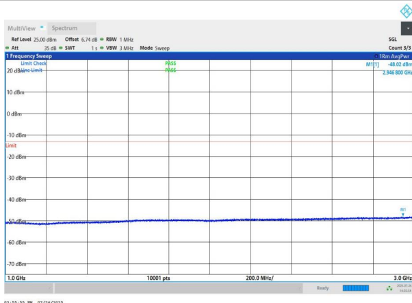
NTNV-n78(3700-3800)-PC2-30-70-L-DFT-QPSK-Edge_1RB_Left- 1000-3000-PASS
