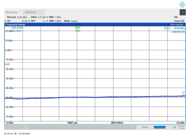
NTNV-n78(3700-3800)-PC2-30-80-H-DFT-BPSK-Edge_1RB_Left 1000-3000-PASS
