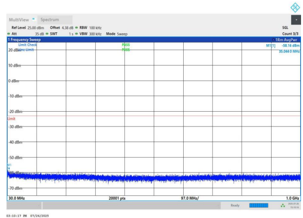
NTNV-n78(3700-3800)-PC2-30-80-H-DFT-QPSK-Edge_1RB_Left -30-1000-PASS
