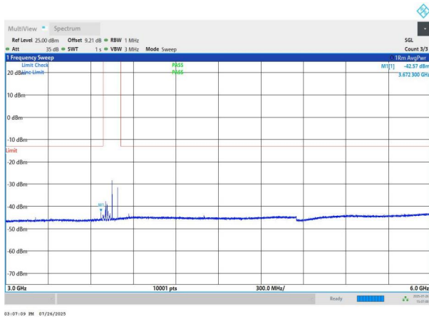
NTNV-n78(3700-3800)-PC2-30-80-M-DFT-BPSK-Edge_1RB_Left -3000-6000-PASS
