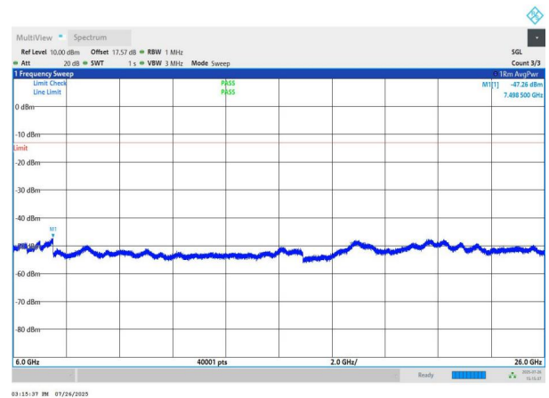
NTNV-n78(3700-3800)-PC2-30-90-M-DFT-BPSK-Edge_1RB_Left -6000-26000-PASS
