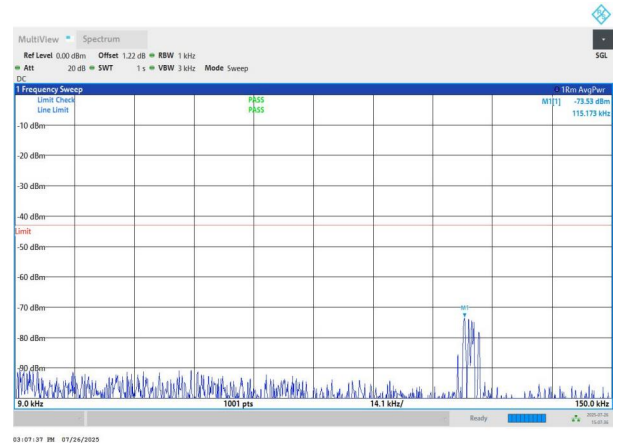
NTNV-n78(3700-3800)-PC2-30-80-M-DFT-QPSK-Edge_1RB_Left -0.009-0.15-PASS
