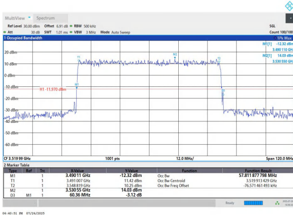
NTNV-n78(3450-3550)-PC2-30-60-H-DFT-256QAM-Outer_Full-An t1-PASS
