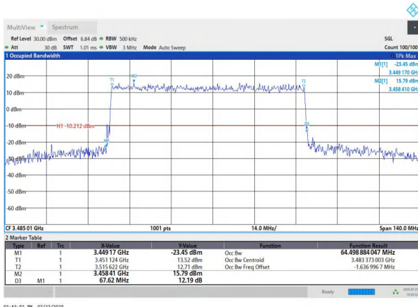
NTNV-n78(3450-3550)-PC2-30-70-L-DFT-QPSK-Outer_Full-Ant1- PASS
