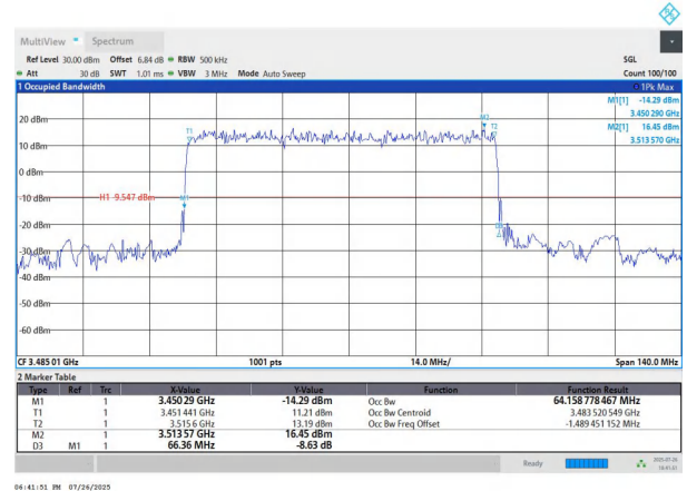
NTNV-n78(3450-3550)-PC2-30-70-L-DFT-BPSK-Outer_Full-Ant1 -PASS
