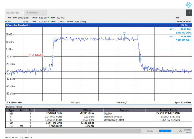
NTNV-n78(3450-3550)-PC2-30-40-H-DFT-64QAM-Outer_Full-An t1-PASS
