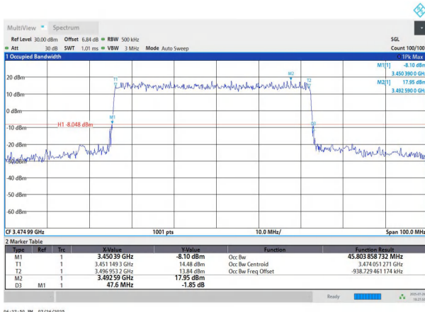
NTNV-n78(3450-3550)-PC2-30-50-L-DFT-QPSK-Outer_Full-Ant1- PASS
