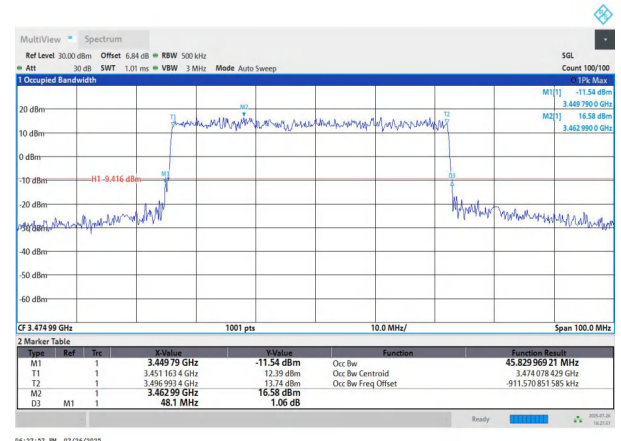
NTNV-n78(3450-3550)-PC2-30-50-L-DFT-16QAM-Outer_Full-Ant 1-PASS
