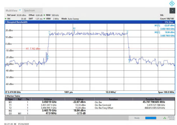
NTNV-n78(3450-3550)-PC2-30-50-L-DFT-BPSK-Outer_Full-Ant1 -PASS
