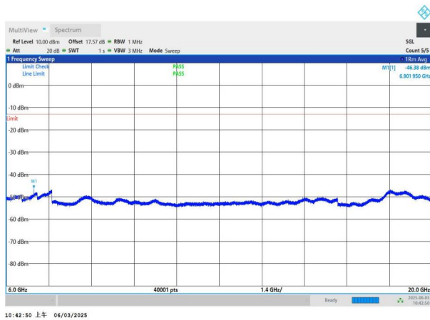
NTNV-n78(3450-3550)-PC2-30-60-L-DFT-QPSK-Edge_1RB_Left- 6000-20000-PASS
