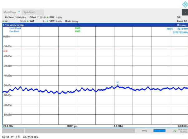
NTNV-n78(3450-3550)-PC2-30-40-H-DFT-BPSK-Edge_1RB_Left -20000-40000-PASS
