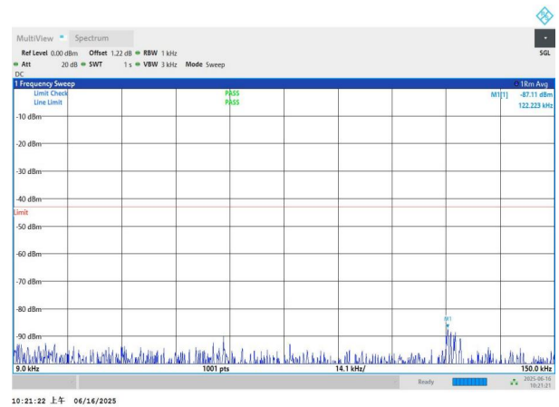
NTNV-n78(3450-3550)-PC2-30-50-L-DFT-QPSK-Edge_1RB_Left- 0.009-0.15-PASS
