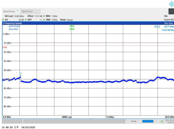
NTNV-n78(3450-3550)-PC2-30-60-H-DFT-QPSK-Edge_1RB_Left -6000-20000-PASS
