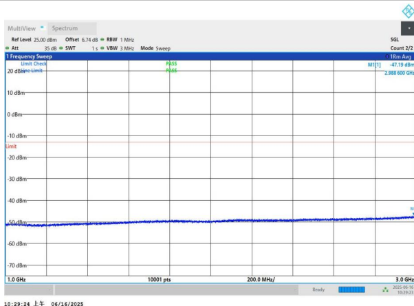
NTNV-n78(3450-3550)-PC2-30-70-L-DFT-QPSK-Edge_1RB_Left- 1000-3000-PASS
