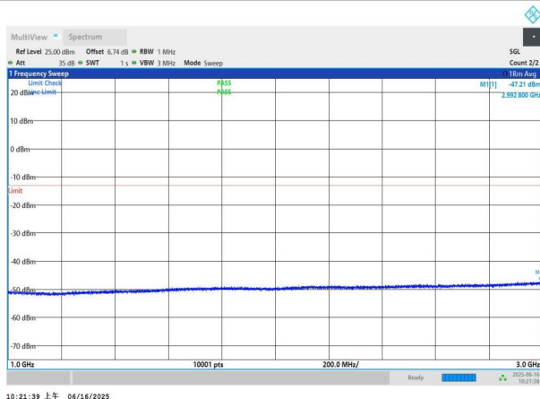
NTNV-n78(3450-3550)-PC2-30-50-L-DFT-QPSK-Edge_1RB_Left- 1000-3000-PASS
