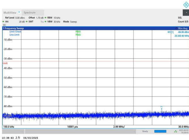
NTNV-n78(3450-3550)-PC2-30-40-H-DFT-QPSK-Edge_1RB_Left -0.15-30-PASS
