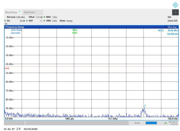
NTNV-n78(3450-3550)-PC2-30-60-L-DFT-QPSK-Edge_1RB_Left- 0.009-0.15-PASS
