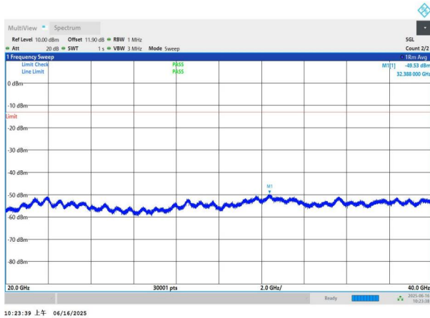
NTNV-n78(3450-3550)-PC2-30-50-M-DFT-BPSK-Edge_1RB_Left -20000-40000-PASS
