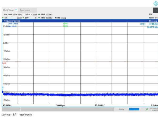
NTNV-n78(3450-3550)-PC2-30-60-L-DFT-BPSK-Edge_1RB_Left- 30-1000-PASS
