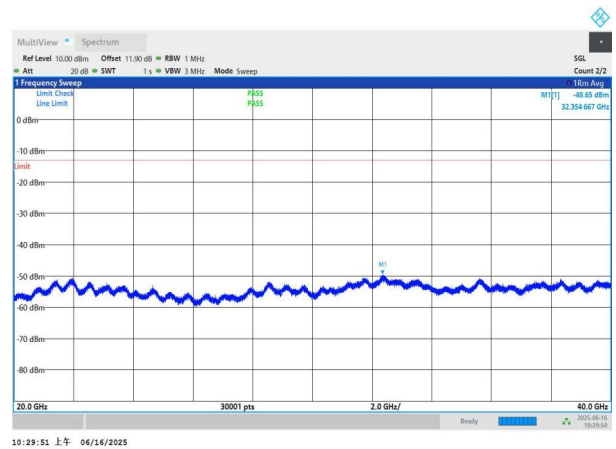
NTNV-n78(3450-3550)-PC2-30-70-L-DFT-QPSK-Edge_1RB_Left- 20000-40000-PASS
