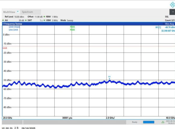
NTNV-n78(3450-3550)-PC2-30-50-H-DFT-BPSK-Edge_1RB_Left -20000-40000-PASS
