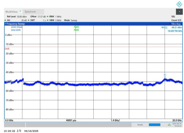
NTNV-n78(3450-3550)-PC2-30-50-H-DFT-BPSK-Edge_1RB_Left 6000-20000-PASS
