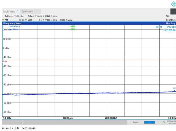
NTNV-n78(3450-3550)-PC2-30-60-H-DFT-QPSK-Edge_1RB_Left -1000-3000-PASS
