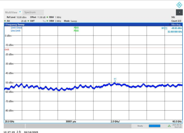
NTNV-n78(3450-3550)-PC2-30-50-H-DFT-QPSK-Edge_1RB_Left -20000-40000-PASS
