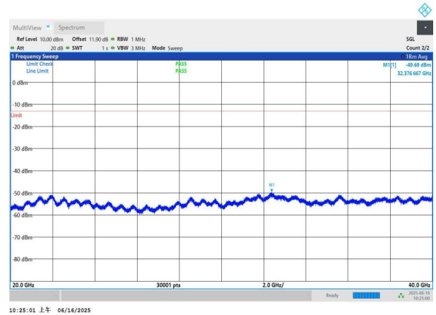
NTNV-n78(3450-3550)-PC2-30-50-M-DFT-QPSK-Edge_1RB_Left -20000-40000-PASS
