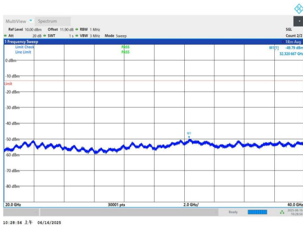
NTNV-n78(3450-3550)-PC2-30-70-L-DFT-BPSK-Edge_1RB_Left- 20000-40000-PASS
