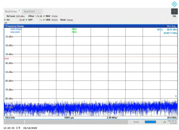
NTNV-n78(3450-3550)-PC2-30-50-M-DFT-BPSK-Edge_1RB_Left -0.15-30-PASS
