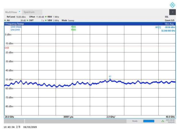
NTNV-n78(3450-3550)-PC2-30-60-L-DFT-QPSK-Edge_1RB_Left- 20000-40000-PASS
