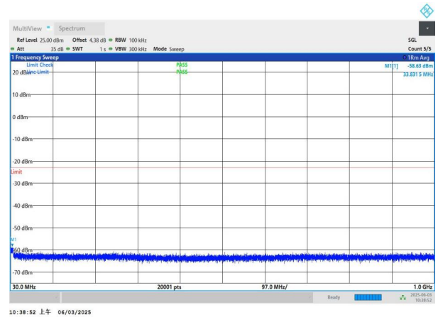
NTNV-n78(3450-3550)-PC2-30-40-H-DFT-QPSK-Edge_1RB_Left -30-1000-PASS
