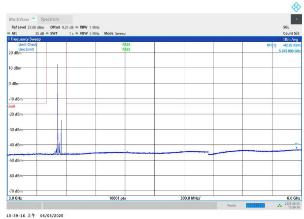
NTNV-n78(3450-3550)-PC2-30-40-H-DFT-QPSK-Edge_1RB_Left -3000-6000-PASS
