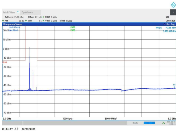
NTNV-n78(3450-3550)-PC2-30-60-M-DFT-BPSK-Edge_1RB_Left -3000-6000-PASS
