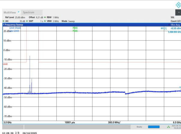
NTNV-n78(3450-3550)-PC2-30-70-L-DFT-BPSK-Edge_1RB_Left- 3000-6000-PASS
