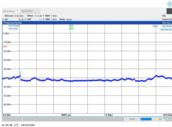
NTNV-n78(3450-3550)-PC2-30-60-M-DFT-QPSK-Edge_1RB_Left -6000-20000-PASS
