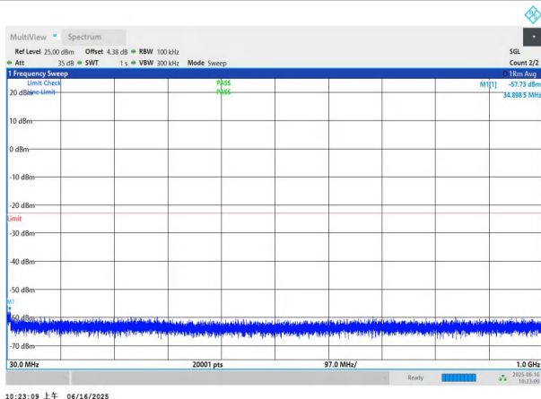
NTNV-n78(3450-3550)-PC2-30-50-M-DFT-BPSK-Edge_1RB_Left -30-1000-PASS
