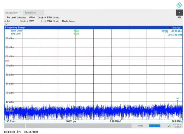
NTNV-n78(3450-3550)-PC2-30-50-L-DFT-BPSK-Edge_1RB_Left- 0.15-30-PASS
