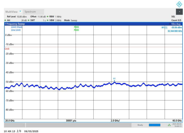
NTNV-n78(3450-3550)-PC2-30-60-H-DFT-QPSK-Edge_1RB_Left -20000-40000-PASS
