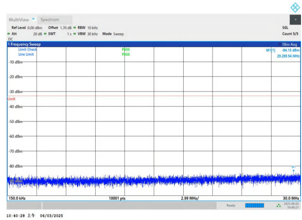
NTNV-n78(3450-3550)-PC2-30-60-L-DFT-BPSK-Edge_1RB_Left- 0.15-30-PASS
