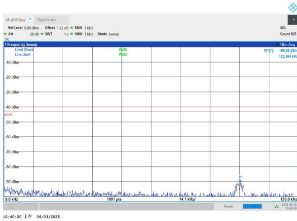
NTNV-n78(3450-3550)-PC2-30-60-L-DFT-BPSK-Edge_1RB_Left- 0.009-0.15-PASS
