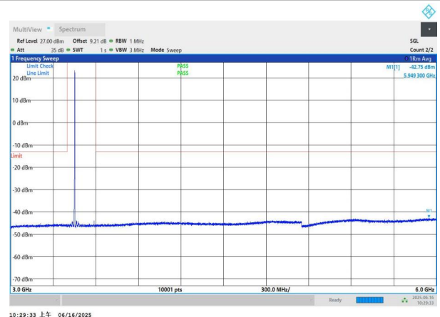
NTNV-n78(3450-3550)-PC2-30-70-L-DFT-QPSK-Edge_1RB_Left- 3000-6000-PASS
