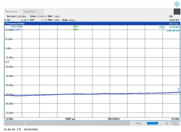
NTNV-n78(3450-3550)-PC2-30-60-L-DFT-BPSK-Edge_1RB_Left- 1000-3000-PASS
