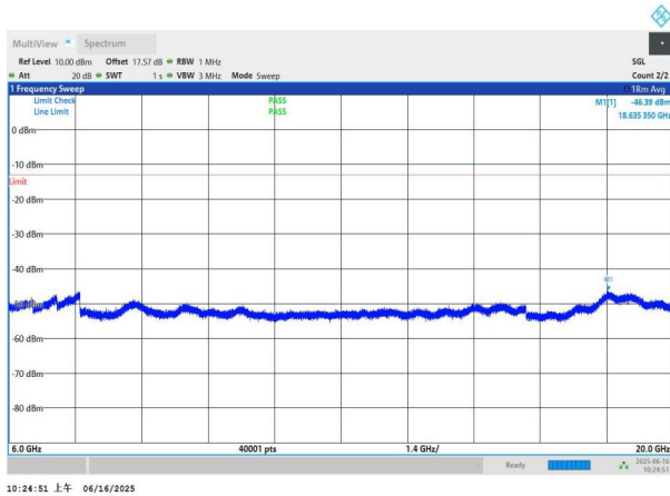
NTNV-n78(3450-3550)-PC2-30-50-M-DFT-QPSK-Edge_1RB_Left -6000-20000-PASS
