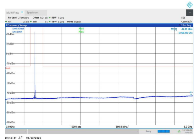
NTNV-n78(3450-3550)-PC2-30-60-M-DFT-QPSK-Edge_1RB_Left -3000-6000-PASS
