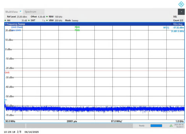
NTNV-n78(3450-3550)-PC2-30-70-L-DFT-QPSK-Edge_1RB_Left- 30-1000-PASS
