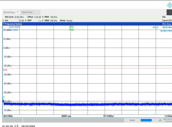
NTNV-n78(3450-3550)-PC2-30-60-M-DFT-BPSK-Edge_1RB_Left -30-1000-PASS
