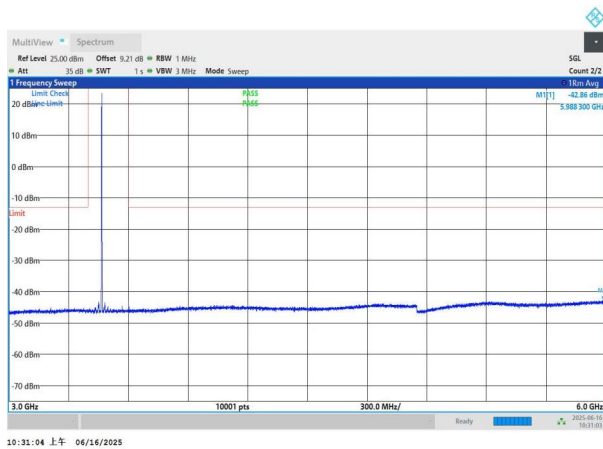
NTNV-n78(3450-3550)-PC2-30-70-M-DFT-BPSK-Edge_1RB_Left -3000-6000-PASS
