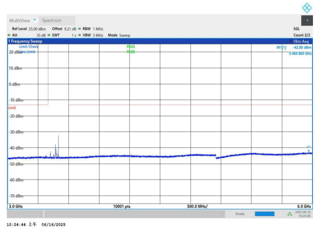
NTNV-n78(3450-3550)-PC2-30-50-M-DFT-QPSK-Edge_1RB_Left -3000-6000-PASS
