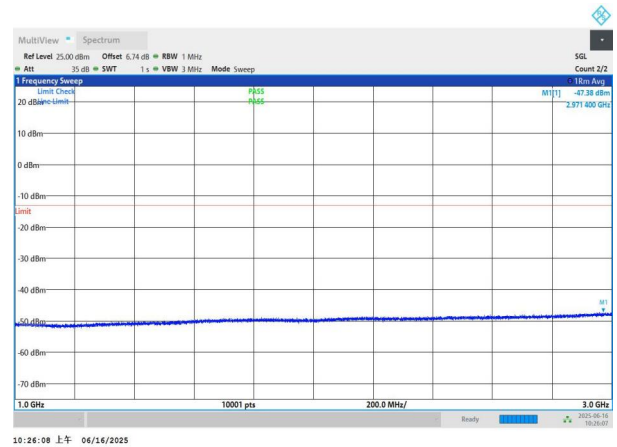
NTNV-n78(3450-3550)-PC2-30-50-H-DFT-BPSK-Edge_1RB_Left 1000-3000-PASS
