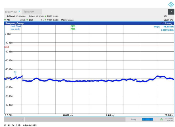
NTNV-n78(3450-3550)-PC2-30-60-L-DFT-BPSK-Edge_1RB_Left- 6000-20000-PASS
