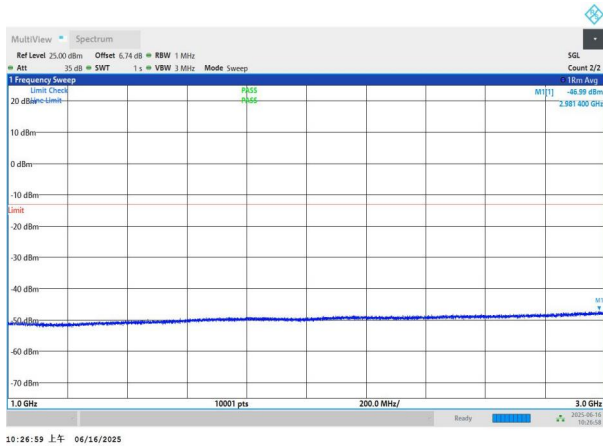
NTNV-n78(3450-3550)-PC2-30-50-H-DFT-QPSK-Edge_1RB_Left -1000-3000-PASS
