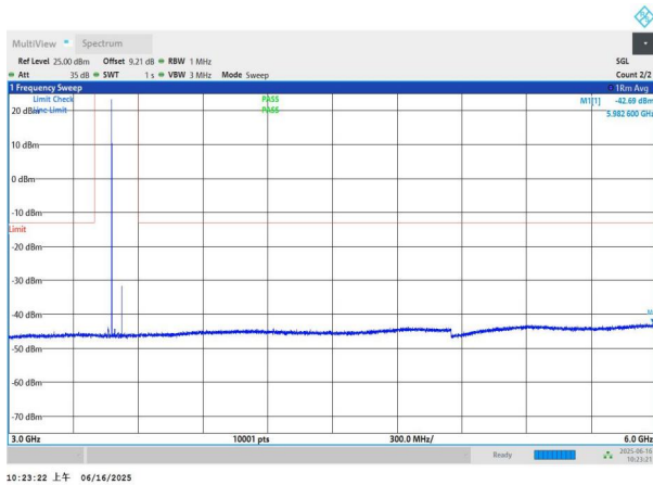
NTNV-n78(3450-3550)-PC2-30-50-M-DFT-BPSK-Edge_1RB_Left -3000-6000-PASS
