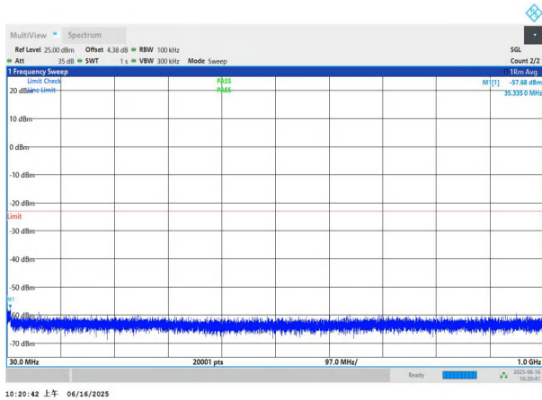
NTNV-n78(3450-3550)-PC2-30-50-L-DFT-BPSK-Edge_1RB_Left- 30-1000-PASS
