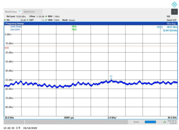
NTNV-n78(3450-3550)-PC2-30-50-L-DFT-QPSK-Edge_1RB_Left- 20000-40000-PASS
