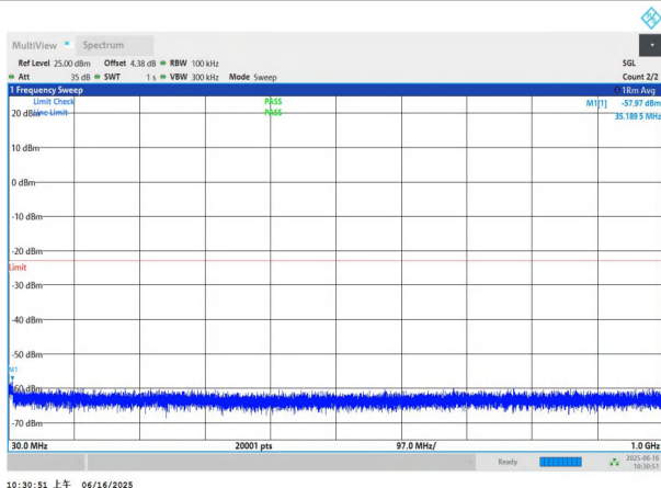
NTNV-n78(3450-3550)-PC2-30-70-M-DFT-BPSK-Edge_1RB_Left -30-1000-PASS
