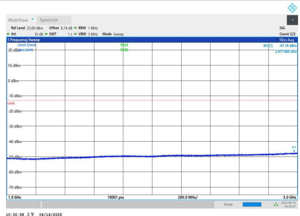
NTNV-n78(3450-3550)-PC2-30-70-M-DFT-BPSK-Edge_1RB_Left -1000-3000-PASS
