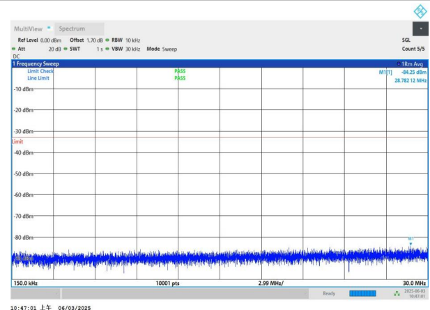
NTNV-n78(3450-3550)-PC2-30-60-H-DFT-BPSK-Edge_1RB_Left 0.15-30-PASS
