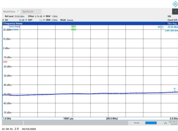
NTNV-n78(3450-3550)-PC2-30-40-H-DFT-QPSK-Edge_1RB_Left -1000-3000-PASS
