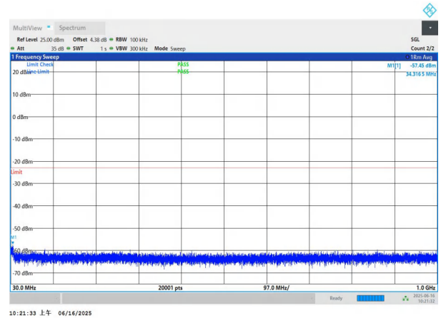
NTNV-n78(3450-3550)-PC2-30-50-L-DFT-QPSK-Edge_1RB_Left- 30-1000-PASS
