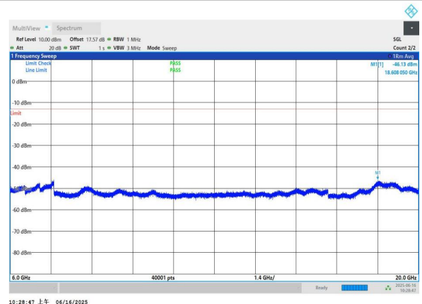
NTNV-n78(3450-3550)-PC2-30-70-L-DFT-BPSK-Edge_1RB_Left- 6000-20000-PASS
