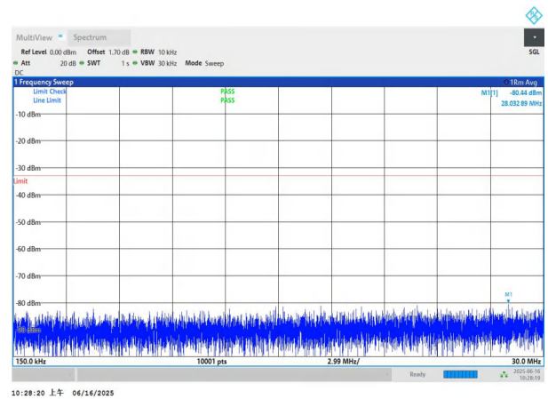
NTNV-n78(3450-3550)-PC2-30-70-L-DFT-BPSK-Edge_1RB_Left- 0.15-30-PASS
