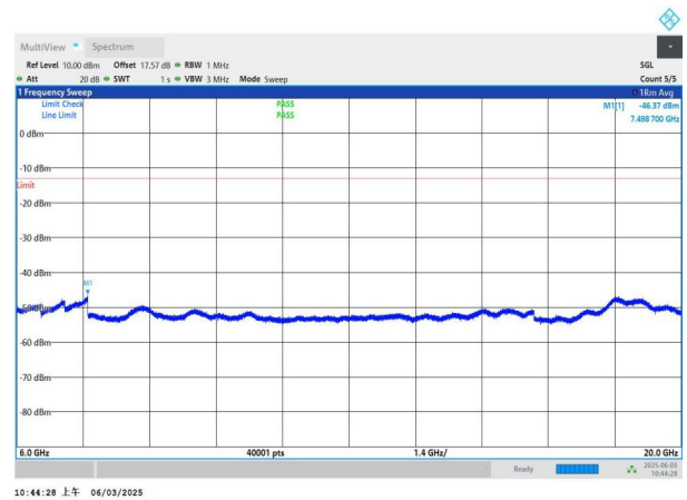
NTNV-n78(3450-3550)-PC2-30-60-M-DFT-BPSK-Edge_1RB_Left -6000-20000-PASS
