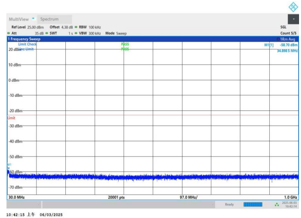
NTNV-n78(3450-3550)-PC2-30-60-L-DFT-QPSK-Edge_1RB_Left- 30-1000-PASS
