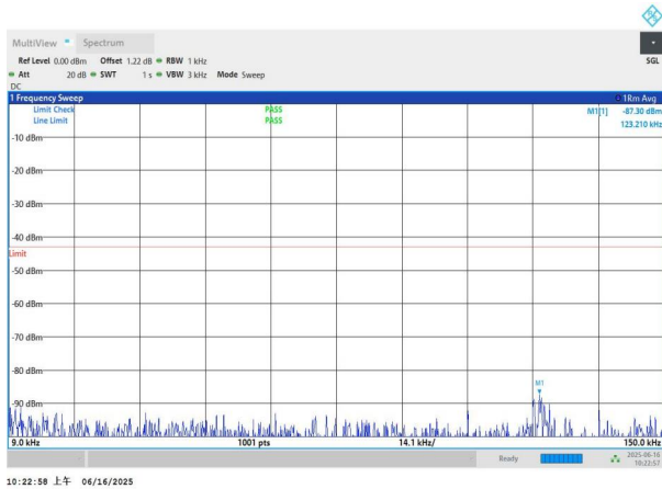
NTNV-n78(3450-3550)-PC2-30-50-M-DFT-BPSK-Edge_1RB_Left -0.009-0.15-PASS
