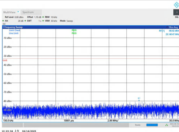
NTNV-n78(3450-3550)-PC2-30-50-M-DFT-QPSK-Edge_1RB_Left -0.15-30-PASS
