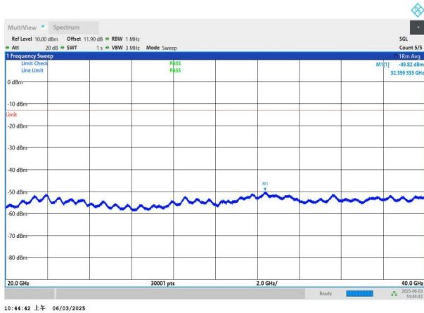
NTNV-n78(3450-3550)-PC2-30-60-M-DFT-BPSK-Edge_1RB_Left -20000-40000-PASS
