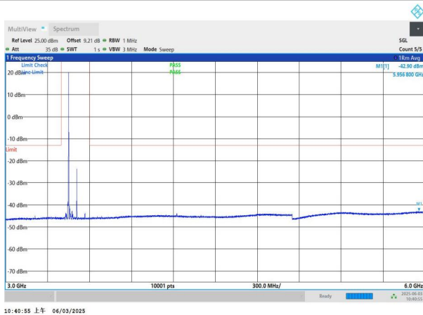
NTNV-n78(3450-3550)-PC2-30-60-L-DFT-BPSK-Edge_1RB_Left- 3000-6000-PASS
