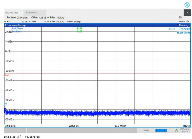
NTNV-n78(3450-3550)-PC2-30-50-H-DFT-QPSK-Edge_1RB_Left -30-1000-PASS
