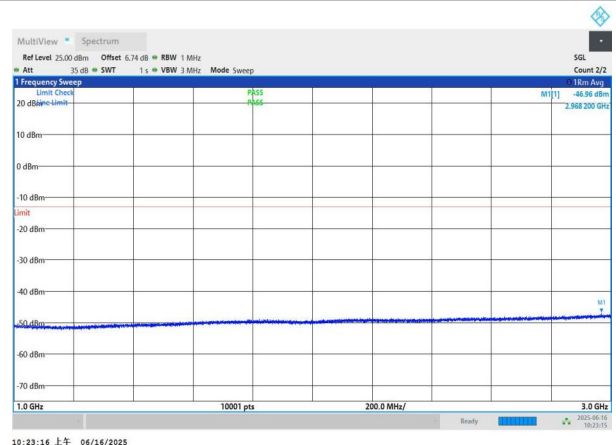
NTNV-n78(3450-3550)-PC2-30-50-M-DFT-BPSK-Edge_1RB_Left -1000-3000-PASS
