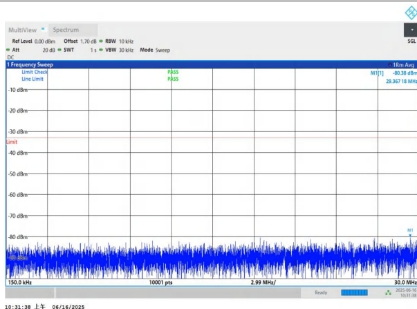
NTNV-n78(3450-3550)-PC2-30-70-M-DFT-QPSK-Edge_1RB_Left -0.15-30-PASS
