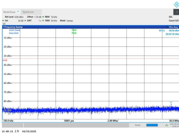
NTNV-n78(3450-3550)-PC2-30-60-H-DFT-QPSK-Edge_1RB_Left -0.15-30-PASS
