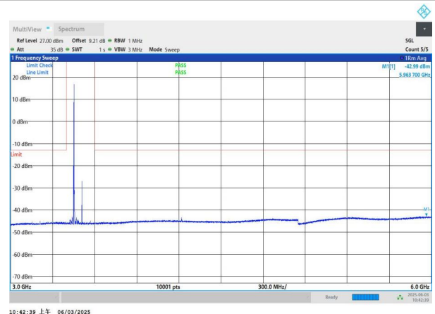
NTNV-n78(3450-3550)-PC2-30-60-L-DFT-QPSK-Edge_1RB_Left- 3000-6000-PASS
