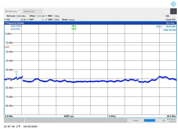
NTNV-n78(3450-3550)-PC2-30-60-H-DFT-BPSK-Edge_1RB_Left 6000-20000-PASS
