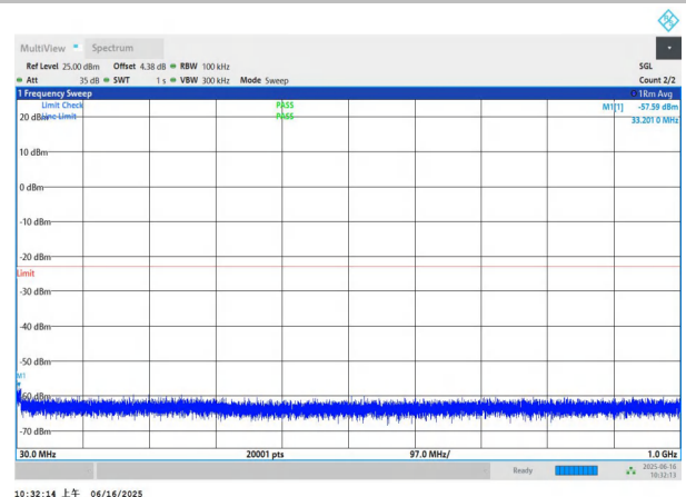
NTNV-n78(3450-3550)-PC2-30-70-M-DFT-QPSK-Edge_1RB_Left -30-1000-PASS
