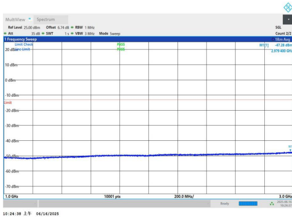
NTNV-n78(3450-3550)-PC2-30-50-M-DFT-QPSK-Edge_1RB_Left -1000-3000-PASS
