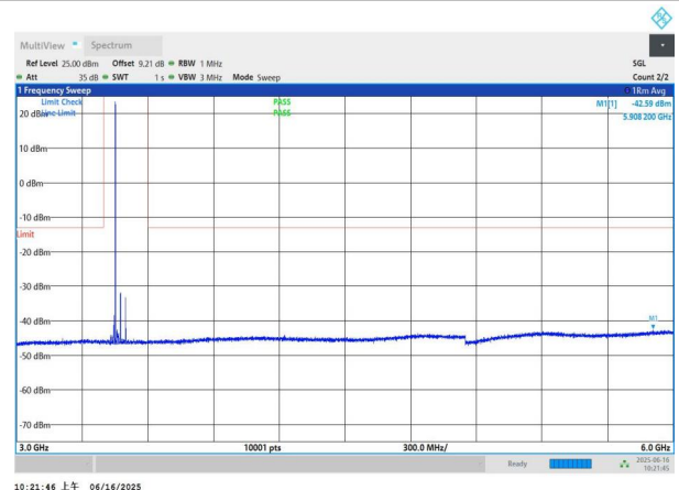
NTNV-n78(3450-3550)-PC2-30-50-L-DFT-QPSK-Edge_1RB_Left- 3000-6000-PASS
