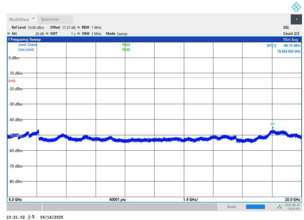
NTNV-n78(3450-3550)-PC2-30-50-L-DFT-BPSK-Edge_1RB_Left- 6000-20000-PASS
