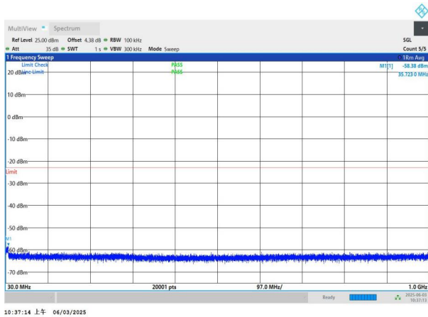
NTNV-n78(3450-3550)-PC2-30-40-H-DFT-BPSK-Edge_1RB_Left -30-1000-PASS
