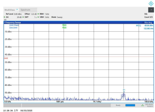
NTNV-n78(3450-3550)-PC2-30-40-H-DFT-QPSK-Edge_1RB_Left -0.009-0.15-PASS
