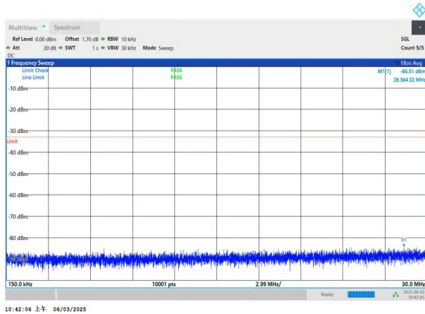
NTNV-n78(3450-3550)-PC2-30-60-L-DFT-QPSK-Edge_1RB_Left- 0.15-30-PASS
