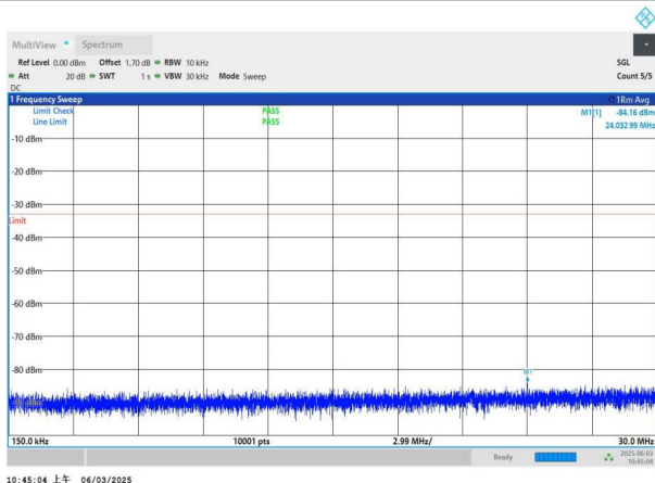
NTNV-n78(3450-3550)-PC2-30-60-M-DFT-QPSK-Edge_1RB_Left -0.15-30-PASS
