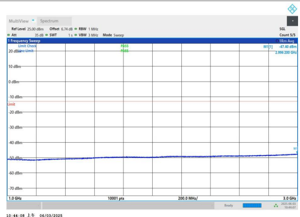
NTNV-n78(3450-3550)-PC2-30-60-M-DFT-BPSK-Edge_1RB_Left -1000-3000-PASS
