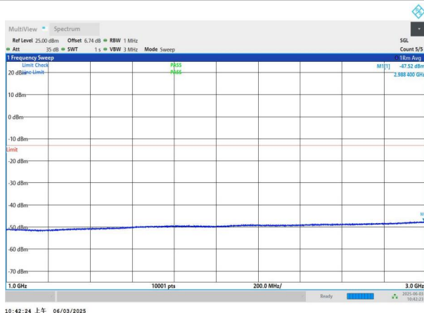
NTNV-n78(3450-3550)-PC2-30-60-L-DFT-QPSK-Edge_1RB_Left- 1000-3000-PASS
