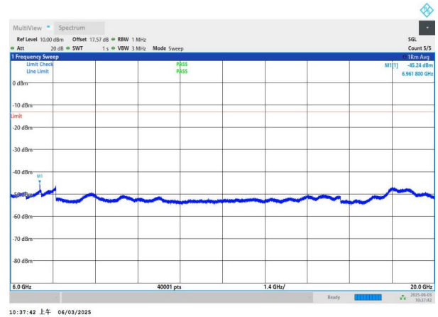
NTNV-n78(3450-3550)-PC2-30-40-H-DFT-BPSK-Edge_1RB_Left 6000-20000-PASS
