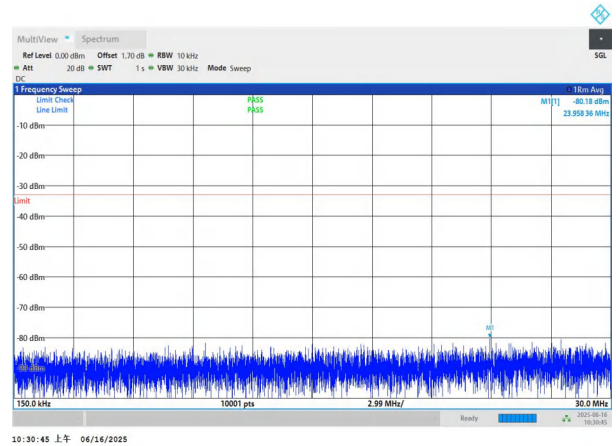
NTNV-n78(3450-3550)-PC2-30-70-M-DFT-BPSK-Edge_1RB_Left -0.15-30-PASS
