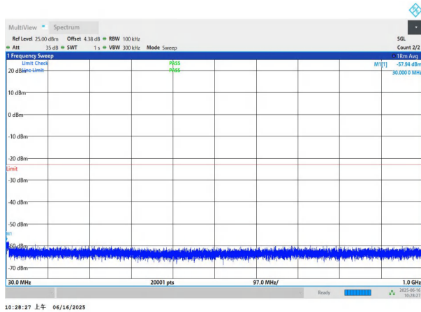
NTNV-n78(3450-3550)-PC2-30-70-L-DFT-BPSK-Edge_1RB_Left- 30-1000-PASS
