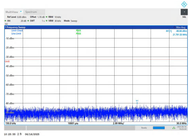
NTNV-n78(3450-3550)-PC2-30-50-H-DFT-BPSK-Edge_1RB_Left 0.15-30-PASS
