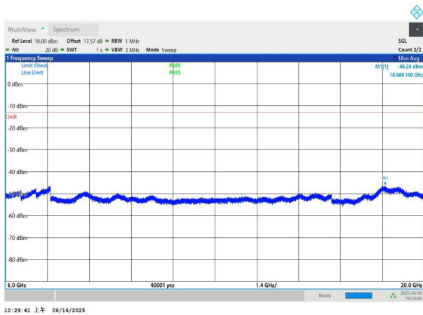
NTNV-n78(3450-3550)-PC2-30-70-L-DFT-QPSK-Edge_1RB_Left- 6000-20000-PASS
