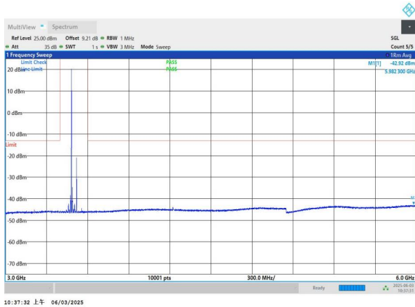
NTNV-n78(3450-3550)-PC2-30-40-H-DFT-BPSK-Edge_1RB_Left -3000-6000-PASS
