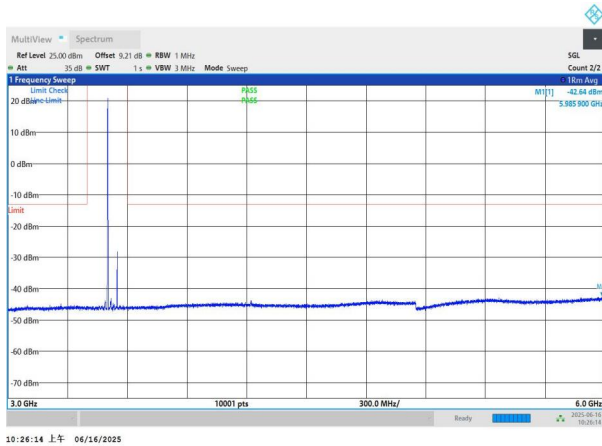
NTNV-n78(3450-3550)-PC2-30-50-H-DFT-BPSK-Edge_1RB_Left -3000-6000-PASS
