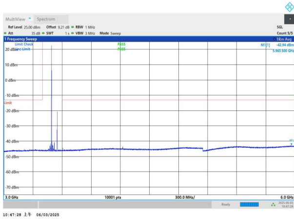
NTNV-n78(3450-3550)-PC2-30-60-H-DFT-BPSK-Edge_1RB_Left -3000-6000-PASS
