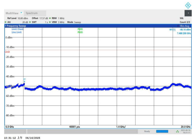
NTNV-n78(3450-3550)-PC2-30-70-M-DFT-BPSK-Edge_1RB_Left -6000-20000-PASS
