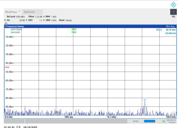
NTNV-n78(3450-3550)-PC2-30-50-H-DFT-QPSK-Edge_1RB_Left -0.009-0.15-PASS
