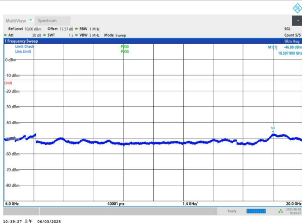
NTNV-n78(3450-3550)-PC2-30-40-H-DFT-QPSK-Edge_1RB_Left -6000-20000-PASS
