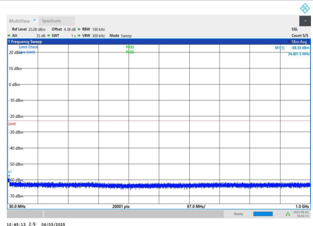
NTNV-n78(3450-3550)-PC2-30-60-M-DFT-QPSK-Edge_1RB_Left -30-1000-PASS
