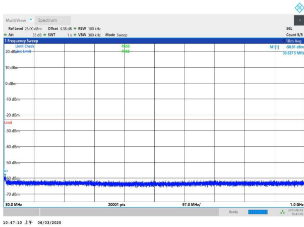
NTNV-n78(3450-3550)-PC2-30-60-H-DFT-BPSK-Edge_1RB_Left -30-1000-PASS
