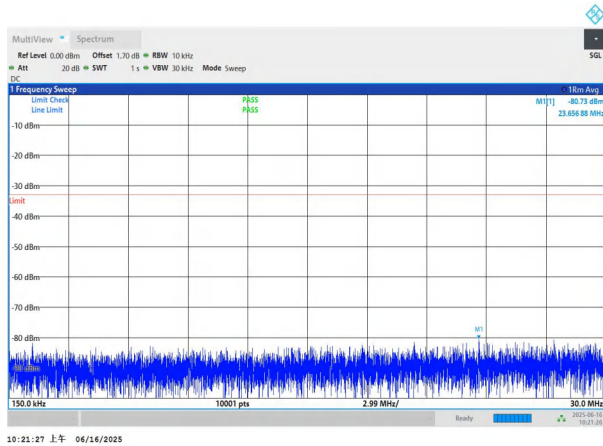
NTNV-n78(3450-3550)-PC2-30-50-L-DFT-QPSK-Edge_1RB_Left- 0.15-30-PASS
