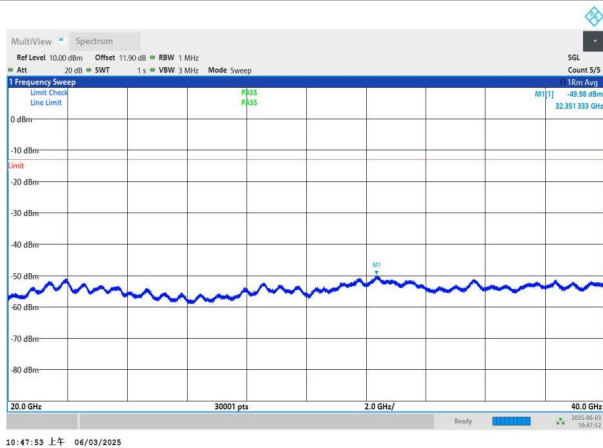
NTNV-n78(3450-3550)-PC2-30-60-H-DFT-BPSK-Edge_1RB_Left -20000-40000-PASS
