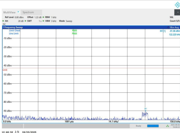
NTNV-n78(3450-3550)-PC2-30-60-H-DFT-BPSK-Edge_1RB_Left -0.009-0.15-PASS
