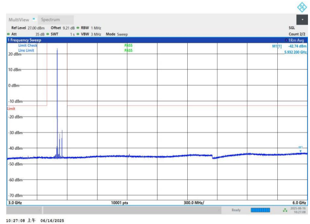
NTNV-n78(3450-3550)-PC2-30-50-H-DFT-QPSK-Edge_1RB_Left -3000-6000-PASS
