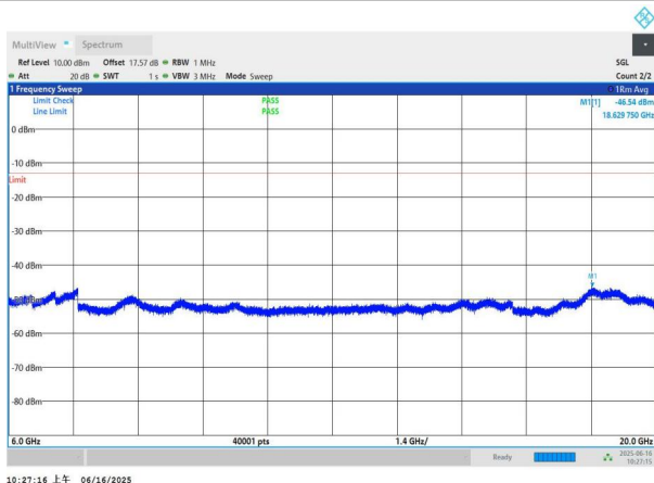
NTNV-n78(3450-3550)-PC2-30-50-H-DFT-QPSK-Edge_1RB_Left -6000-20000-PASS
