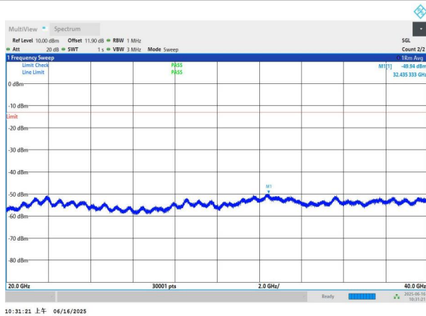
NTNV-n78(3450-3550)-PC2-30-70-M-DFT-BPSK-Edge_1RB_Left -20000-40000-PASS
