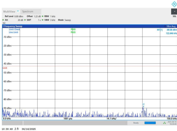
NTNV-n78(3450-3550)-PC2-30-70-M-DFT-BPSK-Edge_1RB_Left -0.009-0.15-PASS
