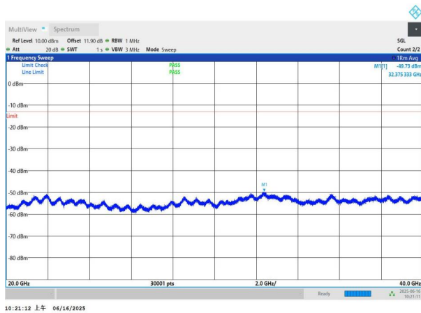
NTNV-n78(3450-3550)-PC2-30-50-L-DFT-BPSK-Edge_1RB_Left- 20000-40000-PASS
