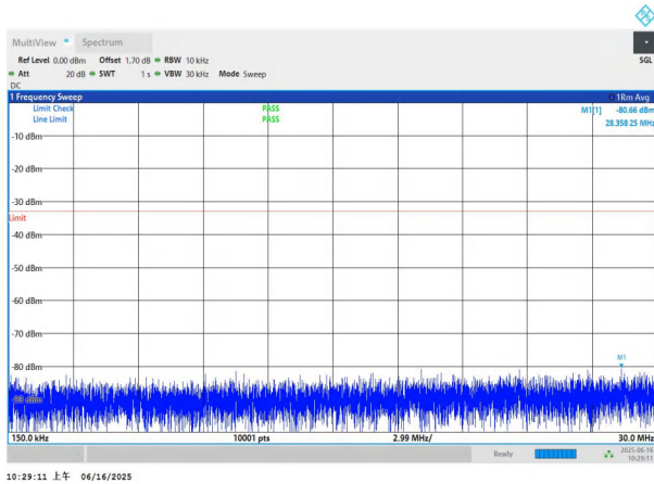
NTNV-n78(3450-3550)-PC2-30-70-L-DFT-QPSK-Edge_1RB_Left- 0.15-30-PASS
