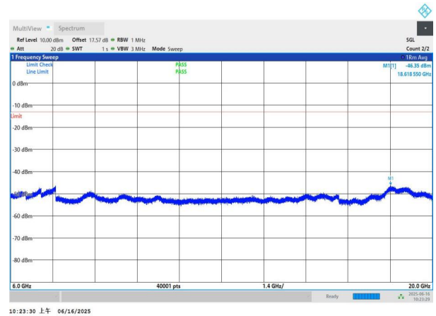
NTNV-n78(3450-3550)-PC2-30-50-M-DFT-BPSK-Edge_1RB_Left -6000-20000-PASS
