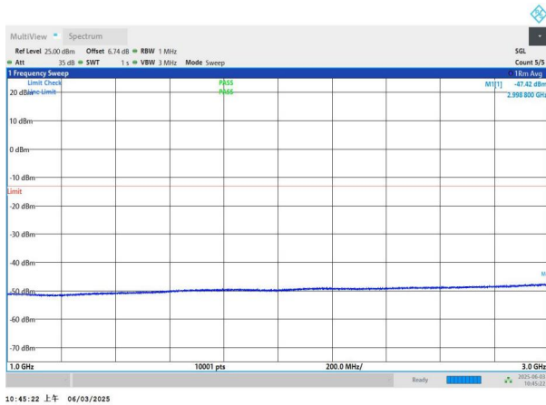
NTNV-n78(3450-3550)-PC2-30-60-M-DFT-QPSK-Edge_1RB_Left -1000-3000-PASS
