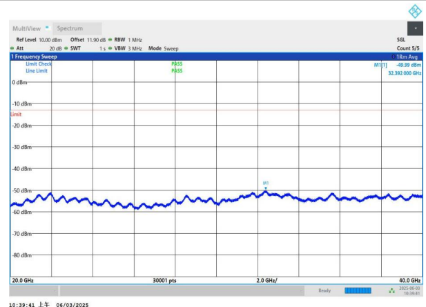
NTNV-n78(3450-3550)-PC2-30-40-H-DFT-QPSK-Edge_1RB_Left -20000-40000-PASS
