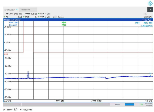
NTNV-n78(3450-3550)-PC2-30-60-H-DFT-QPSK-Edge_1RB_Left -3000-6000-PASS
