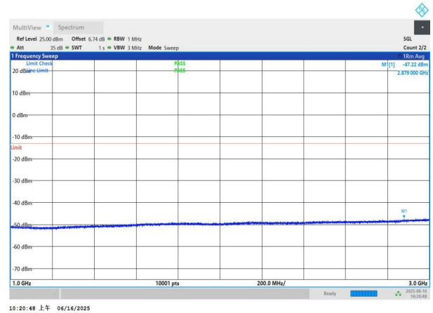
NTNV-n78(3450-3550)-PC2-30-50-L-DFT-BPSK-Edge_1RB_Left- 1000-3000-PASS
