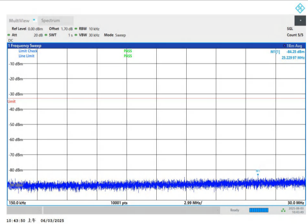
NTNV-n78(3450-3550)-PC2-30-60-M-DFT-BPSK-Edge_1RB_Left -0.15-30-PASS
