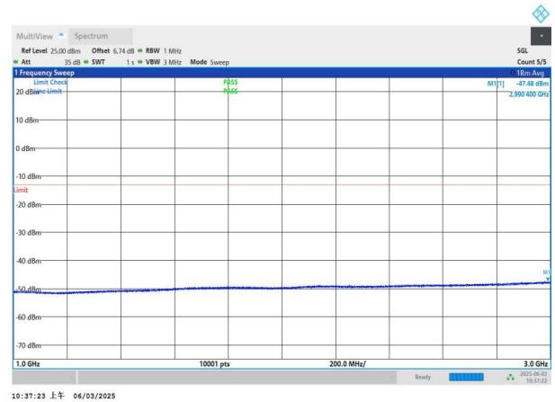
NTNV-n78(3450-3550)-PC2-30-40-H-DFT-BPSK-Edge_1RB_Left 1000-3000-PASS
