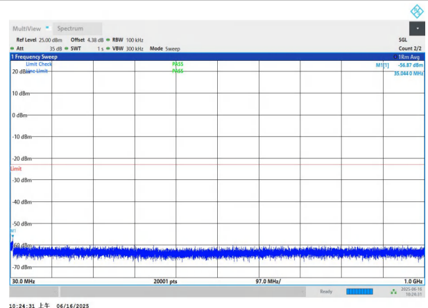
NTNV-n78(3450-3550)-PC2-30-50-M-DFT-QPSK-Edge_1RB_Left -30-1000-PASS
