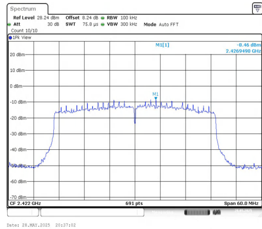
11AX40MIMO-Ant2-2422-0~Reference-PASS
