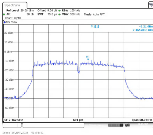
11N40MIMO-Ant1-2452-0~Reference-PASS
