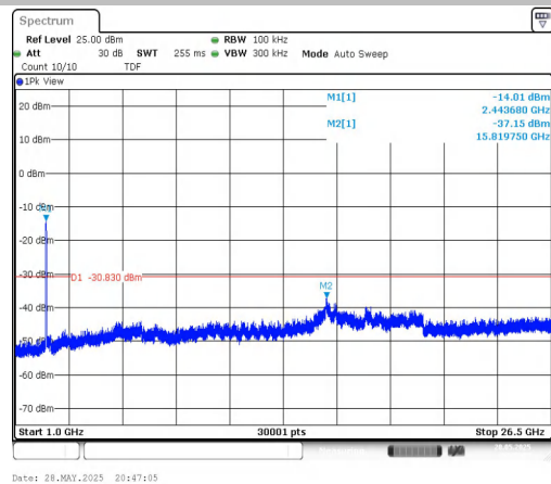
11AX40MIMO-Ant2-2452-1000~26500-PASS
