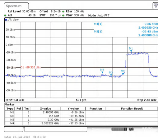
11AX20MIMO-Ant2-2412-PASS
