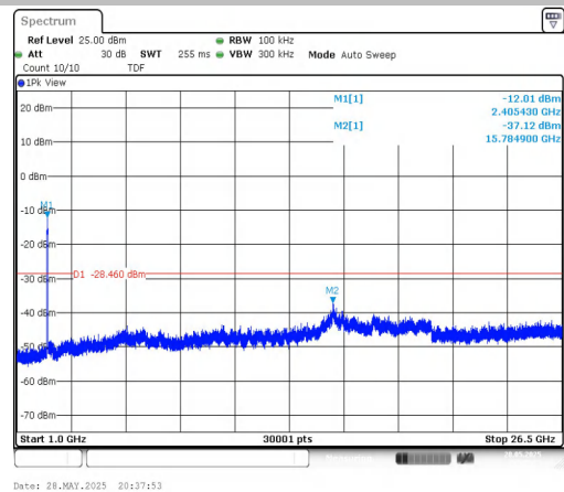
11AX40MIMO-Ant2-2422-1000~26500-PASS
