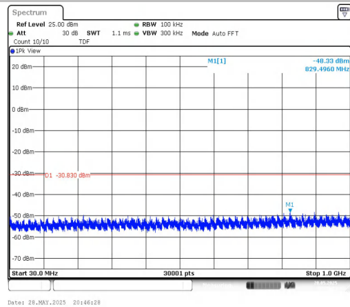
11AX40MIMO-Ant2-2452-30~1000-PASS
