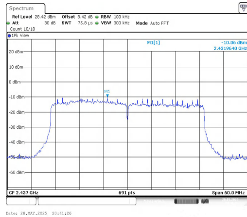
11AX40MIMO-Ant2-2437-0~Reference-PASS
