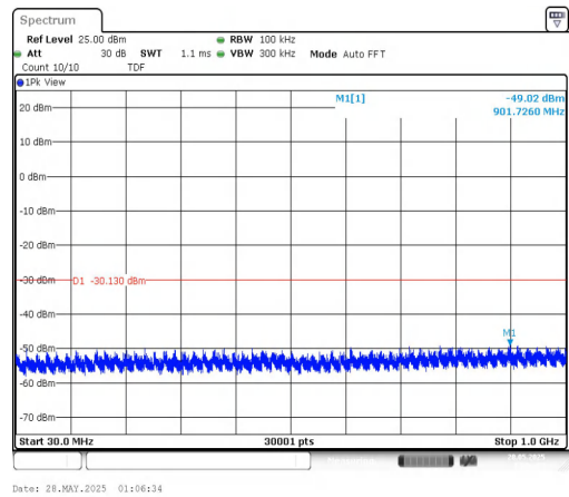
11N40MIMO-Ant2-2452-30~1000-PASS
