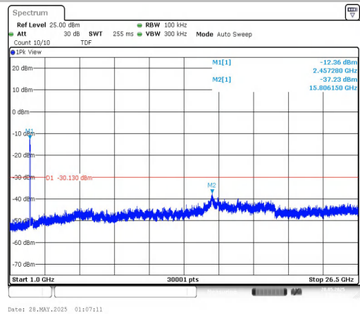
11N40MIMO-Ant2-2452-1000~26500-PASS
