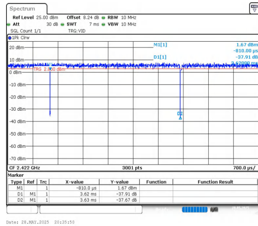
NTNV-11AX40MIMO-Ant2-2422
