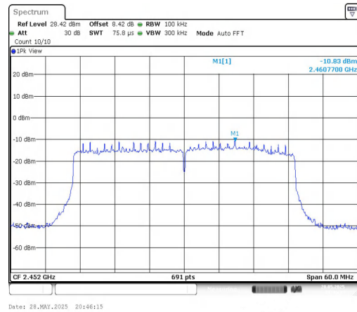
11AX40MIMO-Ant2-2452-0~Reference-PASS
