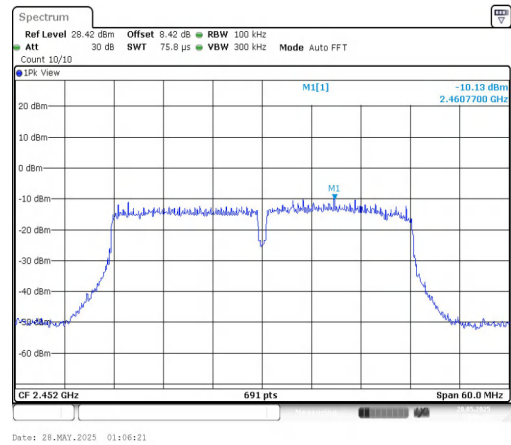
11N40MIMO-Ant2-2452-0~Reference-PASS
