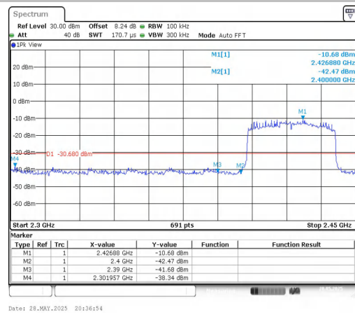
11AX40MIMO-Ant2-2422-PASS
