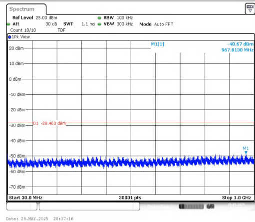
11AX40MIMO-Ant2-2422-30~1000-PASS
