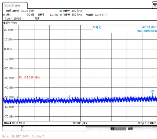
11N40MIMO-Ant1-2452-30~1000-PASS
