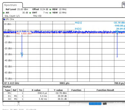
NTNV-11AX20MIMO-Ant2-2412
