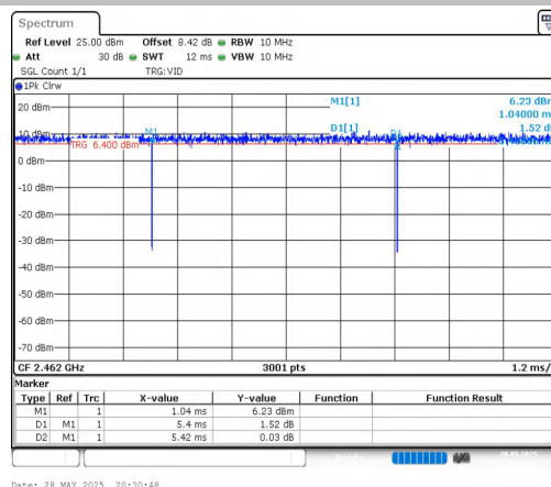
NTNV-11AX20MIMO-Ant2-2462
