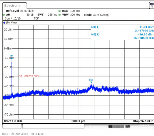
11N40MIMO-Ant1-2452-1000~26500-PASS
