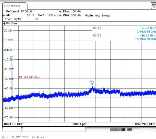
11AX40MIMO-Ant1-2452-1000~26500-PASS
