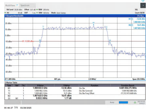
Band2-10MHz-16QAM-19150-50RB#0-PASS
