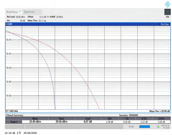
Band2-10MHz-QPSK-19150-50RB#0-PASS
