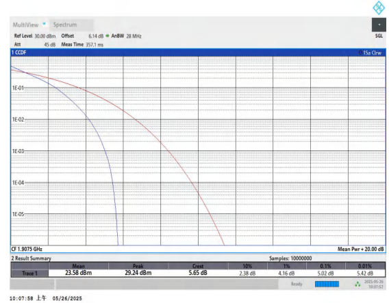
Band2-5MHz-QPSK-19175-25RB#0-PASS
