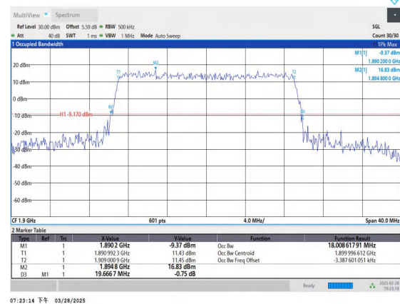
Band2-20MHz-16QAM-19100-100RB#0-PASS
