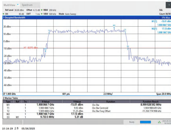
Band2-10MHz-QPSK-19150-50RB#0-PASS
