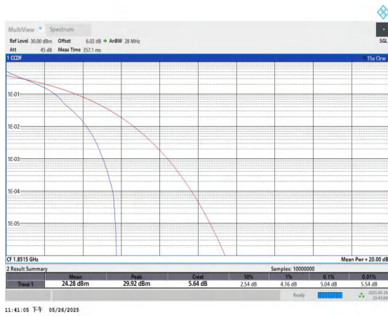
Band25-3MHz-QPSK-26055-1RB#0-PASS
