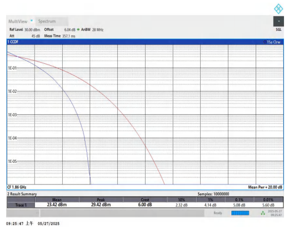
Band25-20MHz-QPSK-26140-100RB#0-PASS
