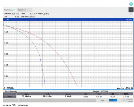
Band25-15MHz-QPSK-26615-75RB#0-PASS
