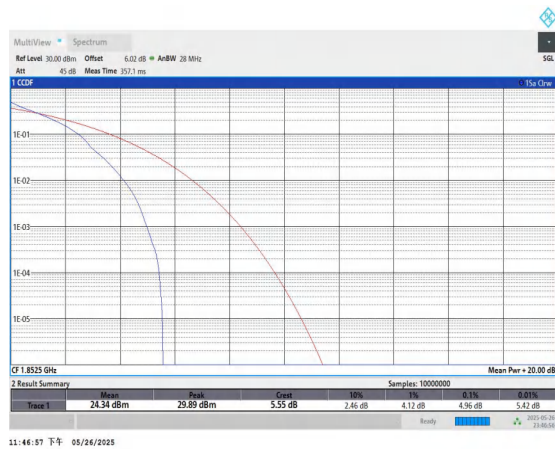
Band25-5MHz-QPSK-26065-1RB#0-PASS
