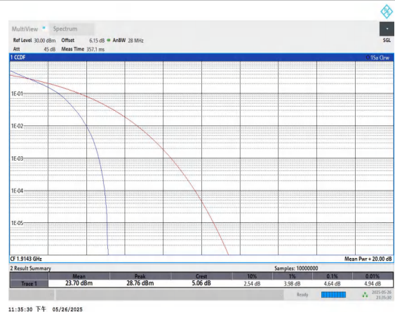
Band25-1.4MHz-QPSK-26683-6RB#0-PASS
