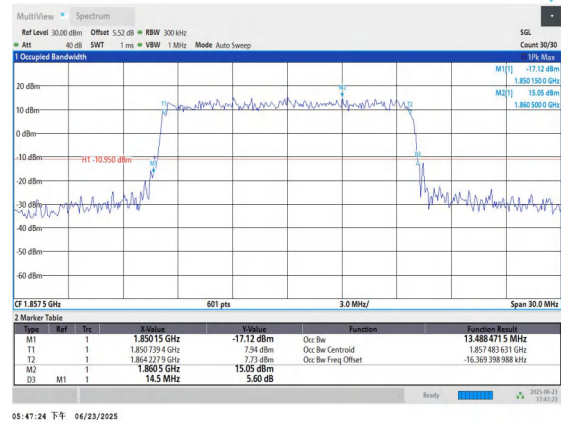
Band25-15MHz-16QAM-26115-75RB#0-PASS
