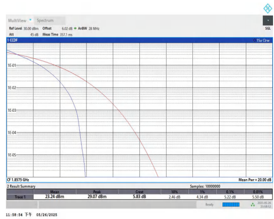
Band25-15MHz-QPSK-26115-75RB#0-PASS
