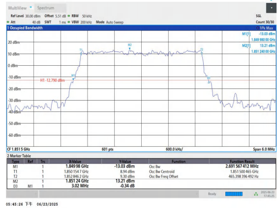
Band25-3MHz-16QAM-26055-15RB#0-PASS
