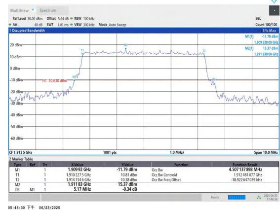
Band25-5MHz-16QAM-26665-25RB#0-PASS
