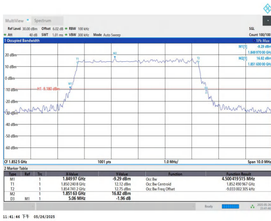
Band25-5MHz-QPSK-26065-25RB#0-PASS
