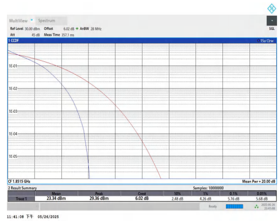
Band25-3MHz-QPSK-26055-15RB#0-PASS
