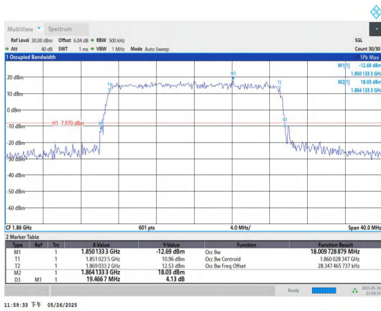
Band25-20MHz-QPSK-26140-100RB#0-PASS
