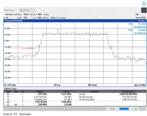
Band25-3MHz-16QAM-26675-15RB#0-PASS
