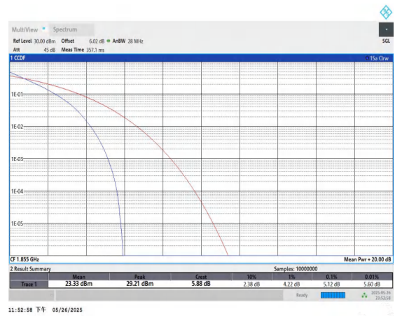
Band25-10MHz-QPSK-26090-50RB#0-PASS
