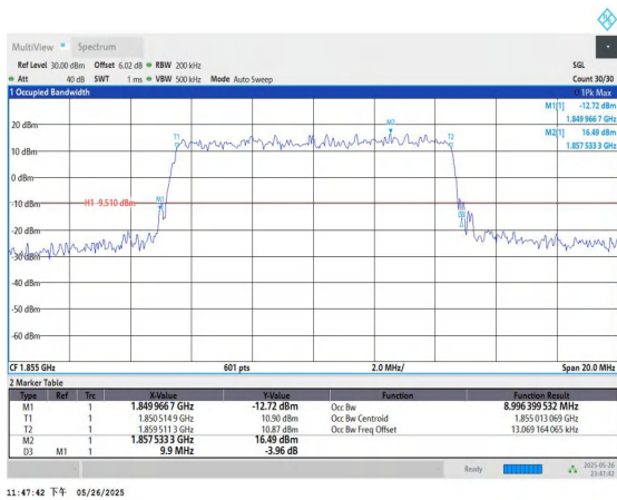
Band25-10MHz-QPSK-26090-50RB#0-PASS
