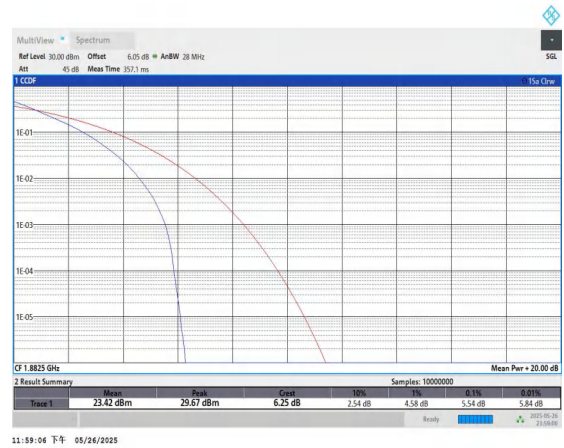
Band25-15MHz-QPSK-26365-75RB#0-PASS
