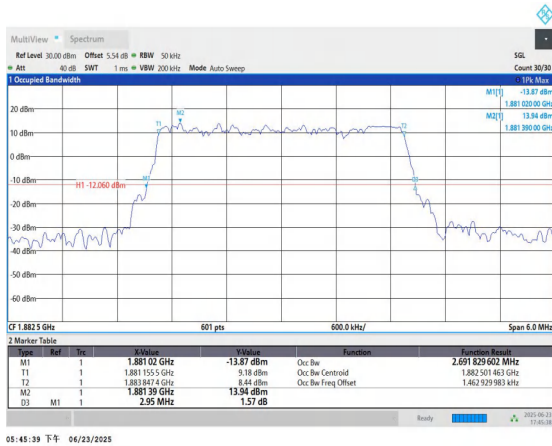
Band25-3MHz-16QAM-26365-15RB#0-PASS
