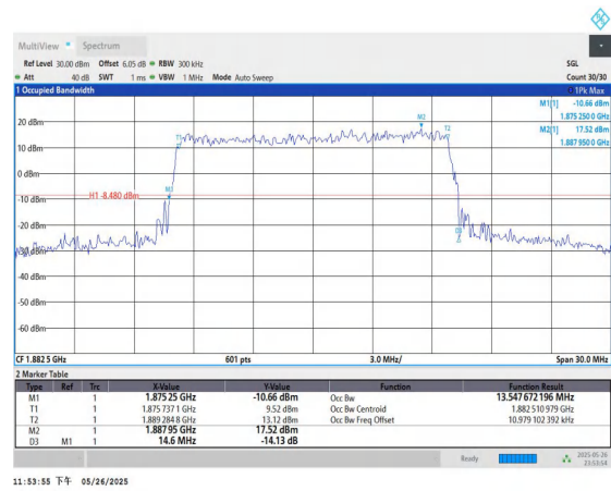
Band25-15MHz-QPSK-26365-75RB#0-PASS
