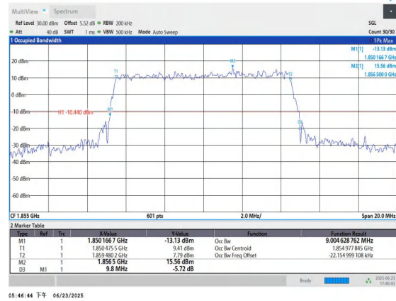
Band25-10MHz-16QAM-26090-50RB#0-PASS
