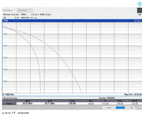
Band25-15MHz-QPSK-26365-1RB#0-PASS
