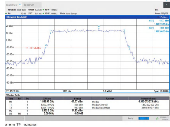
Band25-5MHz-16QAM-26065-25RB#0-PASS
