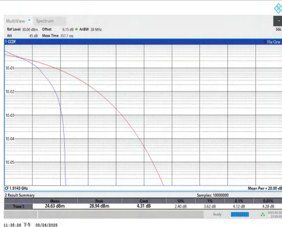
Band25-1.4MHz-QPSK-26683-1RB#0-PASS
