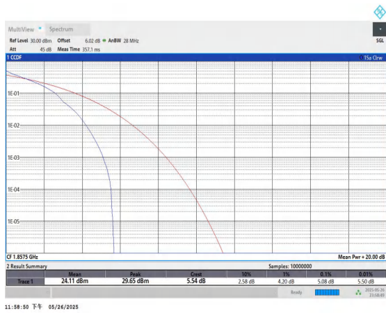
Band25-15MHz-QPSK-26115-1RB#0-PASS
