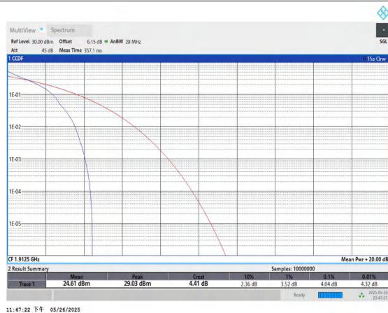
Band25-5MHz-QPSK-26665-1RB#0-PASS
