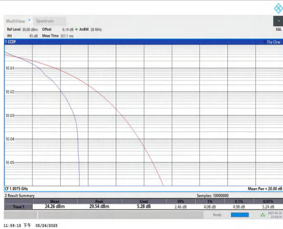
Band25-15MHz-QPSK-26615-1RB#0-PASS
