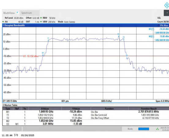
Band25-3MHz-QPSK-26055-15RB#0-PASS
