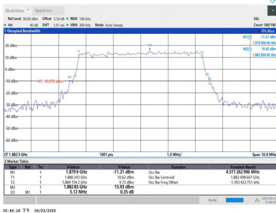
Band25-5MHz-16QAM-26365-25RB#0-PASS
