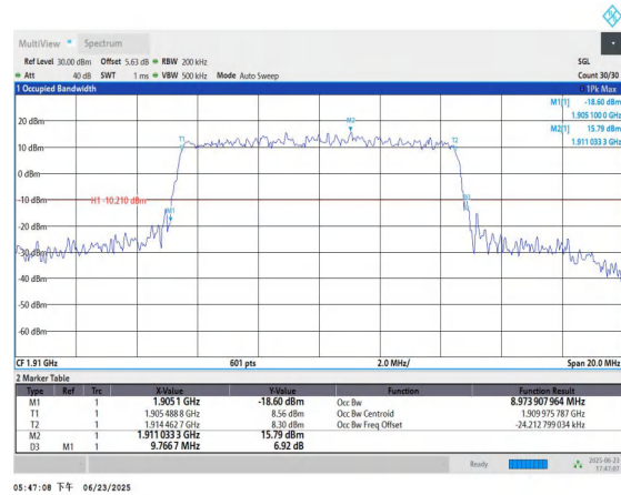
Band25-10MHz-16QAM-26640-50RB#0-PASS
