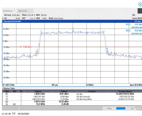
Band25-15MHz-QPSK-26115-75RB#0-PASS
