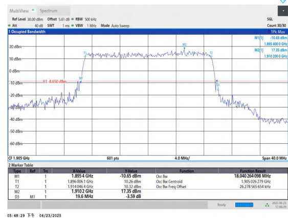
Band25-20MHz-16QAM-26590-100RB#0-PASS
