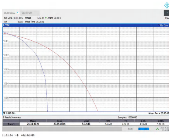
Band25-10MHz-QPSK-26090-1RB#0-PASS
