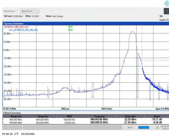
26(824-849)-5MHz-QPSK-27015-1RB#24-PASS
