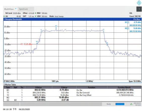
26(824-849)-5MHz-16QAM-27015-25RB#0-PASS
