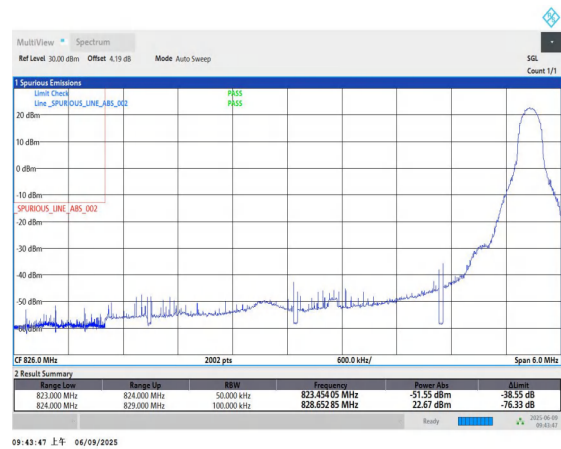
26(824-849)-5MHz-QPSK-26815-1RB#24-PASS
