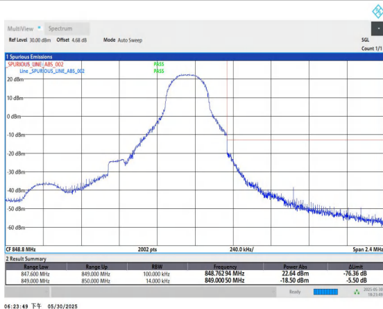
26(824-849)-1.4MHz-QPSK-27033-1RB#5-PASS
