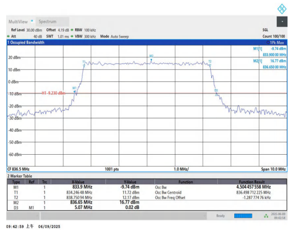
26(824-849)-5MHz-QPSK-26915-25RB#0-PASS
