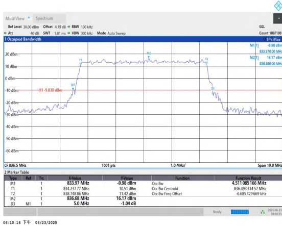
26(824-849)-5MHz-16QAM-26915-25RB#0-PASS
