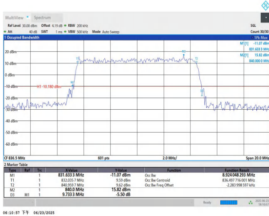
26(824-849)-10MHz-16QAM-26915-50RB#0-PASS
