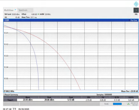
26(824-849)-1.4MHz-QPSK-27033-6RB#0-PASS
