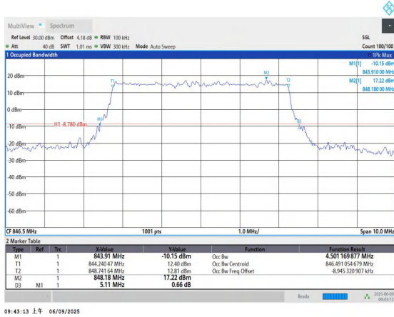
26(824-849)-5MHz-QPSK-27015-25RB#0-PASS
