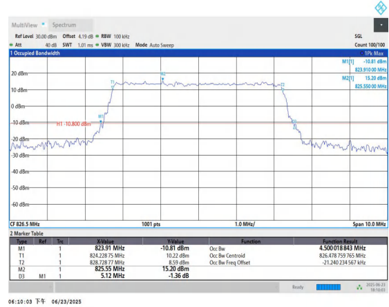
26(824-849)-5MHz-16QAM-26815-25RB#0-PASS
