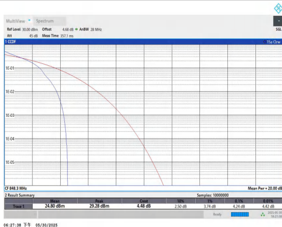
26(824-849)-1.4MHz-QPSK-27033-1RB#0-PASS
