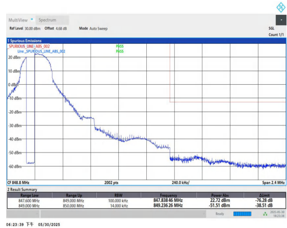
26(824-849)-1.4MHz-QPSK-27033-1RB#0-PASS
