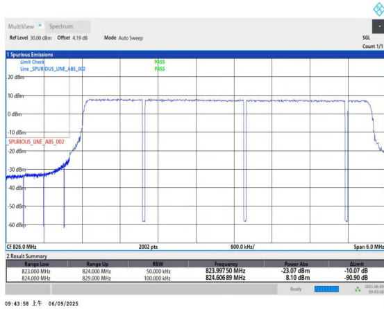
26(824-849)-5MHz-QPSK-26815-25RB#0-PASS
