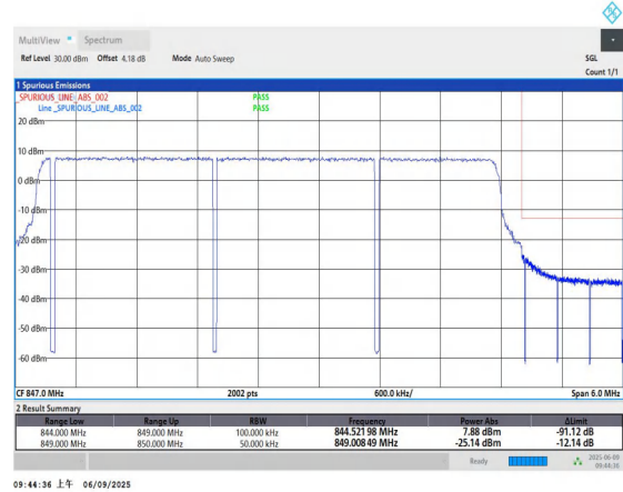
26(824-849)-5MHz-QPSK-27015-25RB#0-PASS
