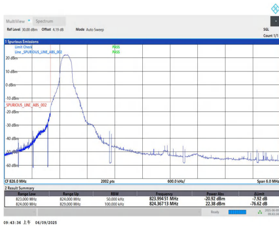
26(824-849)-5MHz-QPSK-26815-1RB#0-PASS
