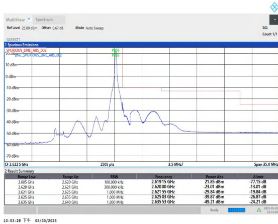
Band38-15MHz-QPSK-38175-1RB#74-PASS
