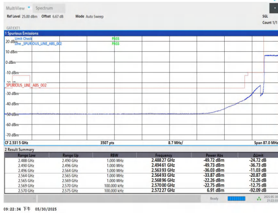
Band38-5MHz-16QAM-37775-25RB#0-PASS
