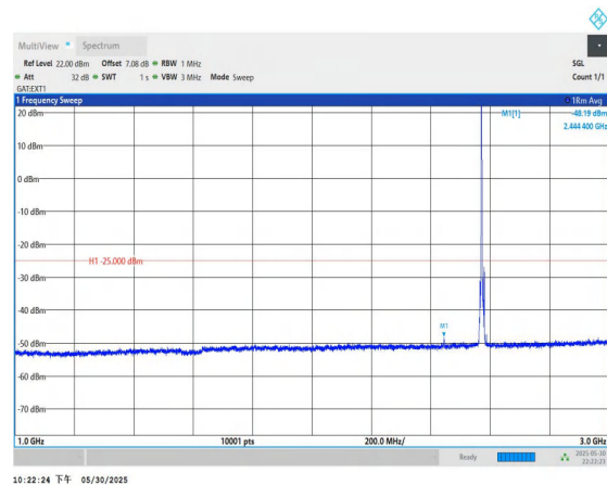
Band38-10MHz-16QAM-37800-1RB#0-1000~3000-PASS
