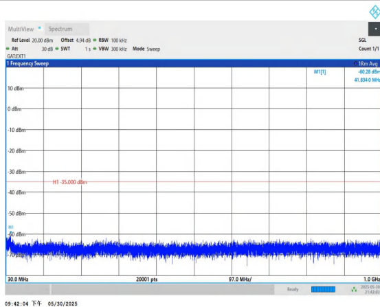
Band38-5MHz-16QAM-38225-1RB#0-30~1000-PASS
