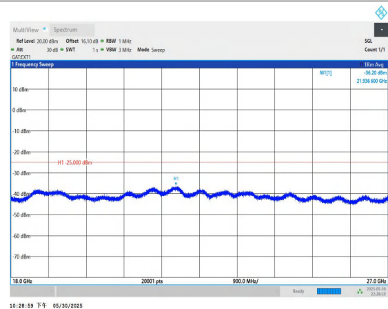
Band38-10MHz-QPSK-38200-1RB#0-18000~27000-PASS
