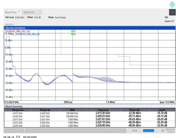
Band38-5MHz-QPSK-38225-1RB#0-PASS
