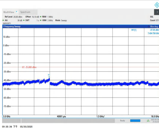
Band38-5MHz-16QAM-37775-1RB#0-3000~18000-PASS
