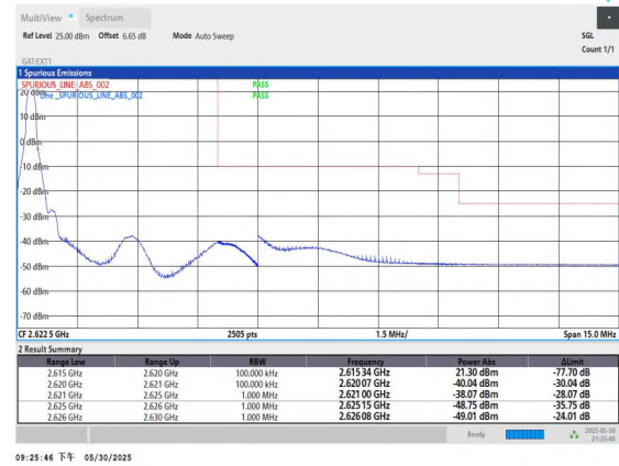
Band38-5MHz-16QAM-38225-1RB#0-PASS
