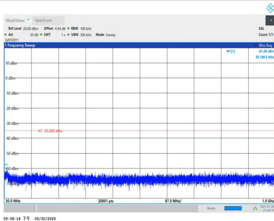
Band38-5MHz-16QAM-38000-1RB#0-30~1000-PASS
