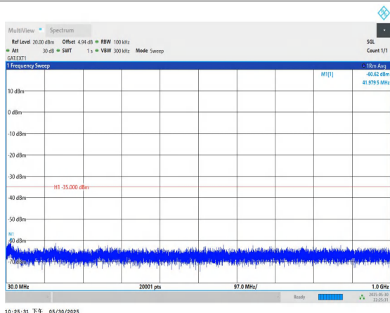
Band38-10MHz-16QAM-38000-1RB#0-30~1000-PASS
