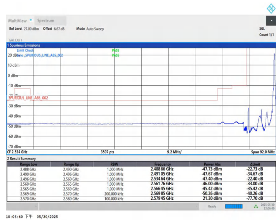
Band38-10MHz-16QAM-37800-1RB#49-PASS
