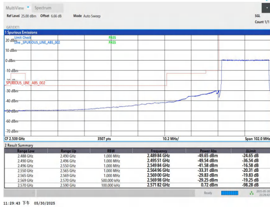
Band38-20MHz-16QAM-37850-100RB#0-PASS
