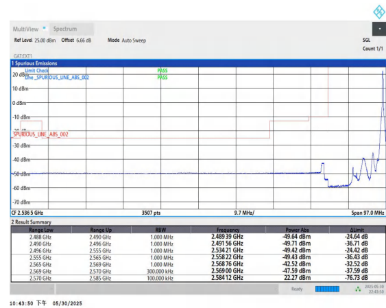
Band38-15MHz-QPSK-37825-1RB#74-PASS
