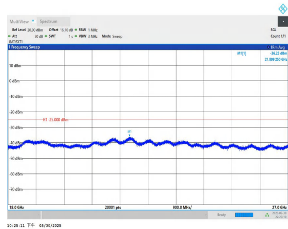
Band38-10MHz-QPSK-38000-1RB#0-18000~27000-PASS
