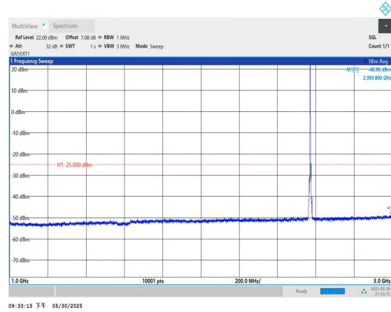
Band38-5MHz-QPSK-37775-1RB#0-1000~3000-PASS
