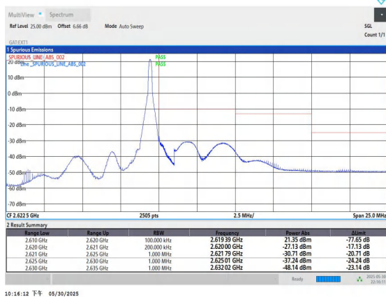
Band38-10MHz-16QAM-38200-1RB#49-PASS
