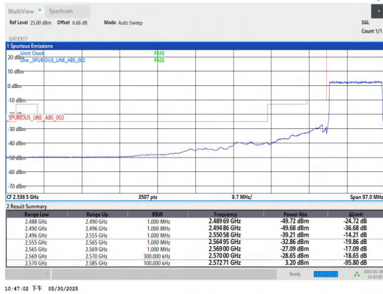
Band38-15MHz-QPSK-37825-75RB#0-PASS
