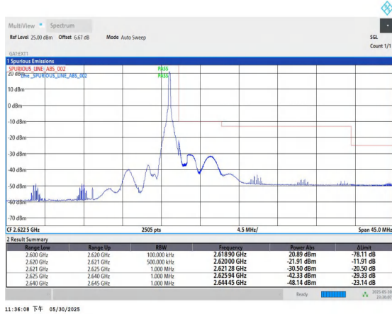
Band38-20MHz-16QAM-38150-1RB#0-PASS
