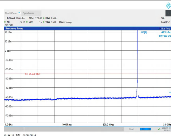
Band38-10MHz-16QAM-38000-1RB#0-1000~3000-PASS
