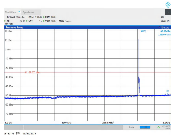
Band38-5MHz-QPSK-38225-1RB#0-1000~3000-PASS
