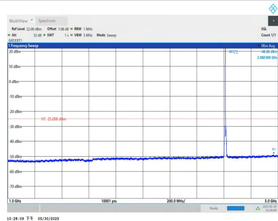
Band38-10MHz-QPSK-38200-1RB#0-1000~3000-PASS
