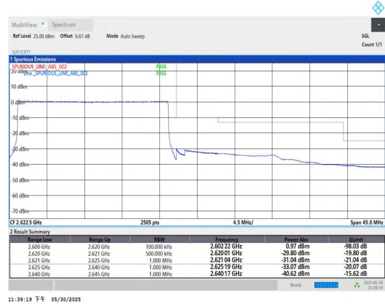
Band38-20MHz-16QAM-38150-100RB#0-PASS
