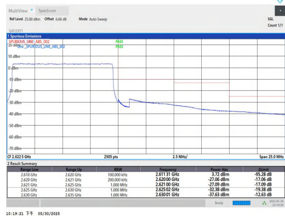
Band38-10MHz-16QAM-38200-50RB#0-PASS
