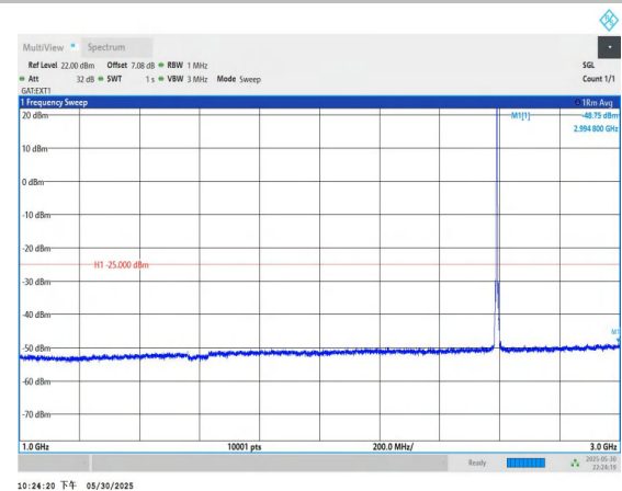
Band38-10MHz-QPSK-38000-1RB#0-1000~3000-PASS
