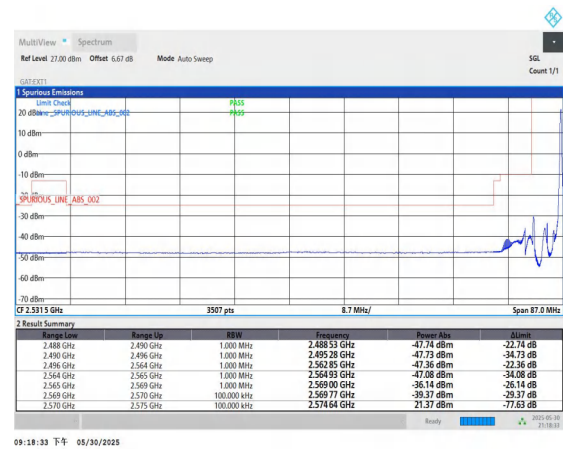
Band38-5MHz-16QAM-37775-1RB#24-PASS
