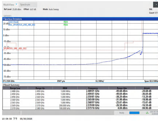
Band38-10MHz-16QAM-37800-50RB#0-PASS
