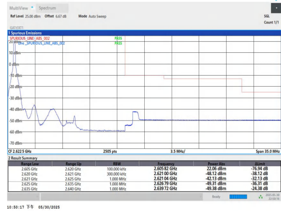
Band38-15MHz-QPSK-38175-1RB#0-PASS
