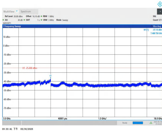
Band38-5MHz-QPSK-37775-1RB#0-3000~18000-PASS
