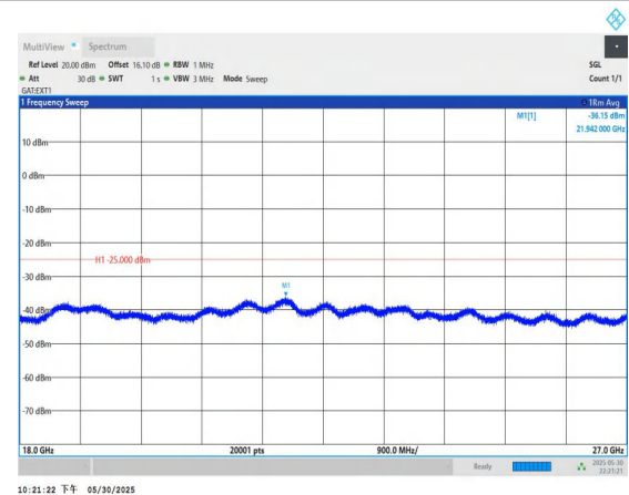
Band38-10MHz-QPSK-37800-1RB#0-18000~27000-PASS
