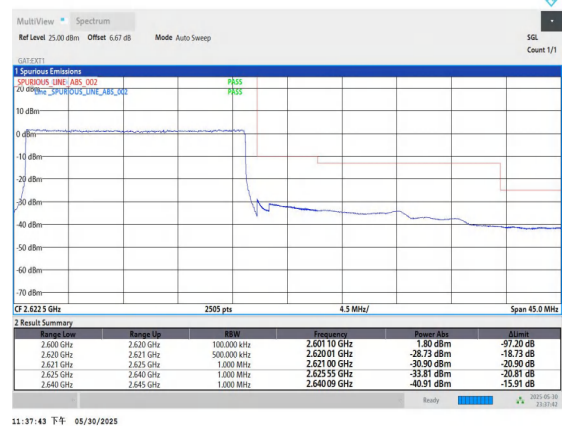
Band38-20MHz-QPSK-38150-100RB#0-PASS
