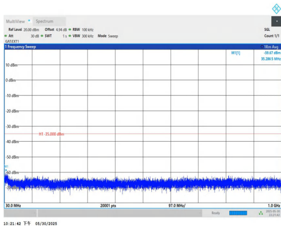
Band38-10MHz-16QAM-37800-1RB#0-30~1000-PASS
