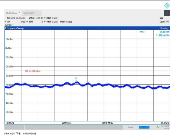
Band38-5MHz-16QAM-38225-1RB#0-18000~27000-PASS
