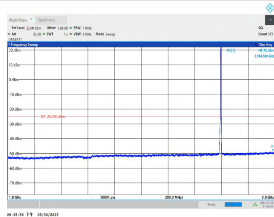
Band38-5MHz-16QAM-38000-1RB#0-1000~3000-PASS
