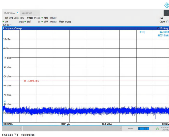
Band38-5MHz-16QAM-37775-1RB#0-30~1000-PASS
