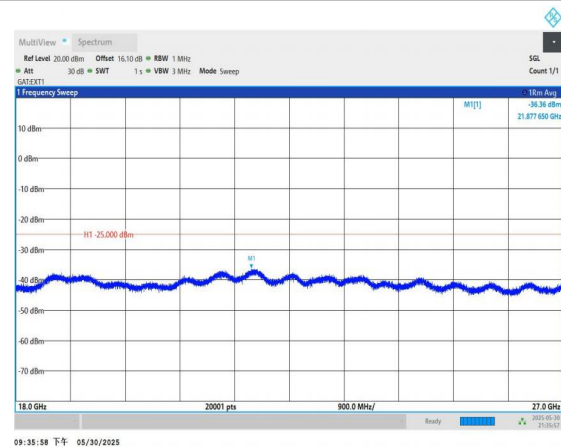
Band38-5MHz-16QAM-37775-1RB#0-18000~27000-PASS
