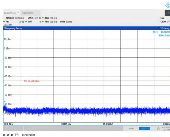
Band38-10MHz-QPSK-37800-1RB#0-30~1000-PASS
