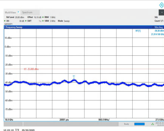
Band38-10MHz-16QAM-37800-1RB#0-18000~27000-PASS
