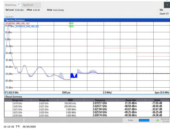
Band38-10MHz-16QAM-38200-1RB#0-PASS
