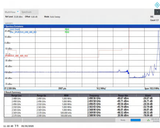
Band38-20MHz-16QAM-37850-1RB#99-PASS
