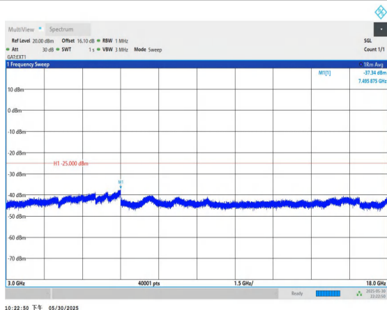
Band38-10MHz-16QAM-37800-1RB#0-3000~18000-PASS
