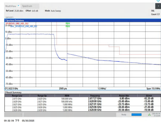
Band38-5MHz-16QAM-38225-25RB#0-PASS
