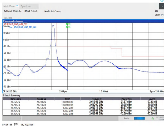
Band38-5MHz-16QAM-38225-1RB#24-PASS
