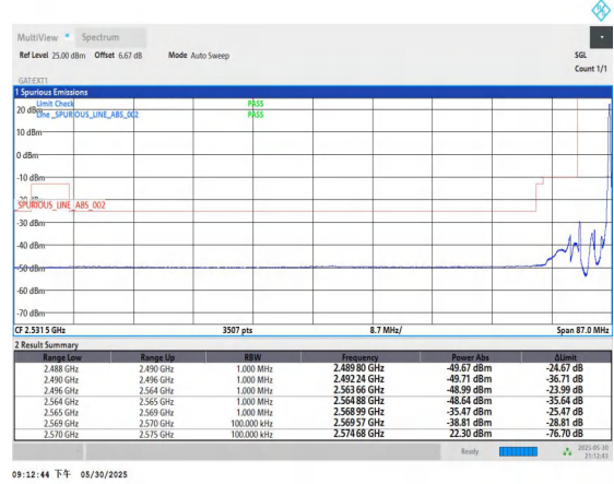
Band38-5MHz-QPSK-37775-1RB#24-PASS
