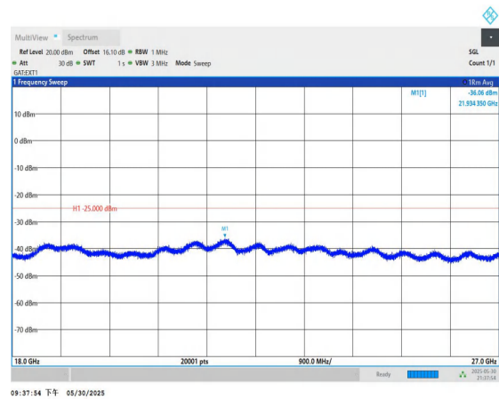
Band38-5MHz-QPSK-38000-1RB#0-18000~27000-PASS
