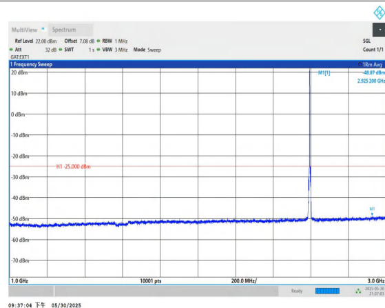
Band38-5MHz-QPSK-38000-1RB#0-1000~3000-PASS
