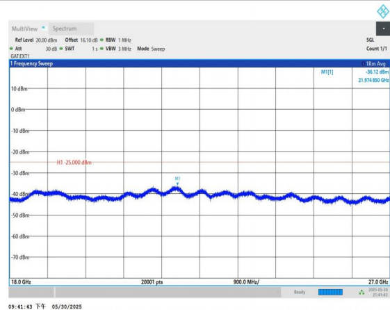
Band38-5MHz-QPSK-38225-1RB#0-18000~27000-PASS
