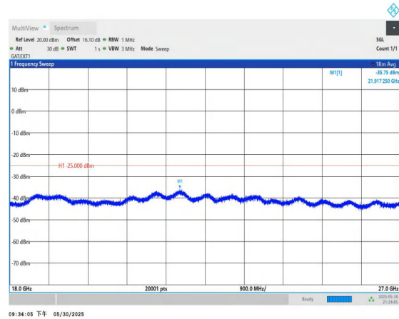
Band38-5MHz-QPSK-37775-1RB#0-18000~27000-PASS
