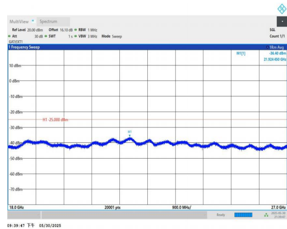
Band38-5MHz-16QAM-38000-1RB#0-18000~27000-PASS
