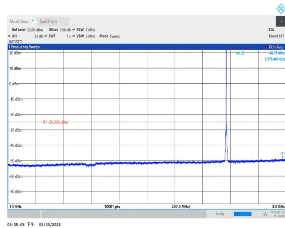
Band38-5MHz-16QAM-37775-1RB#0-1000~3000-PASS
