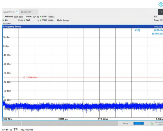
Band38-5MHz-QPSK-38225-1RB#0-30~1000-PASS
