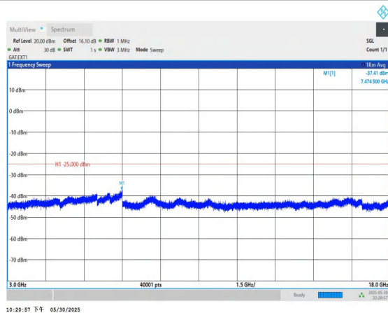
Band38-10MHz-QPSK-37800-1RB#0-3000~18000-PASS
