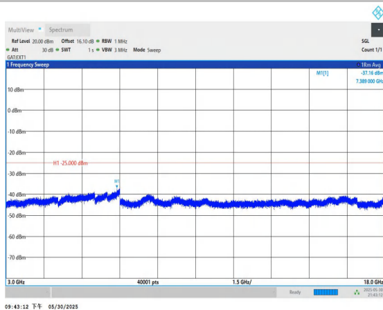
Band38-5MHz-16QAM-38225-1RB#0-3000~18000-PASS
