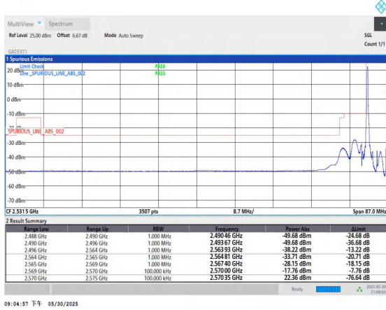
Band38-5MHz-QPSK-37775-1RB#0-PASS
