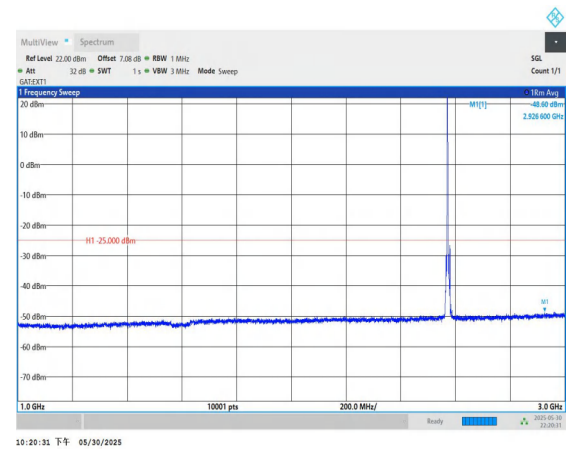
Band38-10MHz-QPSK-37800-1RB#0-1000~3000-PASS
