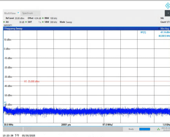
Band38-10MHz-QPSK-38000-1RB#0-30~1000-PASS
