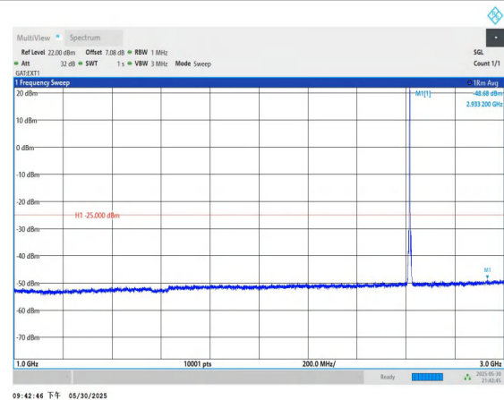
Band38-5MHz-16QAM-38225-1RB#0-1000~3000-PASS
