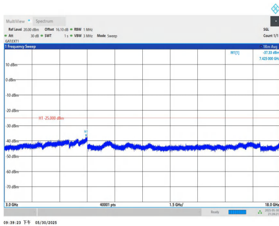
Band38-5MHz-16QAM-38000-1RB#0-3000~18000-PASS
