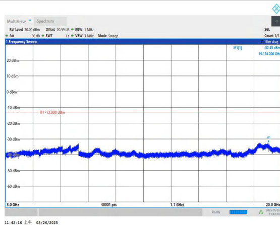
Band4-15MHz-QPSK-20325-1RB#0-3000~20000-PASS
