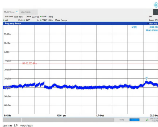
Band4-20MHz-QPSK-20175-1RB#0-3000~20000-PASS
