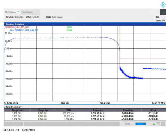
Band4-5MHz-QPSK-20375-25RB#0-PASS
