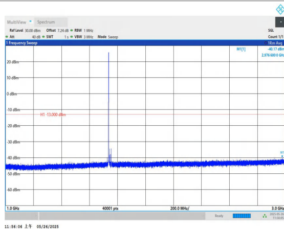
Band4-20MHz-QPSK-20300-1RB#0-1000~3000-PASS
