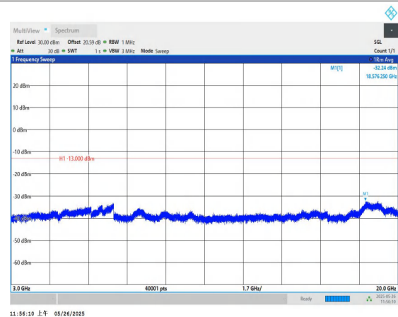
Band4-20MHz-QPSK-20300-1RB#0-3000~20000-PASS
