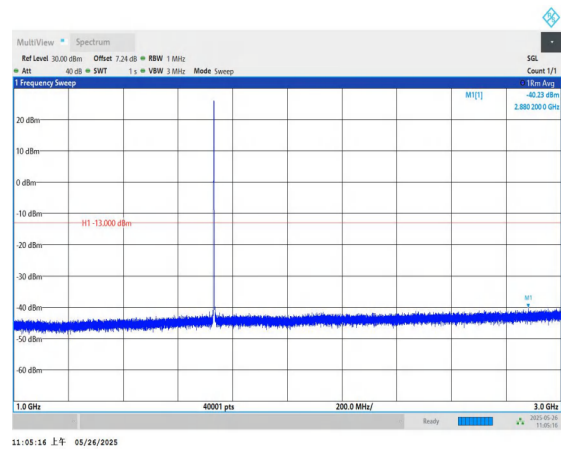
Band4-3MHz-QPSK-20175-1RB#0-1000~3000-PASS
