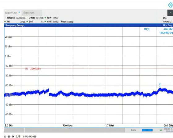
Band4-10MHz-QPSK-20350-1RB#0-3000~20000-PASS
