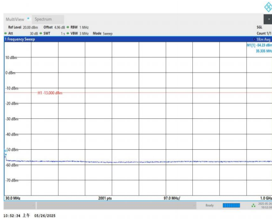
Band4-1.4MHz-QPSK-19957-1RB#0-30~1000-PASS
