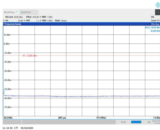
Band4-5MHz-QPSK-19975-1RB#0-30~1000-PASS
