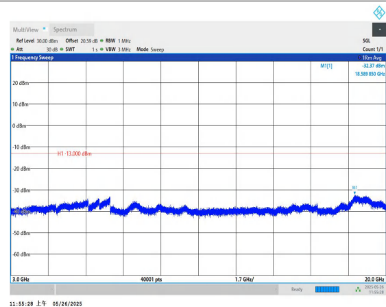
Band4-20MHz-QPSK-20050-1RB#0-3000~20000-PASS
