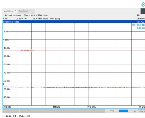
Band4-15MHz-QPSK-20025-1RB#0-30~1000-PASS
