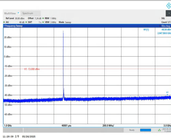
Band4-10MHz-QPSK-20000-1RB#0-1000~3000-PASS
