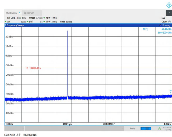
Band4-5MHz-QPSK-20375-1RB#0-1000~3000-PASS
