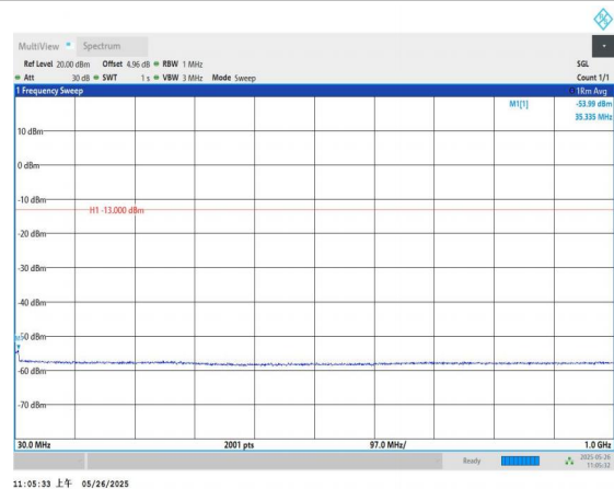
Band4-3MHz-QPSK-20385-1RB#0-30~1000-PASS
