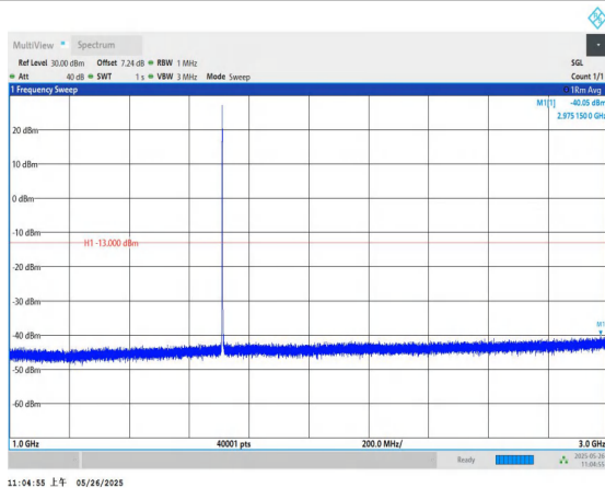
Band4-3MHz-QPSK-19965-1RB#0-1000~3000-PASS
