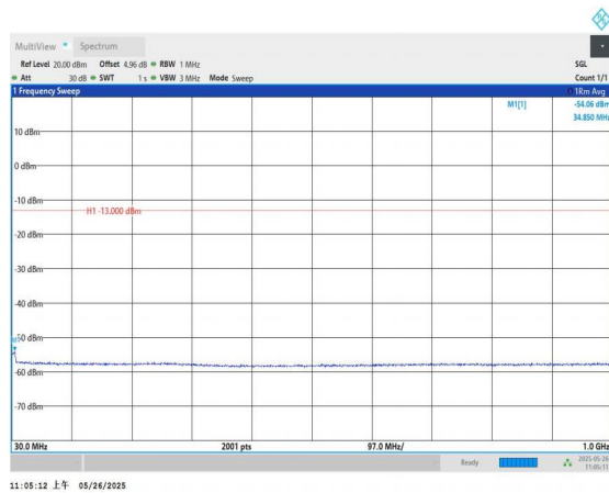
Band4-3MHz-QPSK-20175-1RB#0-30~1000-PASS
