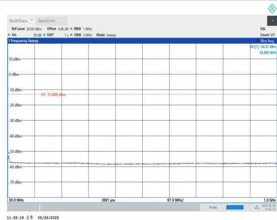
Band4-20MHz-QPSK-20050-1RB#0-30~1000-PASS
