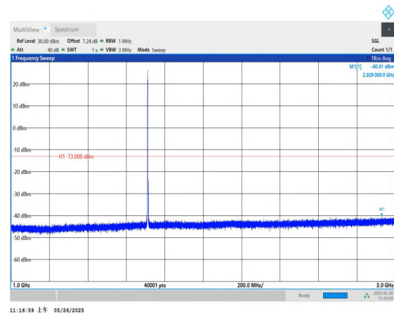
Band4-5MHz-QPSK-19975-1RB#0-1000~3000-PASS
