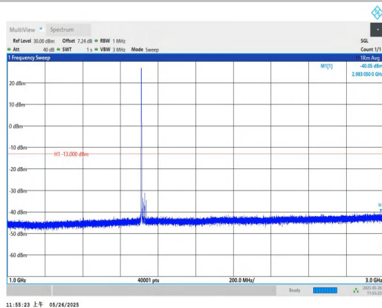
Band4-20MHz-QPSK-20050-1RB#0-1000~3000-PASS
