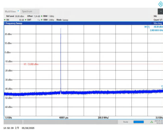
Band4-1.4MHz-QPSK-19957-1RB#0-1000~3000-PASS
