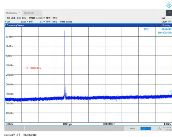
Band4-15MHz-QPSK-20025-1RB#0-1000~3000-PASS
