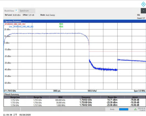
Band4-3MHz-QPSK-20385-15RB#0-PASS
