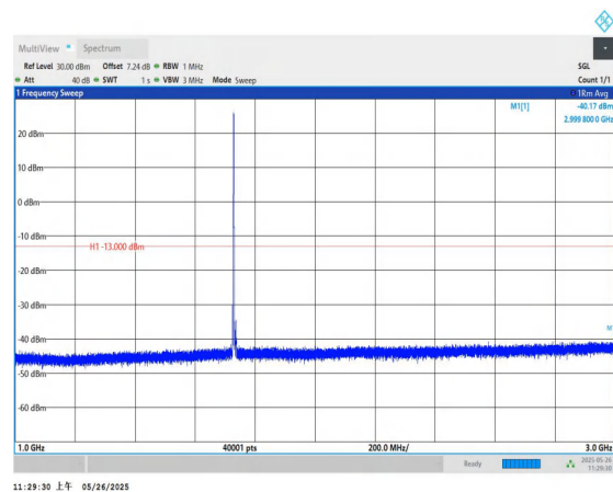
Band4-10MHz-QPSK-20175-1RB#0-1000~3000-PASS
