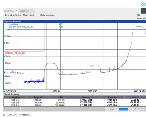
Band4-5MHz-QPSK-19975-1RB#24-PASS
