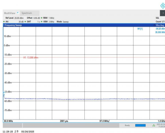
Band4-10MHz-QPSK-20175-1RB#0-30~1000-PASS
