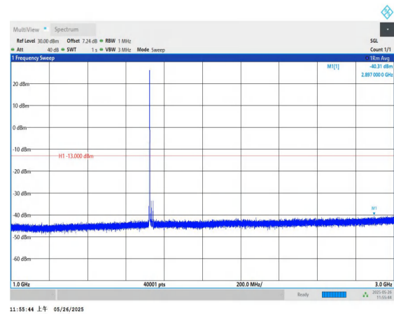
Band4-20MHz-QPSK-20175-1RB#0-1000~3000-PASS
