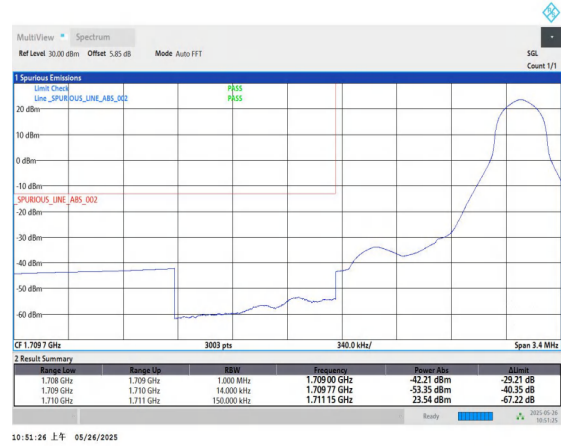
Band4-1.4MHz-QPSK-19957-1RB#5-PASS
