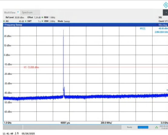
Band4-15MHz-QPSK-20175-1RB#0-1000~3000-PASS
