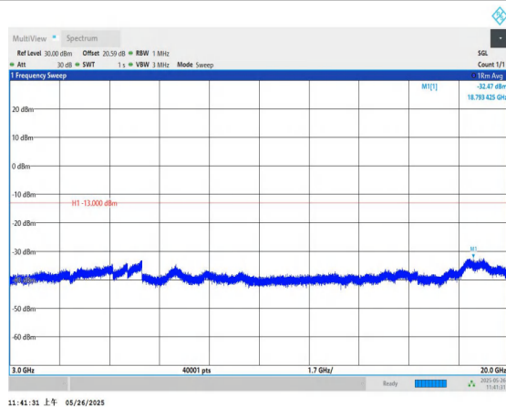
Band4-15MHz-QPSK-20025-1RB#0-3000~20000-PASS
