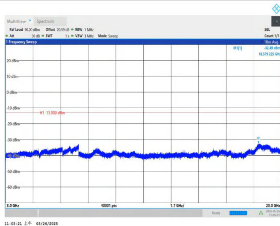
Band4-3MHz-QPSK-20175-1RB#0-3000~20000-PASS
