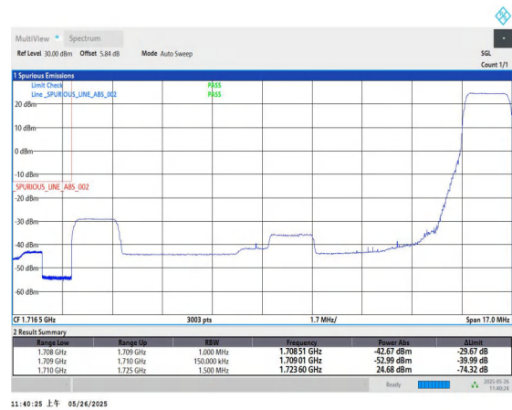
Band4-15MHz-QPSK-20025-1RB#74-PASS
