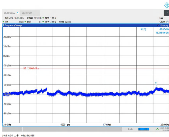
Band4-1.4MHz-QPSK-20393-1RB#0-3000~20000-PASS
