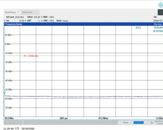
Band4-10MHz-QPSK-20350-1RB#0-30~1000-PASS
