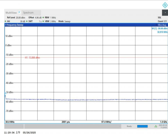
Band4-10MHz-QPSK-20000-1RB#0-30~1000-PASS
