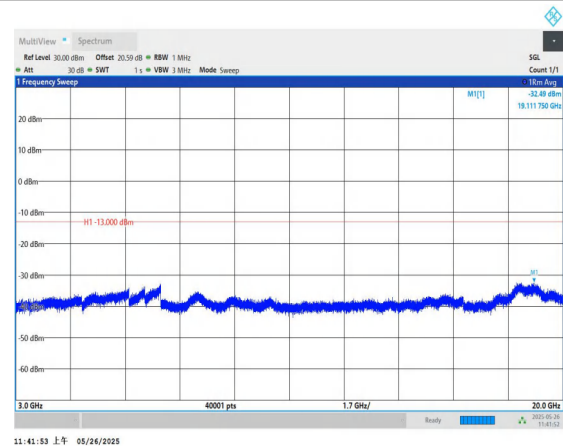
Band4-15MHz-QPSK-20175-1RB#0-3000~20000-PASS
