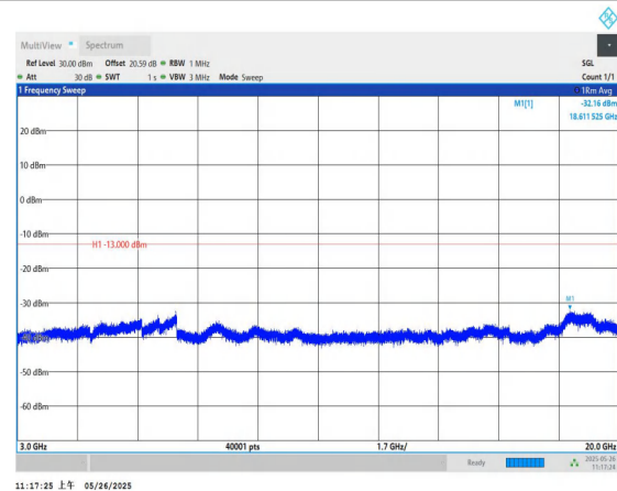
Band4-5MHz-QPSK-20175-1RB#0-3000~20000-PASS
