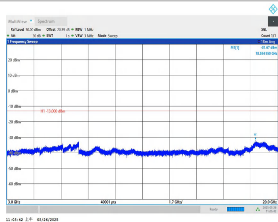
Band4-3MHz-QPSK-20385-1RB#0-3000~20000-PASS
