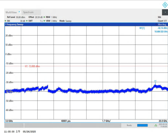
Band4-3MHz-QPSK-19965-1RB#0-3000~20000-PASS
