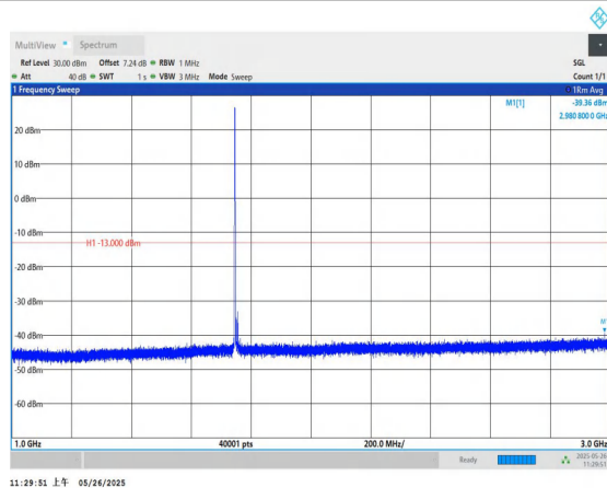
Band4-10MHz-QPSK-20350-1RB#0-1000~3000-PASS
