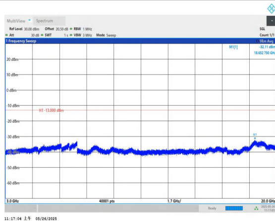
Band4-5MHz-QPSK-19975-1RB#0-3000~20000-PASS
