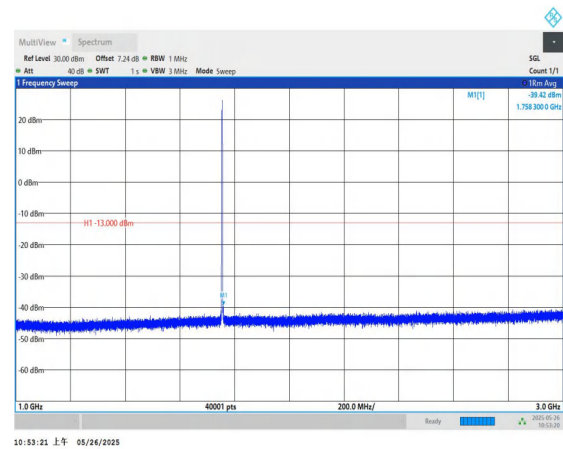
Band4-1.4MHz-QPSK-20393-1RB#0-1000~3000-PASS
