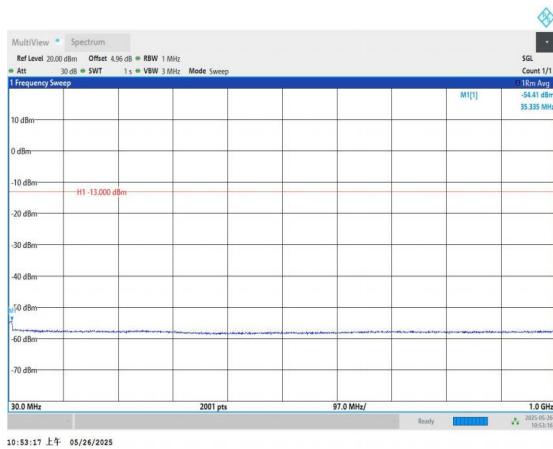
Band4-1.4MHz-QPSK-20393-1RB#0-30~1000-PASS
