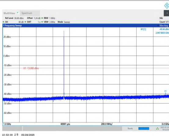
Band4-1.4MHz-QPSK-20175-1RB#0-1000~3000-PASS
