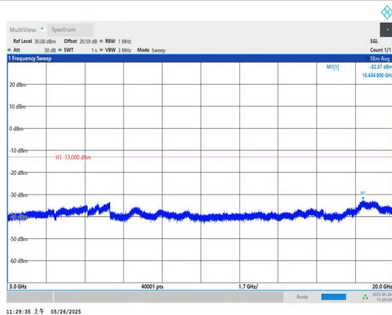
Band4-10MHz-QPSK-20175-1RB#0-3000~20000-PASS
