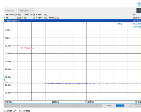
Band4-5MHz-QPSK-20175-1RB#0-30~1000-PASS
