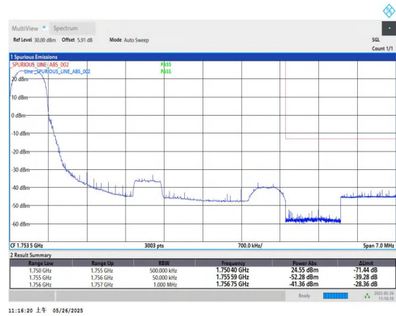
Band4-5MHz-QPSK-20375-1RB#0-PASS
