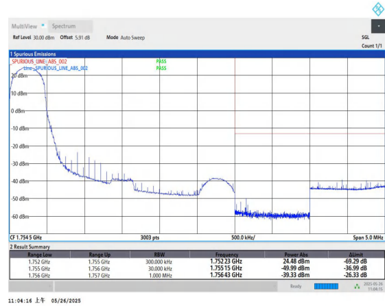
Band4-3MHz-QPSK-20385-1RB#0-PASS
