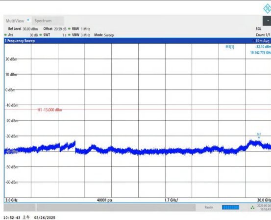
Band4-1.4MHz-QPSK-19957-1RB#0-3000~20000-PASS
