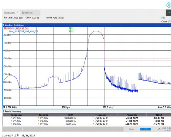
Band4-3MHz-QPSK-20385-1RB#14-PASS
