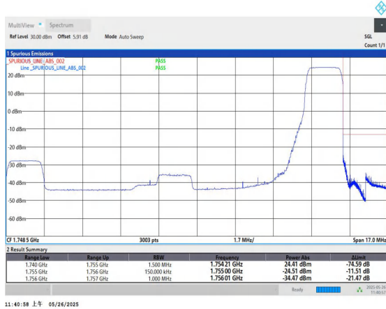
Band4-15MHz-QPSK-20325-1RB#74-PASS
