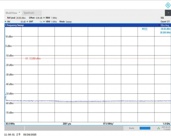
Band4-20MHz-QPSK-20300-1RB#0-30~1000-PASS
