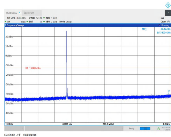
Band4-15MHz-QPSK-20325-1RB#0-1000~3000-PASS
