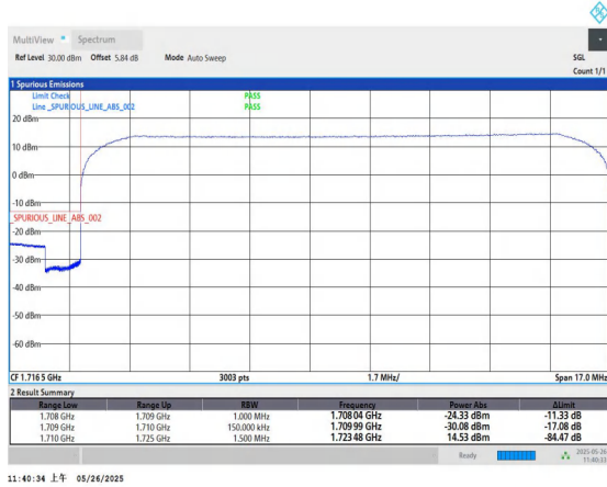
Band4-15MHz-QPSK-20025-75RB#0-PASS
