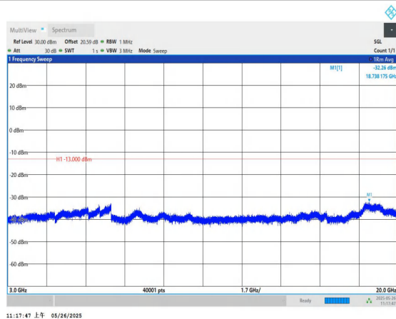
Band4-5MHz-QPSK-20375-1RB#0-3000~20000-PASS
