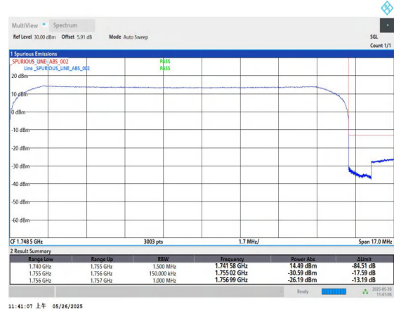
Band4-15MHz-QPSK-20325-75RB#0-PASS
