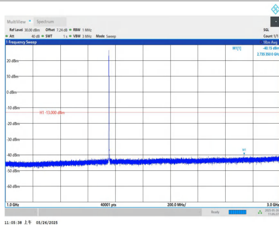
Band4-3MHz-QPSK-20385-1RB#0-1000~3000-PASS
