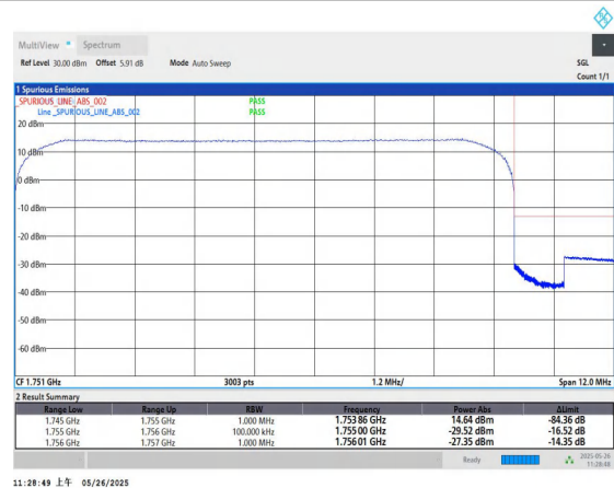
Band4-10MHz-QPSK-20350-50RB#0-PASS
