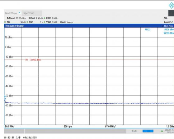
Band4-1.4MHz-QPSK-20175-1RB#0-30~1000-PASS
