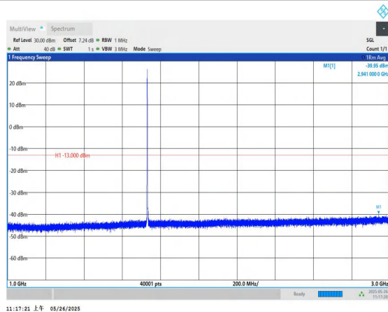
Band4-5MHz-QPSK-20175-1RB#0-1000~3000-PASS
