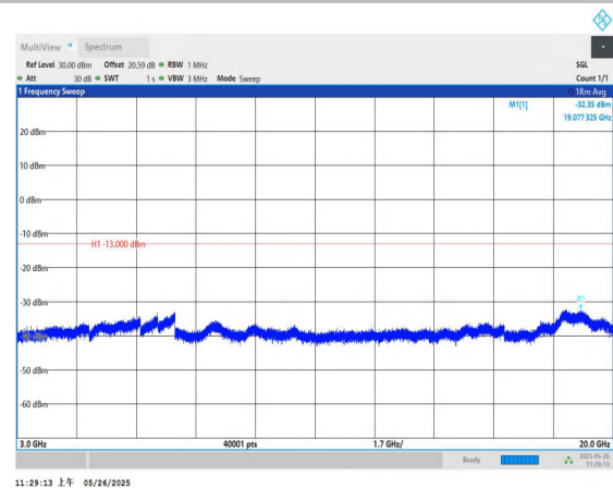
Band4-10MHz-QPSK-20000-1RB#0-3000~20000-PASS
