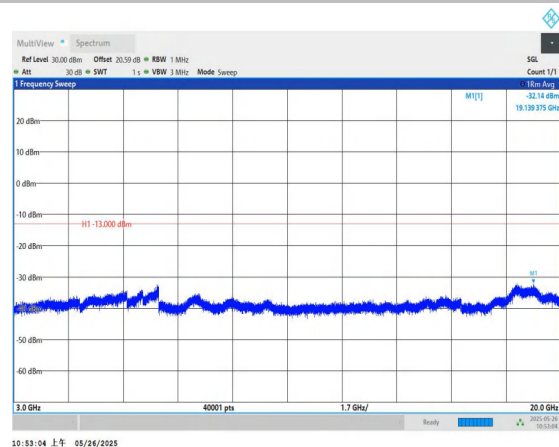
Band4-1.4MHz-QPSK-20175-1RB#0-3000~20000-PASS
