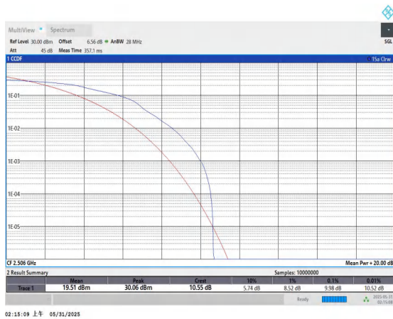
Band41-20MHz-16QAM-39750-1RB#0-PASS
