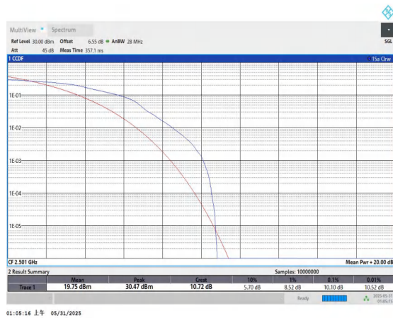
Band41-10MHz-16QAM-39700-1RB#0-PASS
