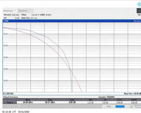
Band41-20MHz-QPSK-40620-1RB#0-PASS
