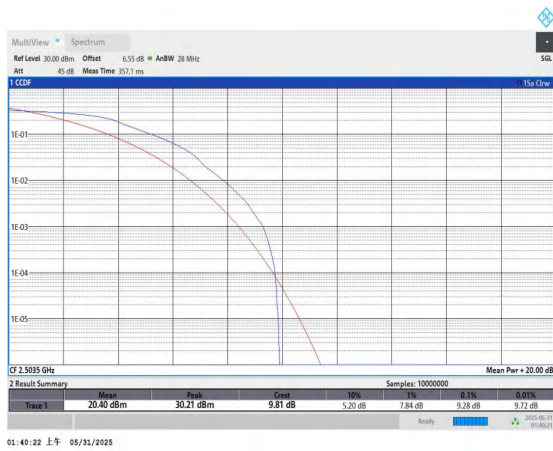
Band41-15MHz-QPSK-39725-1RB#0-PASS
