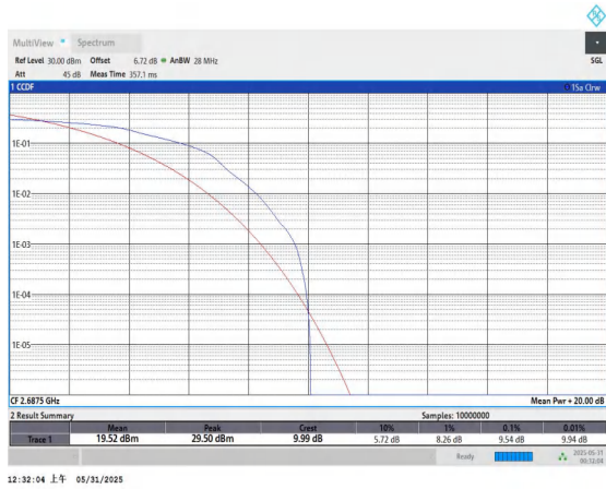
Band41-5MHz-16QAM-41565-1RB#0-PASS
