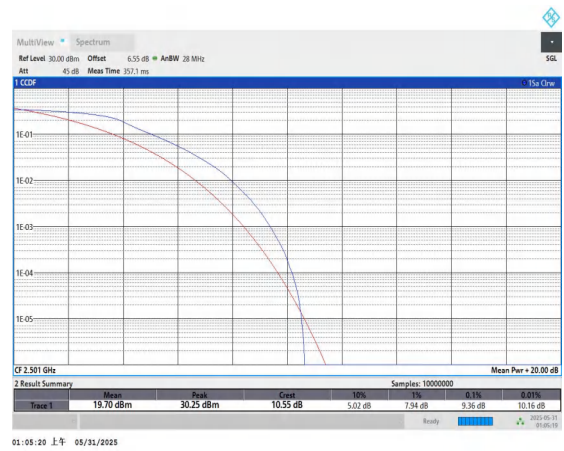
Band41-10MHz-QPSK-39700-50RB#0-PASS
