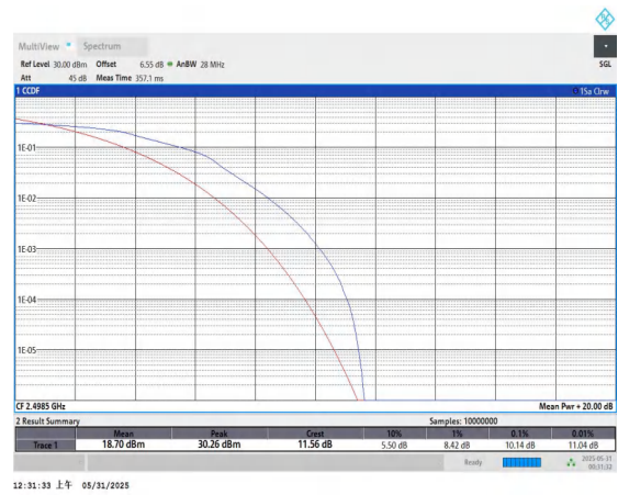
Band41-5MHz-16QAM-39675-25RB#0-PASS
