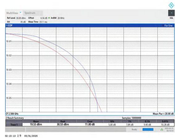
Band41-20MHz-QPSK-39750-100RB#0-PASS
