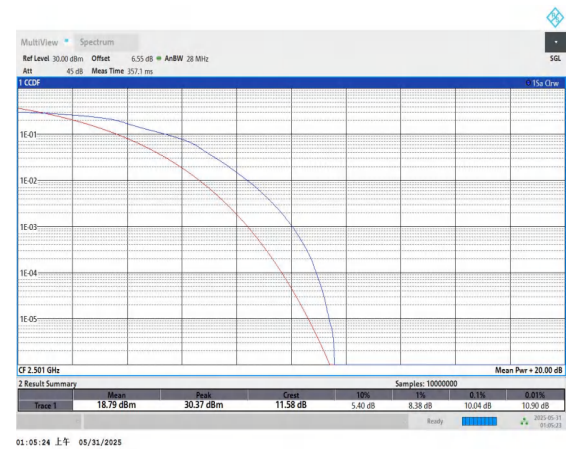
Band41-10MHz-16QAM-39700-50RB#0-PASS
