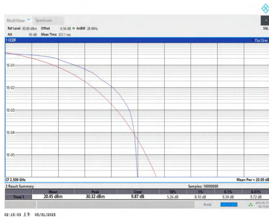
Band41-20MHz-QPSK-39750-1RB#0-PASS
