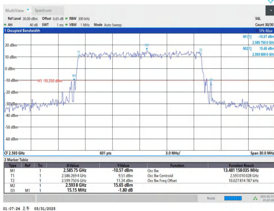
Band41-15MHz-16QAM-40620-75RB#0-PASS
