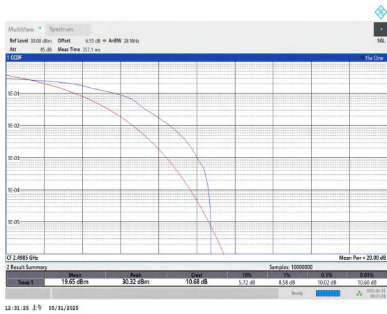
Band41-5MHz-16QAM-39675-1RB#0-PASS
