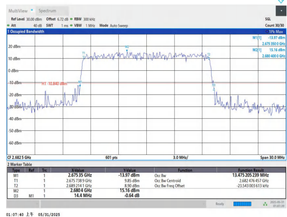
Band41-15MHz-16QAM-41515-75RB#0-PASS
