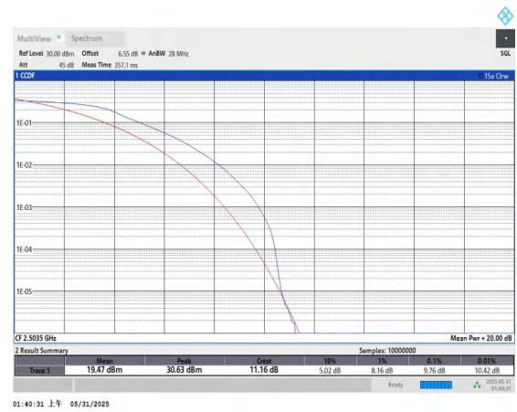
Band41-15MHz-QPSK-39725-75RB#0-PASS
