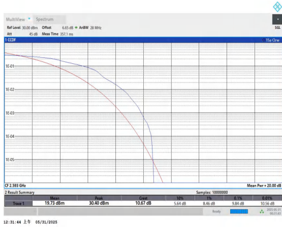
Band41-5MHz-16QAM-40620-1RB#0-PASS
