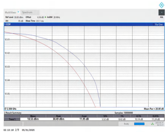
Band41-20MHz-16QAM-39750-100RB#0-PASS
