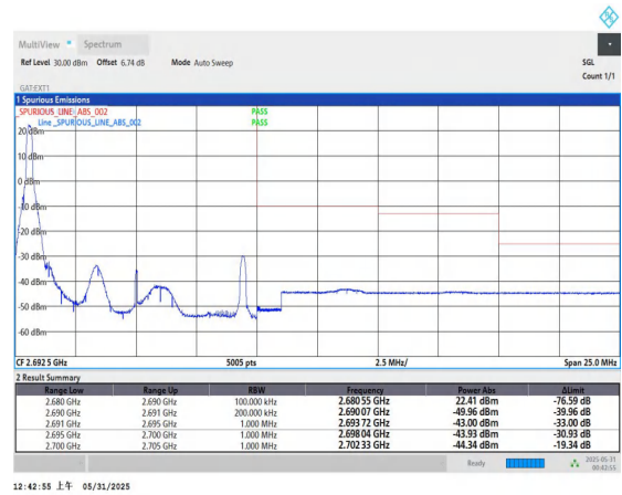
Band41-10MHz-QPSK-41540-1RB#0-PASS
