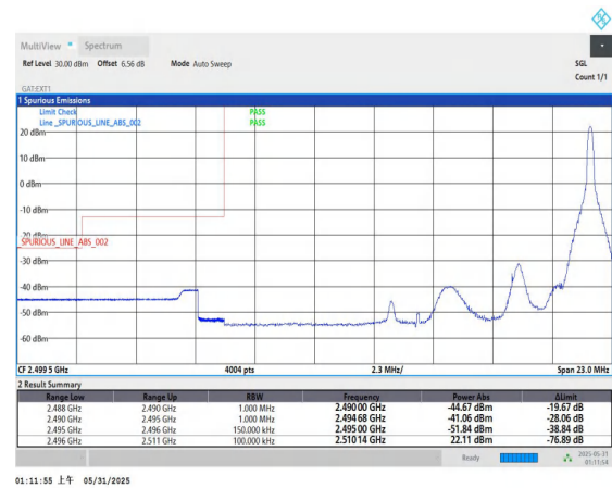
Band41-15MHz-QPSK-39725-1RB#74-PASS
