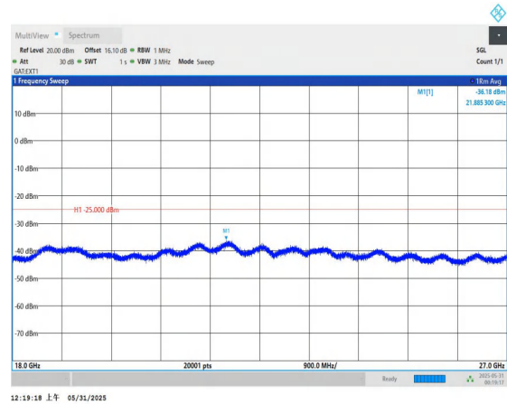
Band41-5MHz-QPSK-39675-1RB#0-18000~27000-PASS
