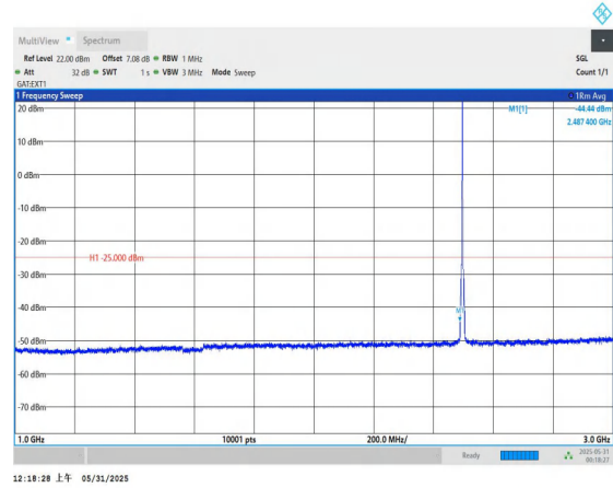
Band41-5MHz-QPSK-39675-1RB#0-1000~3000-PASS
