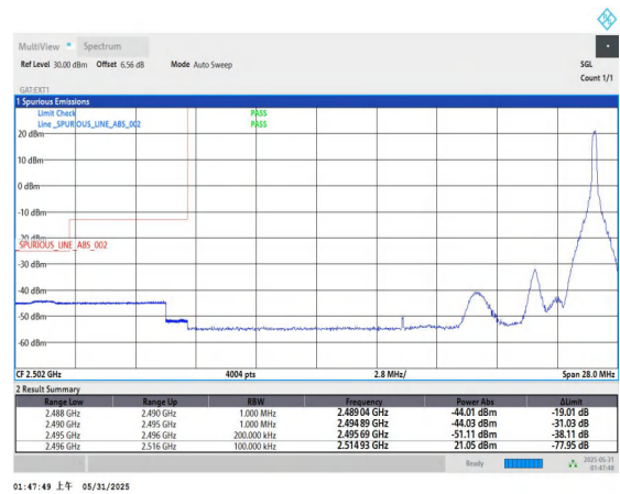
Band41-20MHz-16QAM-39750-1RB#99-PASS
