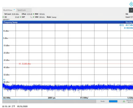
Band41-10MHz-QPSK-39700-1RB#0-30~1000-PASS
