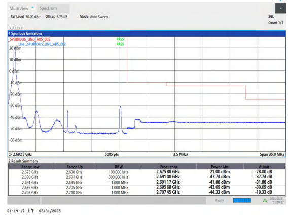
Band41-15MHz-16QAM-41515-1RB#0-PASS
