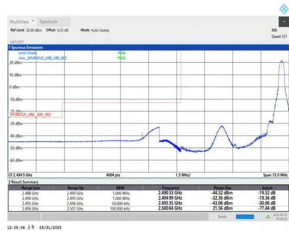
Band41-5MHz-16QAM-39675-1RB#24-PASS
