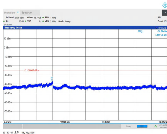
Band41-5MHz-16QAM-39675-1RB#0-3000~18000-PASS
