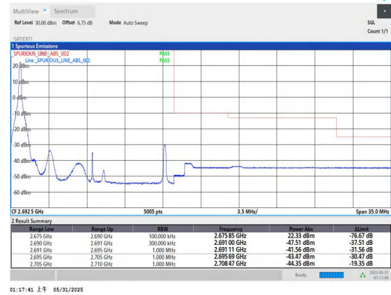
Band41-15MHz-QPSK-41515-1RB#0-PASS
