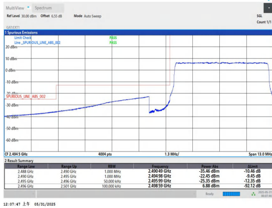
Band41-5MHz-16QAM-39675-25RB#0-PASS
