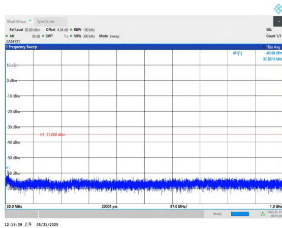
Band41-5MHz-16QAM-39675-1RB#0-30~1000-PASS
