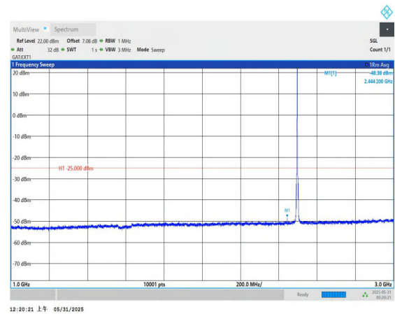
Band41-5MHz-16QAM-39675-1RB#0-1000~3000-PASS
