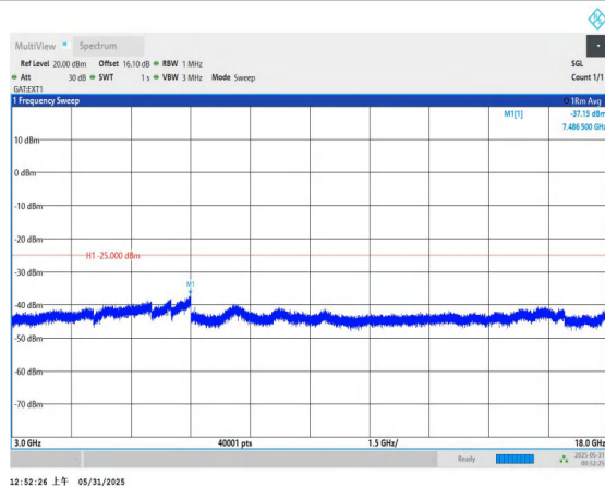
Band41-10MHz-QPSK-39700-1RB#0-3000~18000-PASS
