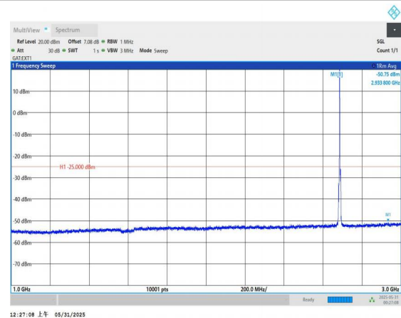
Band41-5MHz-16QAM-41565-1RB#0-1000~3000-PASS
