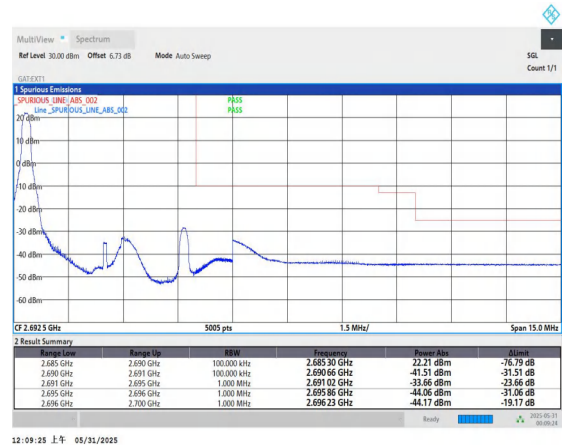
Band41-5MHz-QPSK-41565-1RB#0-PASS
