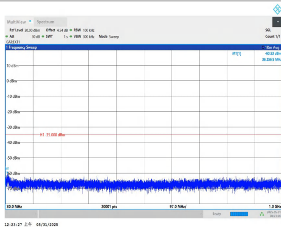
Band41-5MHz-16QAM-40620-1RB#0-30~1000-PASS
