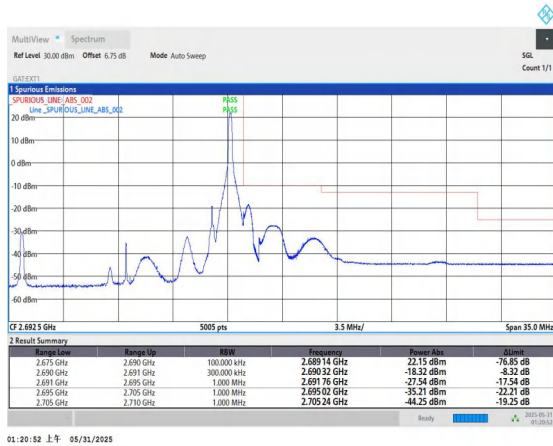
Band41-15MHz-QPSK-41515-1RB#74-PASS
