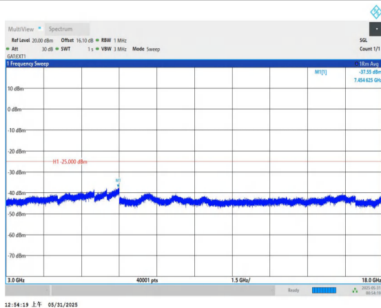
Band41-10MHz-16QAM-39700-1RB#0-3000~18000-PASS
