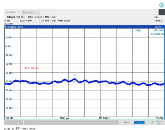
Band41-10MHz-QPSK-39700-1RB#0-18000~27000-PASS
