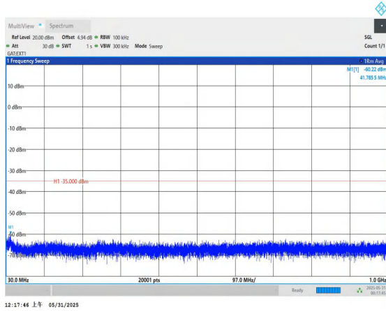
Band41-5MHz-QPSK-39675-1RB#0-30~1000-PASS
