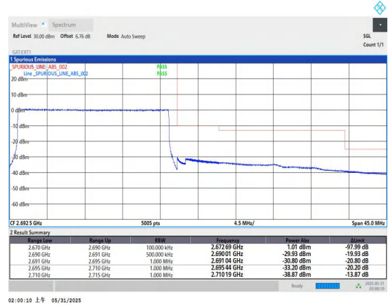
Band41-20MHz-16QAM-41490-100RB#0-PASS
