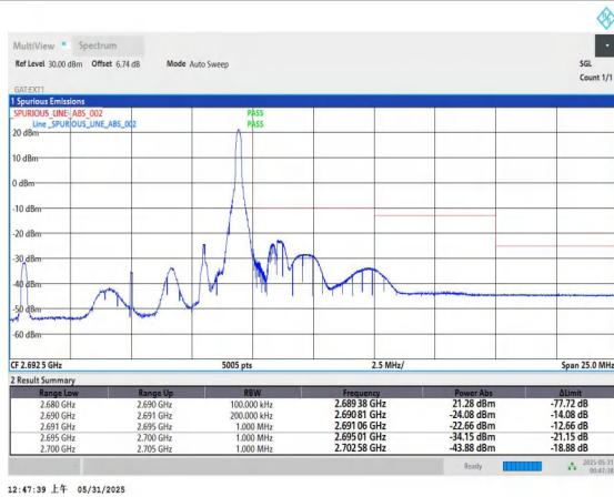
Band41-10MHz-16QAM-41540-1RB#49-PASS
