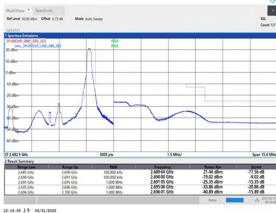
Band41-5MHz-16QAM-41565-1RB#24-PASS
