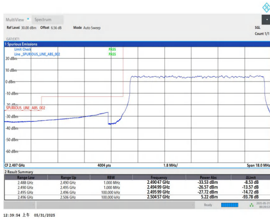
Band41-10MHz-QPSK-39700-50RB#0-PASS
