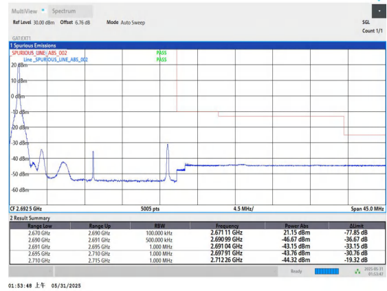
Band41-20MHz-16QAM-41490-1RB#0-PASS
