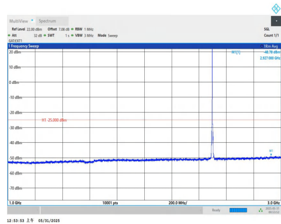
Band41-10MHz-16QAM-39700-1RB#0-1000~3000-PASS
