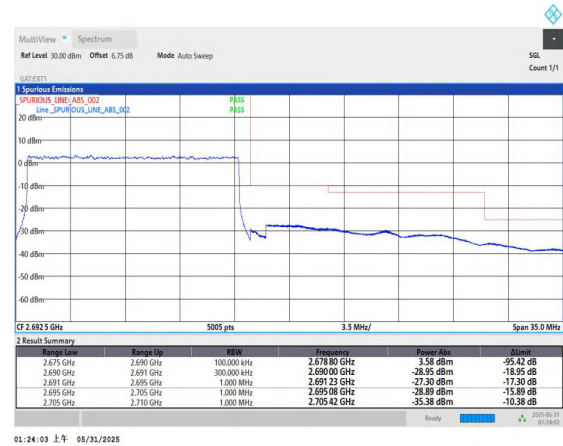
Band41-15MHz-QPSK-41515-75RB#0-PASS
