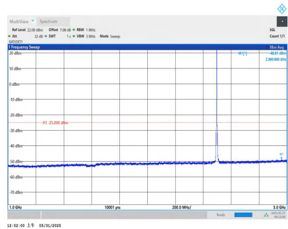
Band41-10MHz-QPSK-39700-1RB#0-1000~3000-PASS
