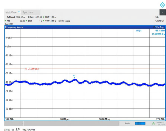
Band41-5MHz-16QAM-39675-1RB#0-18000~27000-PASS
