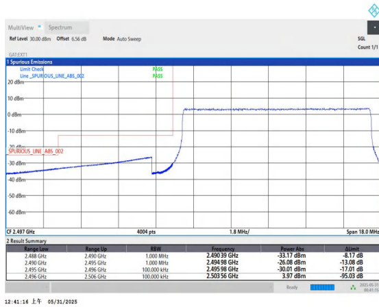
Band41-10MHz-16QAM-39700-50RB#0-PASS
