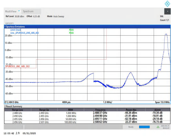
Band41-5MHz-QPSK-39675-1RB#24-PASS
