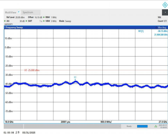
Band41-10MHz-QPSK-41540-1RB#0-18000~27000-PASS
