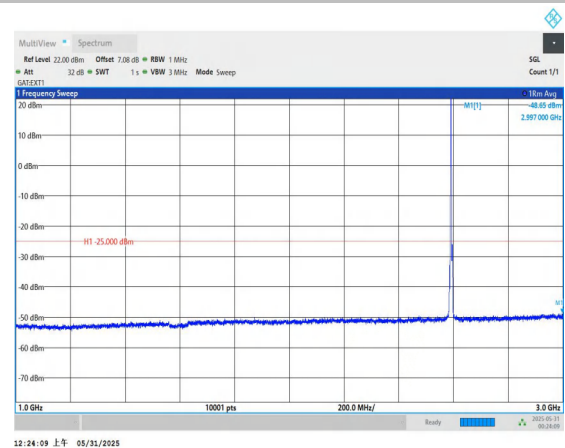
Band41-5MHz-16QAM-40620-1RB#0-1000~3000-PASS
