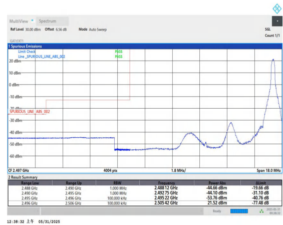
Band41-10MHz-16QAM-39700-1RB#49-PASS
