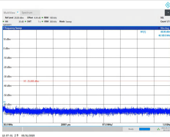
Band41-10MHz-16QAM-40620-1RB#0-30~1000-PASS
