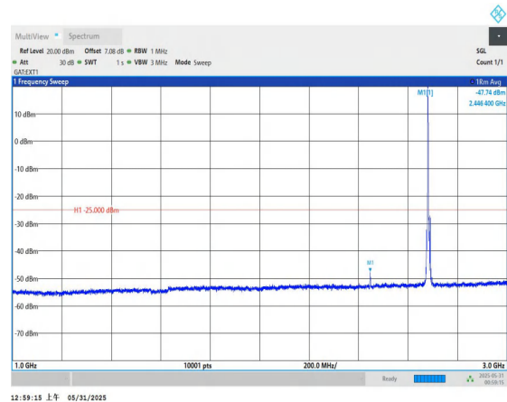
Band41-10MHz-QPSK-41540-1RB#0-1000~3000-PASS
