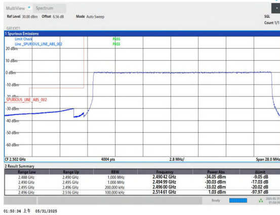
Band41-20MHz-16QAM-39750-100RB#0-PASS
