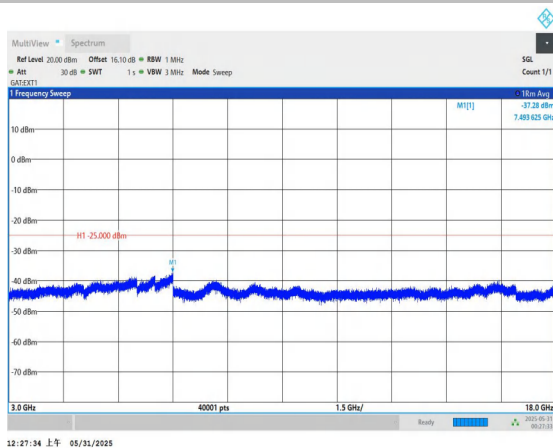
Band41-5MHz-16QAM-41565-1RB#0-3000~18000-PASS
