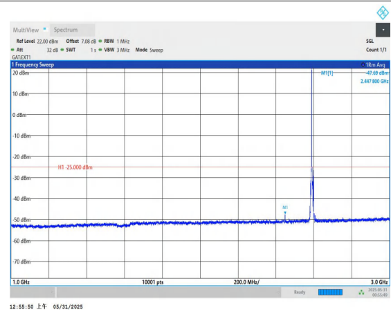
Band41-10MHz-QPSK-40620-1RB#0-1000~3000-PASS
