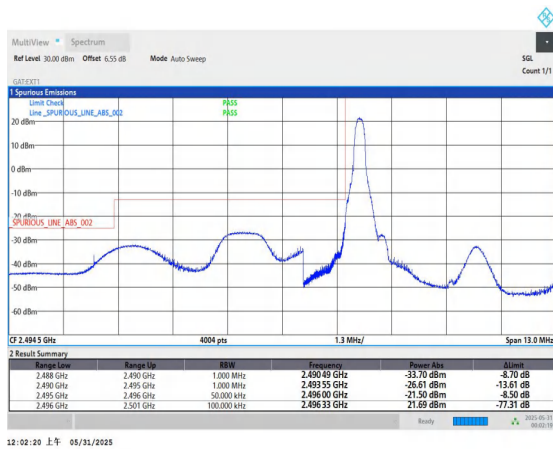
Band41-5MHz-16QAM-39675-1RB#0-PASS
