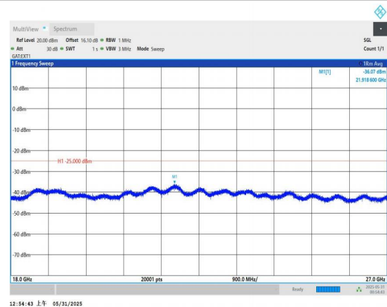
Band41-10MHz-16QAM-39700-1RB#0-18000~27000-PASS
