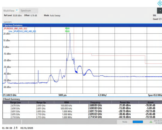
Band41-20MHz-16QAM-41490-1RB#99-PASS
