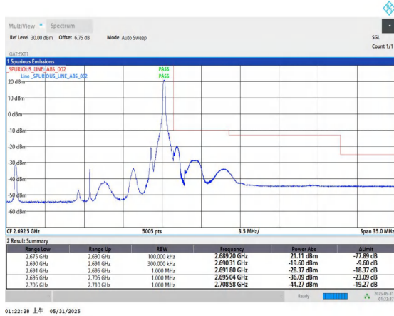
Band41-15MHz-16QAM-41515-1RB#74-PASS
