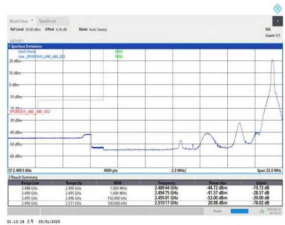
Band41-15MHz-16QAM-39725-1RB#74-PASS
