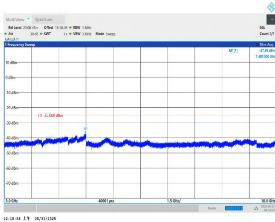
Band41-5MHz-QPSK-39675-1RB#0-3000~18000-PASS
