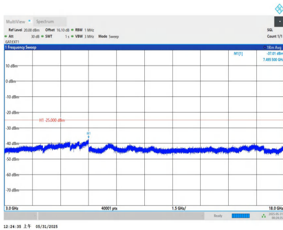
Band41-5MHz-16QAM-40620-1RB#0-3000~18000-PASS
