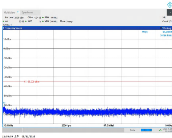
Band41-10MHz-QPSK-41540-1RB#0-30~1000-PASS
