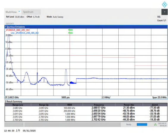
Band41-10MHz-16QAM-41540-1RB#0-PASS
