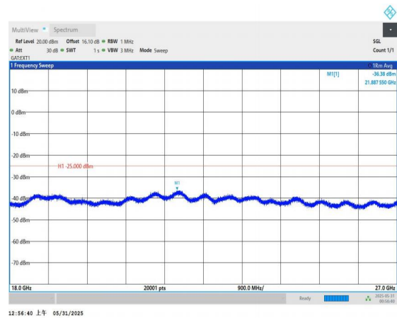
Band41-10MHz-QPSK-40620-1RB#0-18000~27000-PASS
