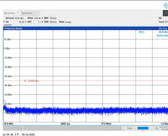
Band41-10MHz-QPSK-40620-1RB#0-30~1000-PASS
