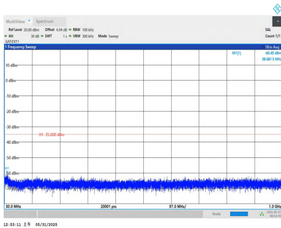
Band41-10MHz-16QAM-39700-1RB#0-30~1000-PASS
