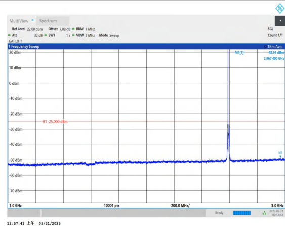
Band41-10MHz-16QAM-40620-1RB#0-1000~3000-PASS
