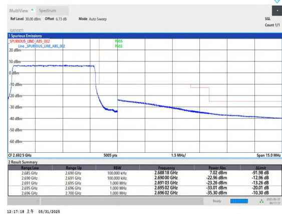
Band41-5MHz-16QAM-41565-25RB#0-PASS
