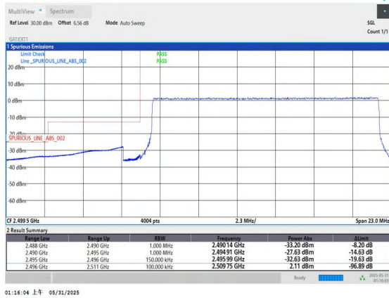
Band41-15MHz-16QAM-39725-75RB#0-PASS
