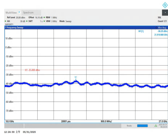
Band41-5MHz-16QAM-40620-1RB#0-18000~27000-PASS
