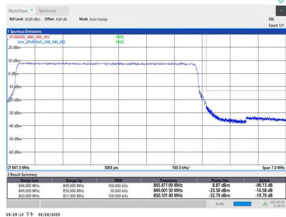
Band5-5MHz-QPSK-20625-25RB#0-PASS
