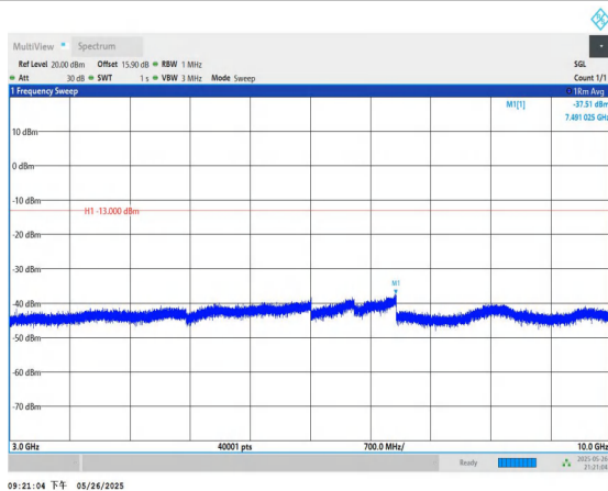
Band5-3MHz-QPSK-20525-1RB#0-3000~10000-PASS
