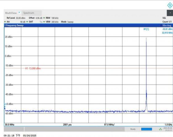
Band5-3MHz-QPSK-20635-1RB#0-30~1000-PASS
