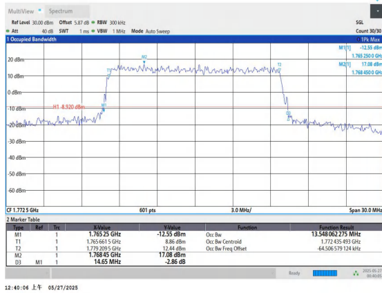
Band66-15MHz-QPSK-132597-75RB#0-PASS
