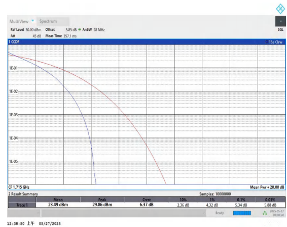
Band66-10MHz-QPSK-132022-50RB#0-PASS
