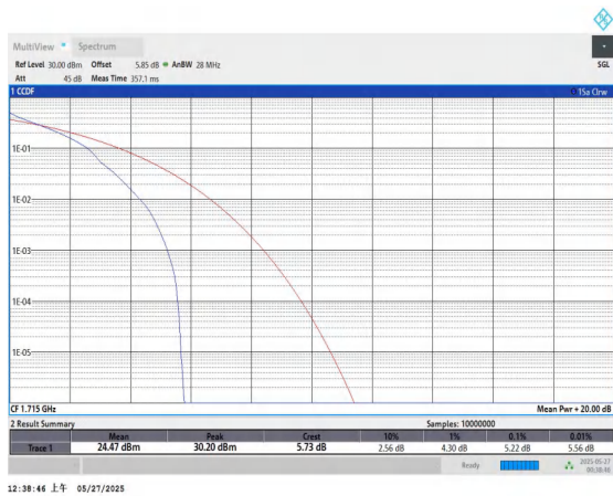
Band66-10MHz-QPSK-132022-1RB#0-PASS
