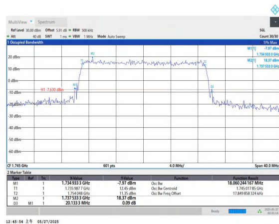
Band66-20MHz-QPSK-132322-100RB#0-PASS
