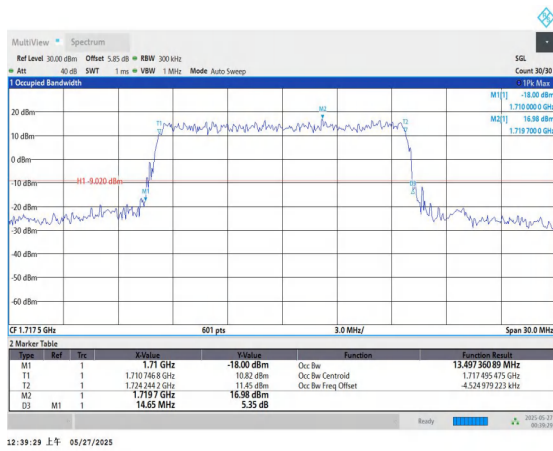
Band66-15MHz-QPSK-132047-75RB#0-PASS
