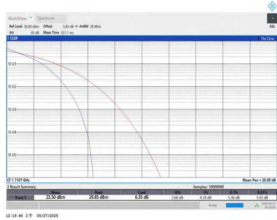
Band66-1.4MHz-QPSK-131979-6RB#0-PASS
