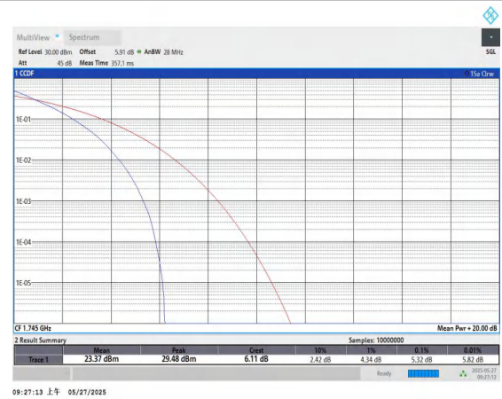
Band66-20MHz-QPSK-132322-100RB#0-PASS
