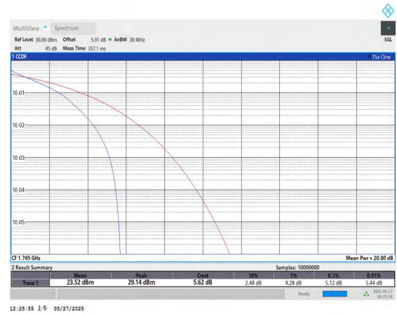
Band66-3MHz-QPSK-132322-15RB#0-PASS
