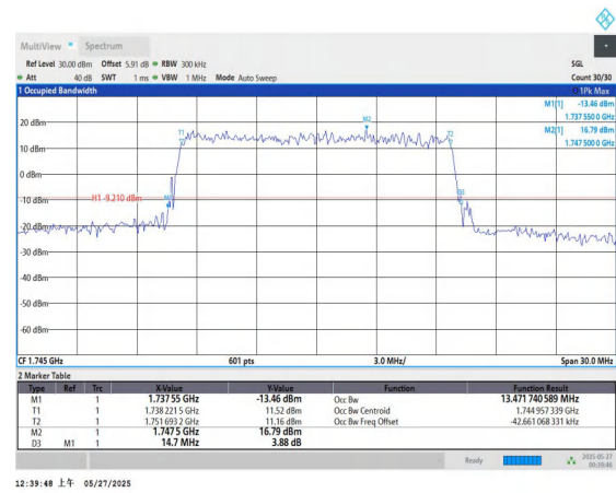
Band66-15MHz-QPSK-132322-75RB#0-PASS
