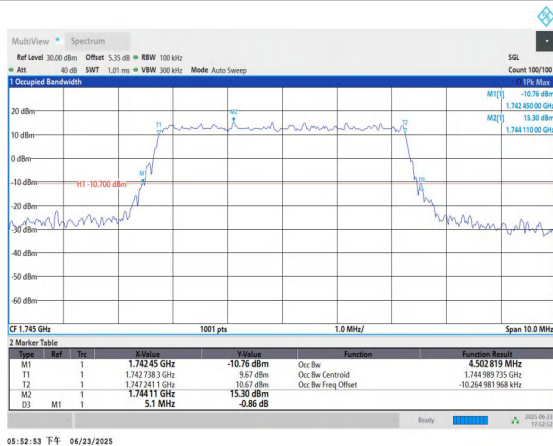
Band66-5MHz-16QAM-132322-25RB#0-PASS
