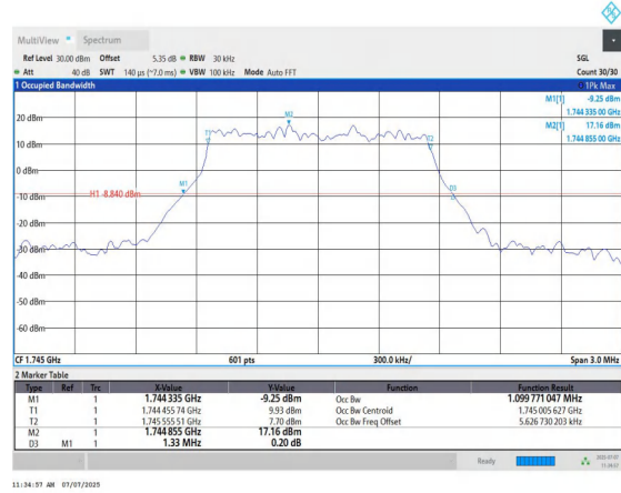
Band66-1.4MHz-QPSK-132322-6RB#0-PASS
