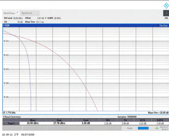
Band66-10MHz-QPSK-132622-1RB#0-PASS
