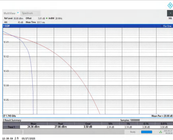
Band66-10MHz-QPSK-132322-1RB#0-PASS
