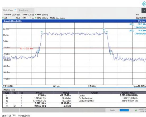
Band66-10MHz-16QAM-132322-50RB#0-PASS
