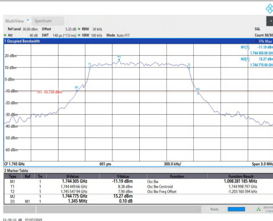
Band66-1.4MHz-16QAM-132322-6RB#0-PASS
