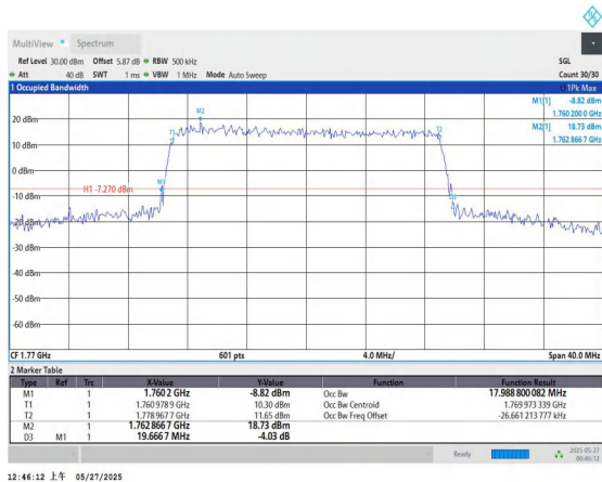
Band66-20MHz-QPSK-132572-100RB#0-PASS
