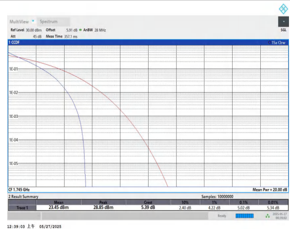
Band66-10MHz-QPSK-132322-50RB#0-PASS
