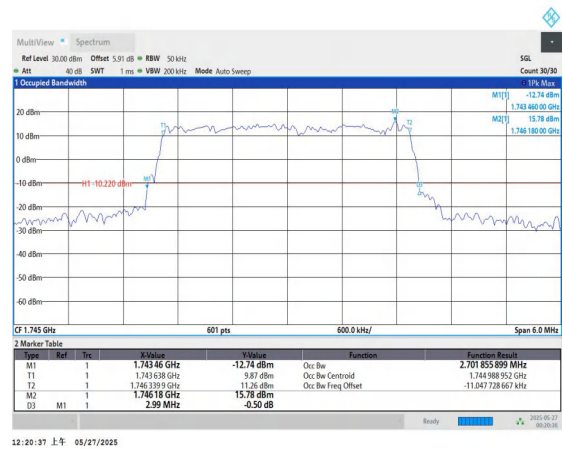
Band66-3MHz-QPSK-132322-15RB#0-PASS
