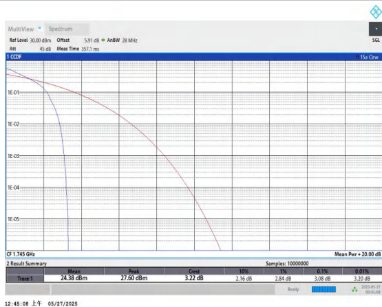
Band66-15MHz-QPSK-132322-1RB#0-PASS
