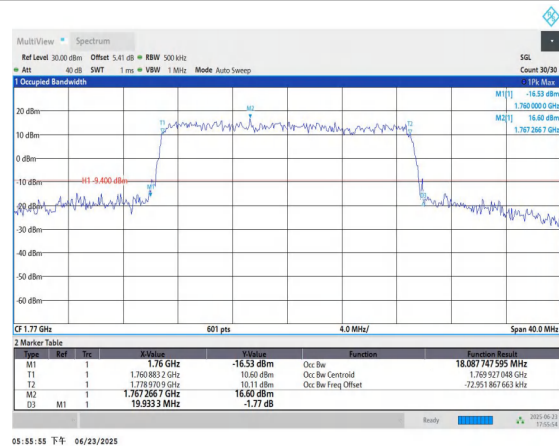
Band66-20MHz-16QAM-132572-100RB#0-PASS
