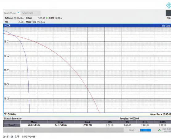
Band66-20MHz-QPSK-132322-1RB#0-PASS
