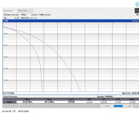
Band66-3MHz-QPSK-131987-1RB#0-PASS
