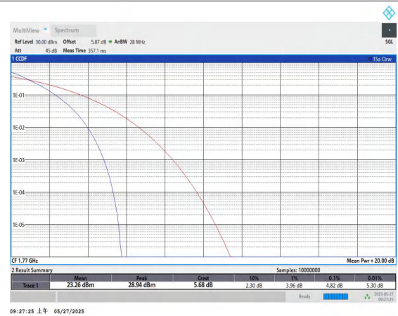
Band66-20MHz-QPSK-132572-100RB#0-PASS
