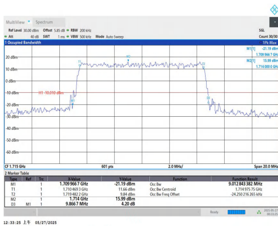
Band66-10MHz-QPSK-132022-50RB#0-PASS
