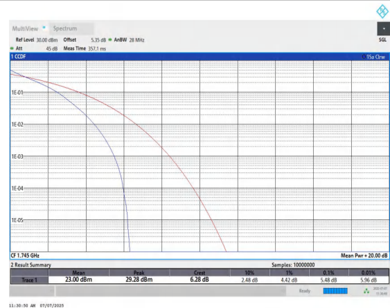
Band66-5MHz-QPSK-132322-25RB#0-PASS
