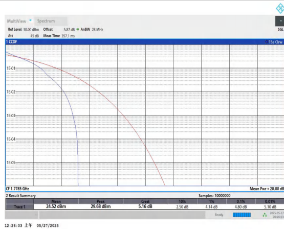
Band66-3MHz-QPSK-132657-1RB#0-PASS
