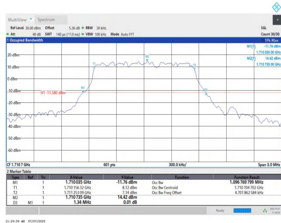
Band66-1.4MHz-16QAM-131979-6RB#0-PASS
