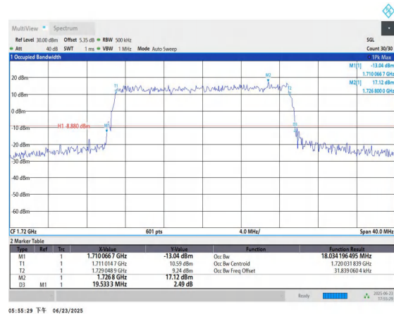
Band66-20MHz-16QAM-132072-100RB#0-PASS
