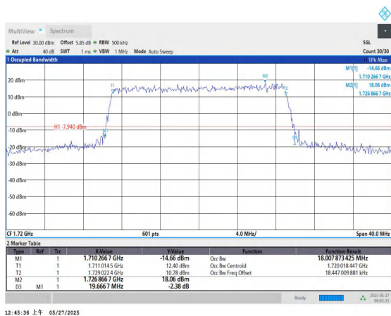
Band66-20MHz-QPSK-132072-100RB#0-PASS
