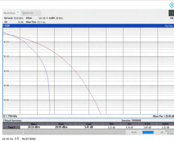
Band66-1.4MHz-QPSK-132665-1RB#0-PASS
