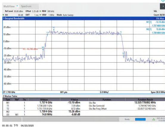
Band66-15MHz-16QAM-132322-75RB#0-PASS
