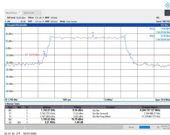
Band66-5MHz-QPSK-132322-25RB#0-PASS
