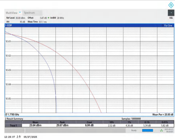
Band66-3MHz-QPSK-132657-15RB#0-PASS
