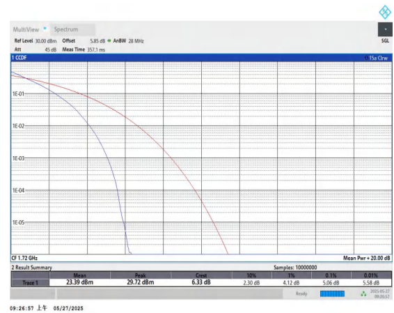
Band66-20MHz-QPSK-132072-100RB#0-PASS
