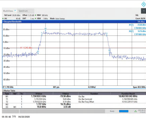
Band66-20MHz-16QAM-132322-100RB#0-PASS
