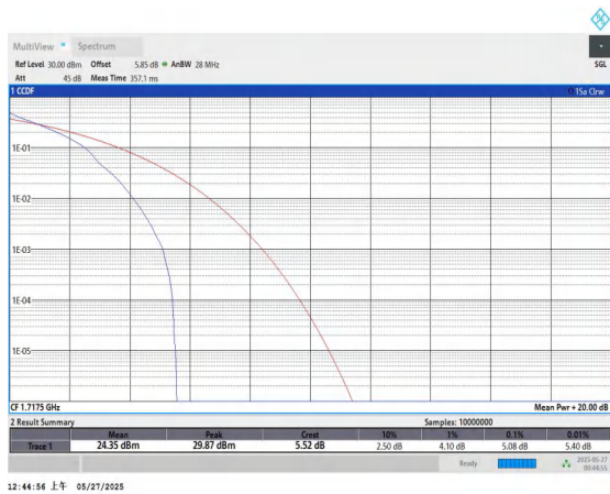
Band66-15MHz-QPSK-132047-1RB#0-PASS
