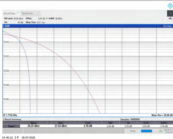
Band66-15MHz-QPSK-132597-1RB#0-PASS
