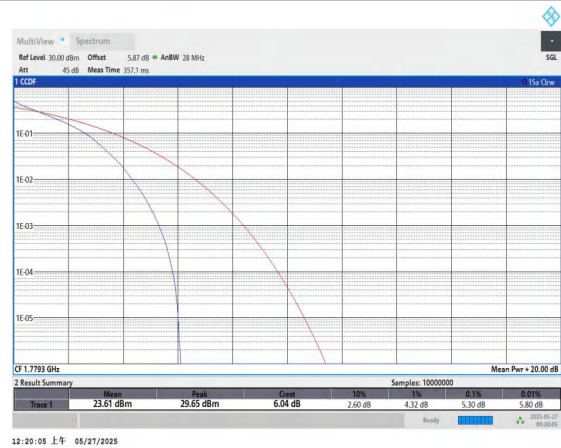
Band66-1.4MHz-QPSK-132665-6RB#0-PASS
