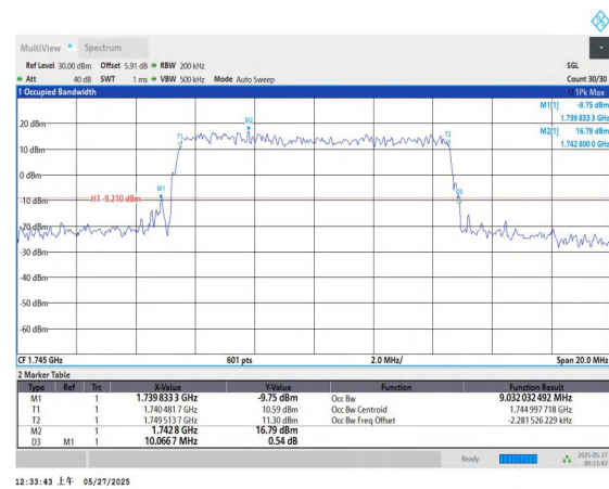
Band66-10MHz-QPSK-132322-50RB#0-PASS
