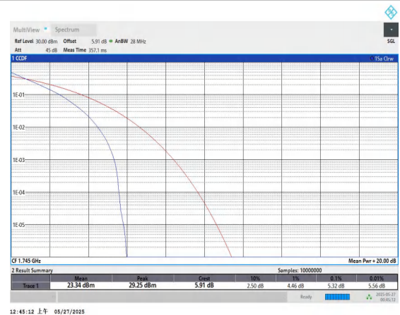
Band66-15MHz-QPSK-132322-75RB#0-PASS
