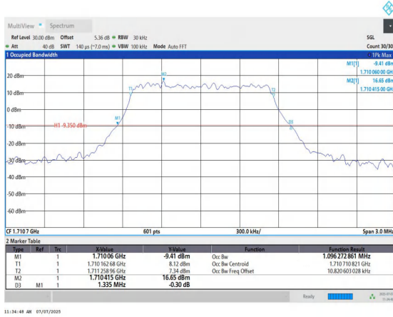
Band66-1.4MHz-QPSK-131979-6RB#0-PASS
