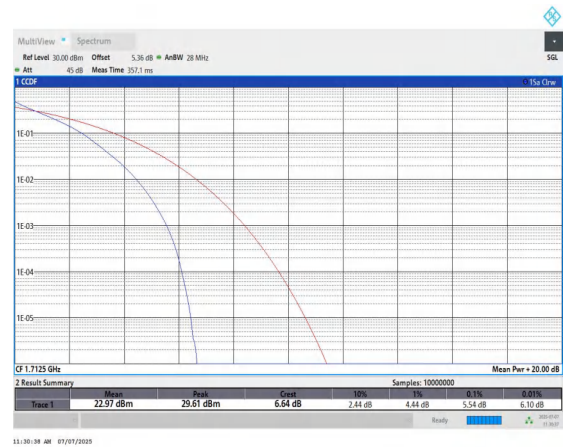
Band66-5MHz-QPSK-131997-25RB#0-PASS
