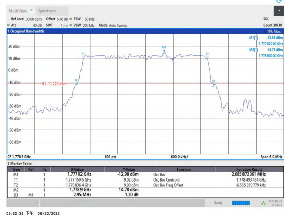
Band66-3MHz-16QAM-132657-15RB#0-PASS
