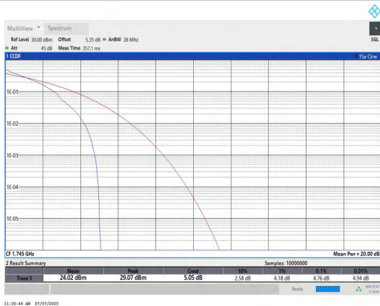
Band66-5MHz-QPSK-132322-1RB#0-PASS
