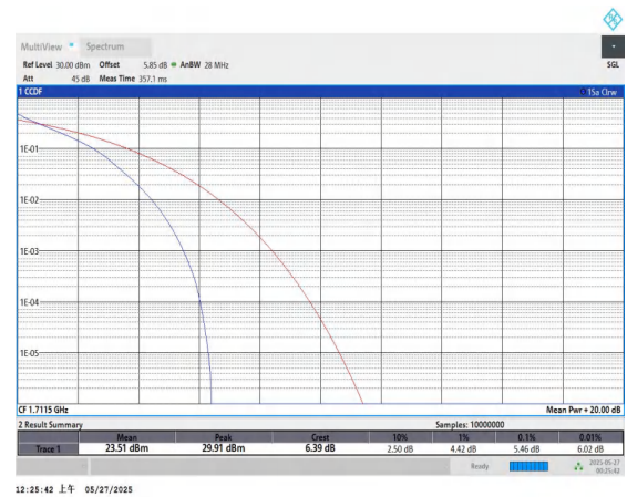
Band66-3MHz-QPSK-131987-15RB#0-PASS
