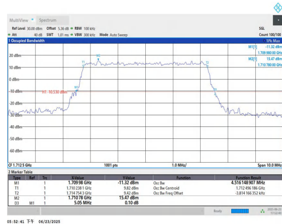
Band66-5MHz-16QAM-131997-25RB#0-PASS
