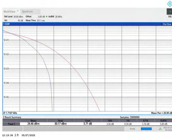
Band66-1.4MHz-QPSK-131979-1RB#0-PASS
