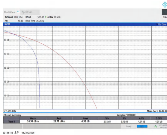
Band66-3MHz-QPSK-132322-1RB#0-PASS
