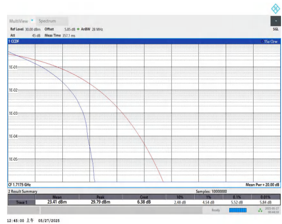
Band66-15MHz-QPSK-132047-75RB#0-PASS
