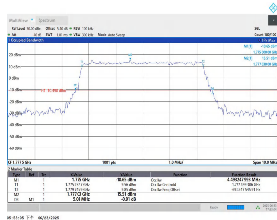
Band66-5MHz-16QAM-132647-25RB#0-PASS
