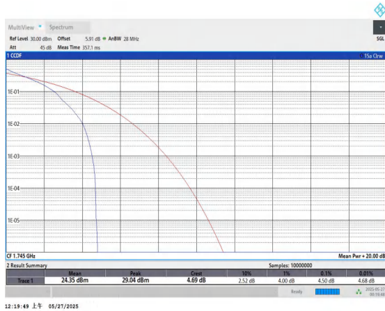
Band66-1.4MHz-QPSK-132322-1RB#0-PASS
