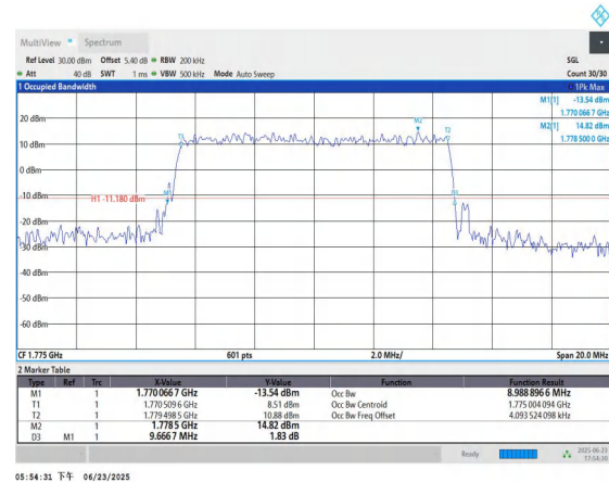
Band66-10MHz-16QAM-132622-50RB#0-PASS
