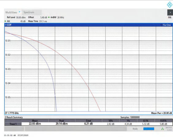
Band66-5MHz-QPSK-132647-25RB#0-PASS
