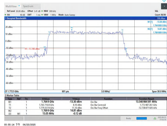
Band66-15MHz-16QAM-132597-75RB#0-PASS
