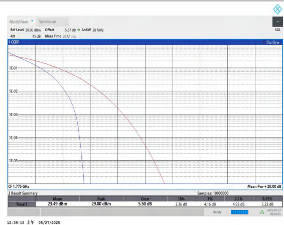
Band66-10MHz-QPSK-132622-50RB#0-PASS
