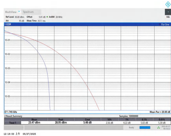
Band66-1.4MHz-QPSK-132322-6RB#0-PASS
