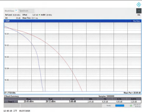
Band66-15MHz-QPSK-132597-75RB#0-PASS
