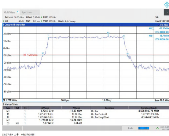
Band66-5MHz-QPSK-132647-25RB#0-PASS
