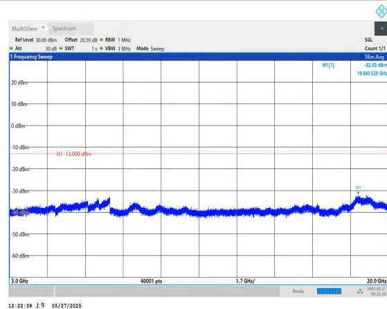
Band66-3MHz-QPSK-131987-1RB#0-3000~20000-PASS
