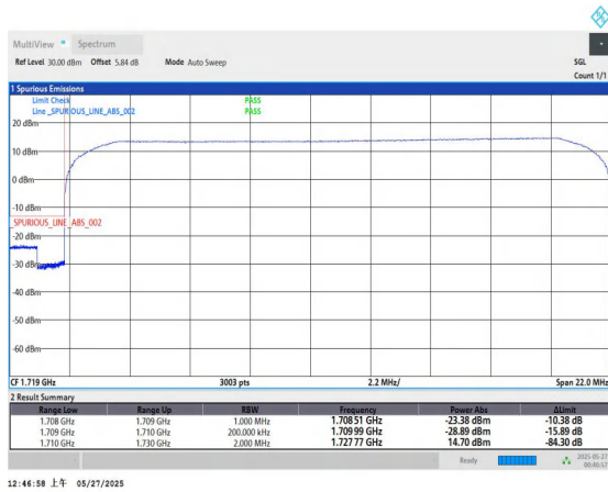
Band66-20MHz-QPSK-132072-100RB#0-PASS
