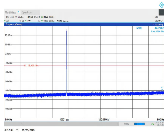
Band66-1.4MHz-QPSK-132665-1RB#0-1000~3000-PASS
