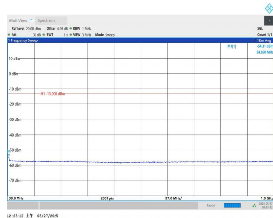
Band66-3MHz-QPSK-132657-1RB#0-30~1000-PASS
