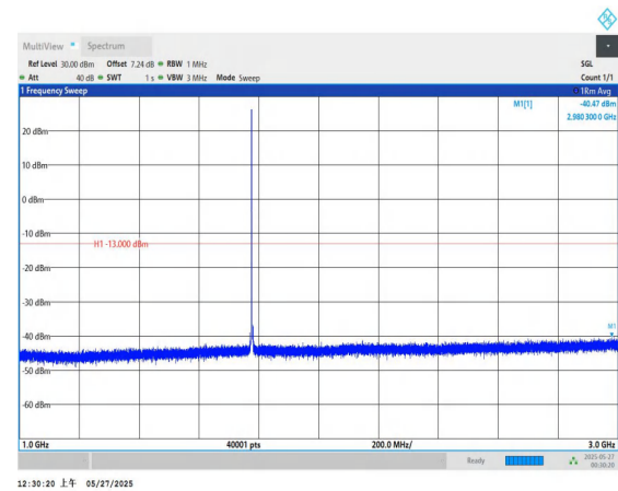
Band66-5MHz-QPSK-132647-1RB#0-1000~3000-PASS
