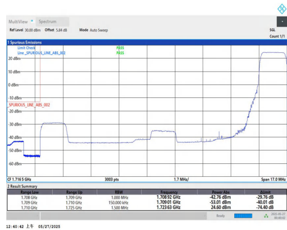
Band66-15MHz-QPSK-132047-1RB#74-PASS
