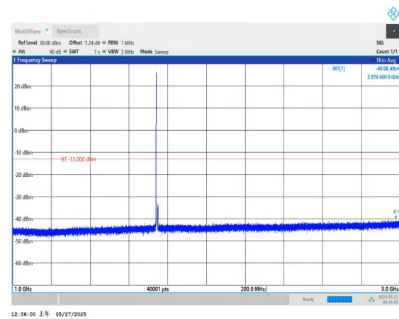
Band66-10MHz-QPSK-132322-1RB#0-1000~3000-PASS
