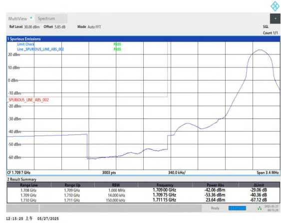
Band66-1.4MHz-QPSK-131979-1RB#5-PASS
