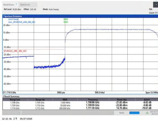
Band66-3MHz-QPSK-131987-15RB#0-PASS
