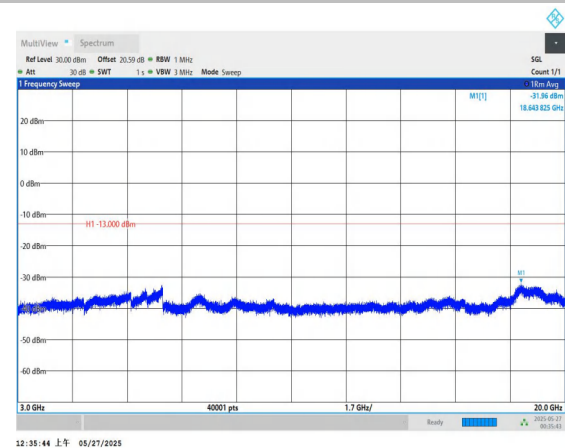
Band66-10MHz-QPSK-132022-1RB#0-3000~20000-PASS
