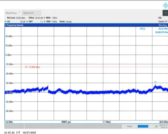
Band66-3MHz-QPSK-132657-1RB#0-3000~20000-PASS
