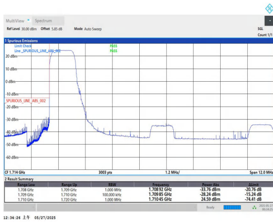
Band66-10MHz-QPSK-132022-1RB#0-PASS
