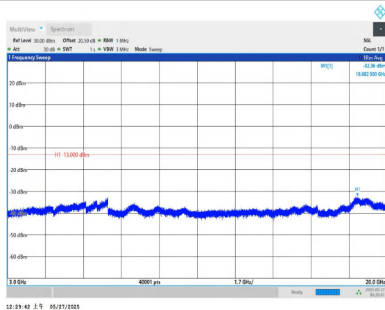
Band66-5MHz-QPSK-131997-1RB#0-3000~20000-PASS
