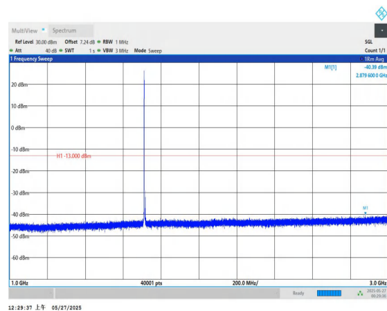
Band66-5MHz-QPSK-131997-1RB#0-1000~3000-PASS
