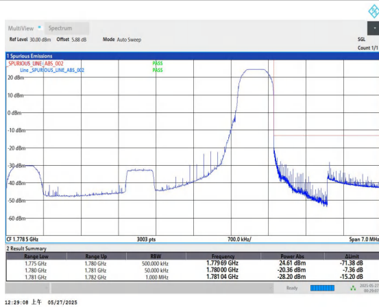
Band66-5MHz-QPSK-132647-1RB#24-PASS
