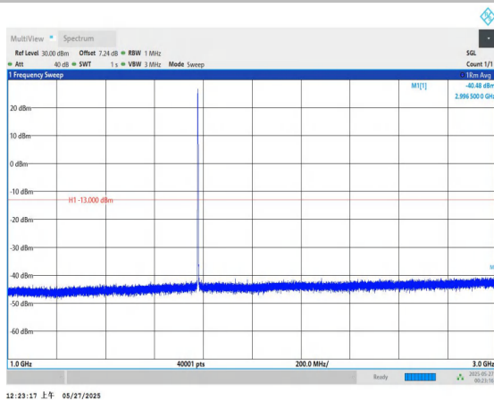
Band66-3MHz-QPSK-132657-1RB#0-1000~3000-PASS
