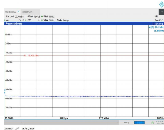
Band66-3MHz-QPSK-131987-1RB#0-30~1000-PASS
