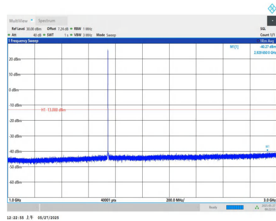
Band66-3MHz-QPSK-132322-1RB#0-1000~3000-PASS
