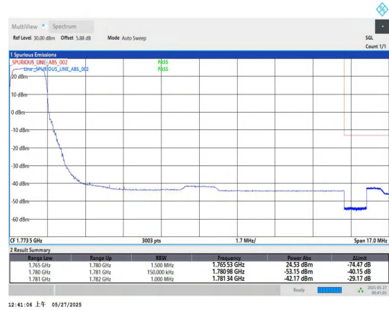
Band66-15MHz-QPSK-132597-1RB#0-PASS
