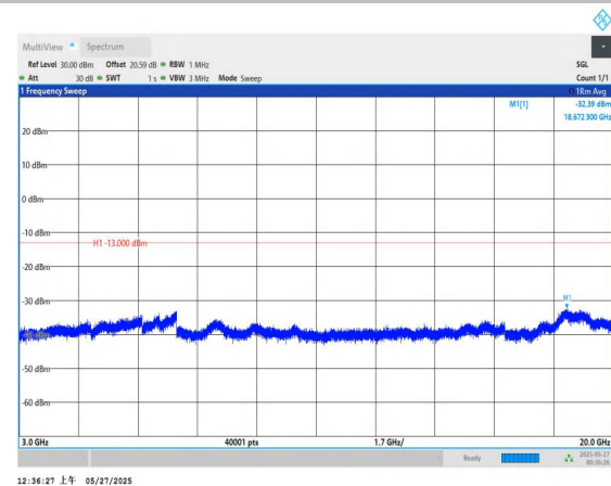
Band66-10MHz-QPSK-132622-1RB#0-3000~20000-PASS
