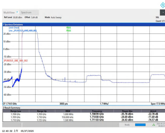
Band66-15MHz-QPSK-132047-1RB#0-PASS
