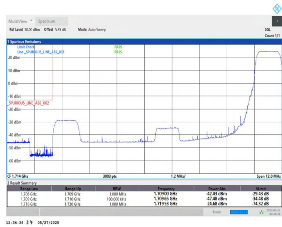
Band66-10MHz-QPSK-132022-1RB#49-PASS
