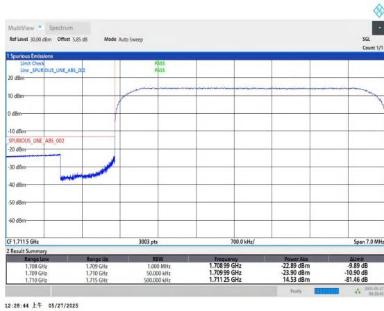
Band66-5MHz-QPSK-131997-25RB#0-PASS
