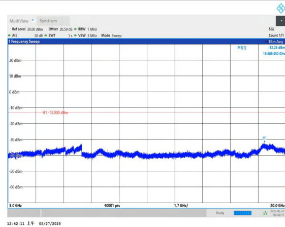
Band66-15MHz-QPSK-132322-1RB#0-3000~20000-PASS
