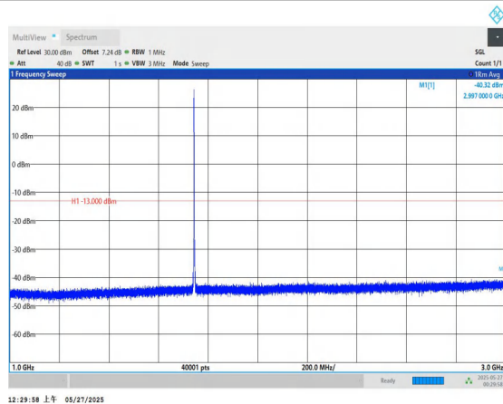
Band66-5MHz-QPSK-132322-1RB#0-1000~3000-PASS
