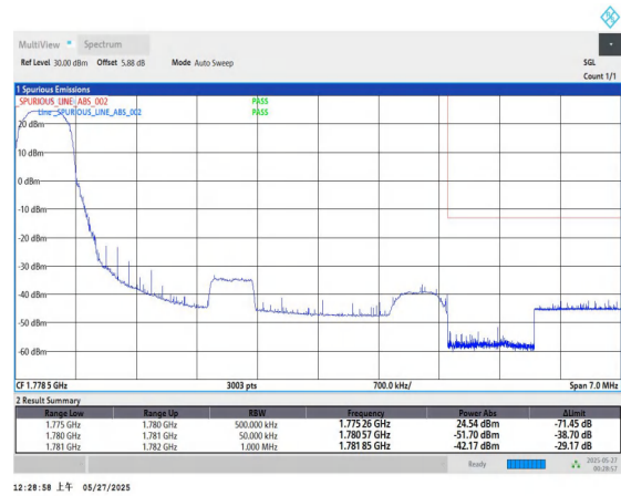
Band66-5MHz-QPSK-132647-1RB#0-PASS
