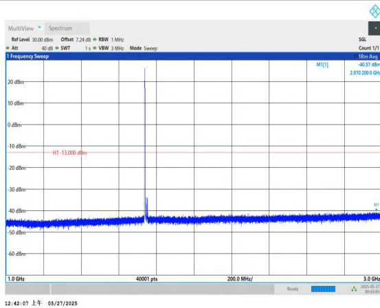
Band66-15MHz-QPSK-132322-1RB#0-1000~3000-PASS
