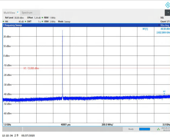
Band66-3MHz-QPSK-131987-1RB#0-1000~3000-PASS
