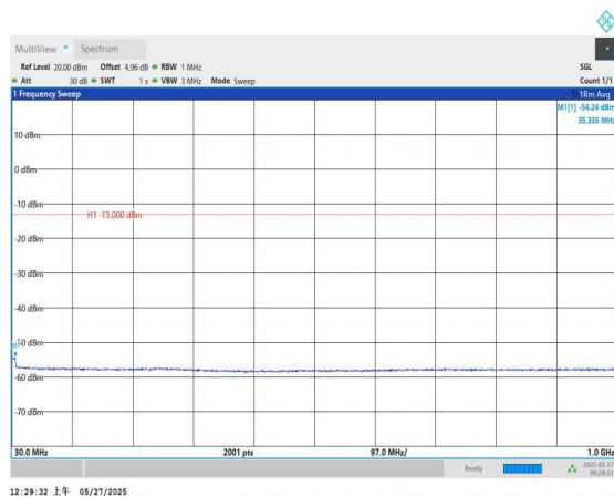
Band66-5MHz-QPSK-131997-1RB#0-30~1000-PASS
