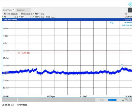
Band66-3MHz-QPSK-132322-1RB#0-3000~20000-PASS
