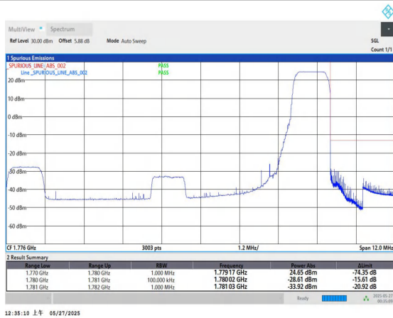
Band66-10MHz-QPSK-132622-1RB#49-PASS
