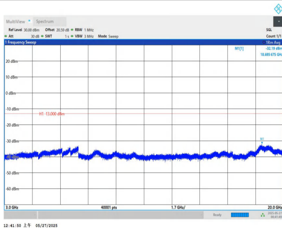
Band66-15MHz-QPSK-132047-1RB#0-3000~20000-PASS
