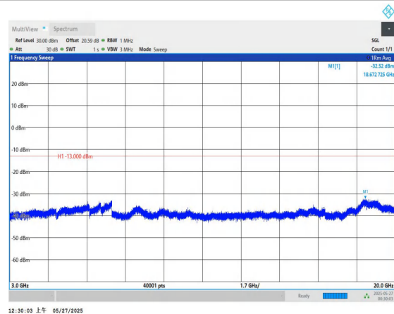
Band66-5MHz-QPSK-132322-1RB#0-3000~20000-PASS
