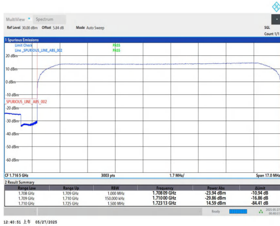
Band66-15MHz-QPSK-132047-75RB#0-PASS
