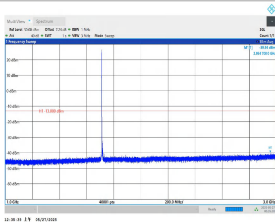
Band66-10MHz-QPSK-132022-1RB#0-1000~3000-PASS
