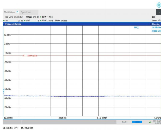
Band66-5MHz-QPSK-132647-1RB#0-30~1000-PASS
