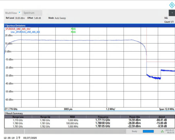
Band66-10MHz-QPSK-132622-50RB#0-PASS
