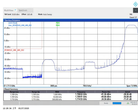
Band66-5MHz-QPSK-131997-1RB#24-PASS
