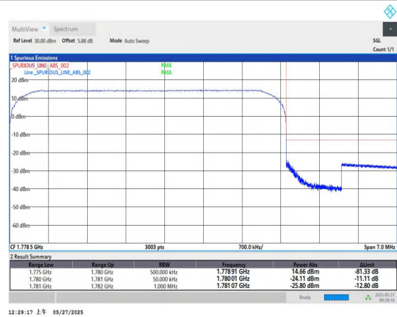
Band66-5MHz-QPSK-132647-25RB#0-PASS
