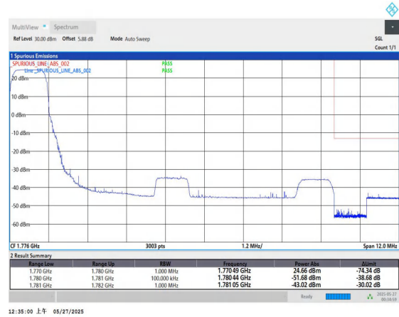
Band66-10MHz-QPSK-132622-1RB#0-PASS
