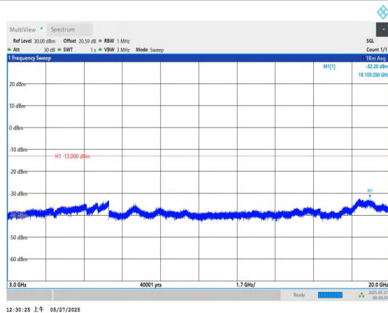
Band66-5MHz-QPSK-132647-1RB#0-3000~20000-PASS
