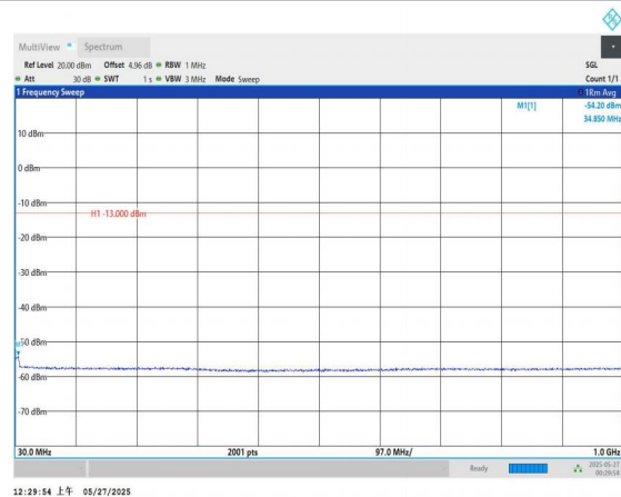
Band66-5MHz-QPSK-132322-1RB#0-30~1000-PASS
