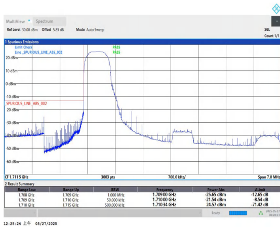
Band66-5MHz-QPSK-131997-1RB#0-PASS
