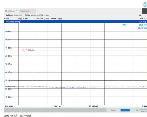
Band66-15MHz-QPSK-132322-1RB#0-30~1000-PASS
