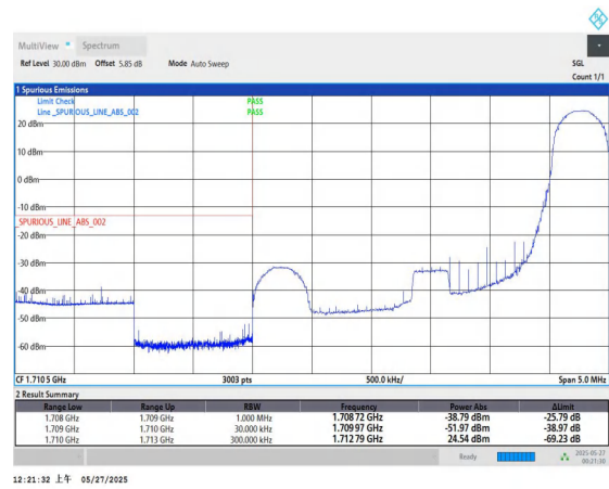
Band66-3MHz-QPSK-131987-1RB#14-PASS
