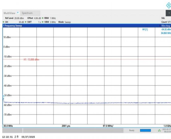
Band66-3MHz-QPSK-132322-1RB#0-30~1000-PASS
