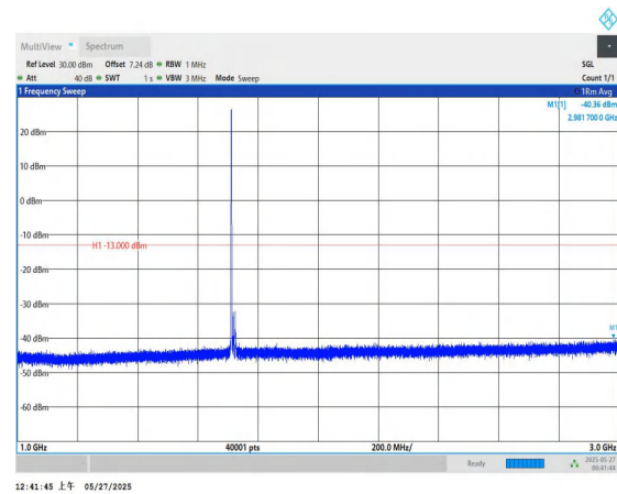
Band66-15MHz-QPSK-132047-1RB#0-1000~3000-PASS
