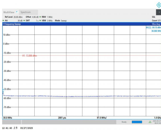
Band66-15MHz-QPSK-132047-1RB#0-30~1000-PASS
