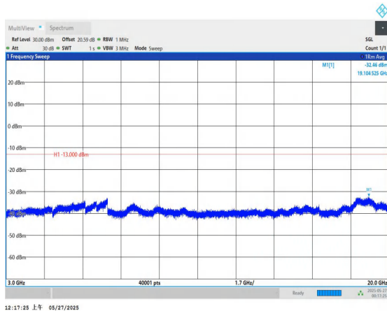
Band66-1.4MHz-QPSK-132665-1RB#0-3000~20000-PASS
