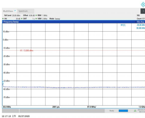
Band66-1.4MHz-QPSK-132665-1RB#0-30~1000-PASS
