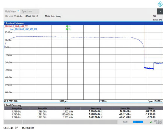
Band66-15MHz-QPSK-132597-75RB#0-PASS
