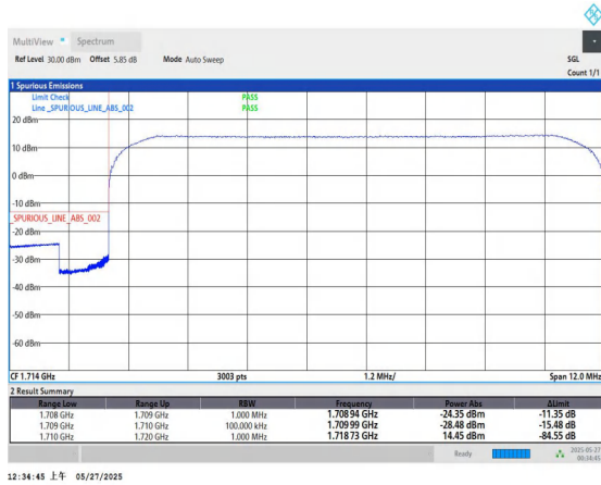
Band66-10MHz-QPSK-132022-50RB#0-PASS
