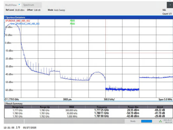
Band66-3MHz-QPSK-132657-1RB#0-PASS
