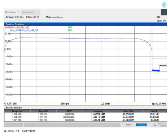
Band66-20MHz-QPSK-132572-100RB#0-PASS
