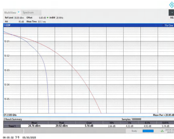
Band7-10MHz-QPSK-21100-1RB#0-PASS
