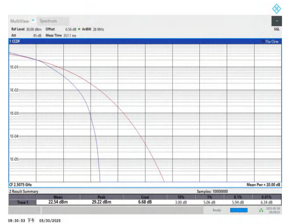
Band7-15MHz-16QAM-20825-75RB#0-PASS
