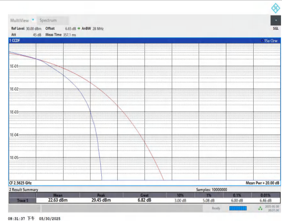
Band7-15MHz-16QAM-21375-75RB#0-PASS
