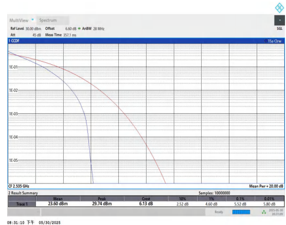
Band7-15MHz-QPSK-21100-75RB#0-PASS
