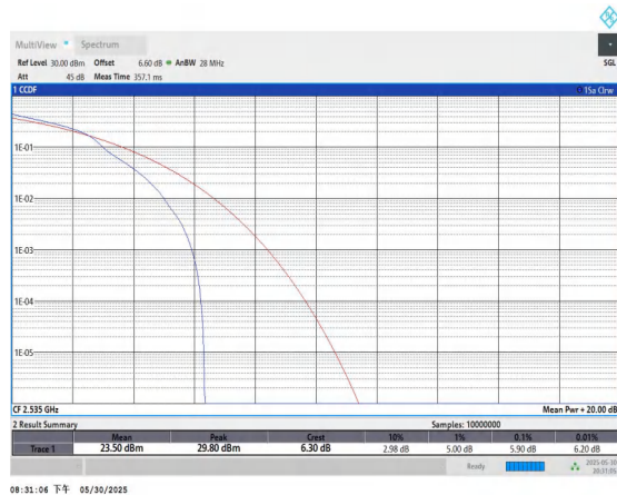
Band7-15MHz-16QAM-21100-1RB#0-PASS
