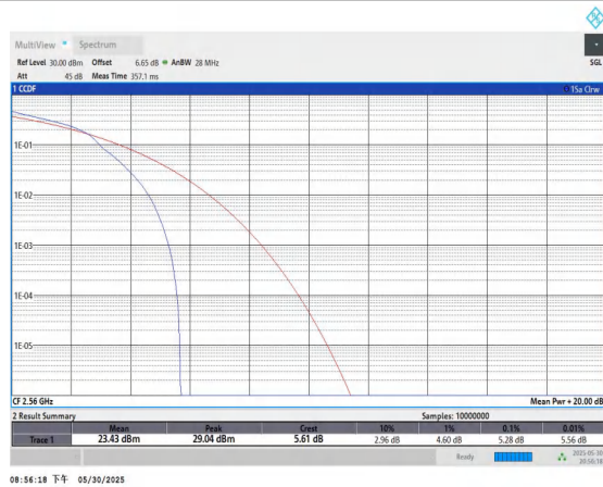
Band7-20MHz-16QAM-21350-1RB#0-PASS
