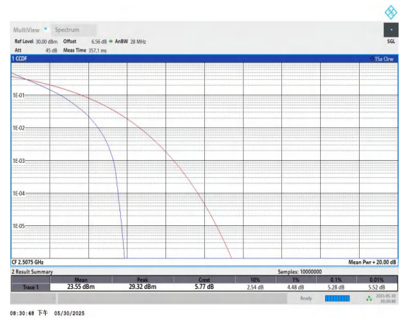
Band7-15MHz-QPSK-20825-75RB#0-PASS
