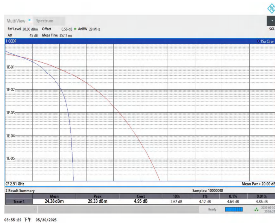
Band7-20MHz-QPSK-20850-1RB#0-PASS
