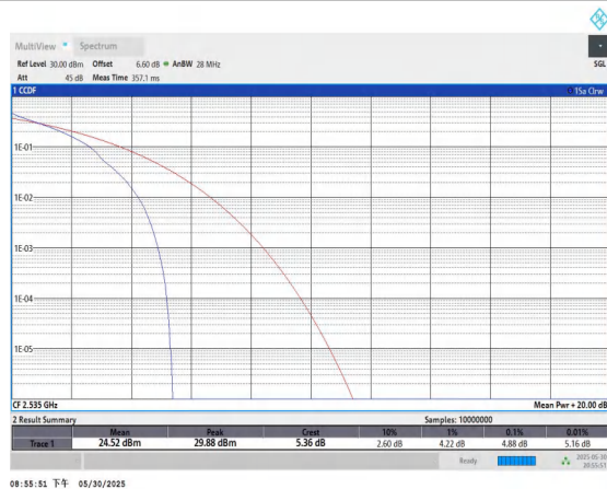
Band7-20MHz-QPSK-21100-1RB#0-PASS
