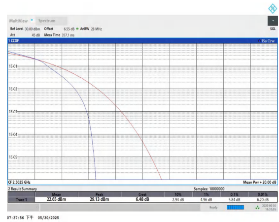
Band7-5MHz-16QAM-20775-25RB#0-PASS
