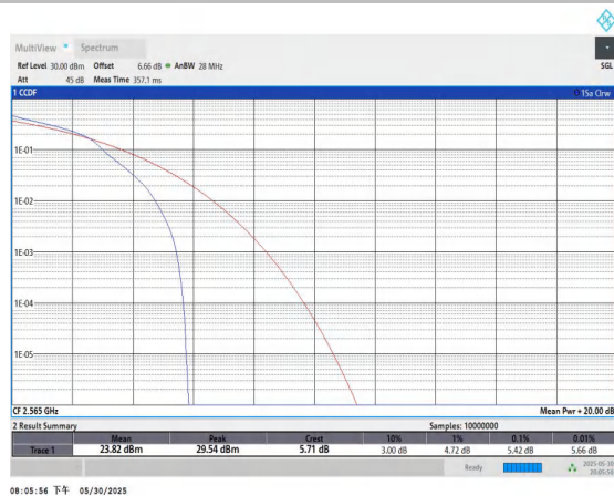
Band7-10MHz-16QAM-21400-1RB#0-PASS
