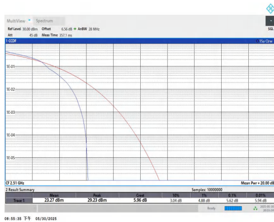
Band7-20MHz-16QAM-20850-1RB#0-PASS
