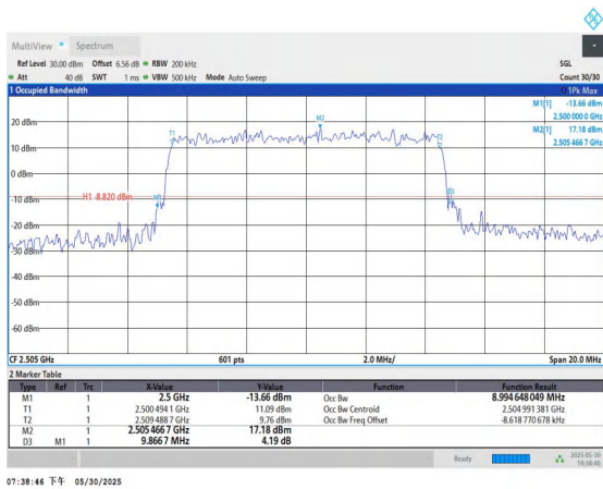
Band7-10MHz-QPSK-20800-50RB#0-PASS
