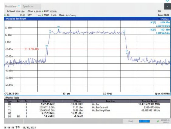
Band7-15MHz-16QAM-21375-75RB#0-PASS
