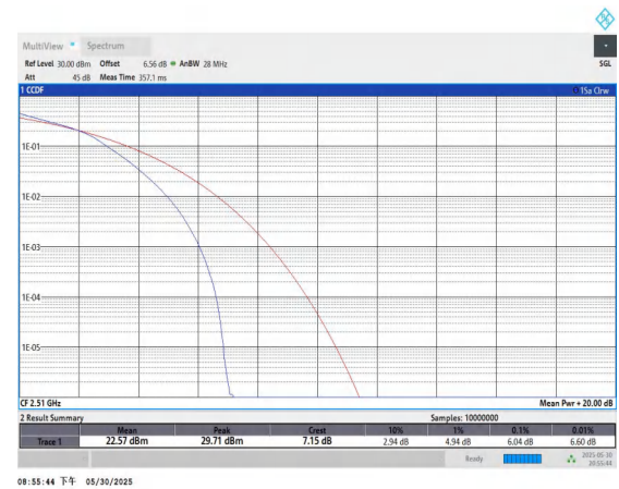
Band7-20MHz-16QAM-20850-100RB#0-PASS
