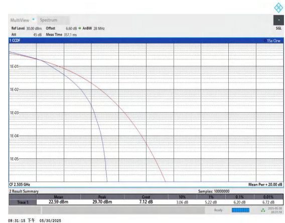
Band7-15MHz-16QAM-21100-75RB#0-PASS
