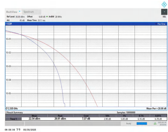
Band7-20MHz-16QAM-21100-100RB#0-PASS
