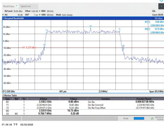
Band7-10MHz-16QAM-21100-50RB#0-PASS
