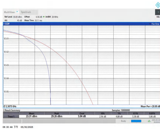
Band7-15MHz-16QAM-20825-1RB#0-PASS
