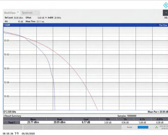
Band7-10MHz-16QAM-21100-1RB#0-PASS
