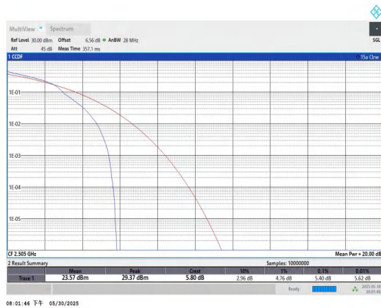
Band7-10MHz-16QAM-20800-1RB#0-PASS
