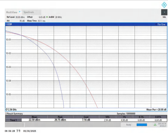
Band7-20MHz-16QAM-21350-100RB#0-PASS
