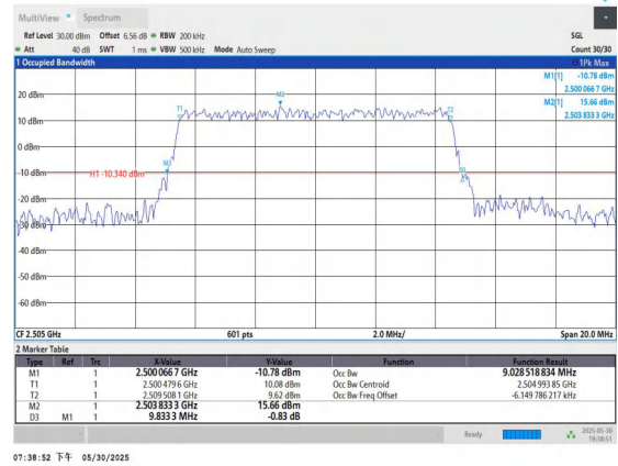
Band7-10MHz-16QAM-20800-50RB#0-PASS
