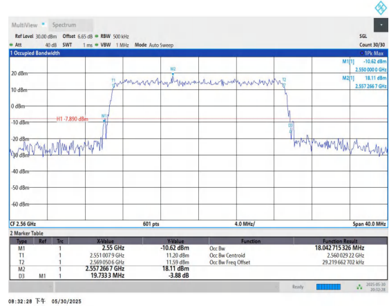
Band7-20MHz-16QAM-21350-100RB#0-PASS
