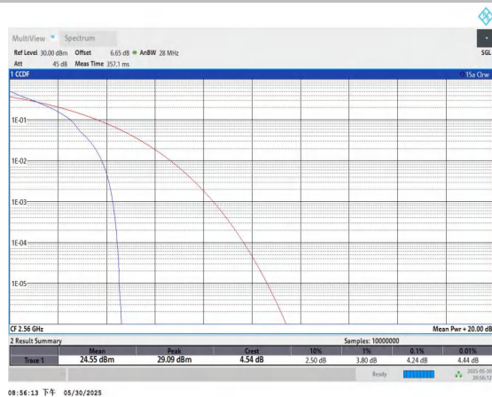
Band7-20MHz-QPSK-21350-1RB#0-PASS
