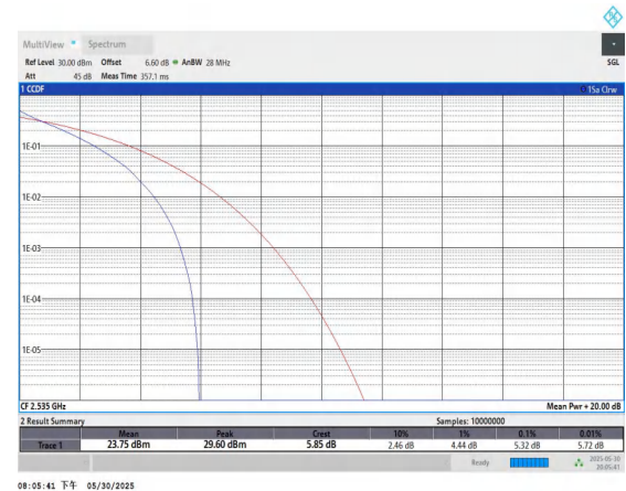
Band7-10MHz-QPSK-21100-50RB#0-PASS
