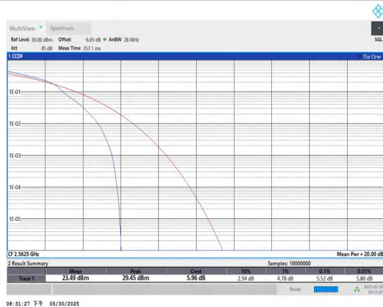
Band7-15MHz-16QAM-21375-1RB#0-PASS
