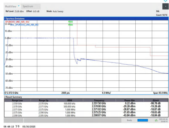
Band7-20MHz-16QAM-21350-100RB#0-PASS
