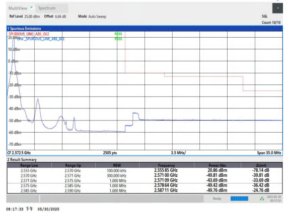
Band7-15MHz-16QAM-21375-1RB#0-PASS
