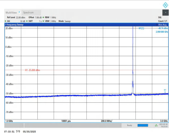
Band7-5MHz-QPSK-21425-1RB#0-1000~3000-PASS
