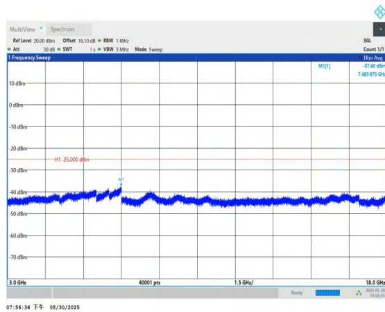
Band7-10MHz-QPSK-21100-1RB#0-3000~18000-PASS
