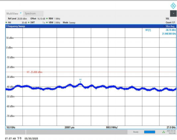
Band7-10MHz-QPSK-21400-1RB#0-18000~27000-PASS
