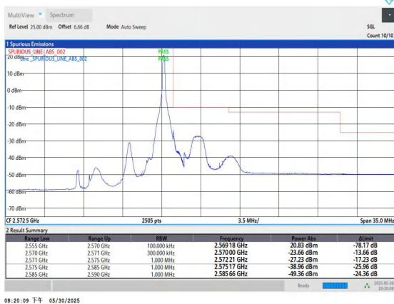
Band7-15MHz-16QAM-21375-1RB#74-PASS
