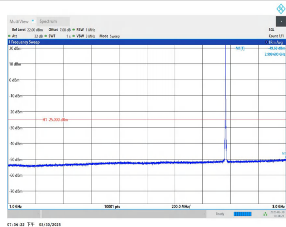
Band7-5MHz-16QAM-21425-1RB#0-1000~3000-PASS
