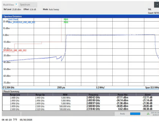
Band7-20MHz-16QAM-20850-100RB#0-PASS
