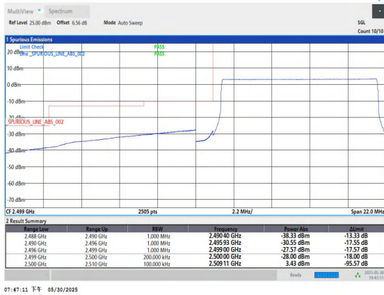
Band7-10MHz-16QAM-20800-50RB#0-PASS
