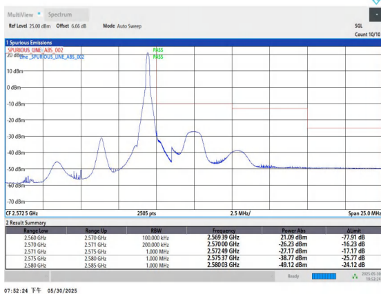
Band7-10MHz-16QAM-21400-1RB#49-PASS
