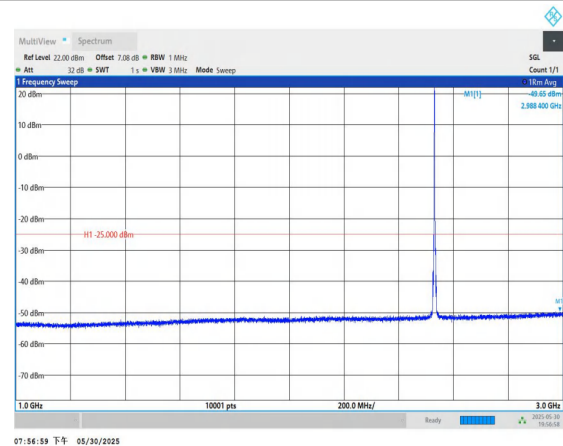
Band7-10MHz-16QAM-21100-1RB#0-1000~3000-PASS
