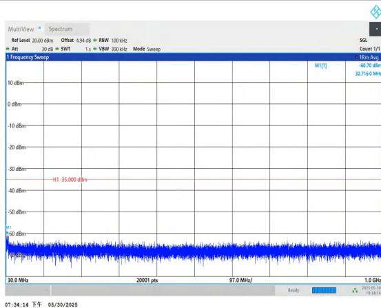
Band7-5MHz-16QAM-21425-1RB#0-30~1000-PASS
