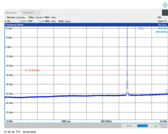
Band7-10MHz-16QAM-20800-1RB#0-1000~3000-PASS
