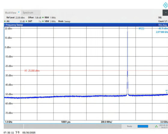
Band7-5MHz-16QAM-20775-1RB#0-1000~3000-PASS
