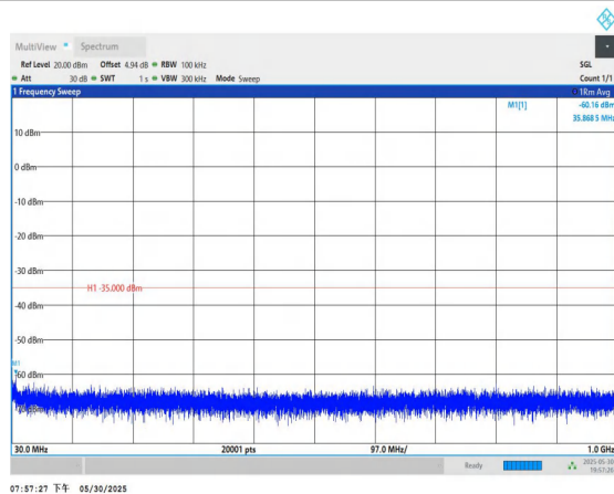
Band7-10MHz-QPSK-21400-1RB#0-30~1000-PASS
