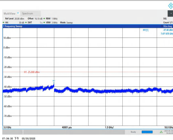
Band7-5MHz-16QAM-21425-1RB#0-3000~18000-PASS
