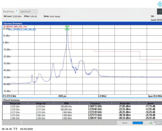
Band7-15MHz-QPSK-21375-1RB#74-PASS
