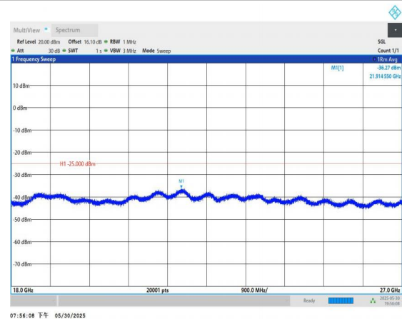
Band7-10MHz-16QAM-20800-1RB#0-18000~27000-PASS
