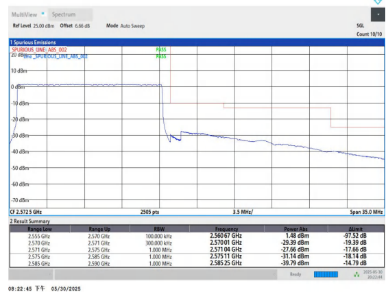
Band7-15MHz-16QAM-21375-75RB#0-PASS
