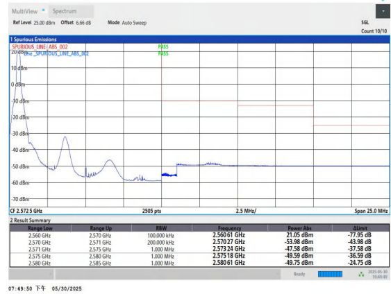
Band7-10MHz-16QAM-21400-1RB#0-PASS
