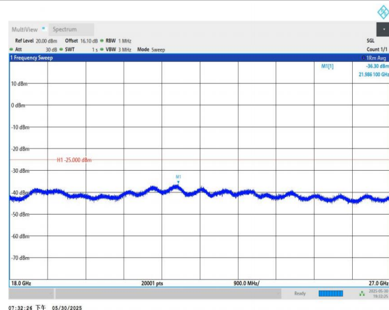
Band7-5MHz-16QAM-20775-1RB#0-18000~27000-PASS
