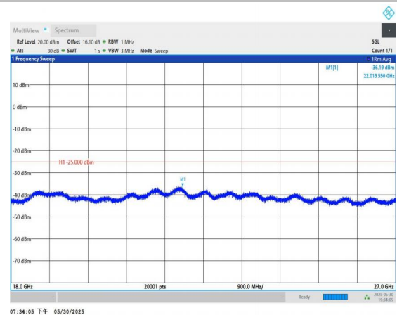
Band7-5MHz-QPSK-21425-1RB#0-18000~27000-PASS
