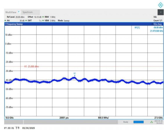
Band7-5MHz-QPSK-21100-1RB#0-18000~27000-PASS
