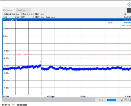
Band7-10MHz-QPSK-21400-1RB#0-3000~18000-PASS
