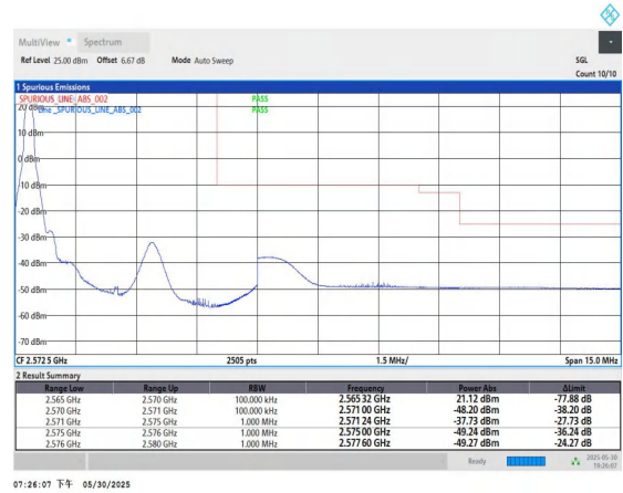
Band7-5MHz-16QAM-21425-1RB#0-PASS
