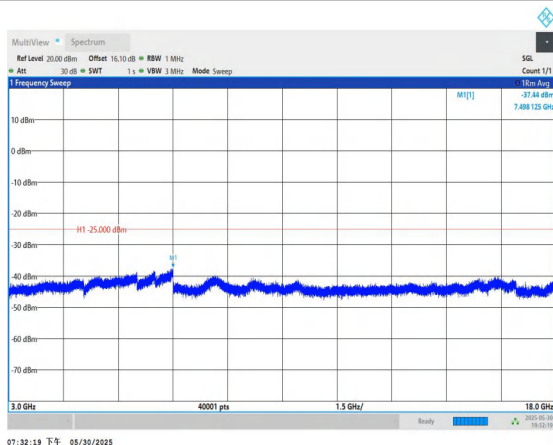
Band7-5MHz-16QAM-20775-1RB#0-3000~18000-PASS
