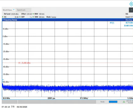
Band7-5MHz-16QAM-21100-1RB#0-30~1000-PASS
