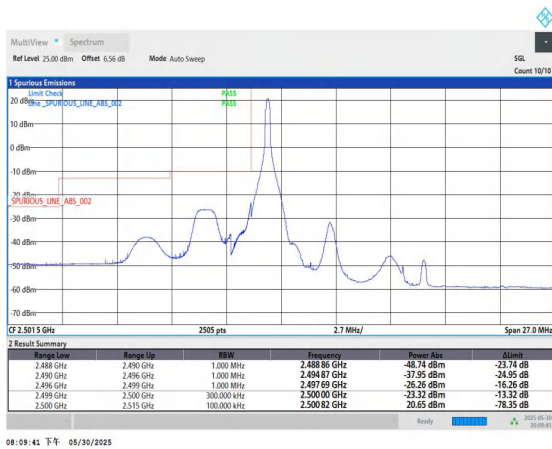
Band7-15MHz-16QAM-20825-1RB#0-PASS
