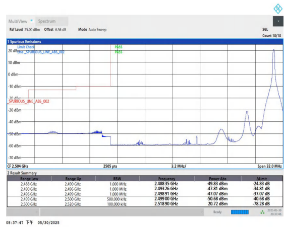
Band7-20MHz-16QAM-20850-1RB#99-PASS
