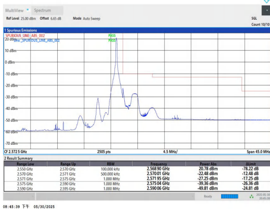
Band7-20MHz-16QAM-21350-1RB#99-PASS
