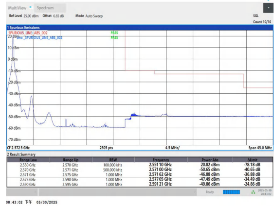
Band7-20MHz-16QAM-21350-1RB#0-PASS
