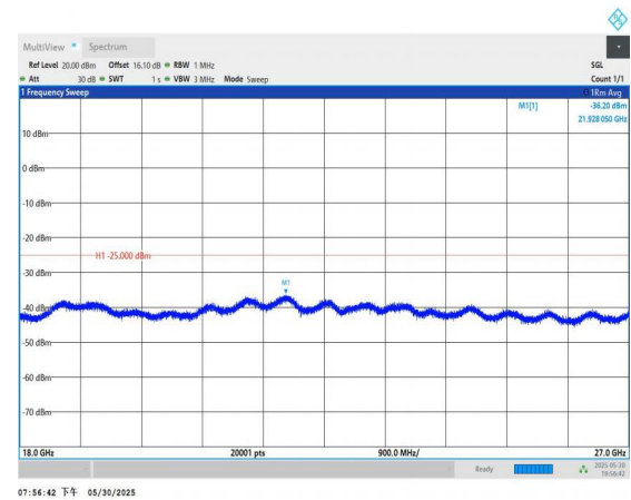
Band7-10MHz-QPSK-21100-1RB#0-18000~27000-PASS
