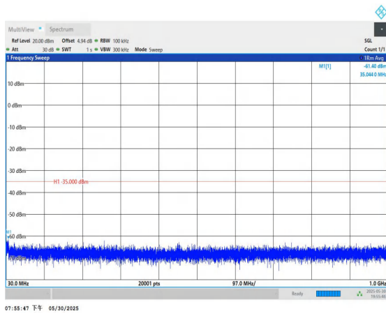
Band7-10MHz-16QAM-20800-1RB#0-30~1000-PASS
