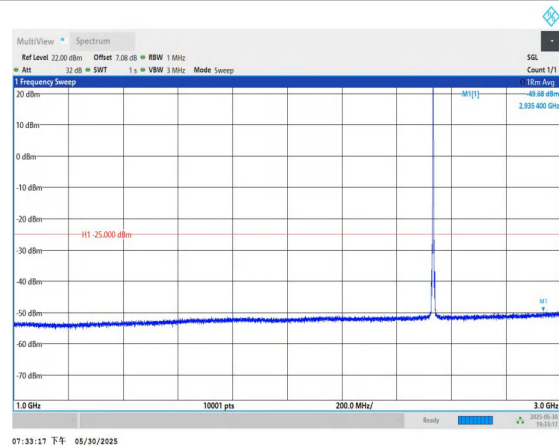
Band7-5MHz-16QAM-21100-1RB#0-1000~3000-PASS
