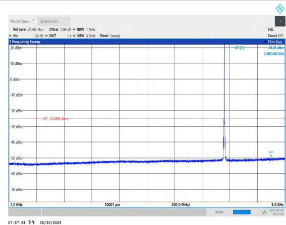
Band7-10MHz-QPSK-21400-1RB#0-1000~3000-PASS
