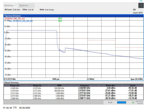
Band7-10MHz-16QAM-21400-50RB#0-PASS
