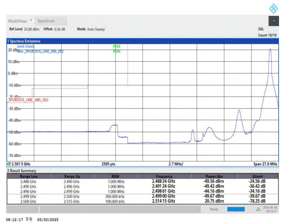
Band7-15MHz-16QAM-20825-1RB#74-PASS
