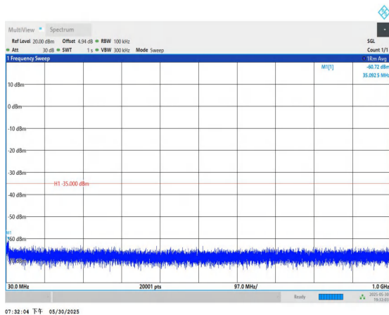
Band7-5MHz-16QAM-20775-1RB#0-30~1000-PASS
