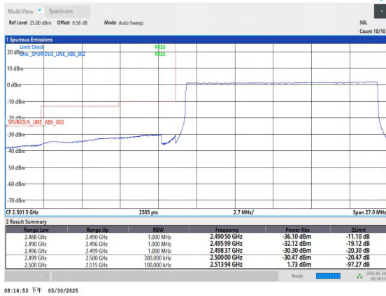
Band7-15MHz-16QAM-20825-75RB#0-PASS
