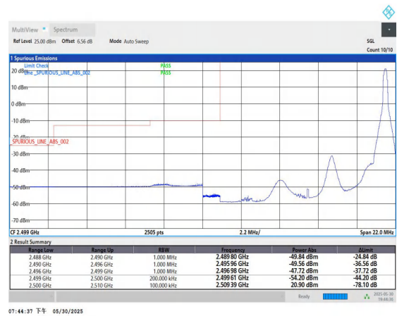
Band7-10MHz-16QAM-20800-1RB#49-PASS
