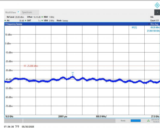
Band7-5MHz-16QAM-21425-1RB#0-18000~27000-PASS
