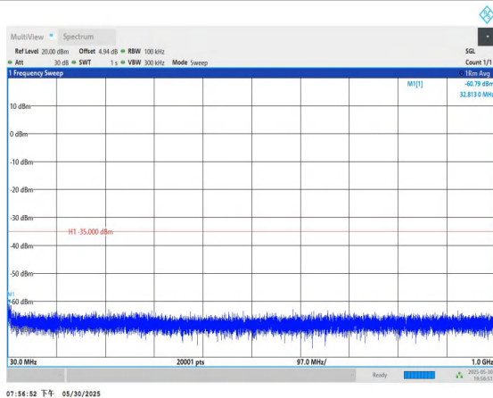
Band7-10MHz-16QAM-21100-1RB#0-30~1000-PASS
