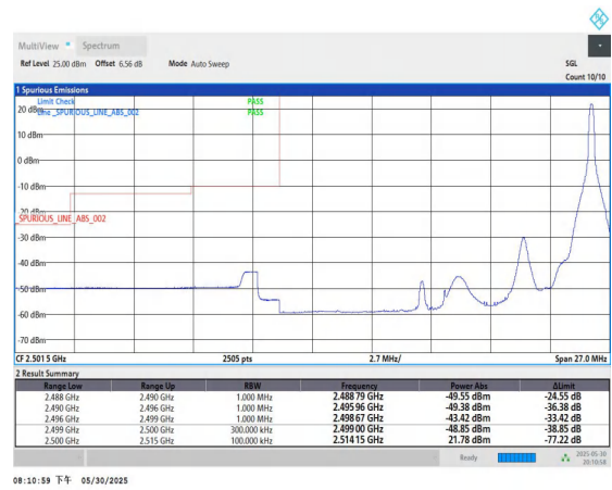
Band7-15MHz-QPSK-20825-1RB#74-PASS
