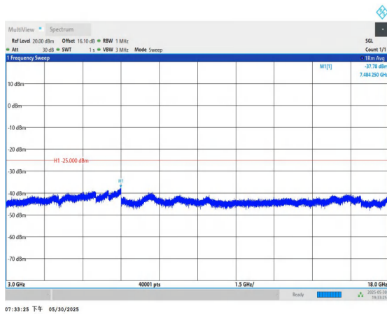
Band7-5MHz-16QAM-21100-1RB#0-3000~18000-PASS
