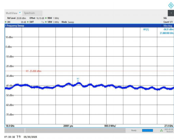
Band7-5MHz-16QAM-21100-1RB#0-18000~27000-PASS
