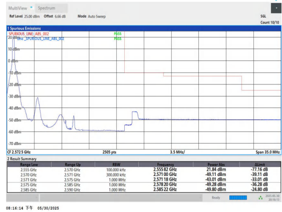
Band7-15MHz-QPSK-21375-1RB#0-PASS
