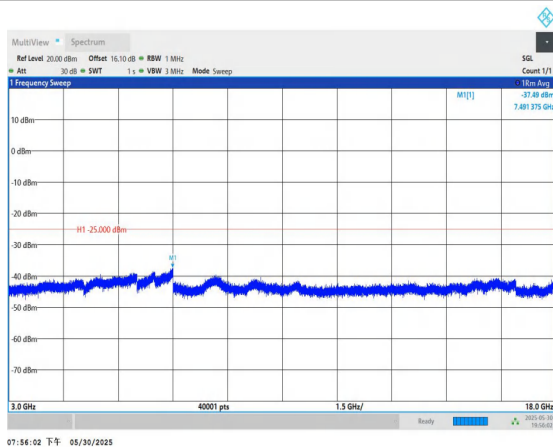
Band7-10MHz-16QAM-20800-1RB#0-3000~18000-PASS
