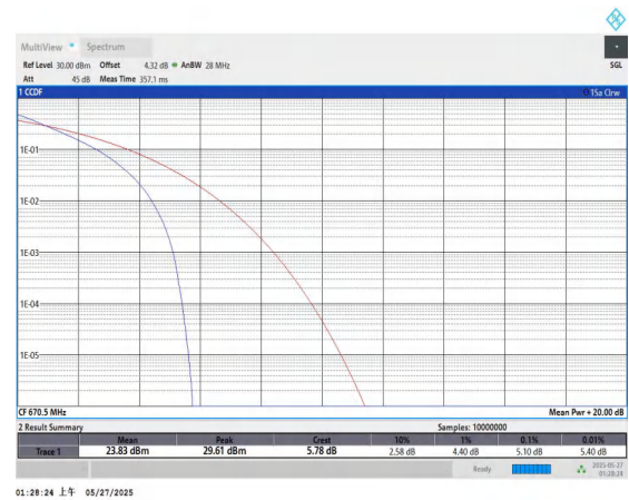
Band71-15MHz-QPSK-133197-75RB#0-PASS
