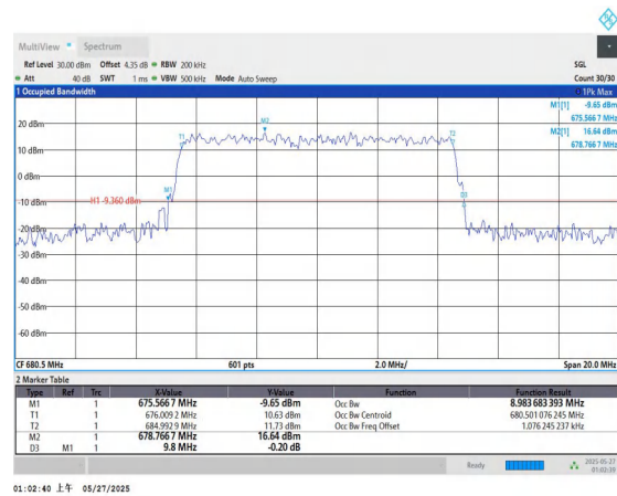
Band71-10MHz-QPSK-133297-50RB#0-PASS
