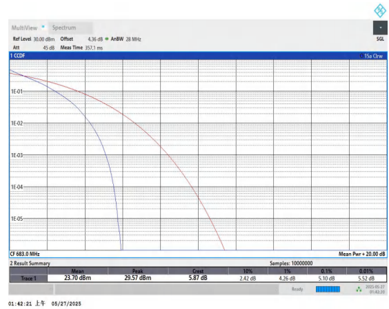
Band71-20MHz-QPSK-133322-100RB#0-PASS
