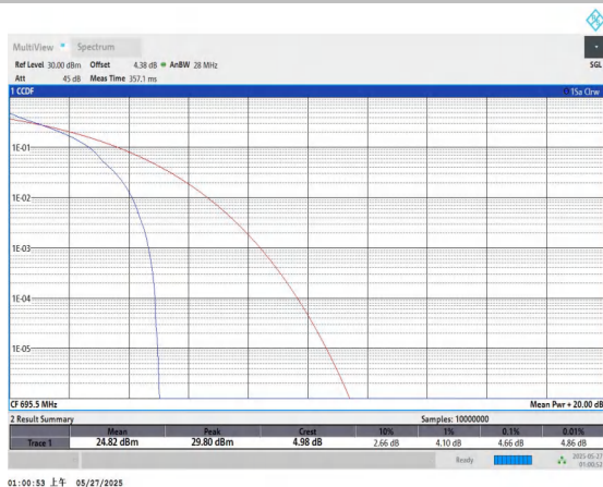
Band71-5MHz-QPSK-133447-1RB#0-PASS
