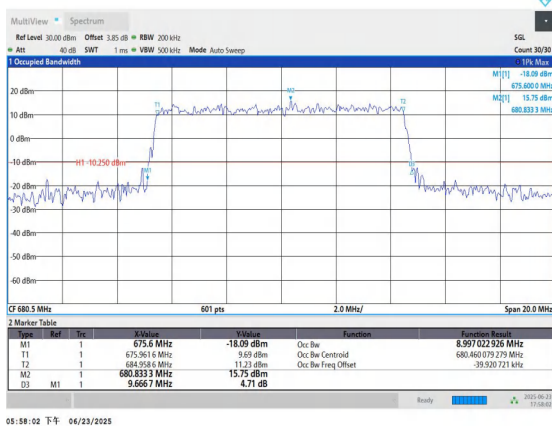
Band71-10MHz-16QAM-133297-50RB#0-PASS
