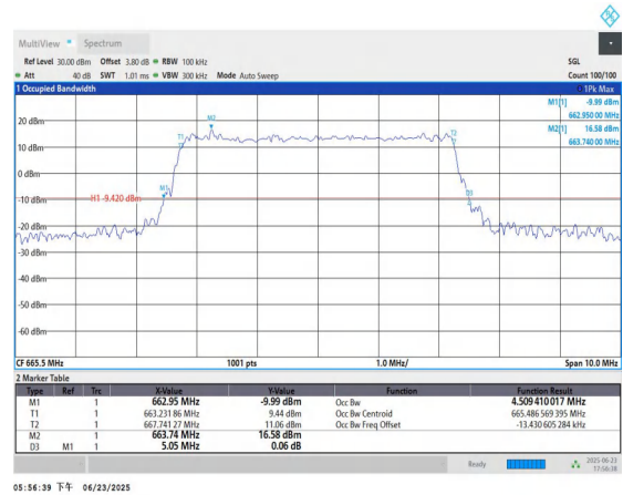
Band71-5MHz-16QAM-133147-25RB#0-PASS
