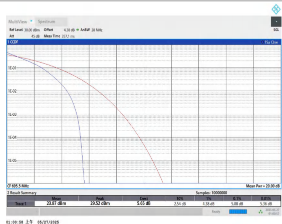
Band71-5MHz-QPSK-133447-25RB#0-PASS
