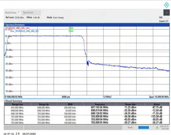
Band71-5MHz-QPSK-133447-25RB#0-PASS
