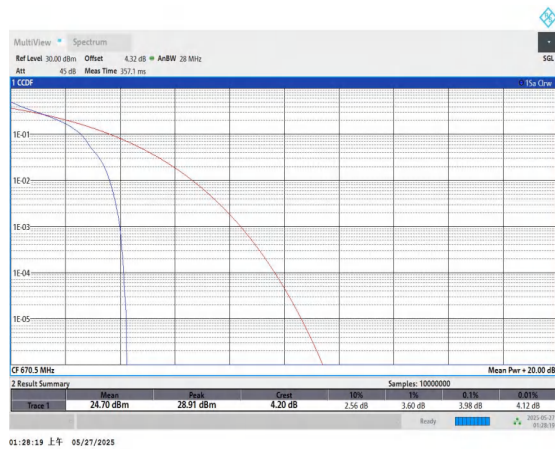
Band71-15MHz-QPSK-133197-1RB#0-PASS
