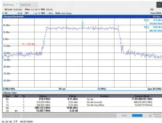
Band71-20MHz-QPSK-133372-100RB#0-PASS
