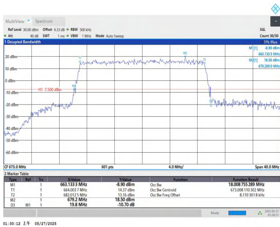
Band71-20MHz-QPSK-133222-100RB#0-PASS
