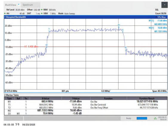
Band71-20MHz-16QAM-133222-100RB#0-PASS
