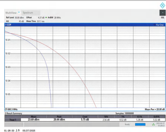
Band71-15MHz-QPSK-133397-75RB#0-PASS
