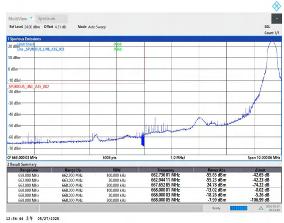
Band71-5MHz-QPSK-133147-1RB#24-PASS
