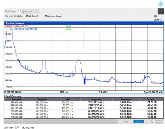
Band71-5MHz-QPSK-133447-1RB#0-PASS
