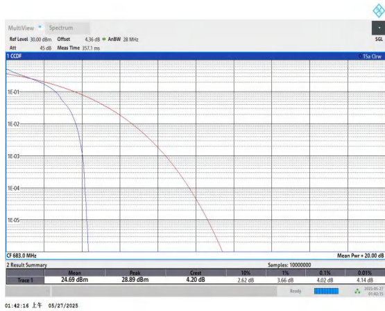
Band71-20MHz-QPSK-133322-1RB#0-PASS
