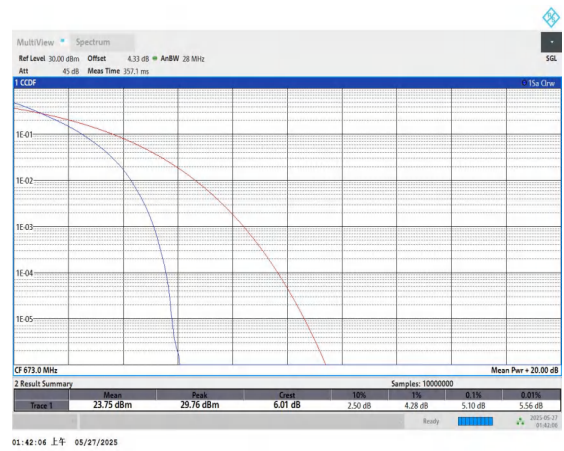
Band71-20MHz-QPSK-133222-100RB#0-PASS
