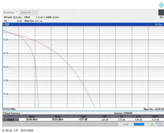
Band71-20MHz-QPSK-133222-1RB#0-PASS
