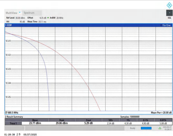
Band71-15MHz-QPSK-133297-75RB#0-PASS
