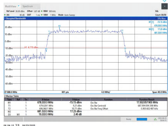
Band71-20MHz-16QAM-133372-100RB#0-PASS
