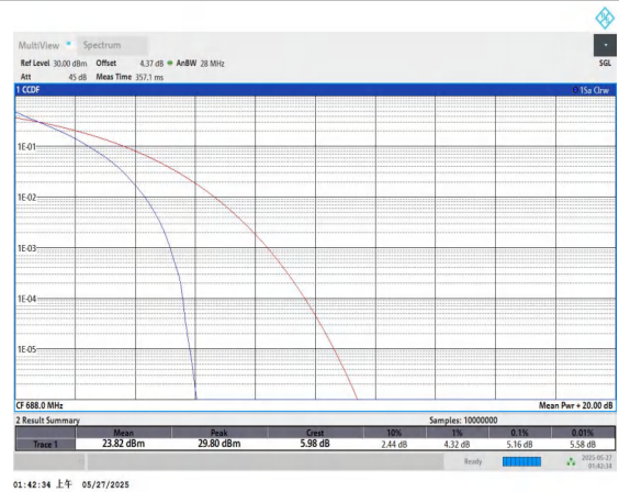
Band71-20MHz-QPSK-133372-100RB#0-PASS
