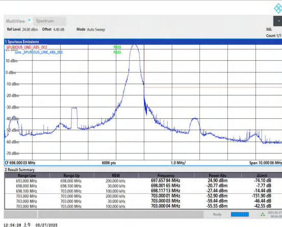
Band71-5MHz-QPSK-133447-1RB#24-PASS
