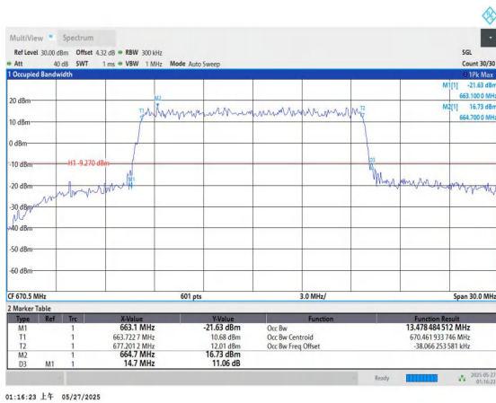
Band71-15MHz-QPSK-133197-75RB#0-PASS
