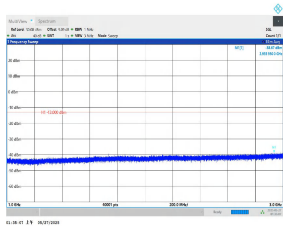
Band71-20MHz-QPSK-133322-1RB#0-1000~3000-PASS
