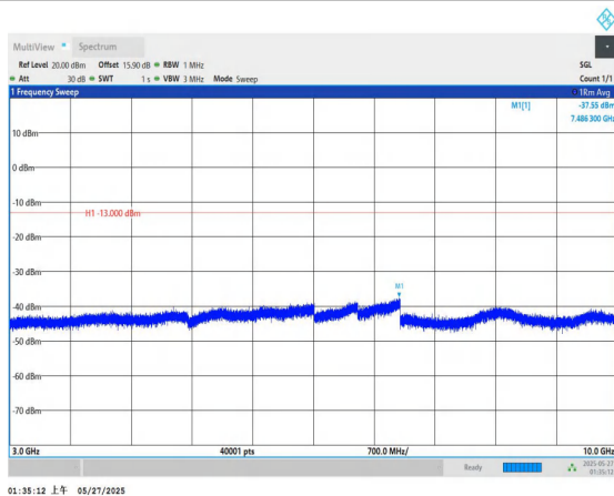
Band71-20MHz-QPSK-133322-1RB#0-3000~10000-PASS
