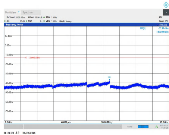
Band71-15MHz-QPSK-133297-1RB#0-3000~10000-PASS
