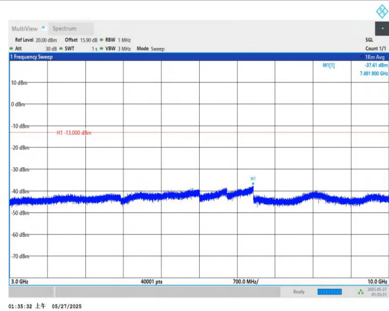
Band71-20MHz-QPSK-133372-1RB#0-3000~10000-PASS
