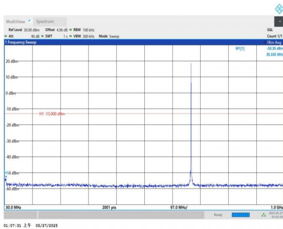
Band71-10MHz-QPSK-133297-1RB#0-30~1000-PASS
