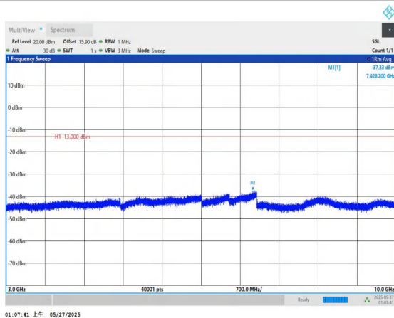
Band71-10MHz-QPSK-133297-1RB#0-3000~10000-PASS
