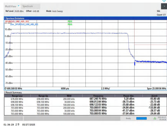
Band71-20MHz-QPSK-133372-100RB#0-PASS
