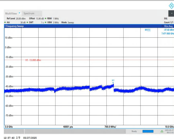
Band71-5MHz-QPSK-133297-1RB#0-3000~10000-PASS
