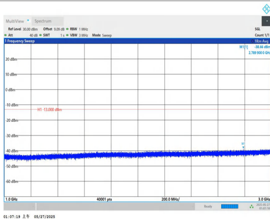
Band71-10MHz-QPSK-133172-1RB#0-1000~3000-PASS
