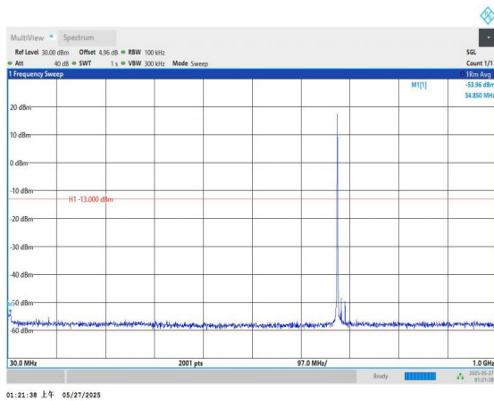
Band71-15MHz-QPSK-133397-1RB#0-30~1000-PASS
