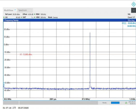
Band71-10MHz-QPSK-133172-1RB#0-30~1000-PASS
