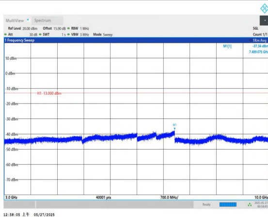
Band71-5MHz-QPSK-133447-1RB#0-3000~10000-PASS
