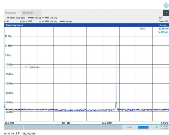
Band71-10MHz-QPSK-133422-1RB#0-30~1000-PASS
