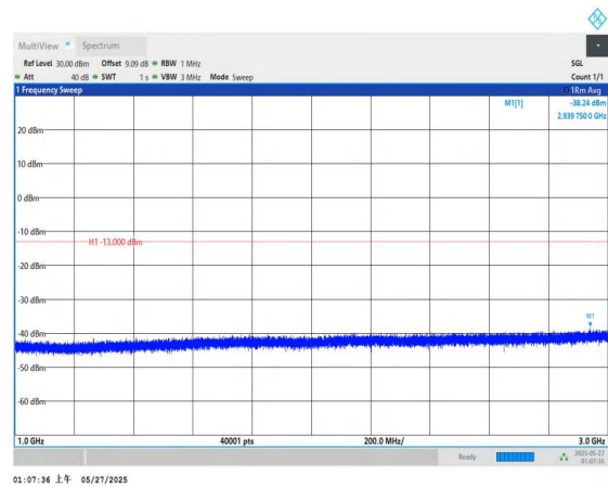
Band71-10MHz-QPSK-133297-1RB#0-1000~3000-PASS
