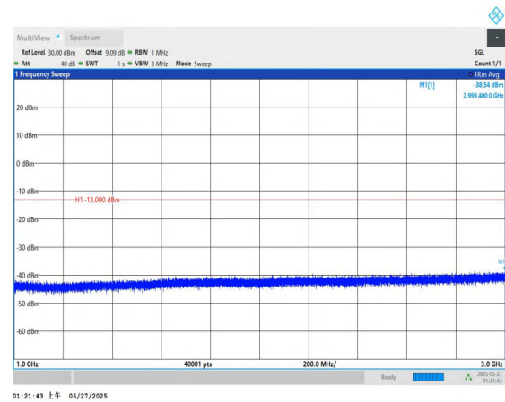
Band71-15MHz-QPSK-133397-1RB#0-1000~3000-PASS
