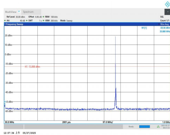
Band71-5MHz-QPSK-133297-1RB#0-30~1000-PASS
