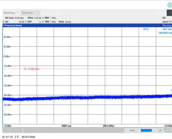
Band71-10MHz-QPSK-133422-1RB#0-1000~3000-PASS
