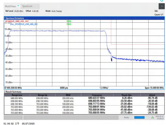
Band71-10MHz-QPSK-133422-50RB#0-PASS
