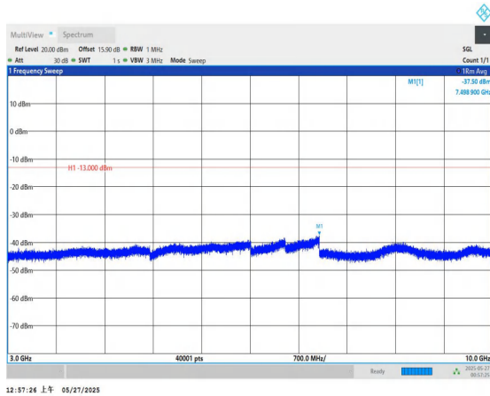
Band71-5MHz-QPSK-133147-1RB#0-3000~10000-PASS
