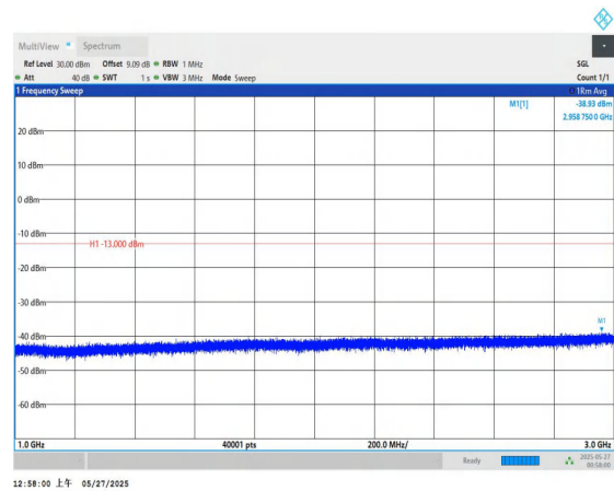
Band71-5MHz-QPSK-133447-1RB#0-1000~3000-PASS
