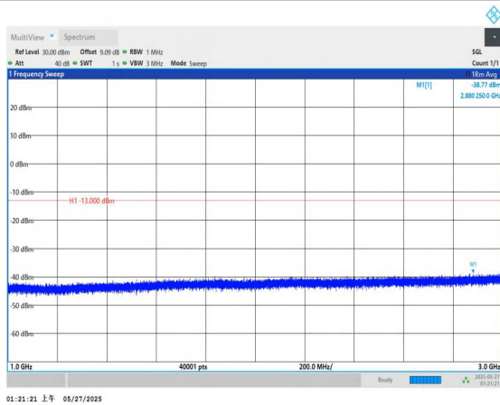
Band71-15MHz-QPSK-133297-1RB#0-1000~3000-PASS
