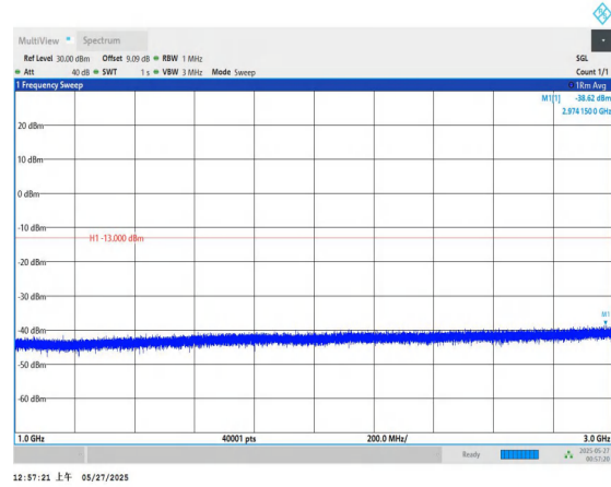
Band71-5MHz-QPSK-133147-1RB#0-1000~3000-PASS
