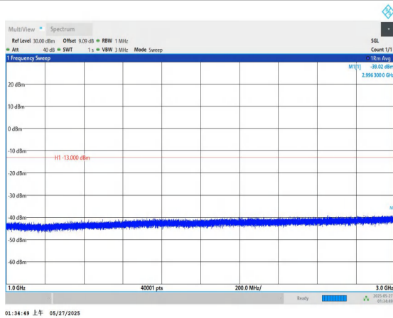
Band71-20MHz-QPSK-133222-1RB#0-1000~3000-PASS
