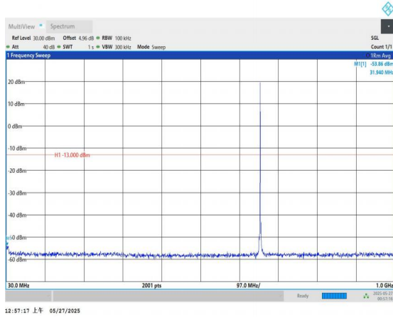
Band71-5MHz-QPSK-133147-1RB#0-30~1000-PASS
