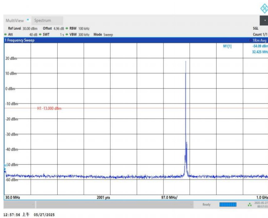
Band71-5MHz-QPSK-133447-1RB#0-30~1000-PASS
