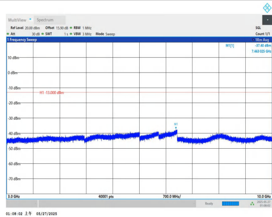
Band71-10MHz-QPSK-133422-1RB#0-3000~10000-PASS
