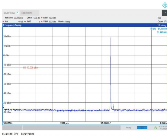
Band71-15MHz-QPSK-133197-1RB#0-30~1000-PASS
