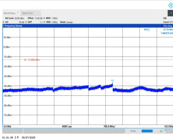
Band71-15MHz-QPSK-133197-1RB#0-3000~10000-PASS
