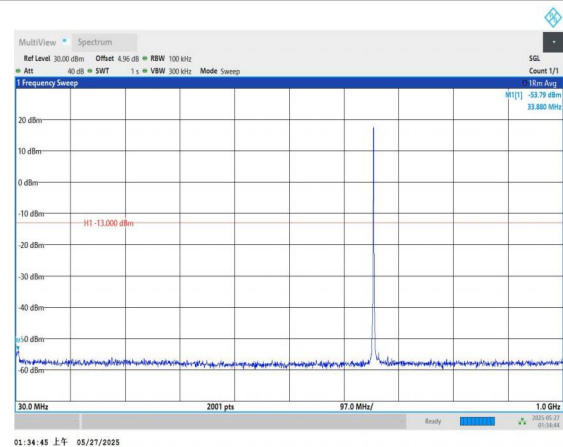
Band71-20MHz-QPSK-133222-1RB#0-30~1000-PASS
