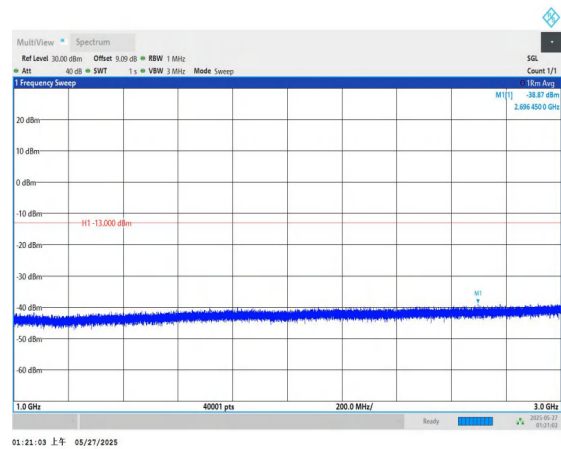
Band71-15MHz-QPSK-133197-1RB#0-1000~3000-PASS
