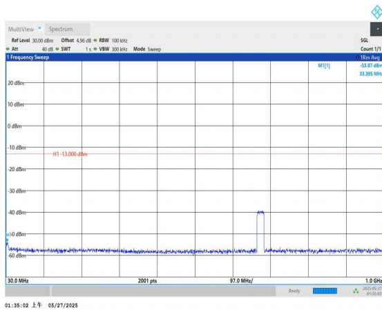
Band71-20MHz-QPSK-133322-1RB#0-30~1000-PASS
