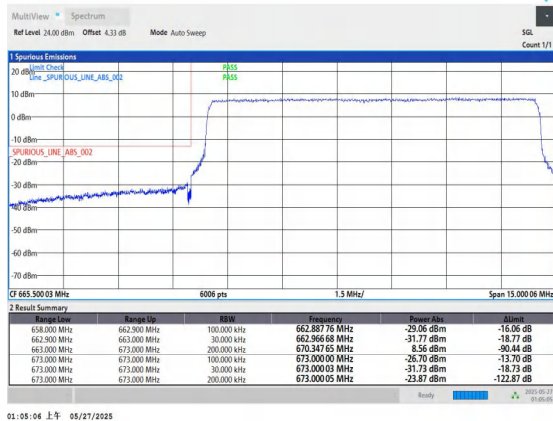
Band71-10MHz-QPSK-133172-50RB#0-PASS
