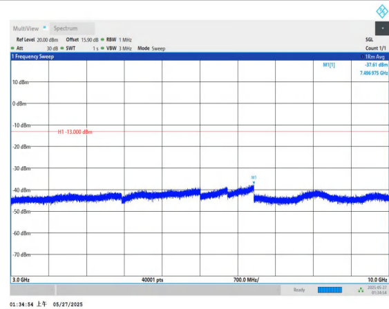
Band71-20MHz-QPSK-133222-1RB#0-3000~10000-PASS
