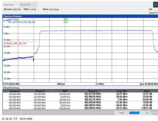
Band71-20MHz-QPSK-133222-100RB#0-PASS
