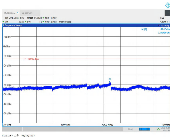
Band71-15MHz-QPSK-133397-1RB#0-3000~10000-PASS
