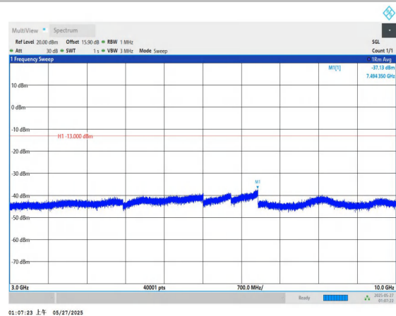
Band71-10MHz-QPSK-133172-1RB#0-3000~10000-PASS
