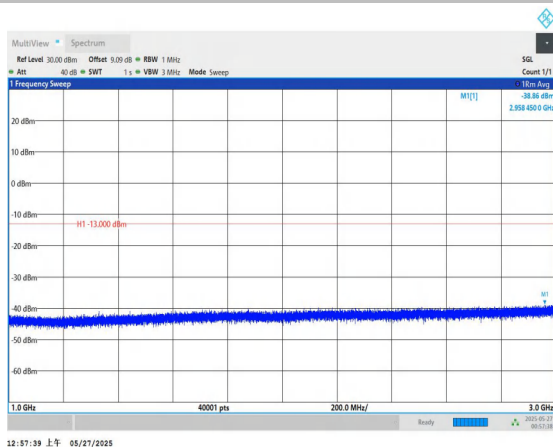
Band71-5MHz-QPSK-133297-1RB#0-1000~3000-PASS
