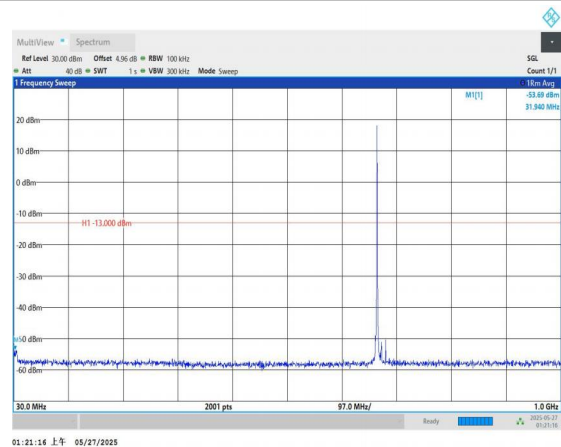
Band71-15MHz-QPSK-133297-1RB#0-30~1000-PASS
