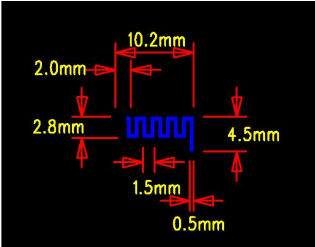
Antenna Photo & Length (mm)
