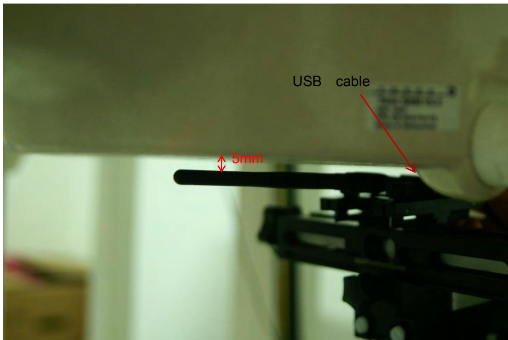
Horizontal-Down-1(5mm separation)
