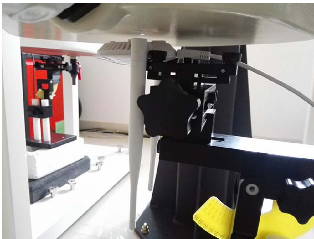
Horizontal Up Position with the antennas bent at 90 degrees perpendicular to the phantom (antennas pointing down and away from the phantom) Setup Photo
