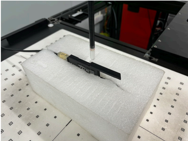
Photo 21: Power Density_2mm_Right Side _Ant angle 180°_Ant Main+Aux
