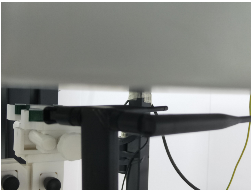
10mm body Vertical-Back Side Setup Photo – Test Position 1
