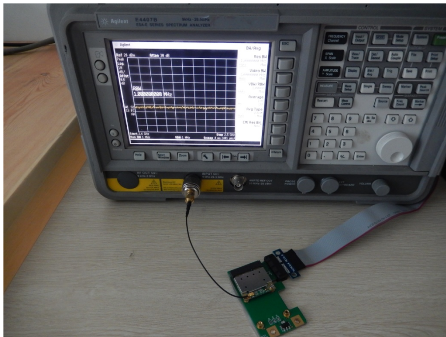
DTS RF conduction test photos
