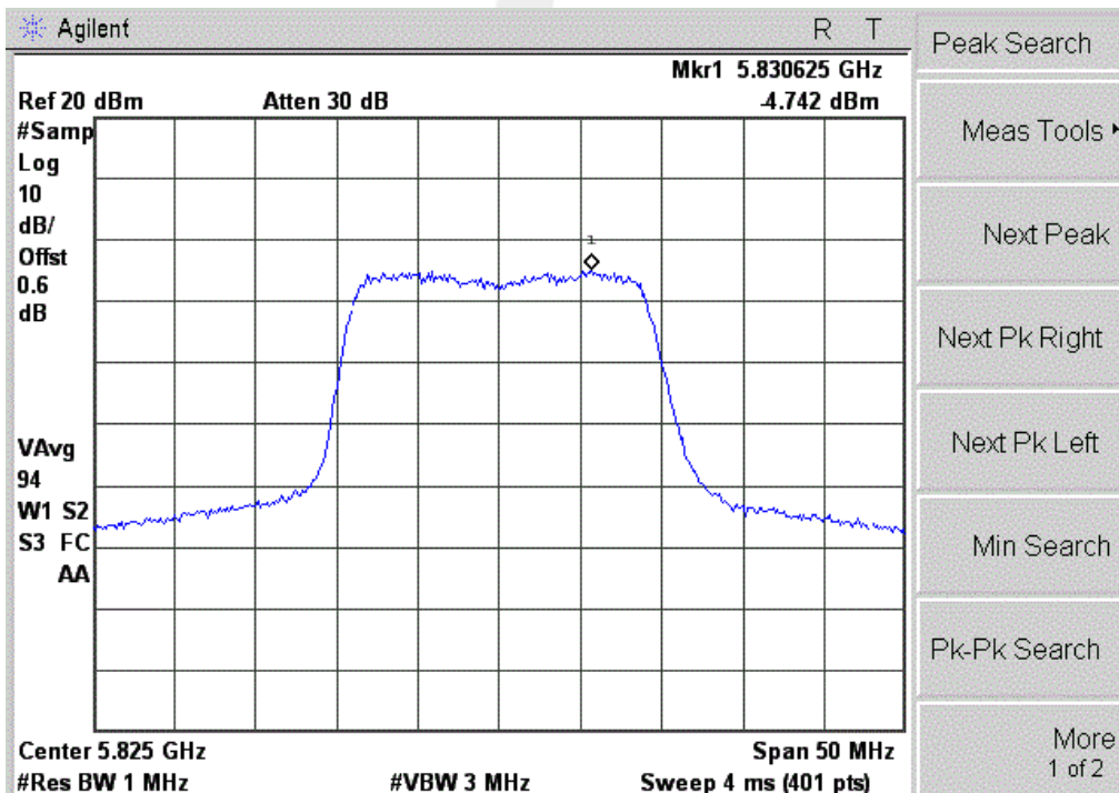
PSD Plot on 802.11n Channel 165
