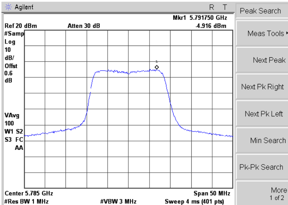
PSD Plot on 802.11a Channel 157
