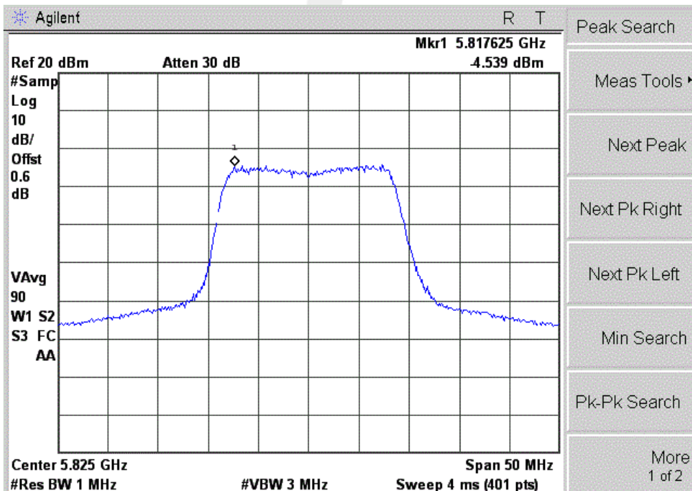
PSD Plot on 802.11a Channel 165
