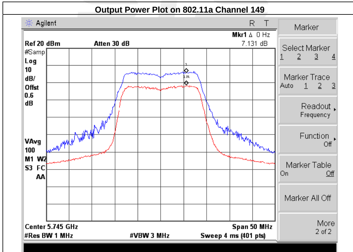
Plot on 802.11a
