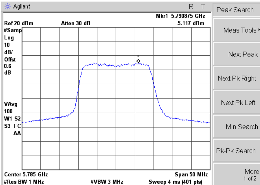
PSD Plot on 802.11n Channel 157
