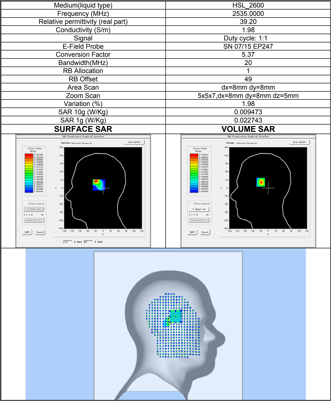
Plot 14:LTE BAND7, Middle channel (Left Head Cheek) Product Description:Smart phone Test Date: 2019-05-31
