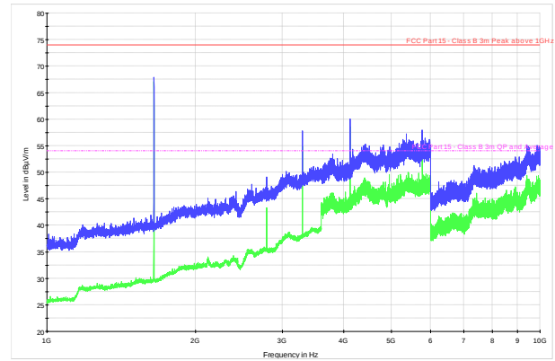
Figure 8.1-2: Radiated spurious emissions, OB protocol @ mid channel / GSM850@ ch128
