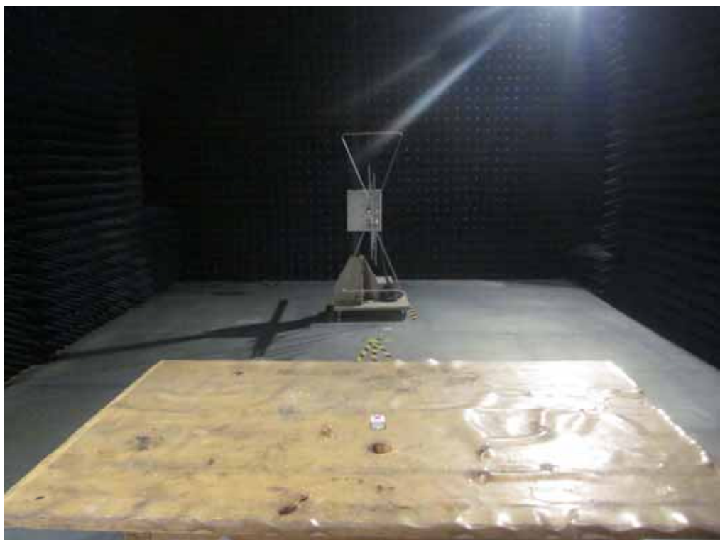
Test frequency from 30MHz to 1GHz Test Site 1#
