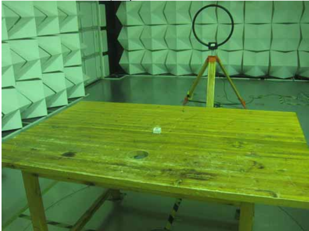
Test frequency below 30MHz Test Site 2#
