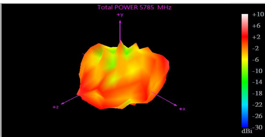
5785 MHz
