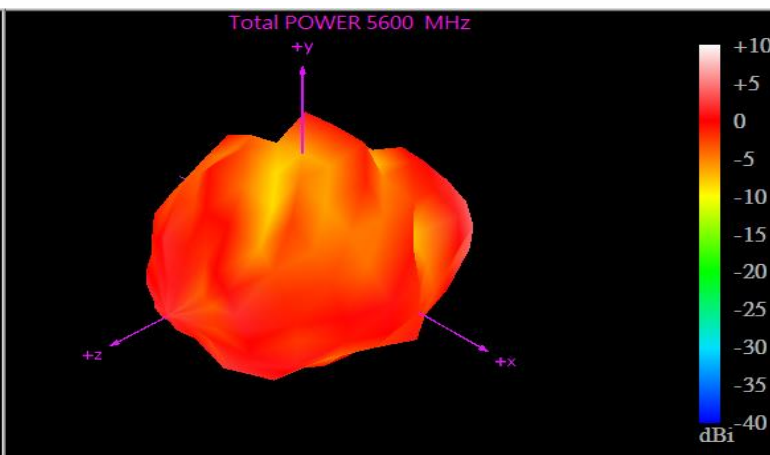
5600 MHz
