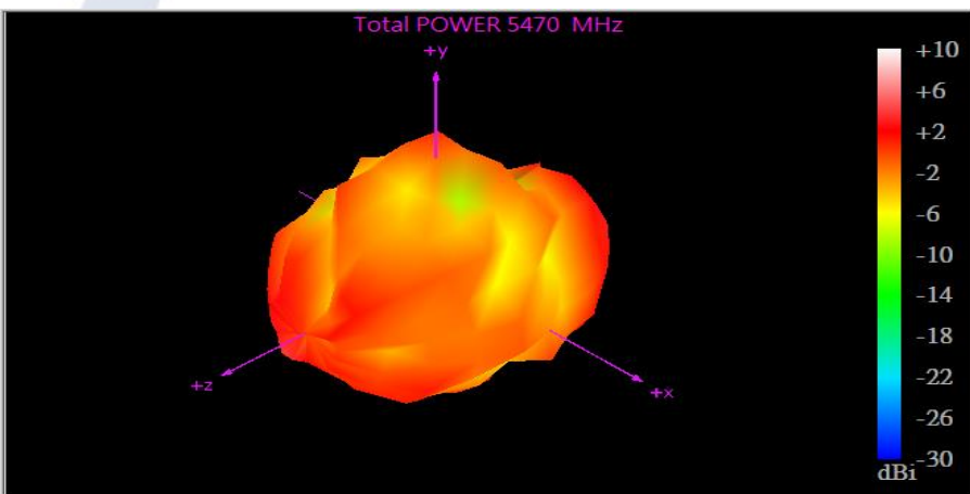
5470 MHz
