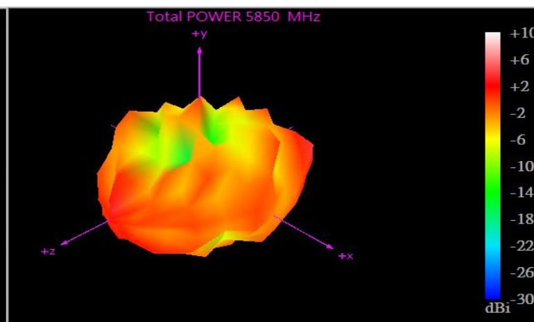
5850 MHz
