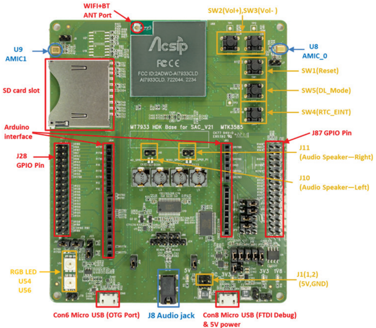
Figure 2. Jumpers and connectors on the EK-AI7933ALD
