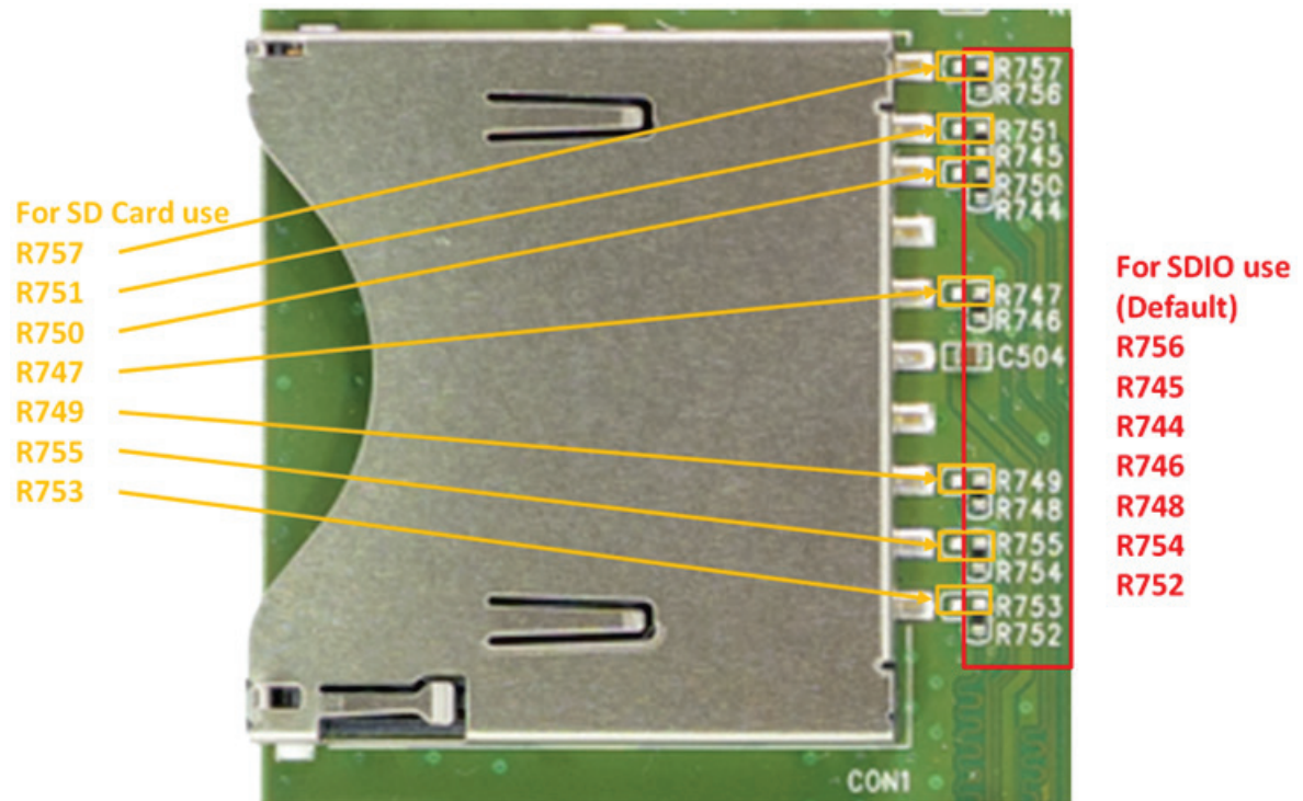
Figure 8. SD card slot rework
