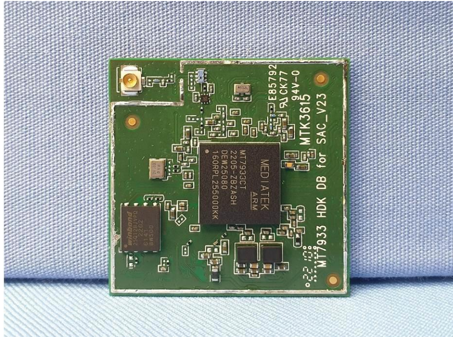
EUT Photo (1)
