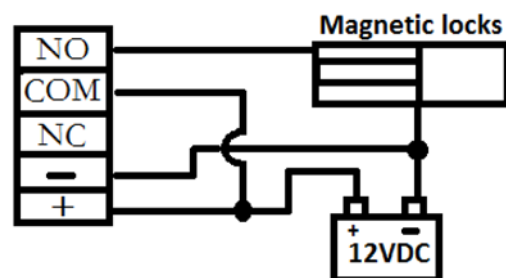
Typical N.O. Application
