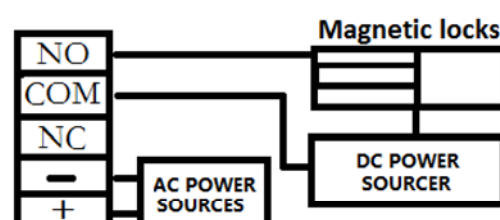
N.O.Application with Independent Power Sources
