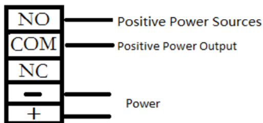
Positive Output
