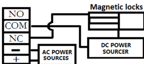
N.C.Application with Independent Power Sources
