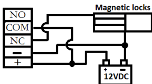
Typical N.C. Application
