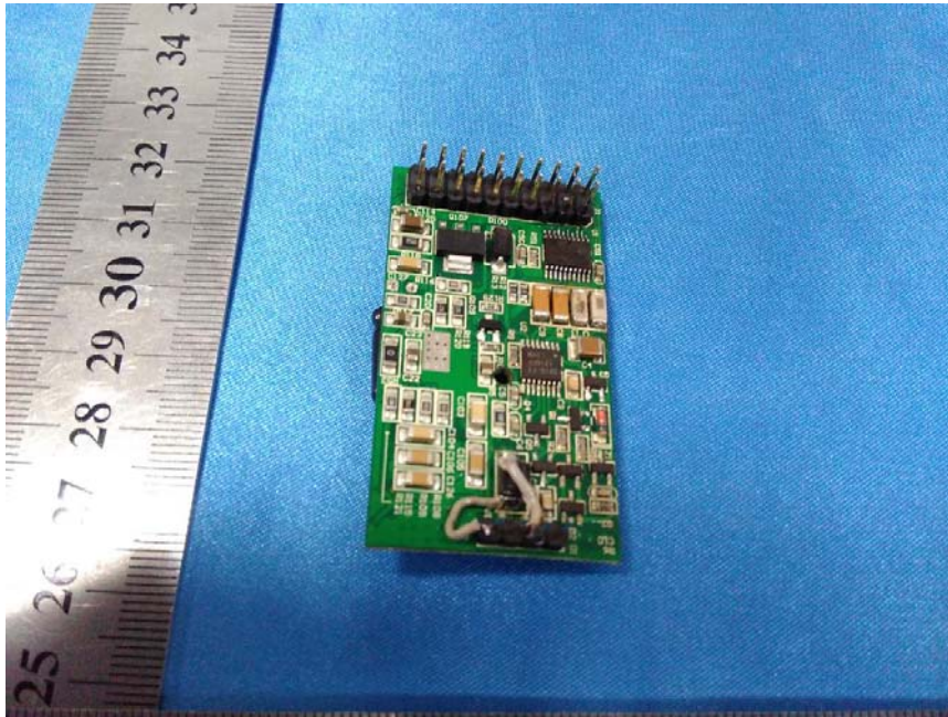
EUT – Module Bottom View
