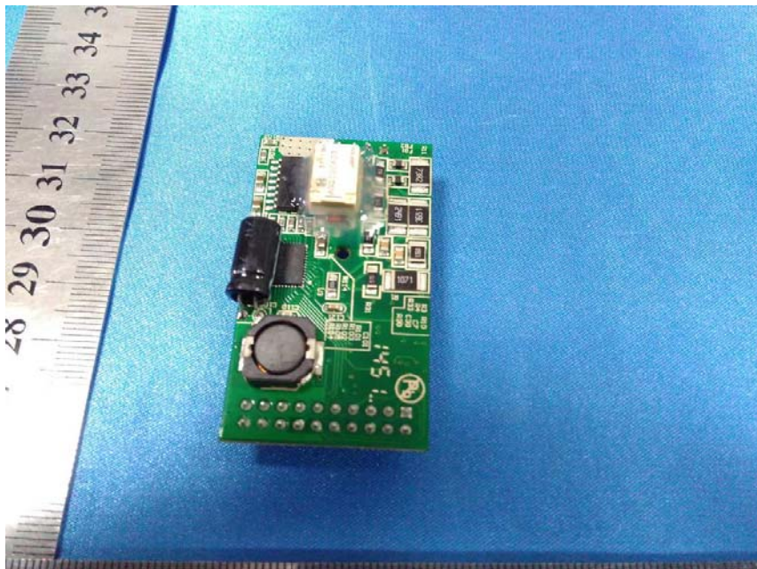
EUT – Module Top View
