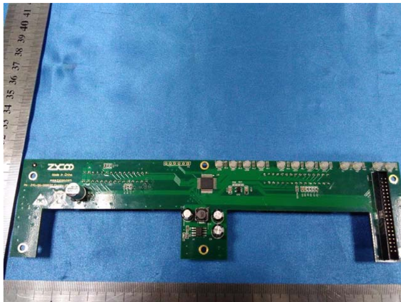
EUT – LED Board Top View
