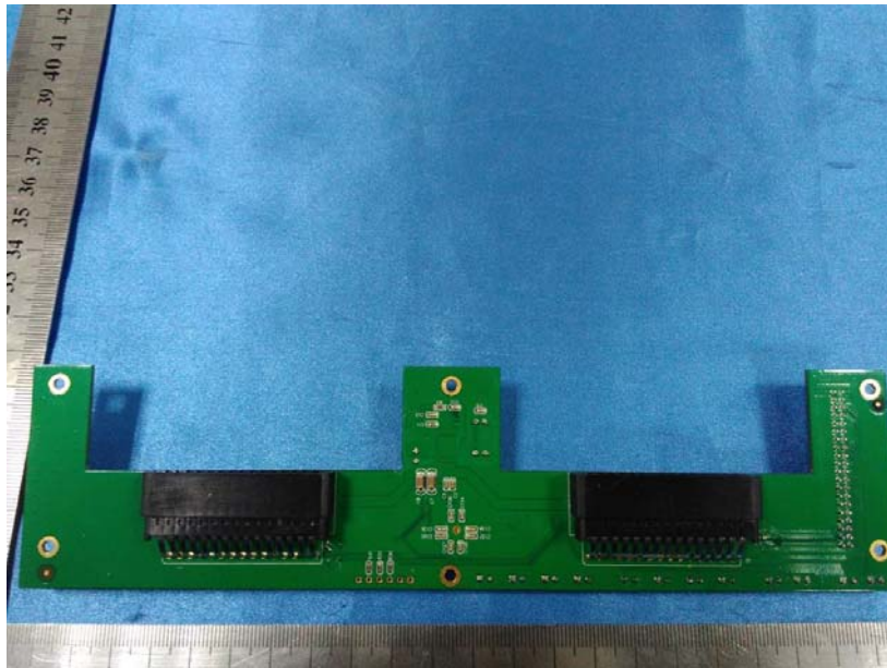
EUT – LED Board Bottom View
