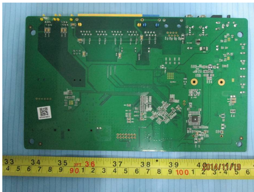
EUT – Main Board Bottom 1 View
