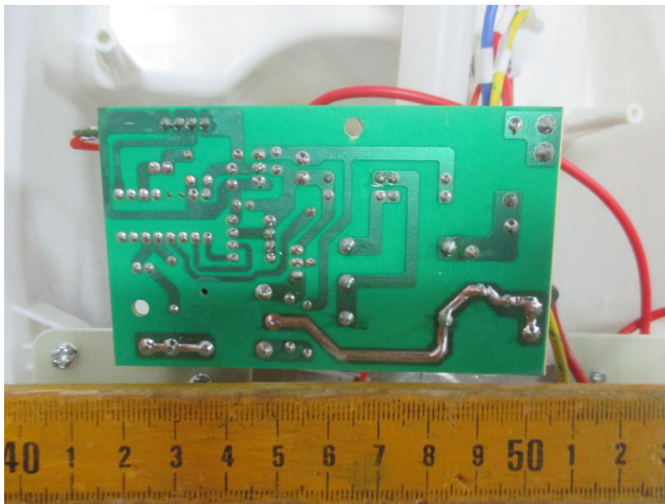
(11) Power Board Back
