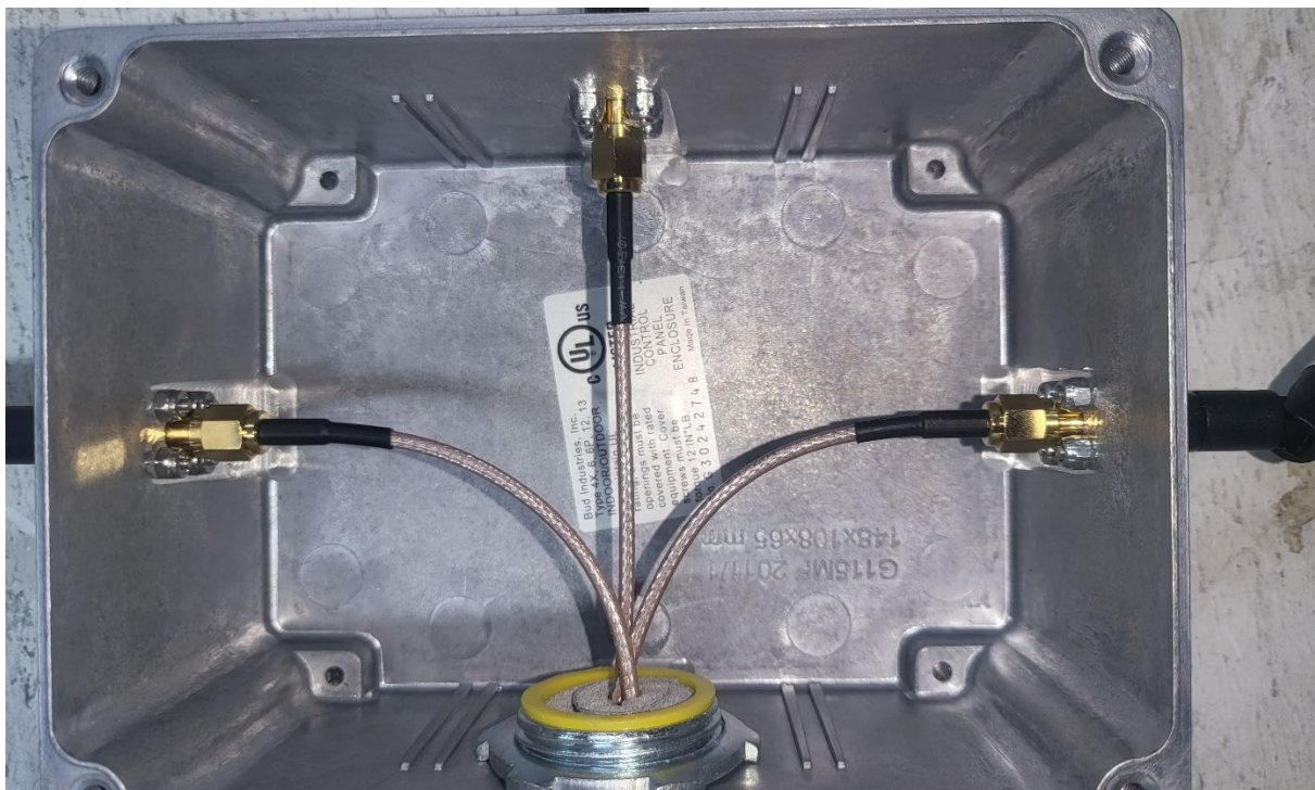
Figure 8. Antenna Enclosure - Lid Removed
