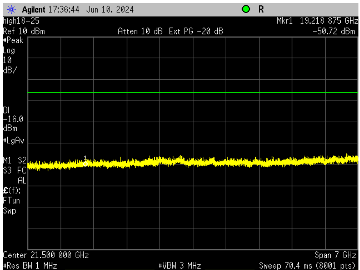
Figure 14. Radio 1, High, 18-25 GHz
