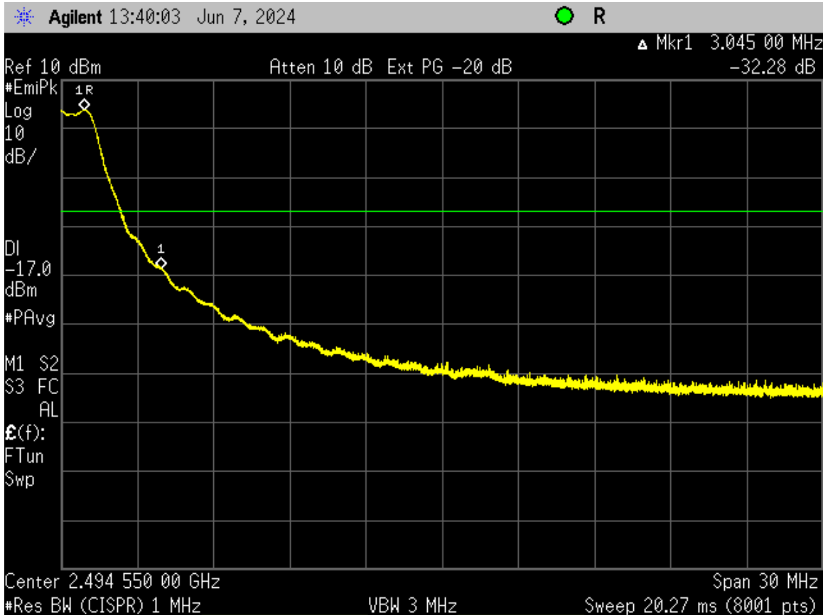
Figure 51. Band Edge Compliance – Radio 3 High Channel Delta – Peak
