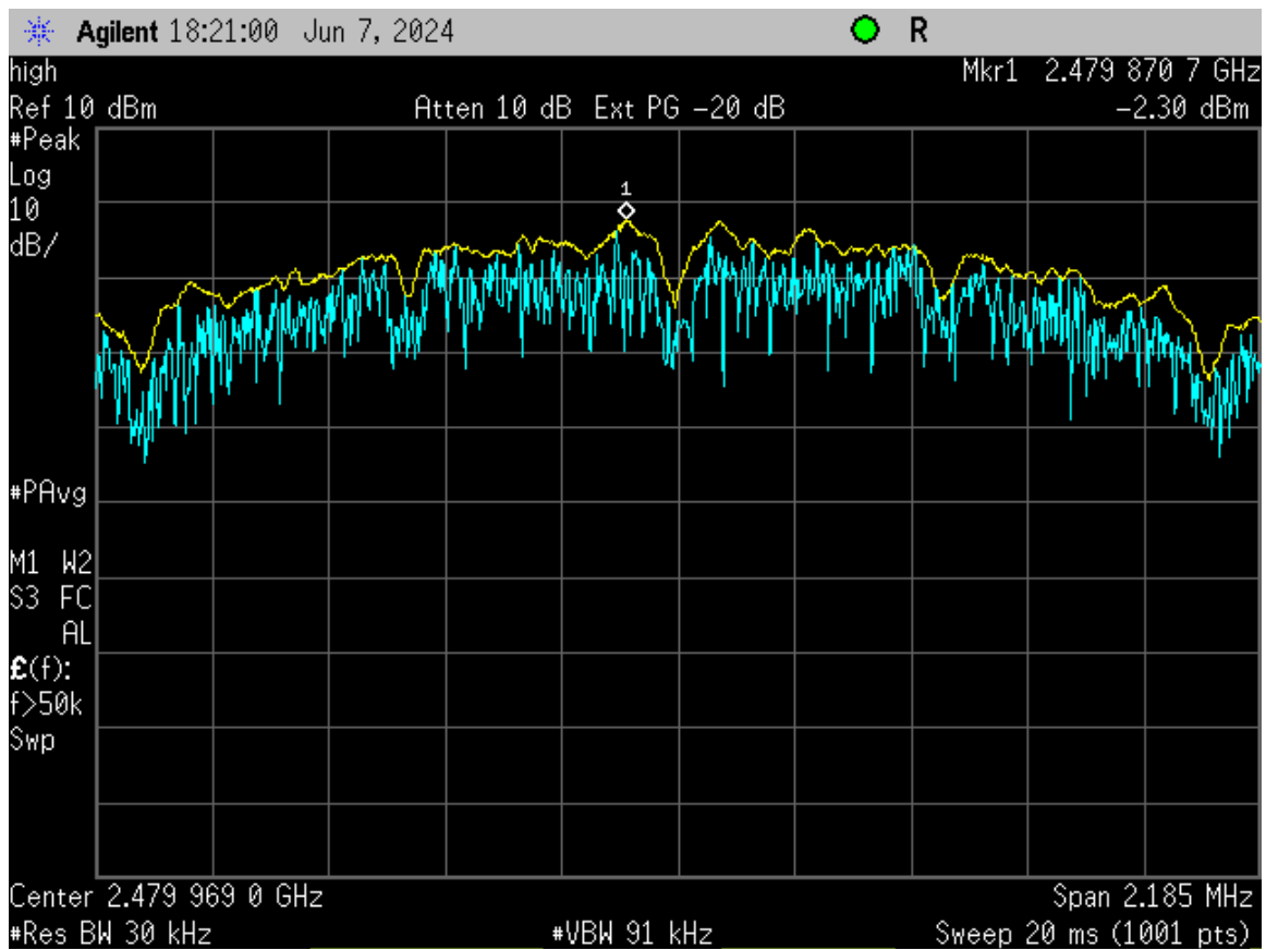
Figure 89. Power Spectral Density, Radio 2 High Channel
