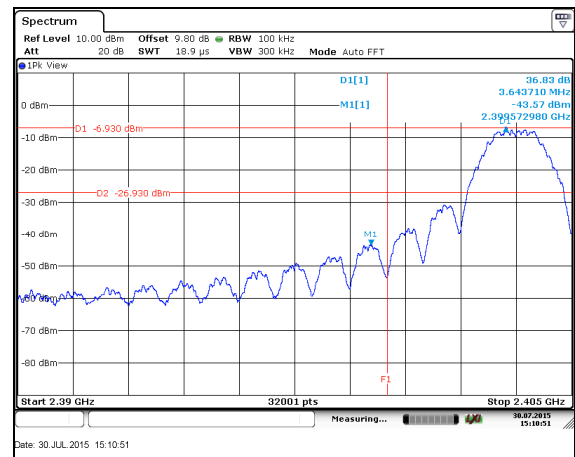
Figure 7.5.1.2-9: Lower Band-edge – Radio 2 - LCH
