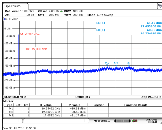
Figure 7.5.1.2-1: 30 MHz – 25 GHz – Radio 1 - LCH
