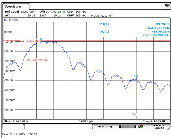
Figure 7.5.1.2-10: Upper Band-edge – Radio 2- HCH
