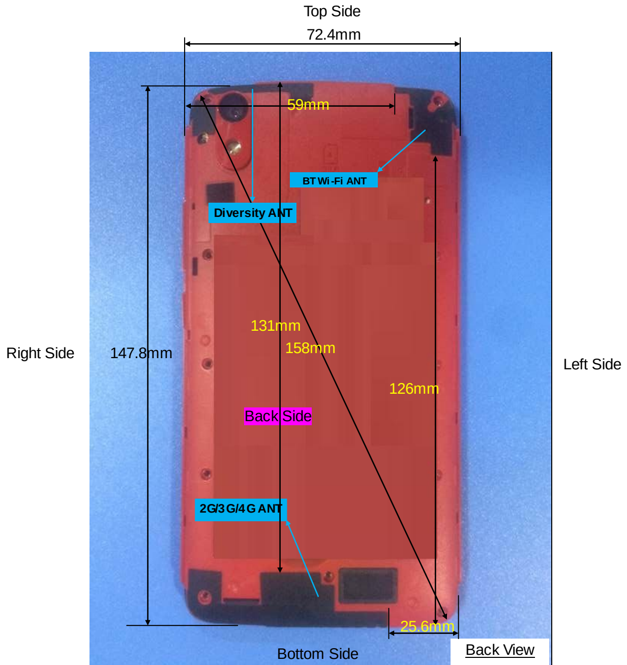
Distance of the Antenna to the EUT surface/edge
