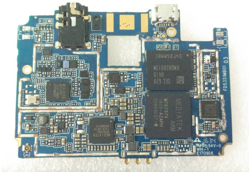
EUT – IC Chip View
