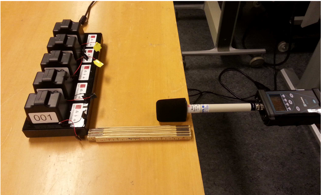
E-Field Measurement, Front Position
