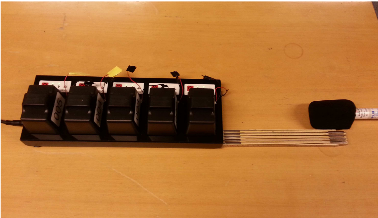
E-Field Measurement, Left Position
