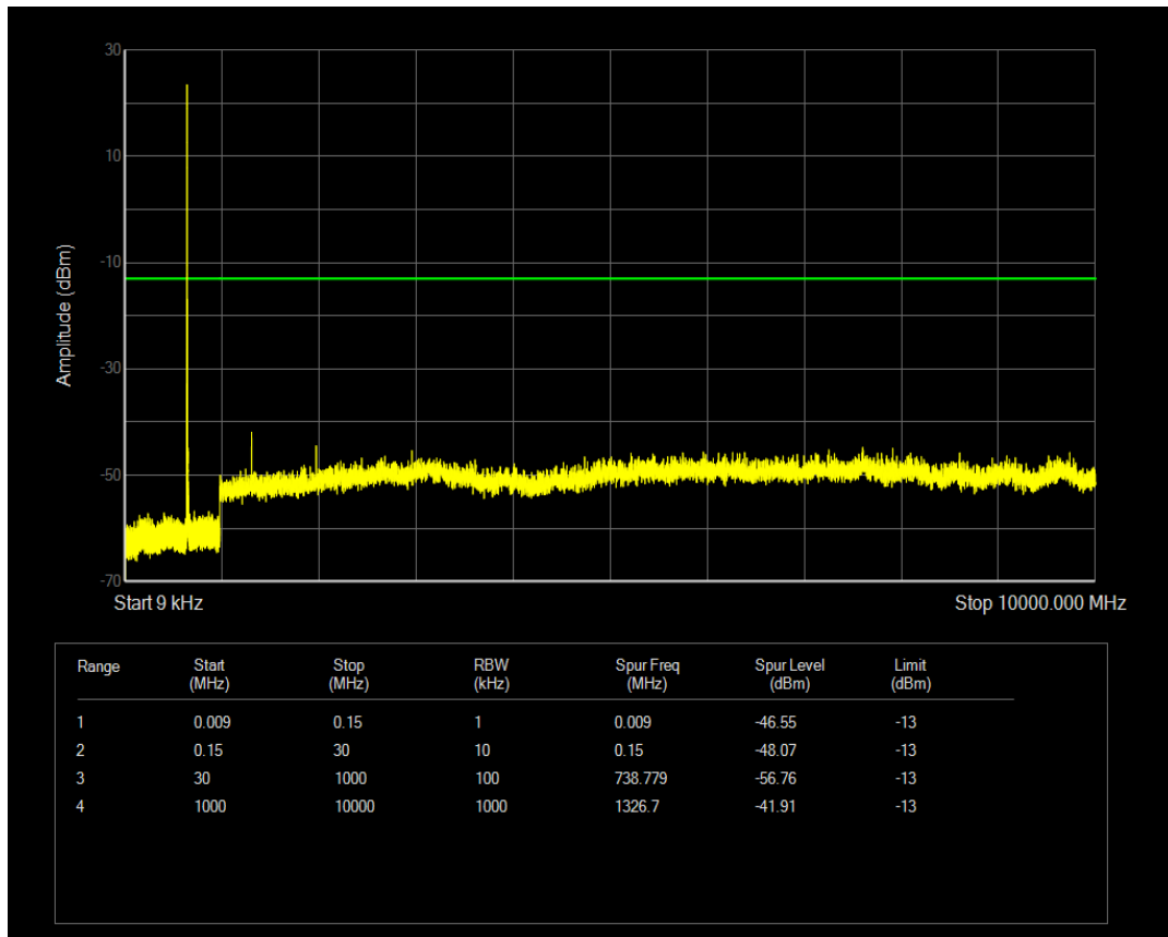
Band71 QAM16 BW=20MHz Channel=133372 RB Size=100 Position=#0
