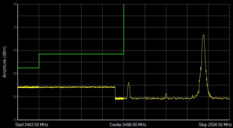
Band41 QPSK BW=10MHz Channel=39700 RB Size=1 Position=#Max
