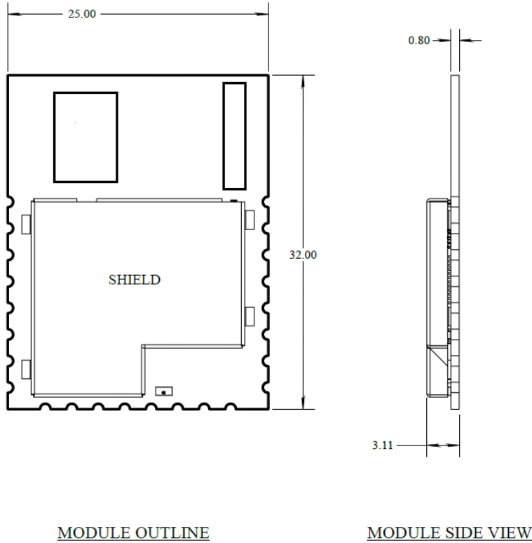
FIGURE 7. DIMENSION OF RTLS MODULE
